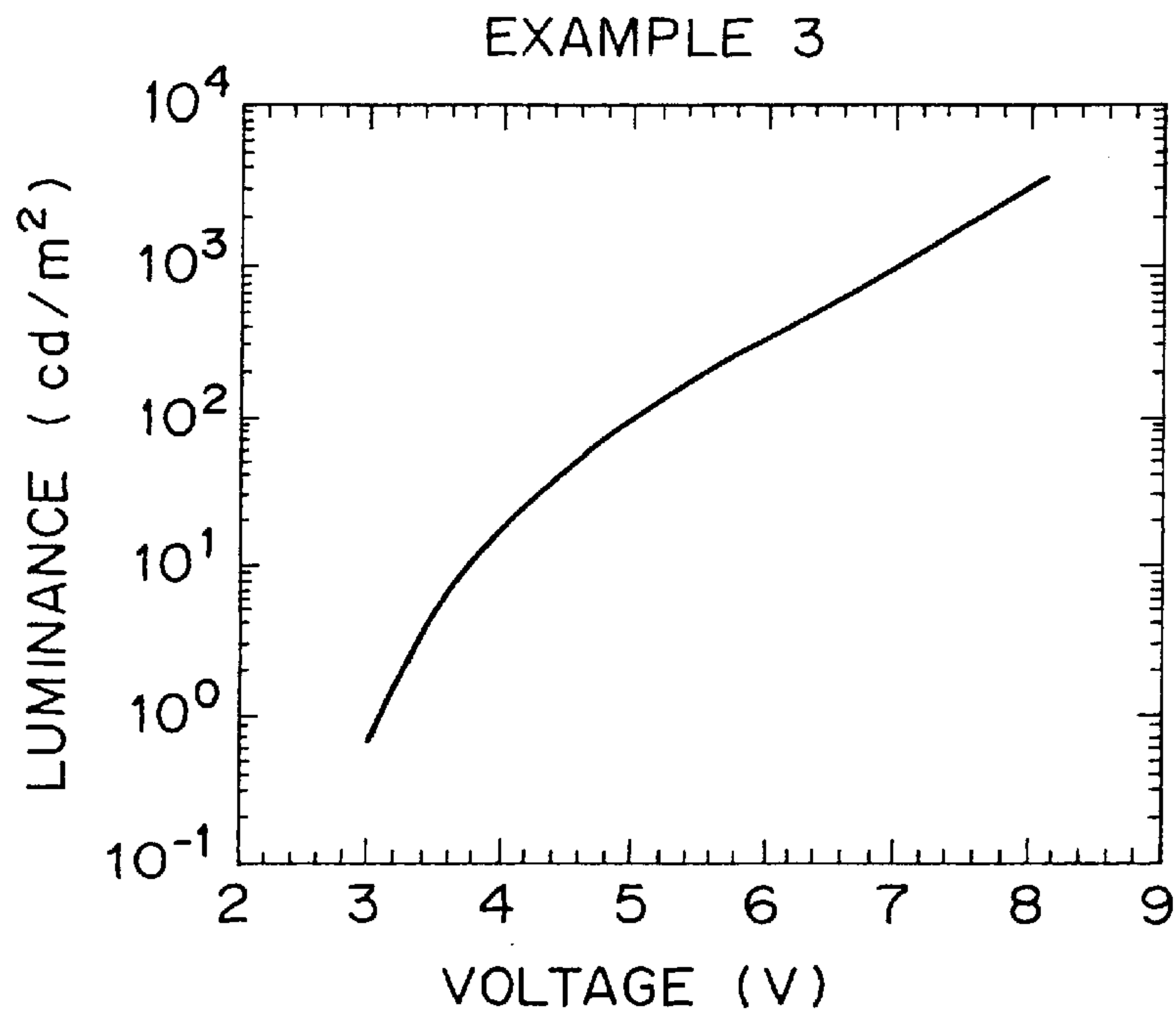
VOLTAGE - LUMINANCE CHARACTERISTIC
