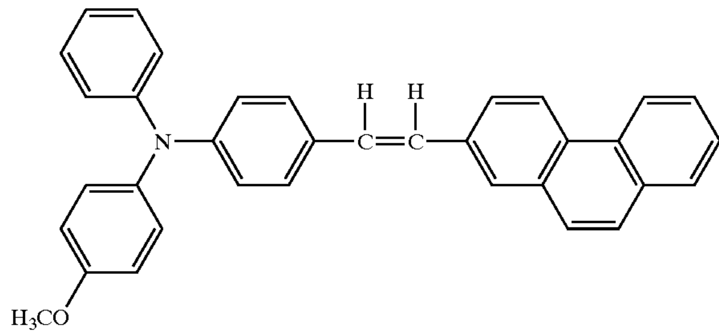
Structural Formula (20)-14:
