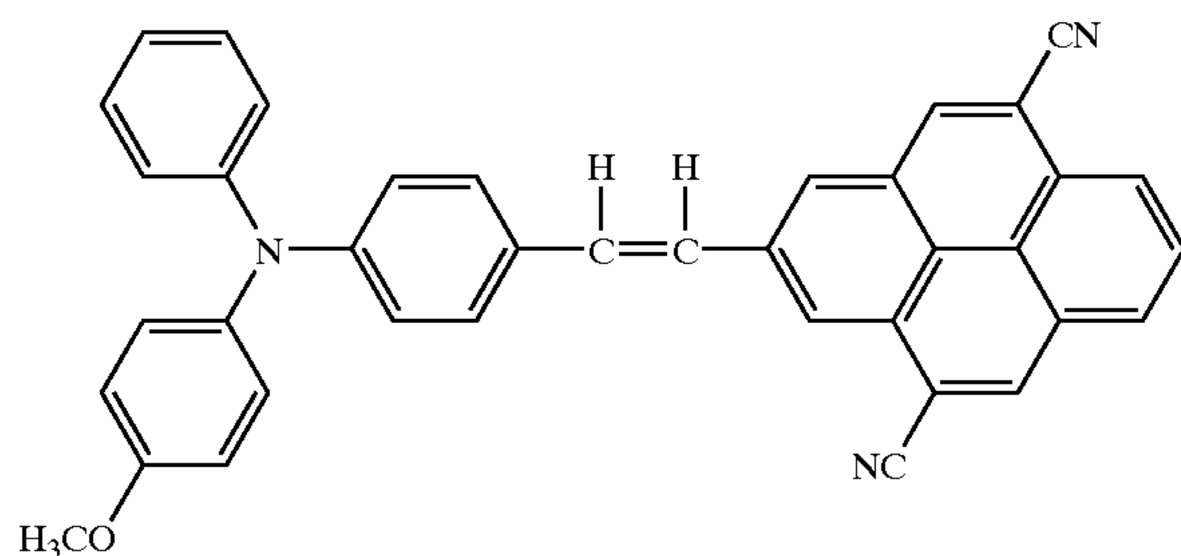
Structural Formula (20)-17:
