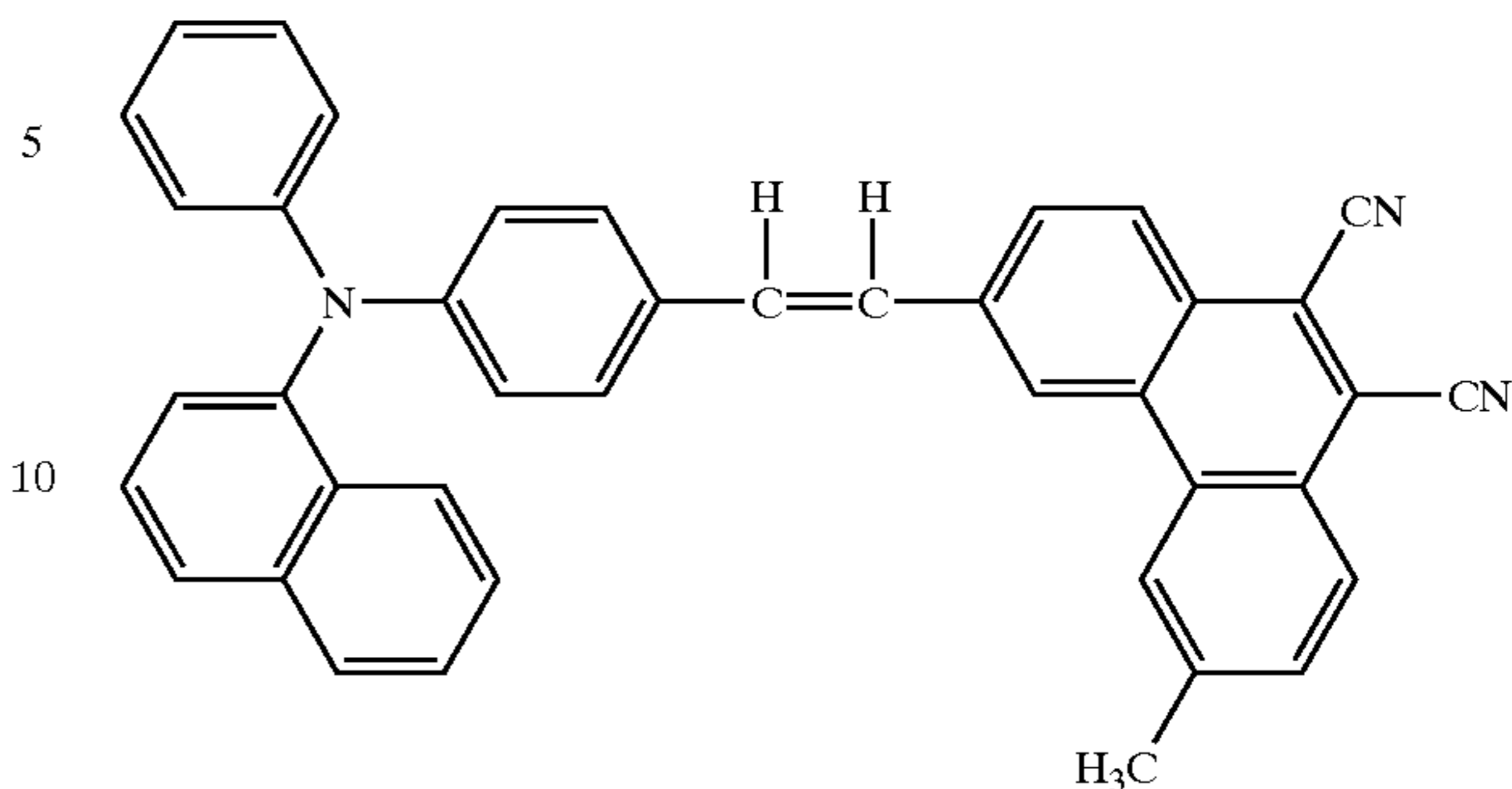
Structure Formula (20)-23:
