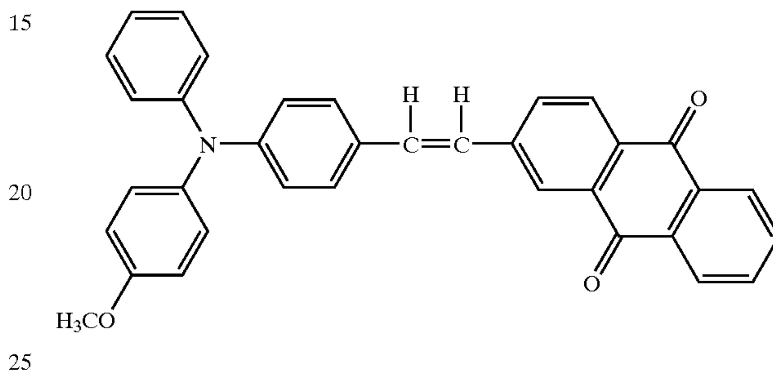
Structural Formula (20)-19:
