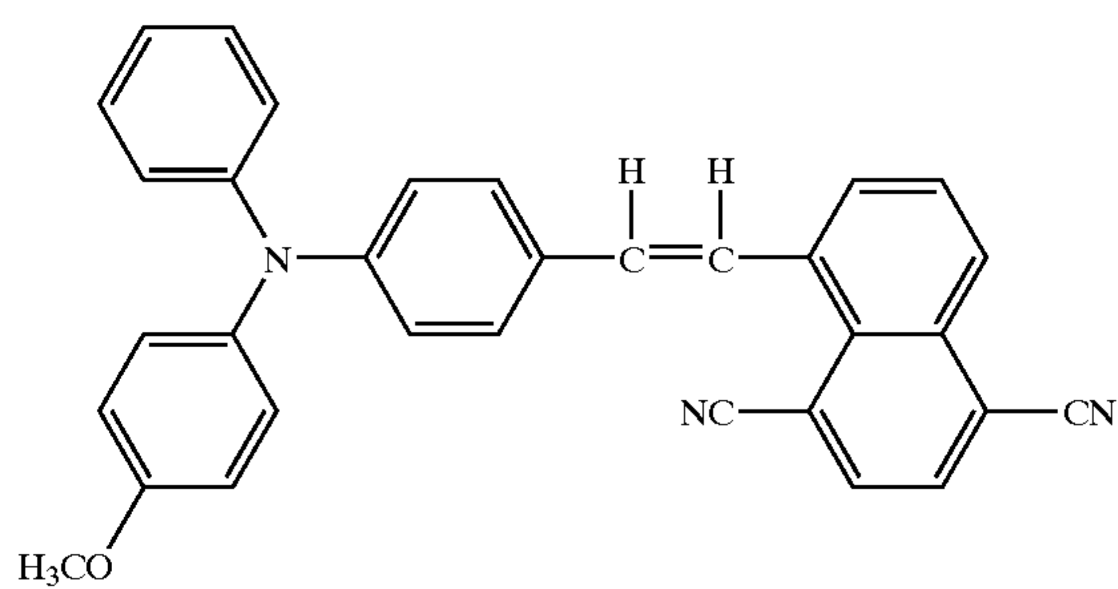
Structural Formula (20)-9:
