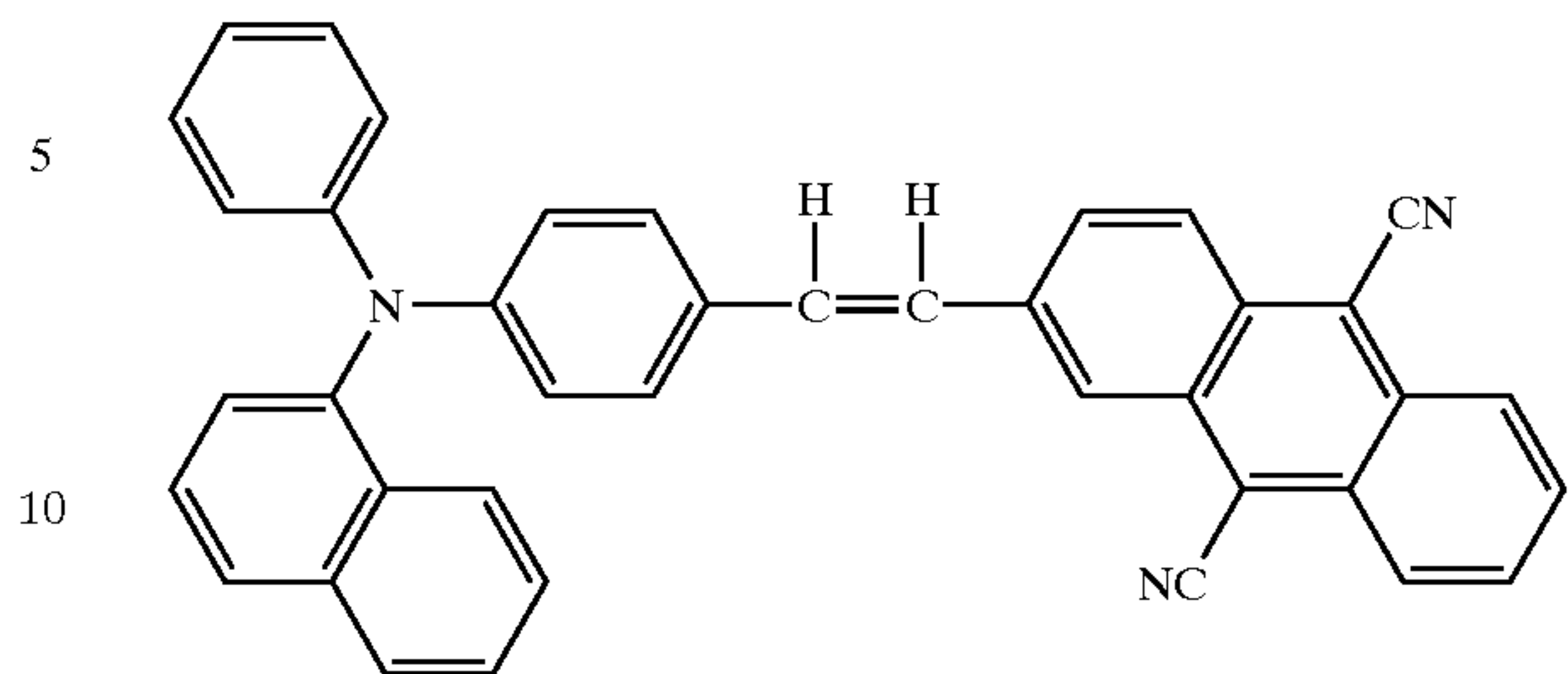
Structural Formula (20)-2:
