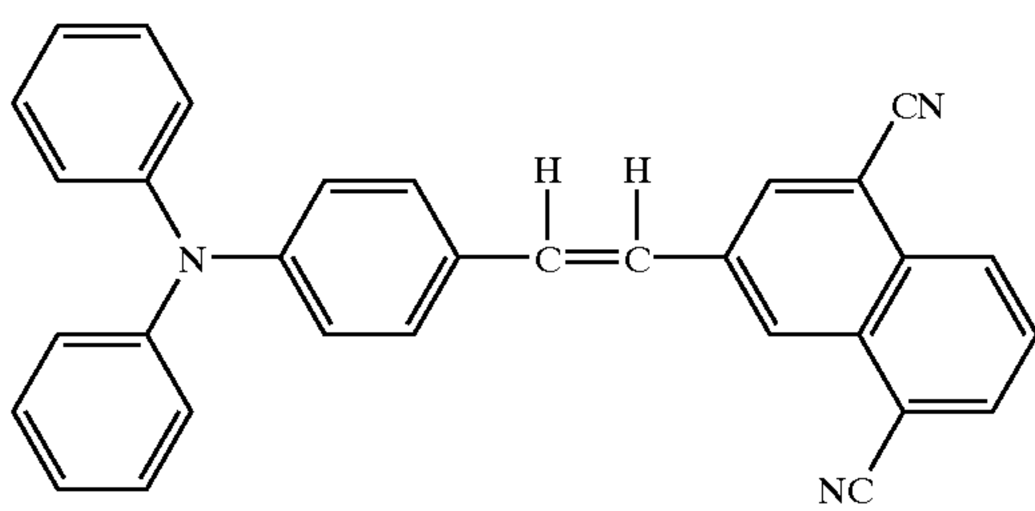
Structural Formula (20)-7:
