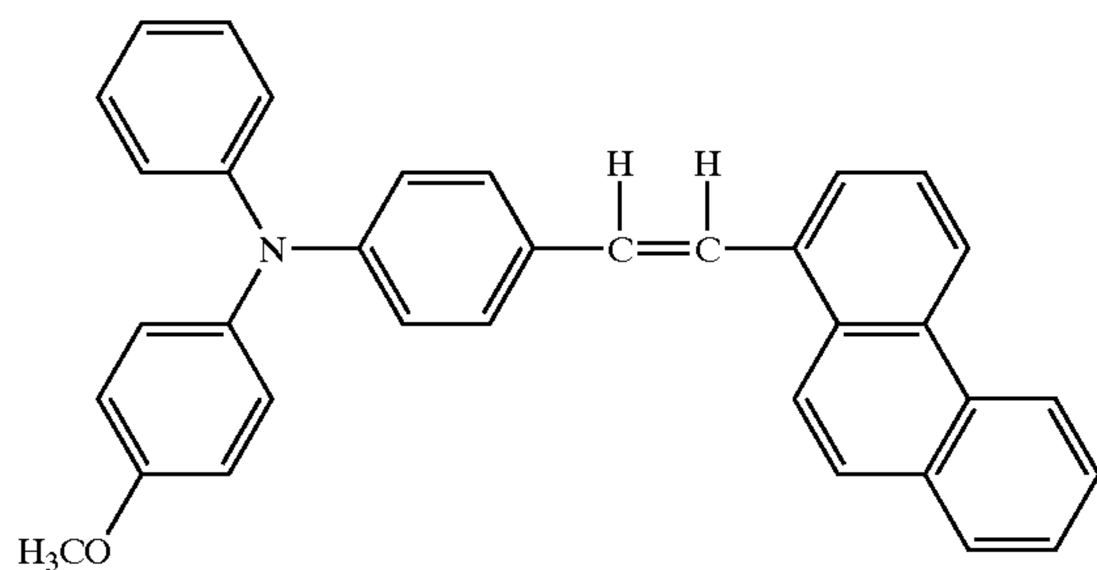
Structural Formula (20)-14:
