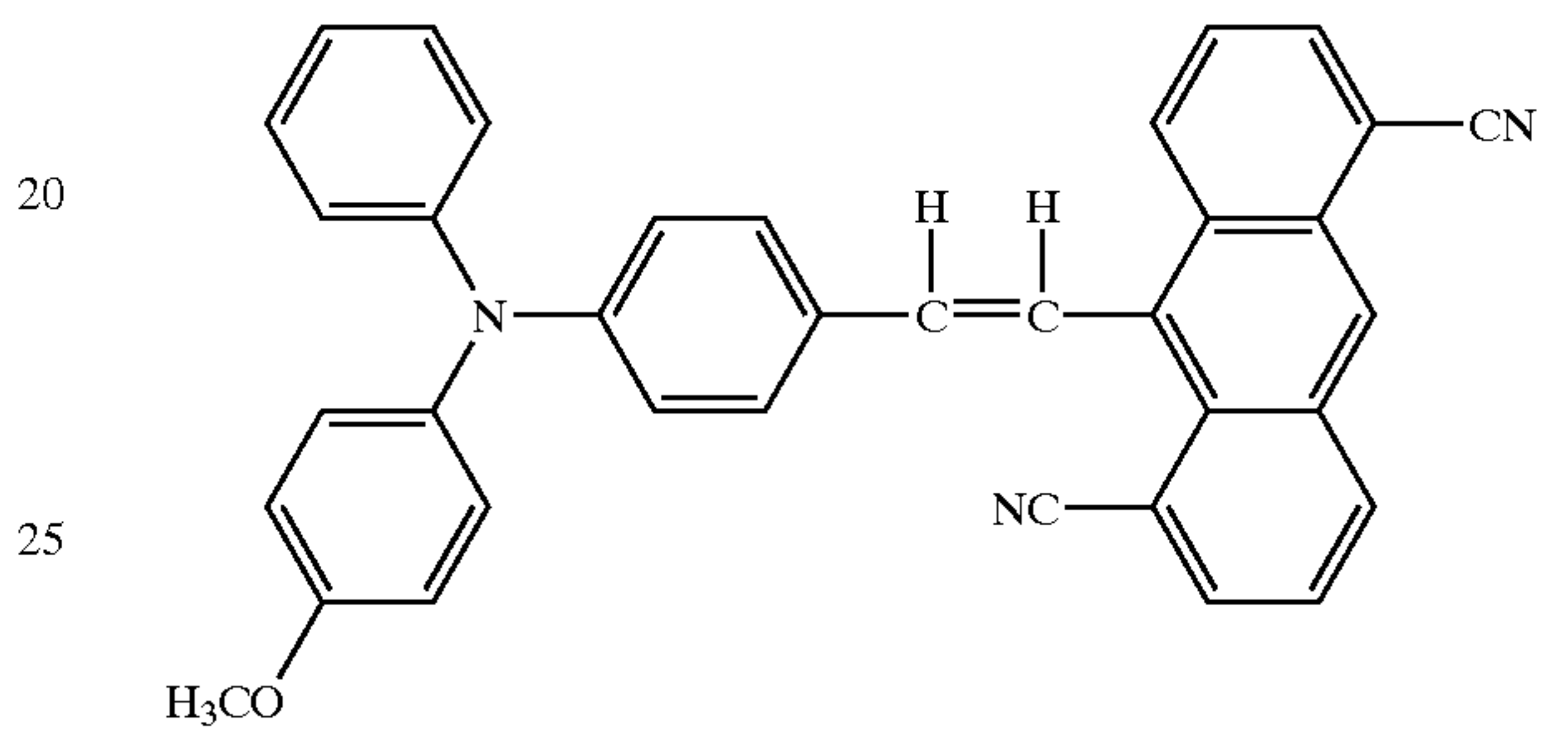
Structural Formula (20)-16:
