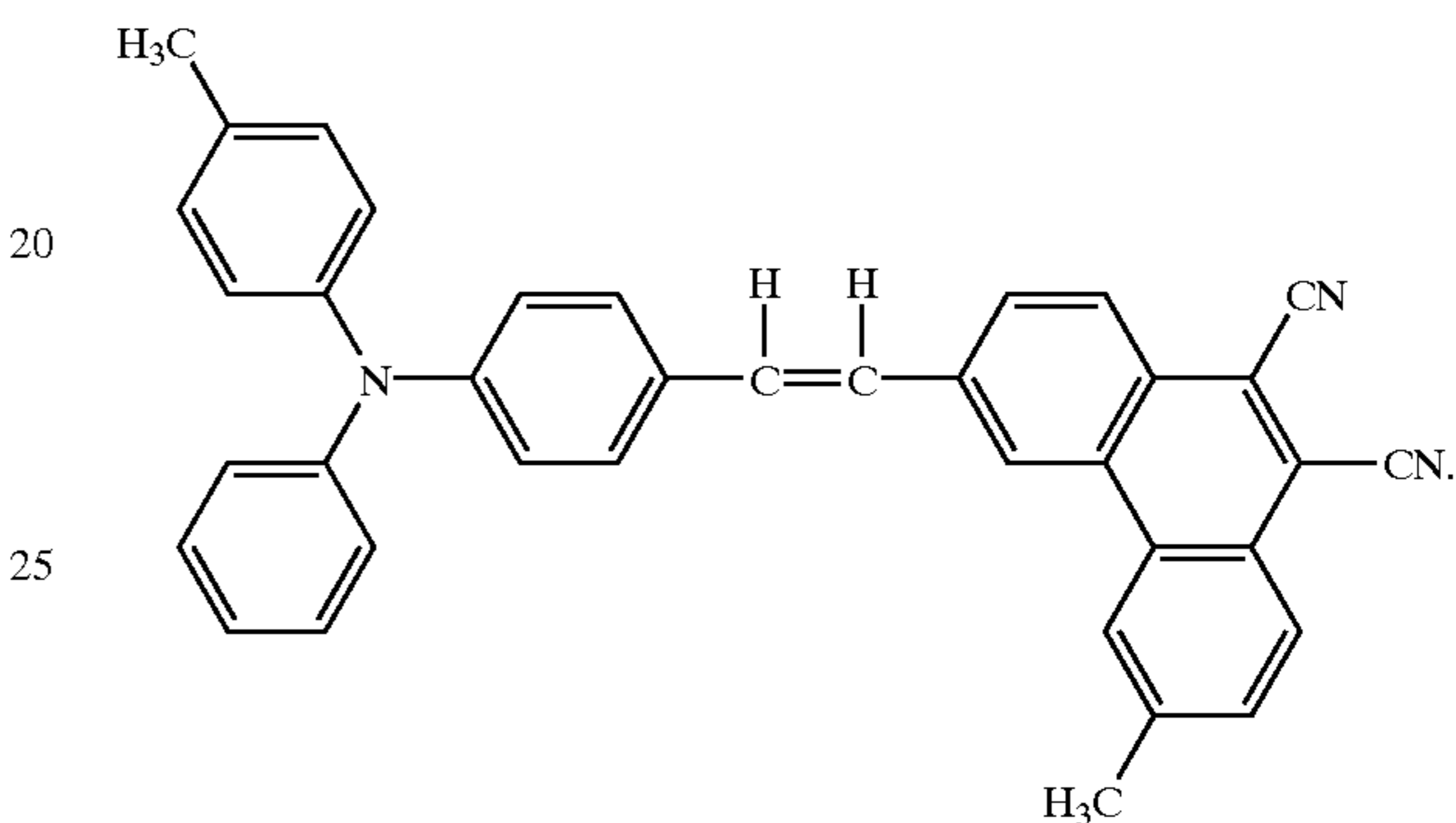
Structure Formula (20)-23:
