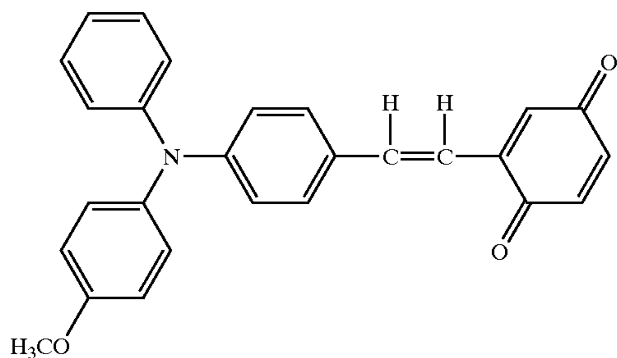
Structural Formula (20)-18:
