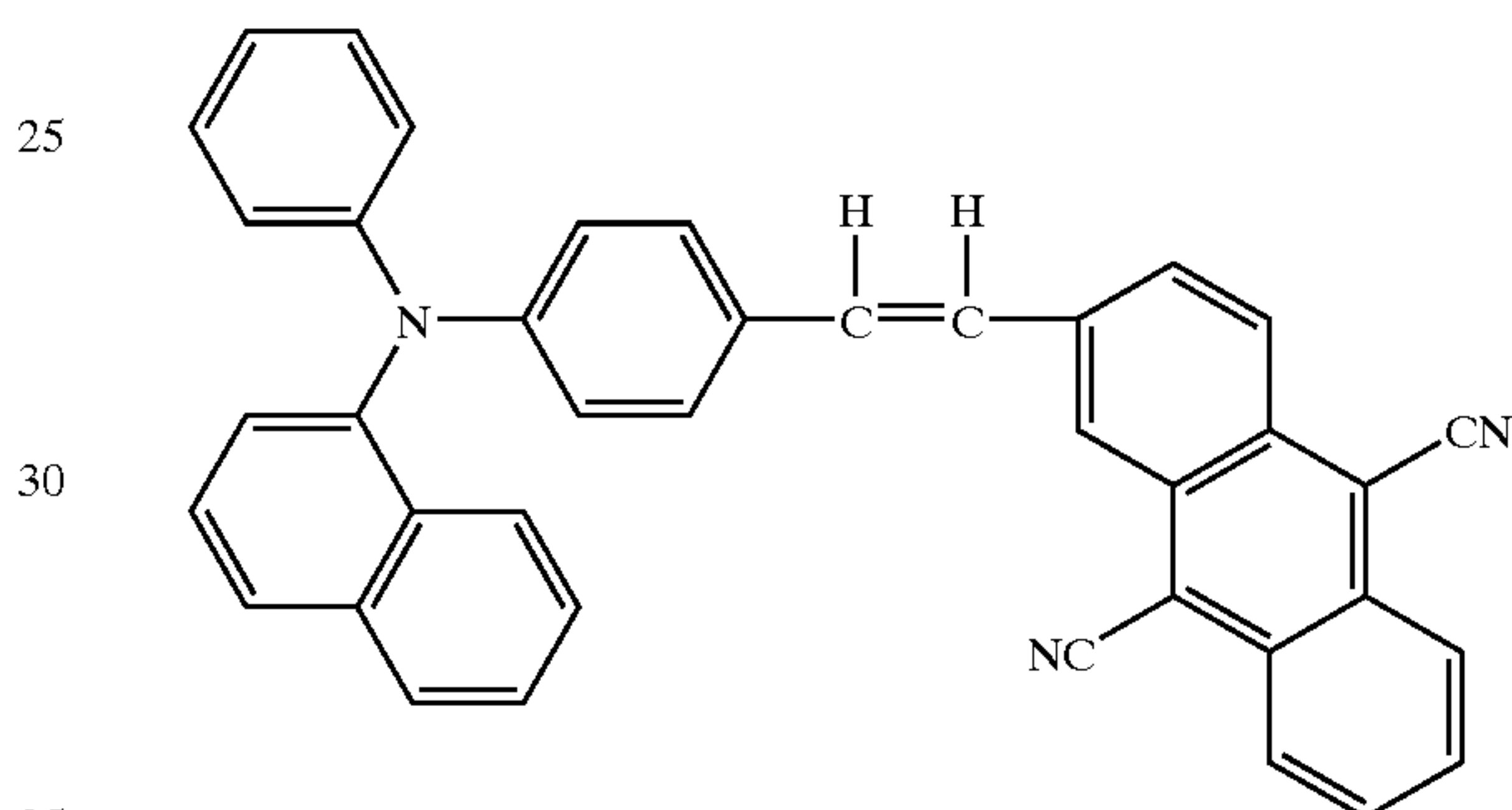
Structural Formula (20)-3:
