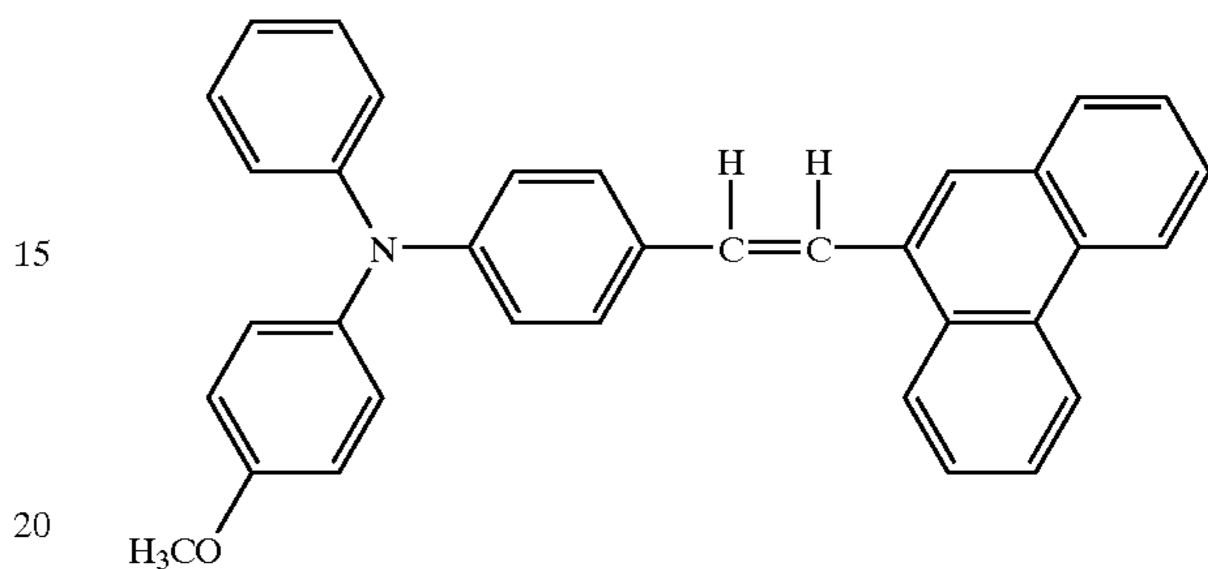
Structural Formula (20)-15:
