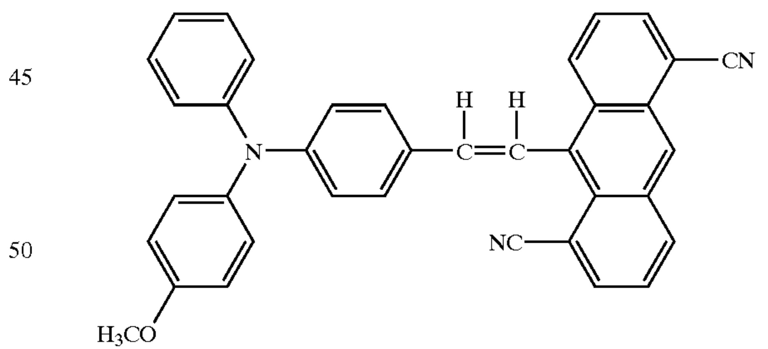
Structural Formula (20)-12:
