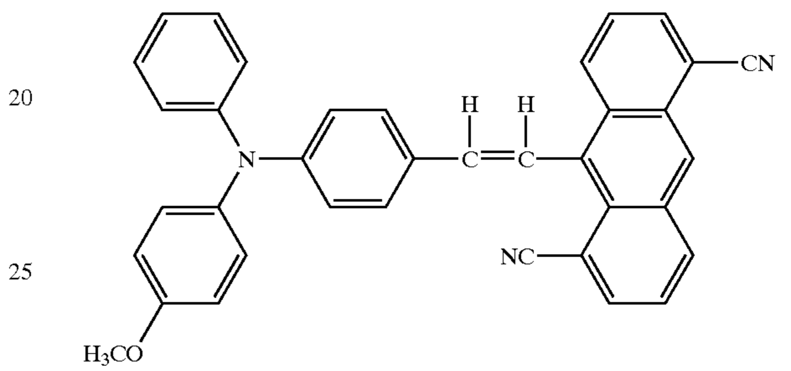
Structural Formula (20)-16:
