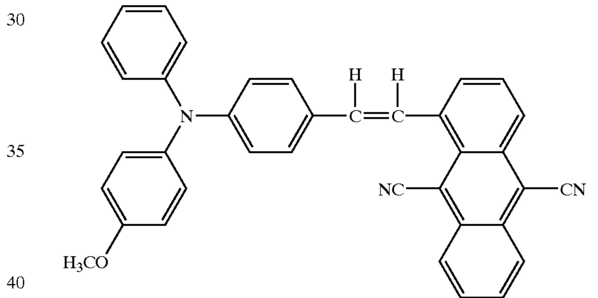
Structural Formula (20)-11:
