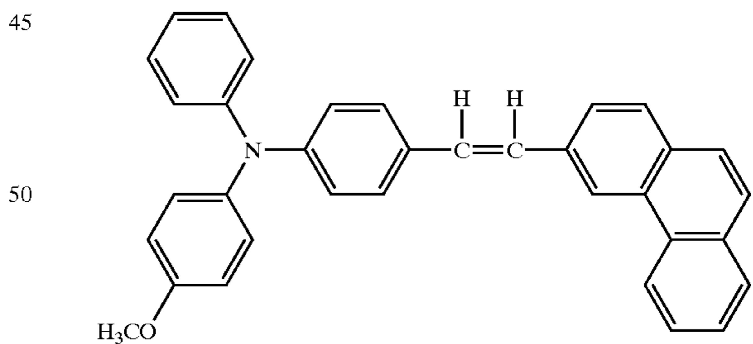
Structural Formula (20)-12:
