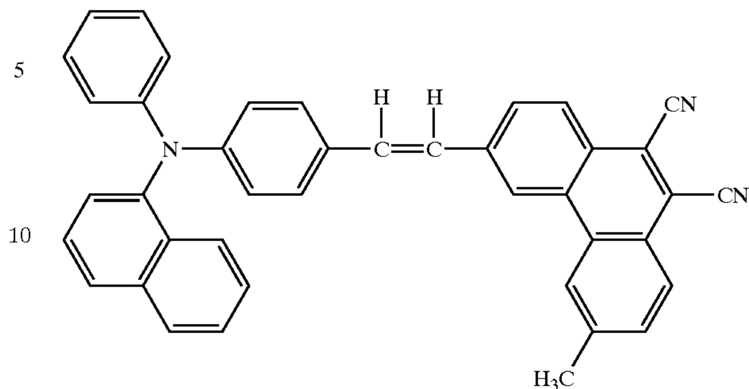
Structure Formula (20)-23:
