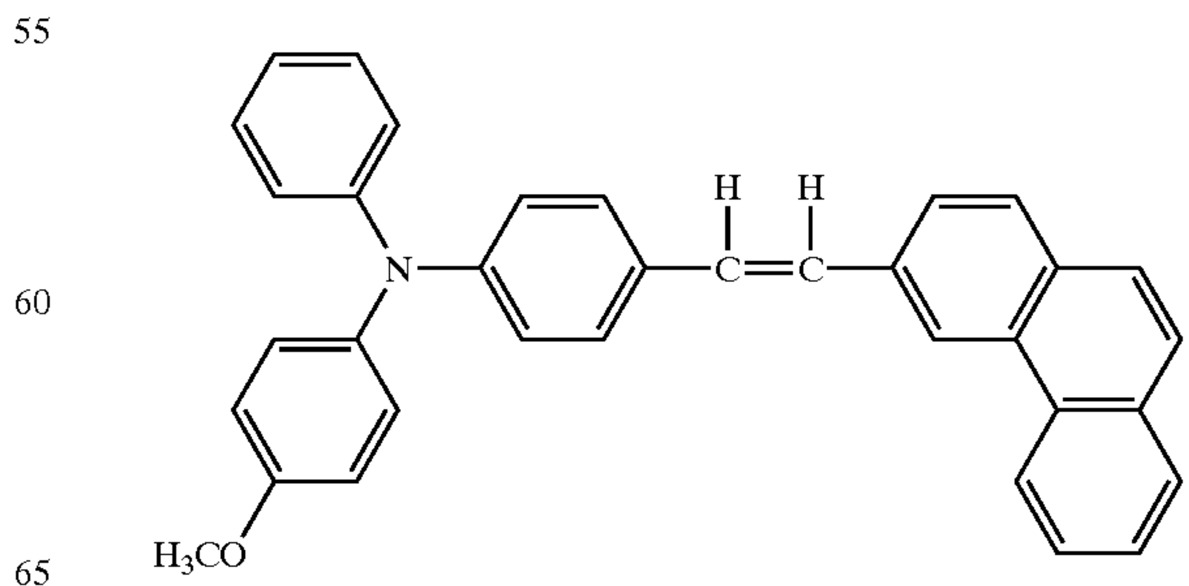
Structural Formula (20)-12:
