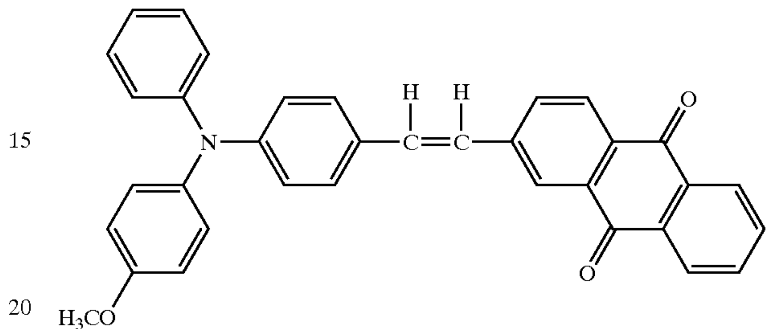
10 Structural Formula (20)-19:
