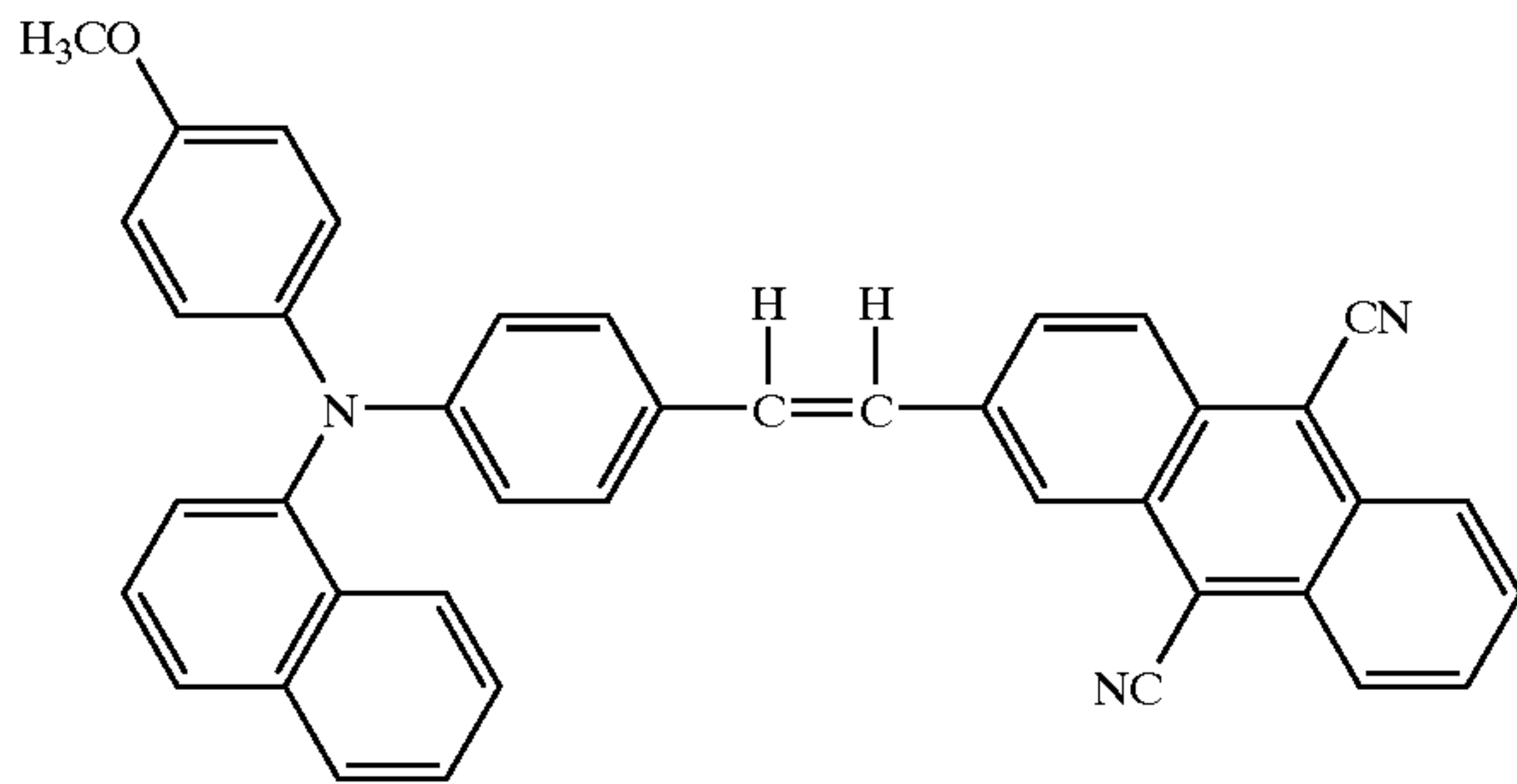
Structural Formula (20)-4:
