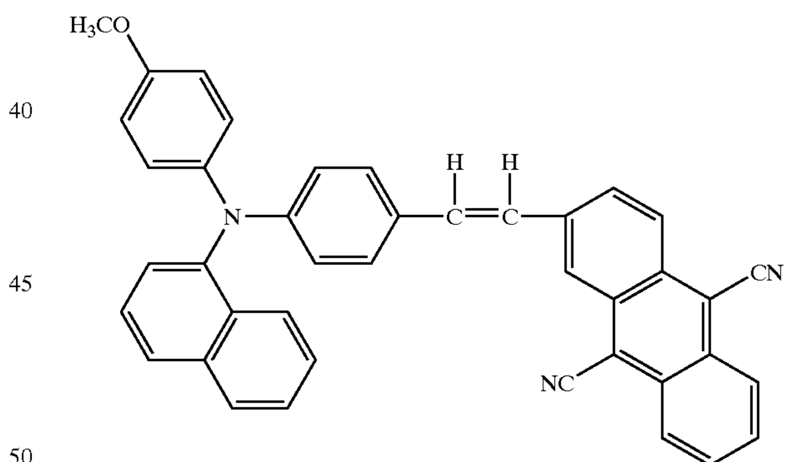
Structural Formula (20)-4:
