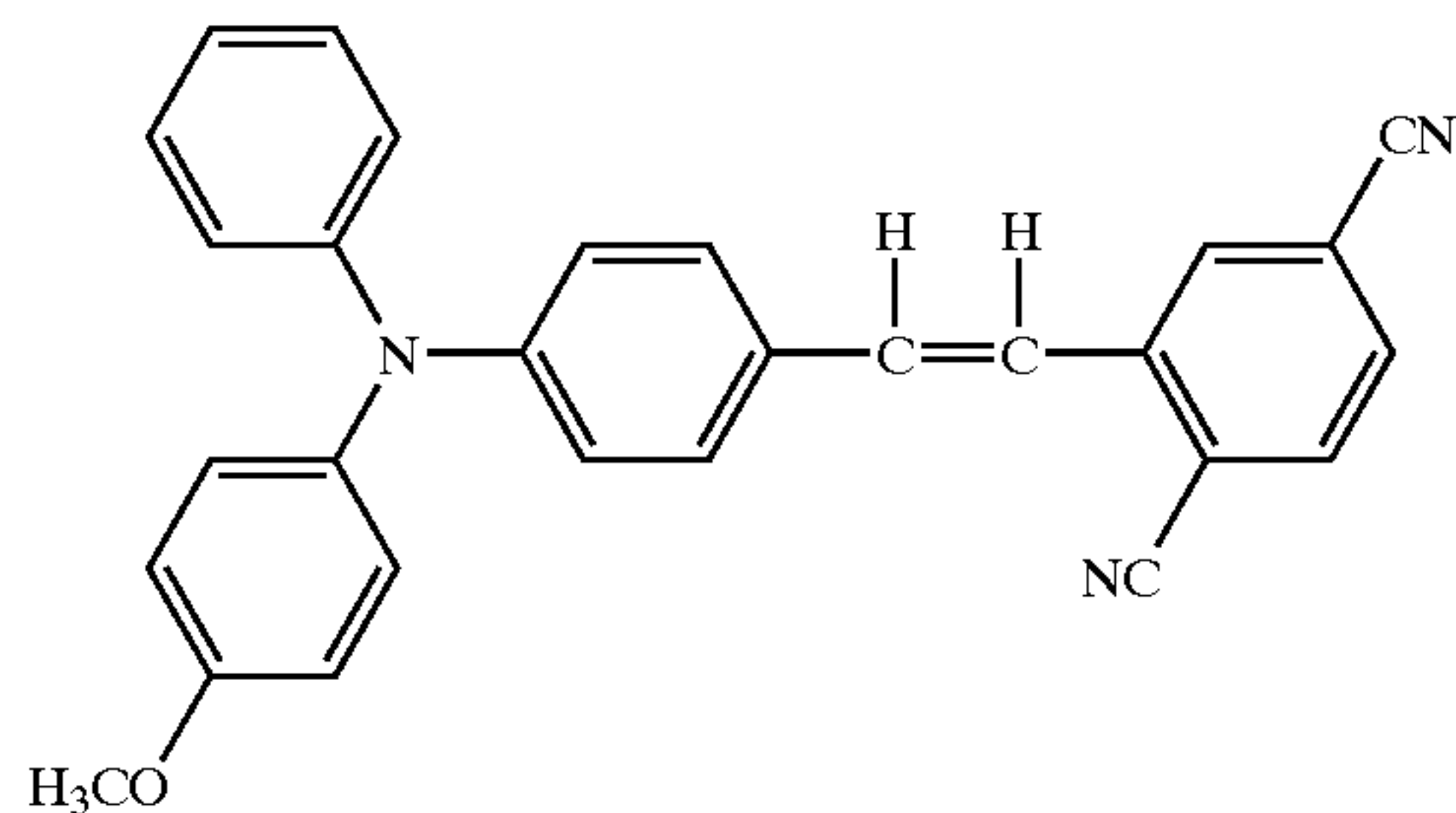
Structural Formula (20)-16:
