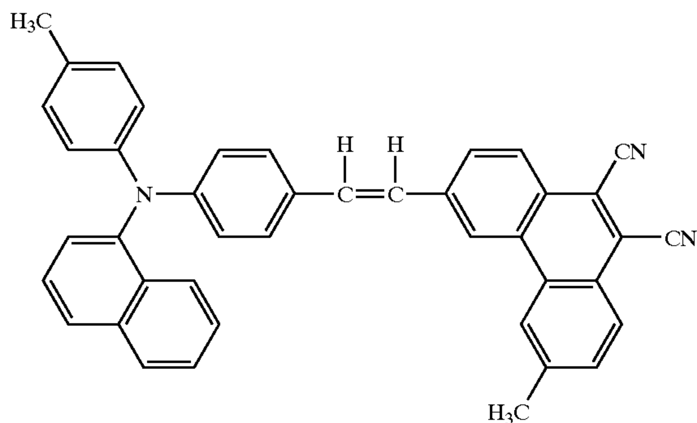
Structural Formula (20)-21:
