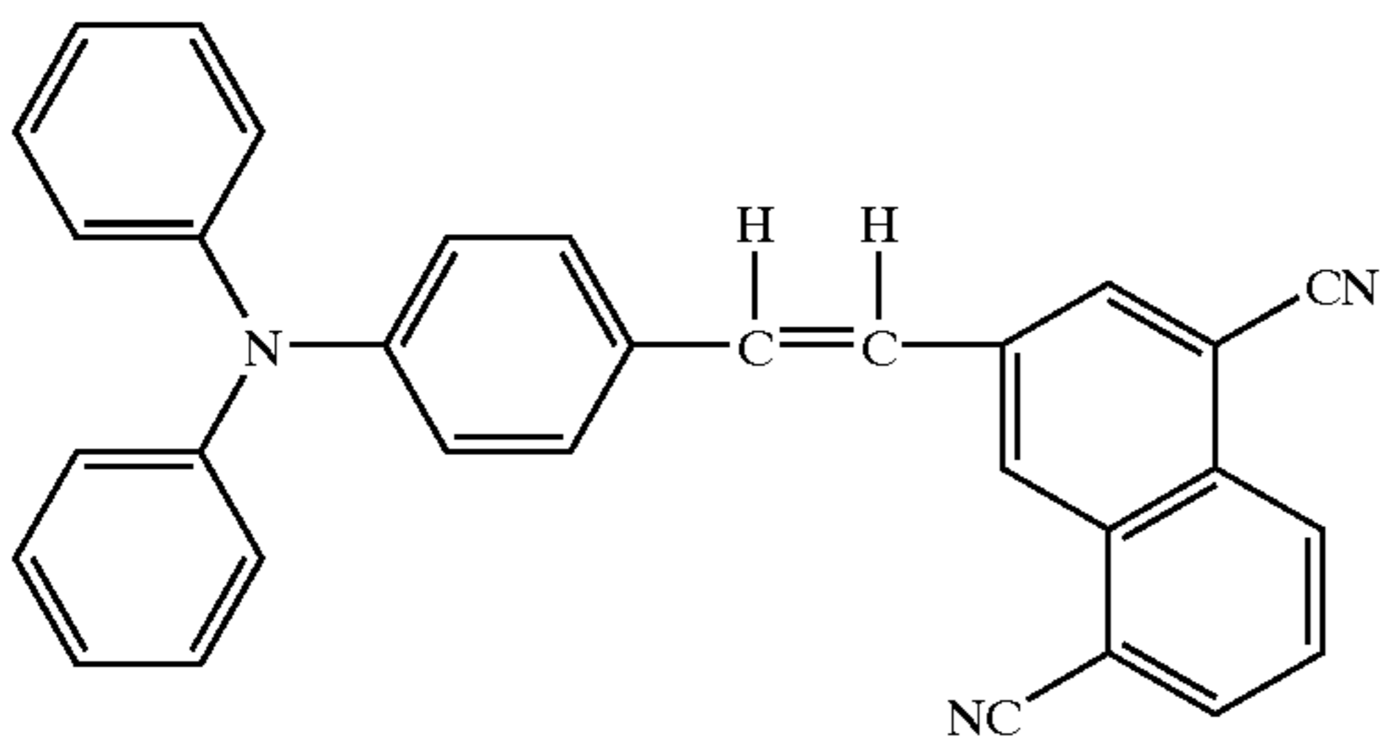
Structural Formula (20)-8:
