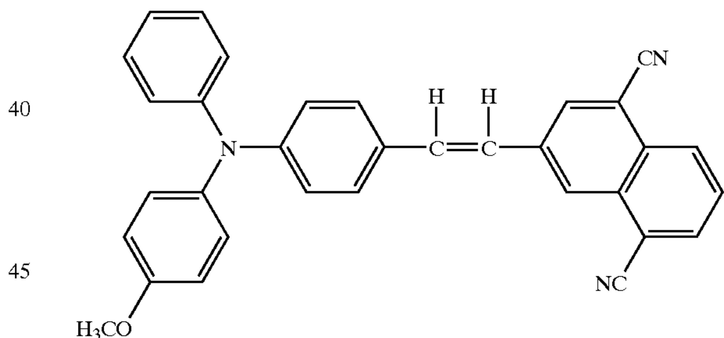
Structural Formula (20)-8:
