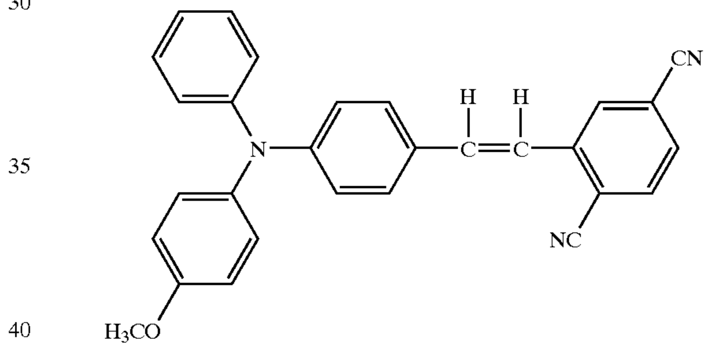
Structural Formula (20)-17:
