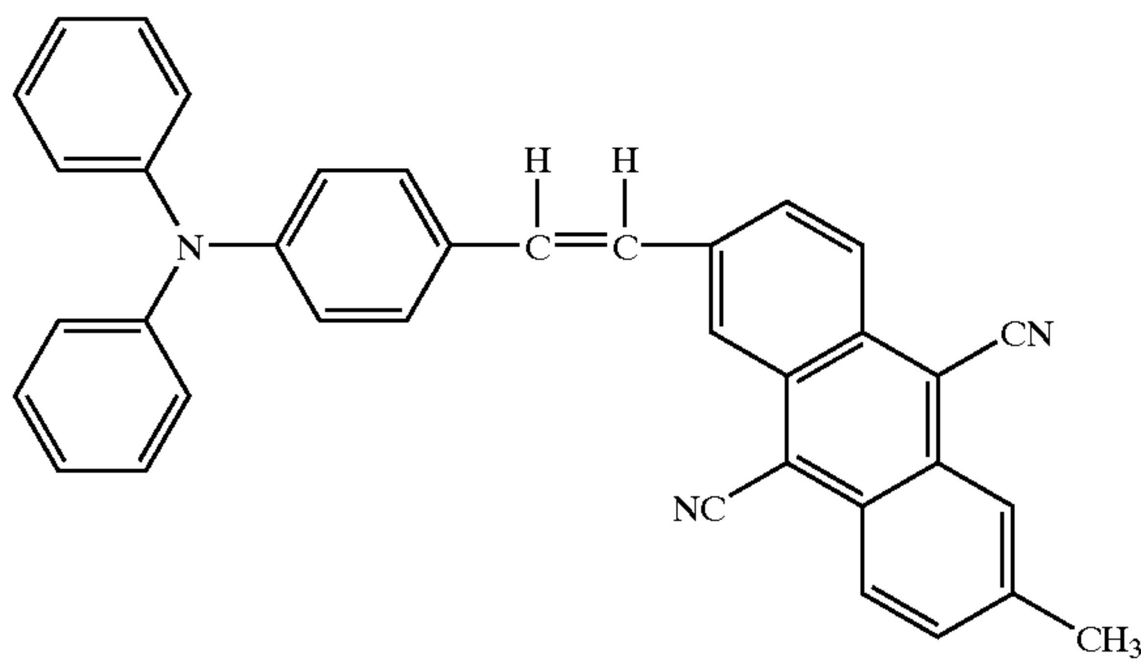
Structural Formula (20)-7:
