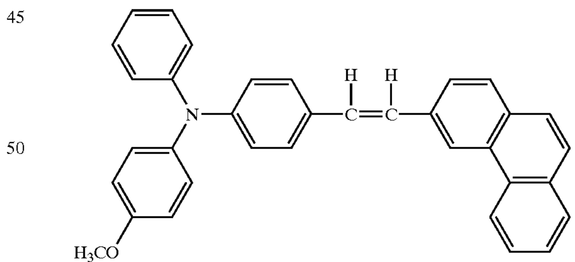
Structural Formula (20)-12:
