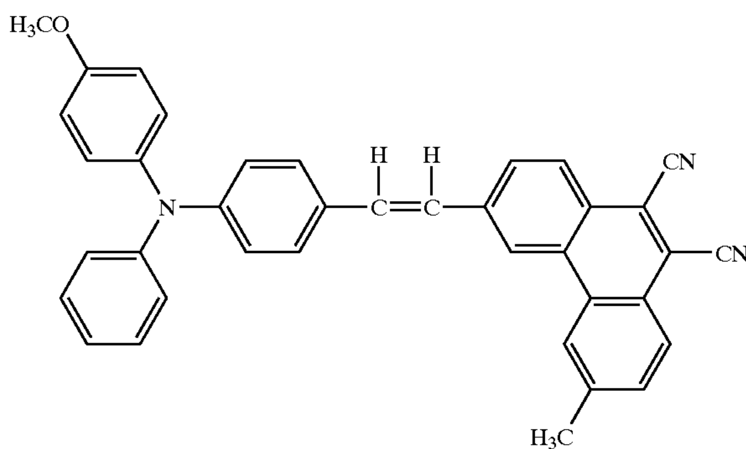
Structural Formula (20)-21:
