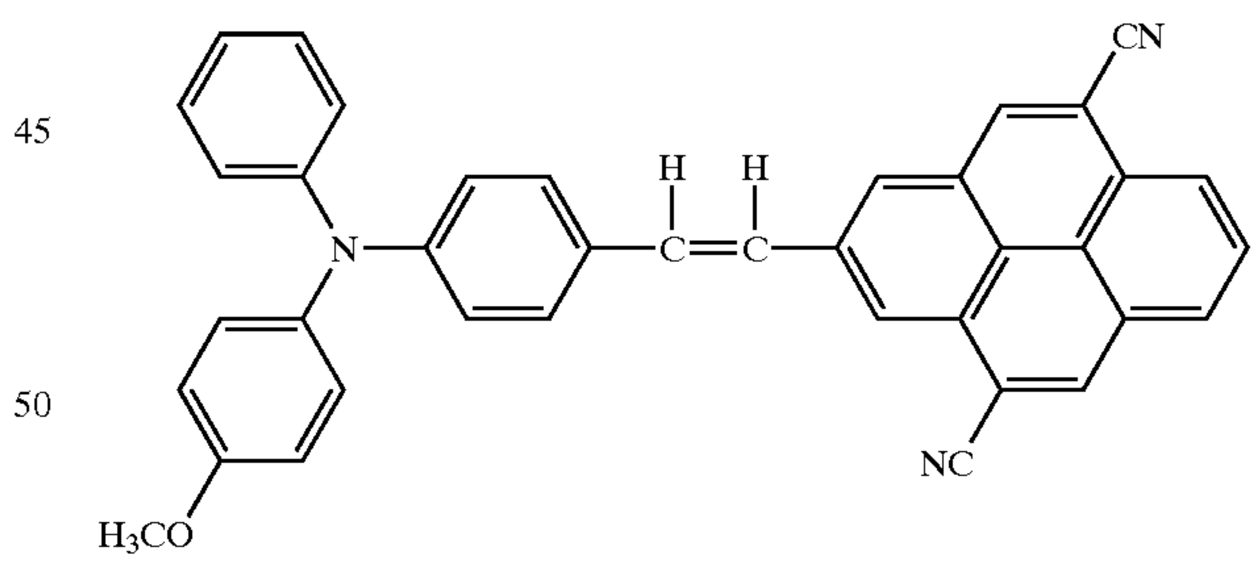
Structural Formula (20)-18:
