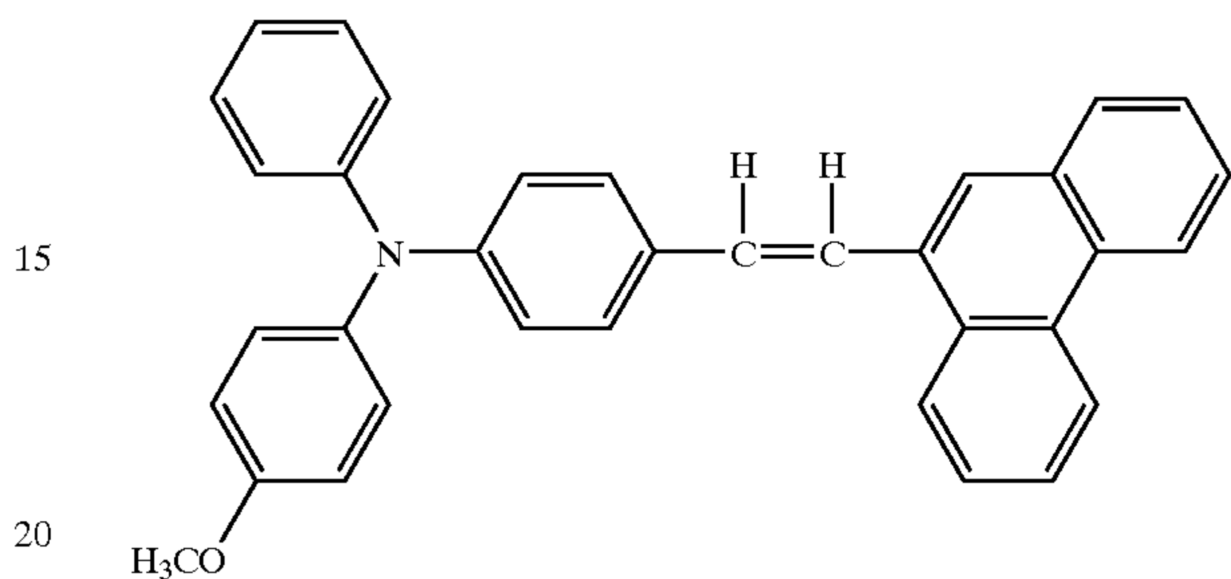
Structural Formula (20)-15:
