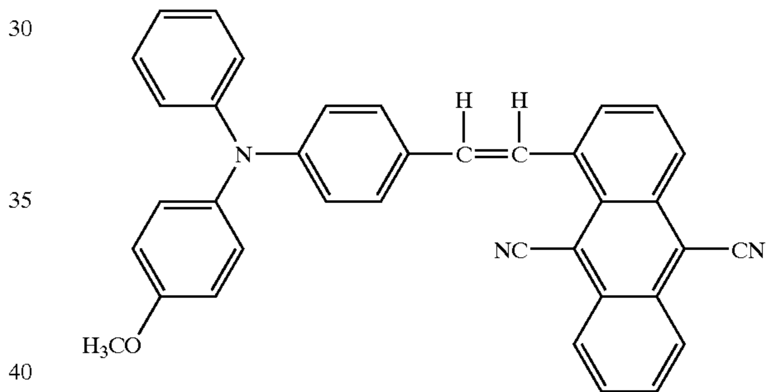
Structural Formula (20)-11:
