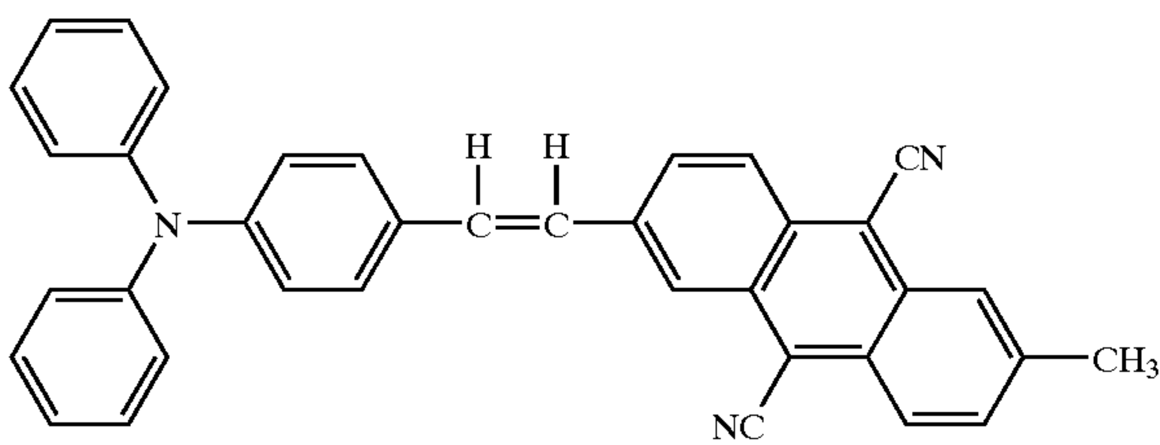
Structural Formula (20)-7:
