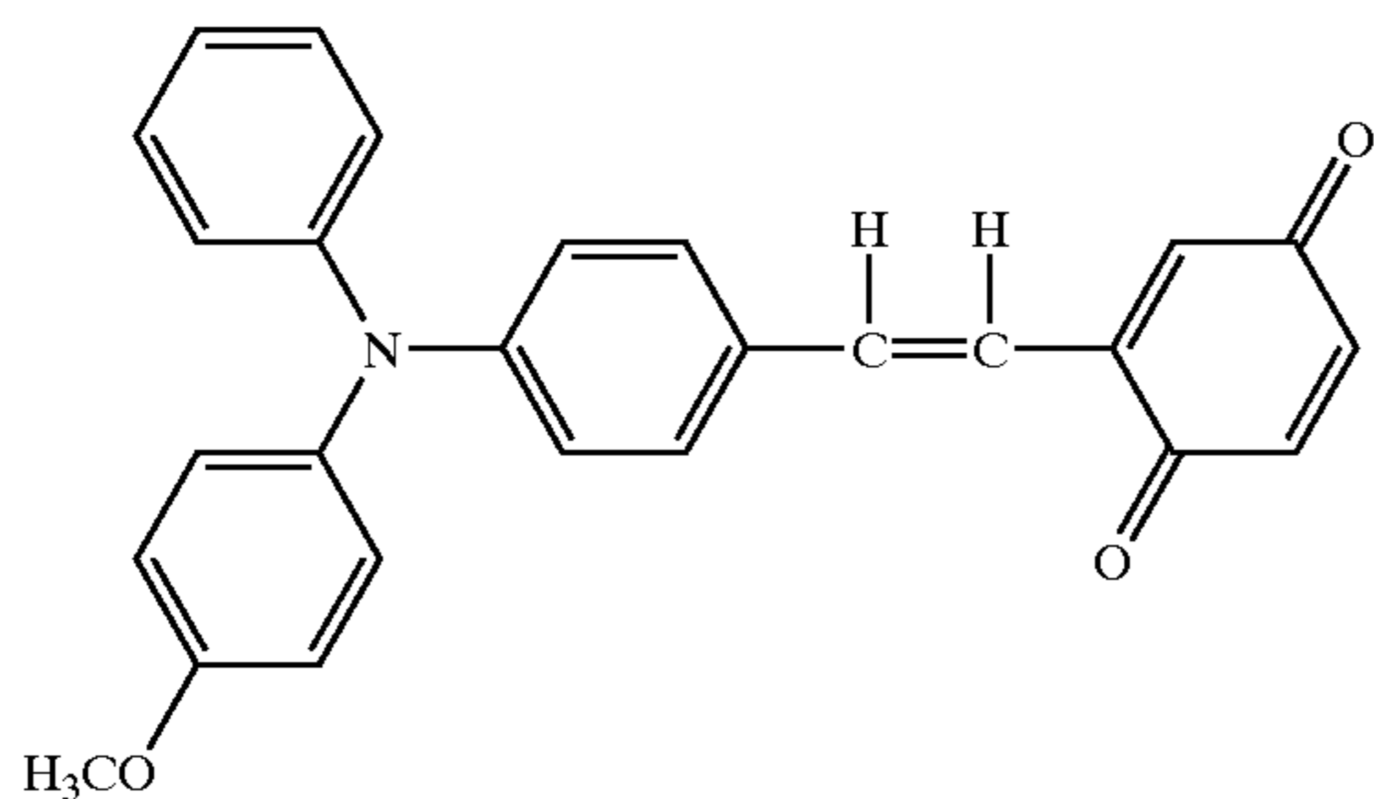
Structural Formula (20)-18:
