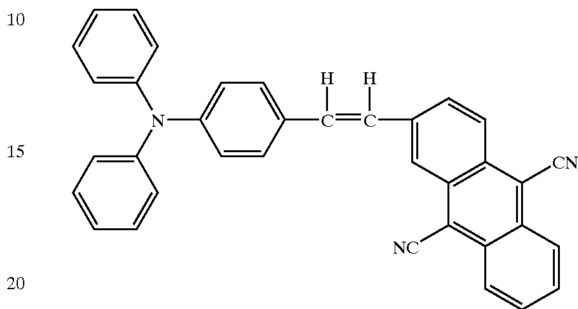
Structural Formula (20)-2:
