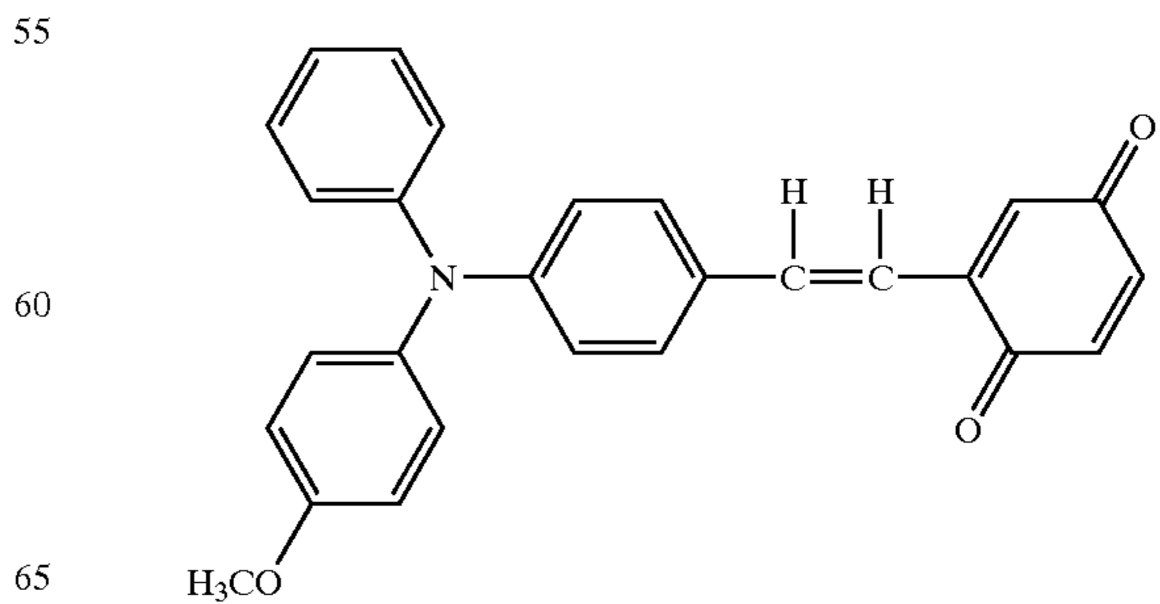
Structural Formula (20)-18:
