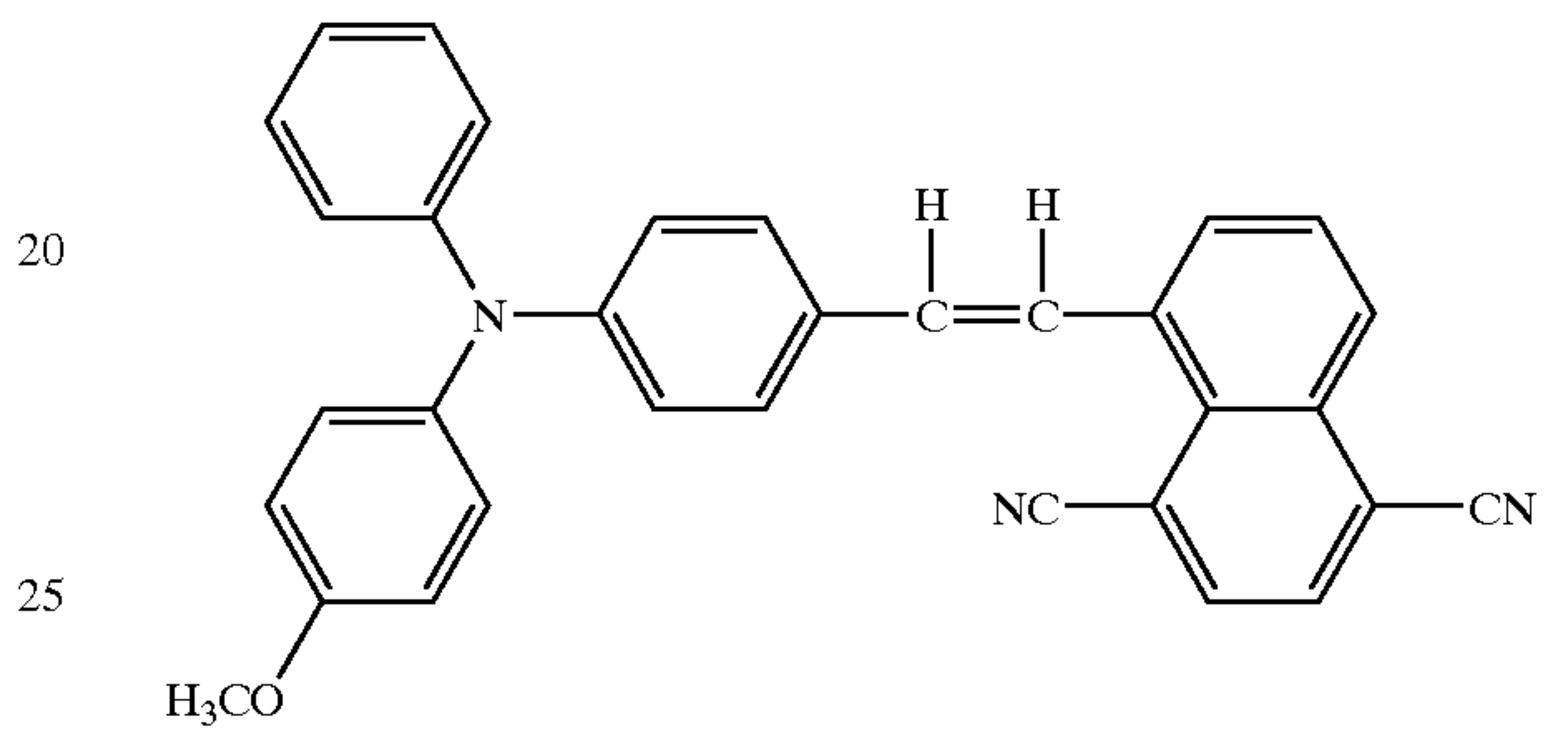
Structural Formula (20)-10:
