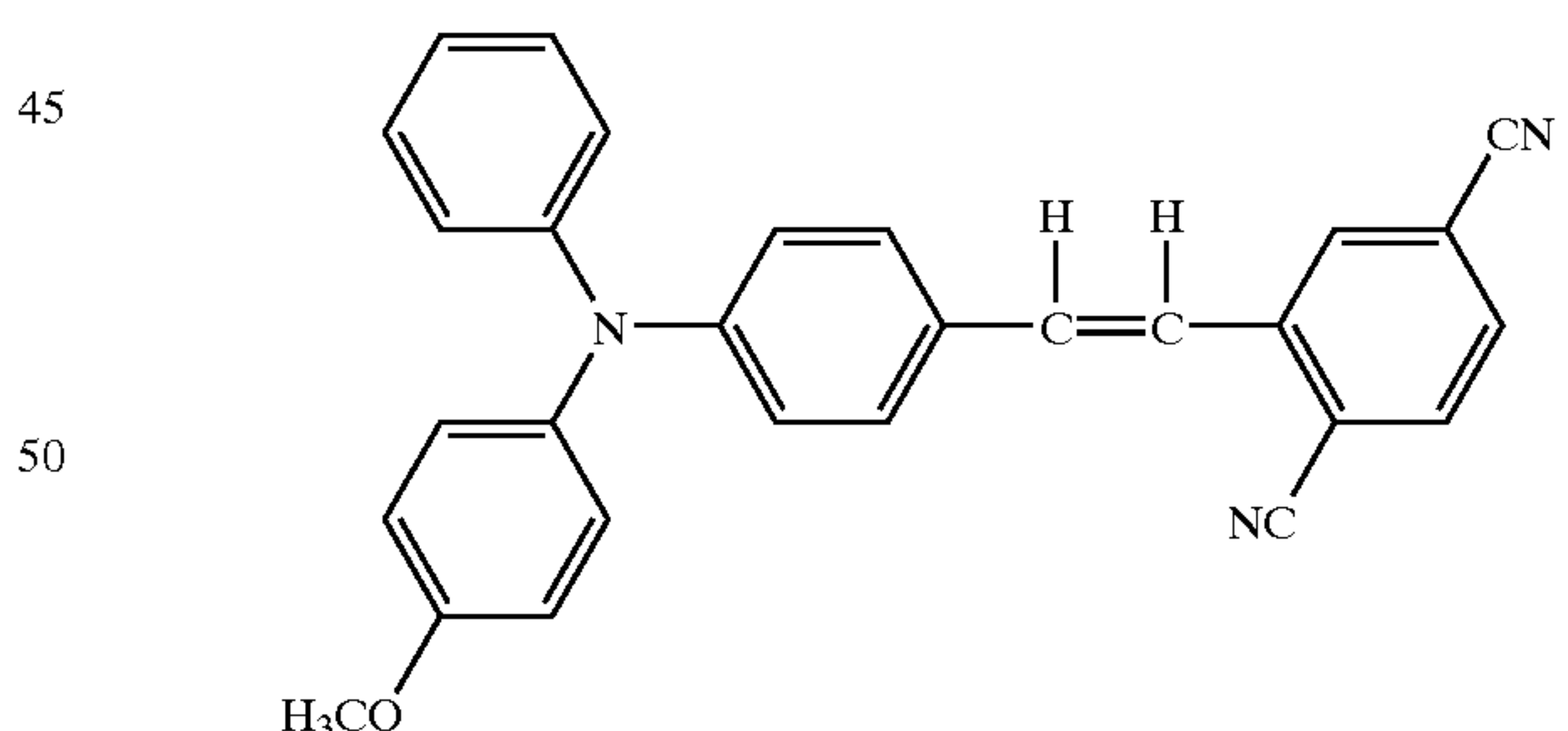
Structural Formula (20)-16:
