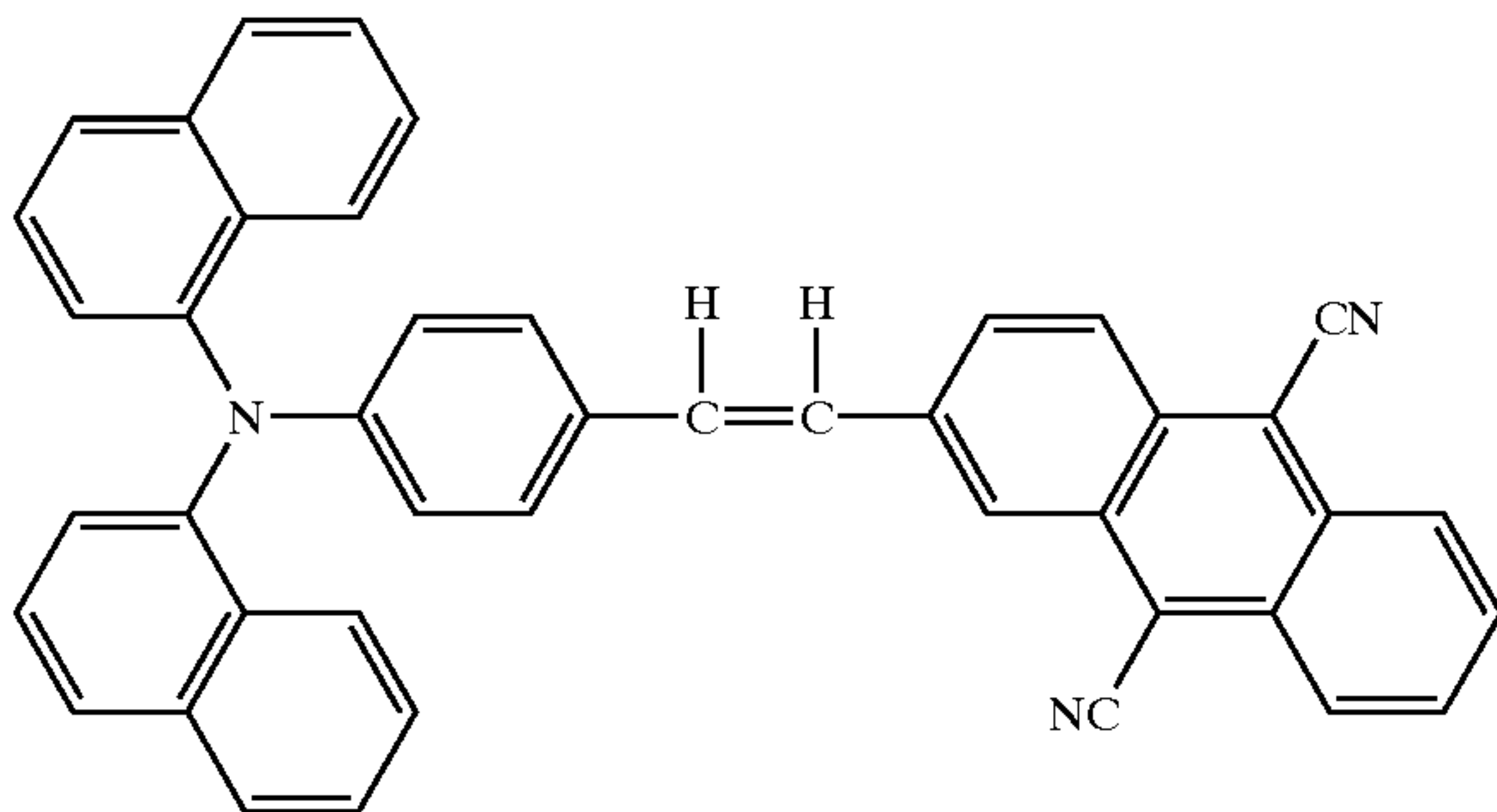
Structural Formula (20)-5:
