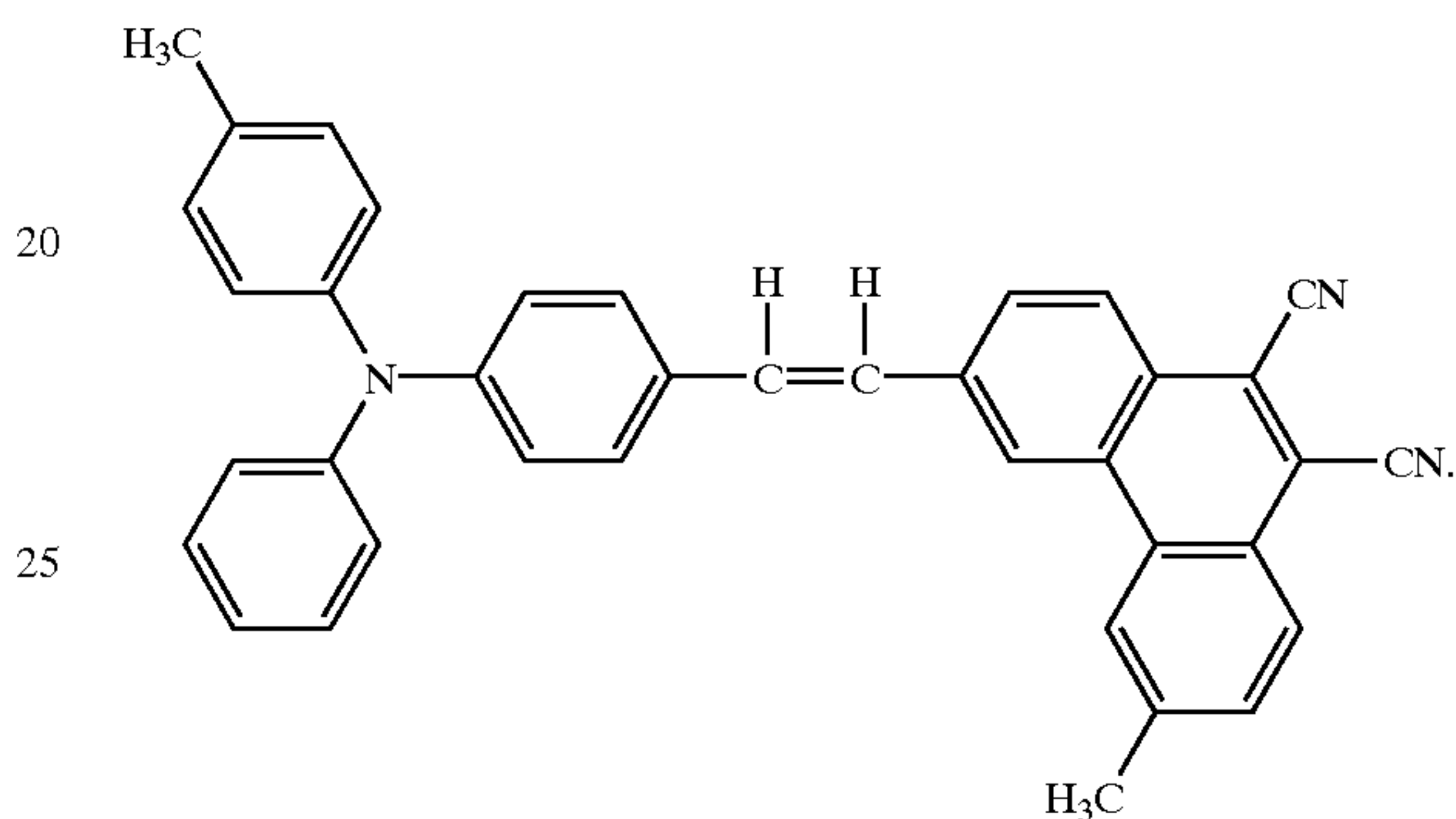
Structure Formula (20)-23:
