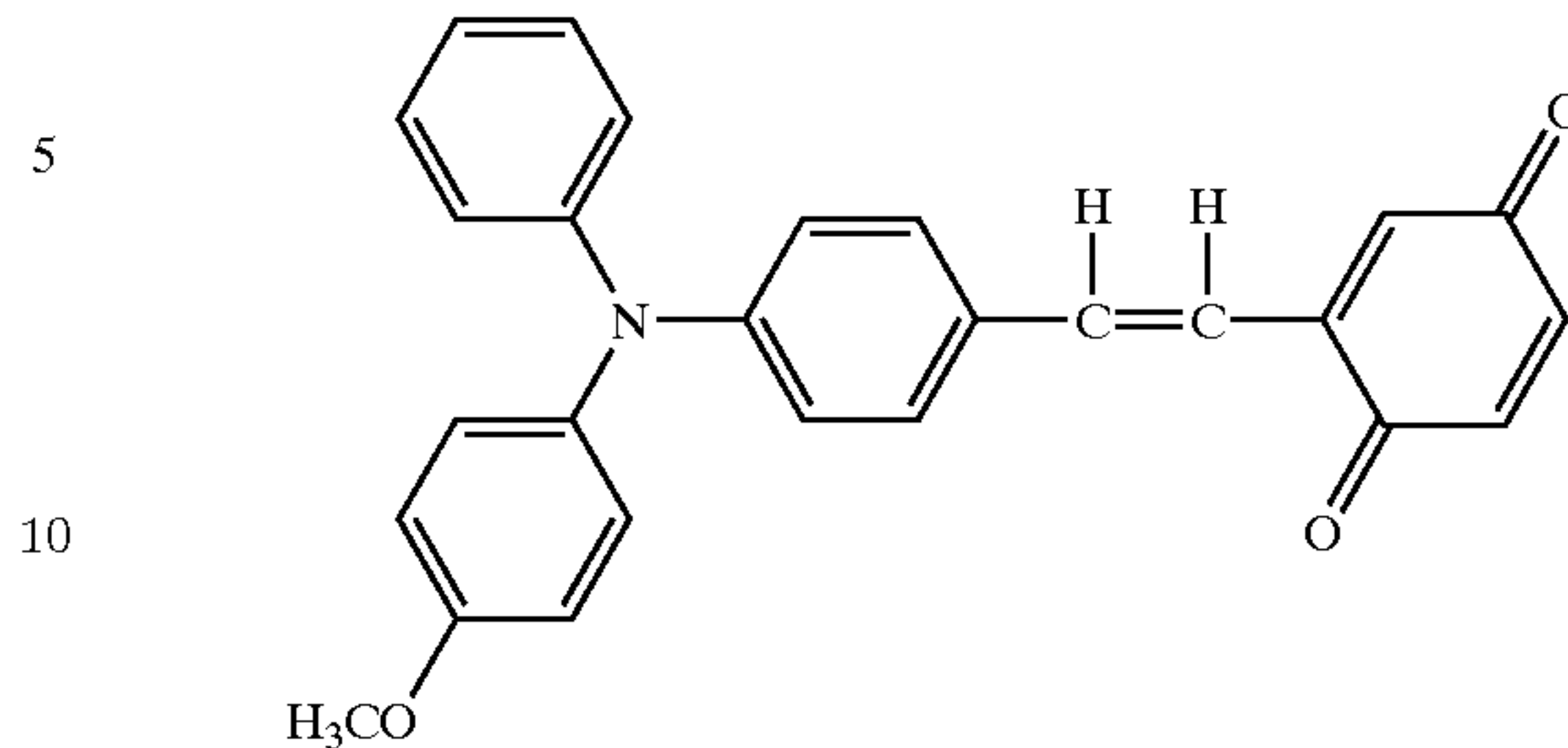
Structural Formula (20)-19:
