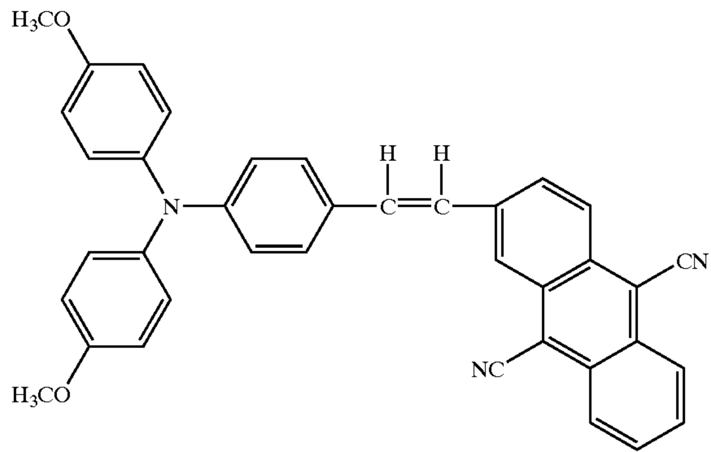
Structural Formula (20)-6:
