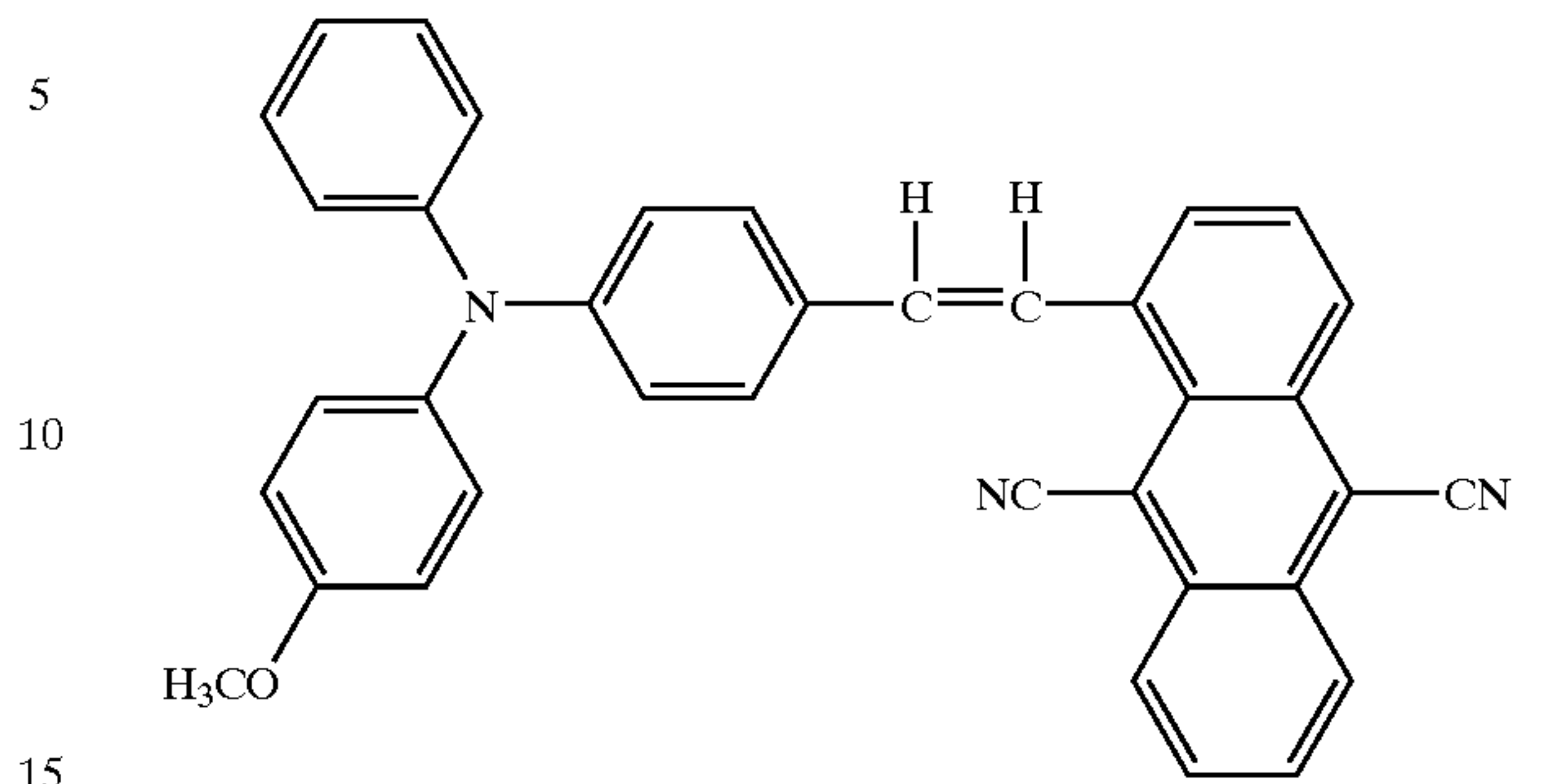
Structural Formula (20)-11:
