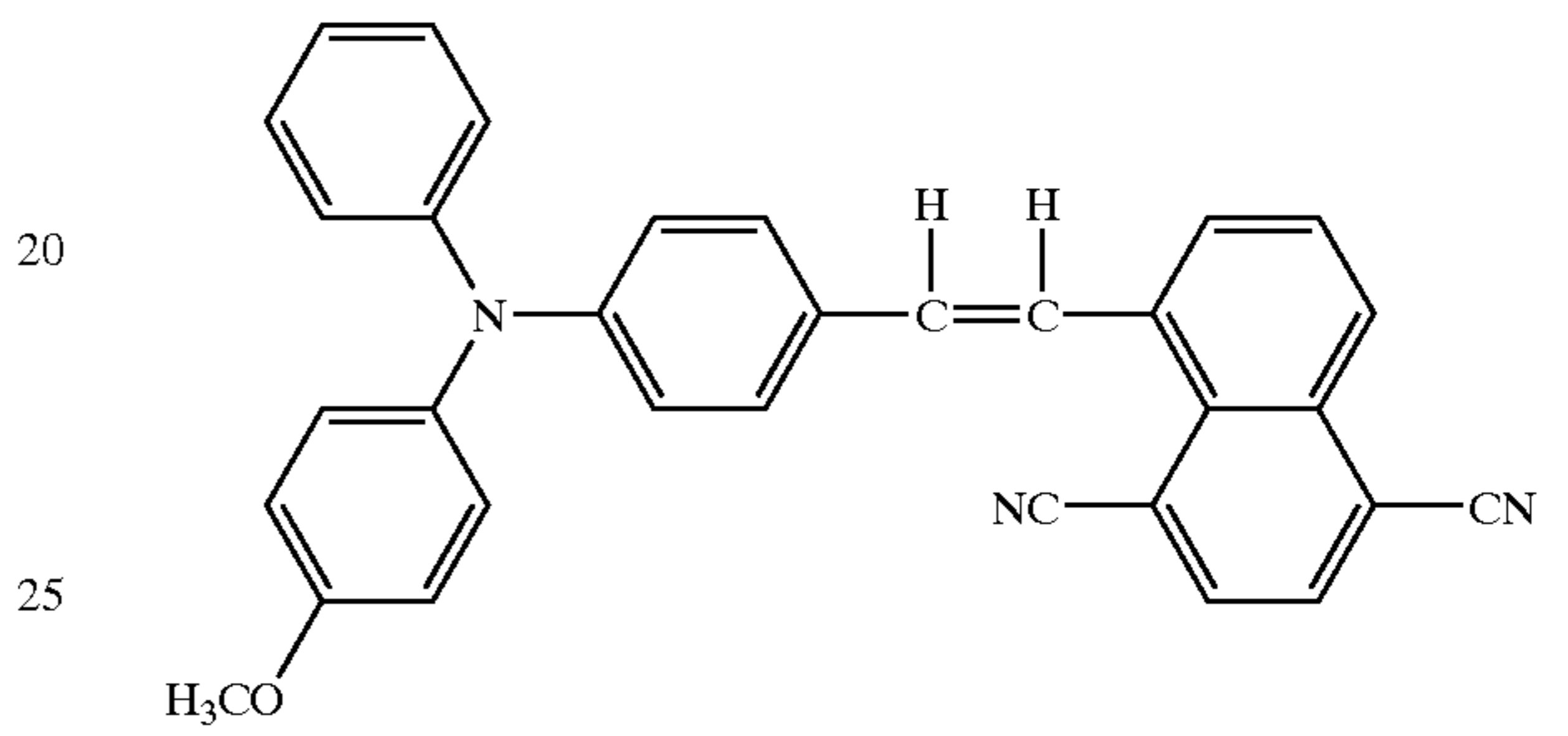
Structural Formula (20)-10:
