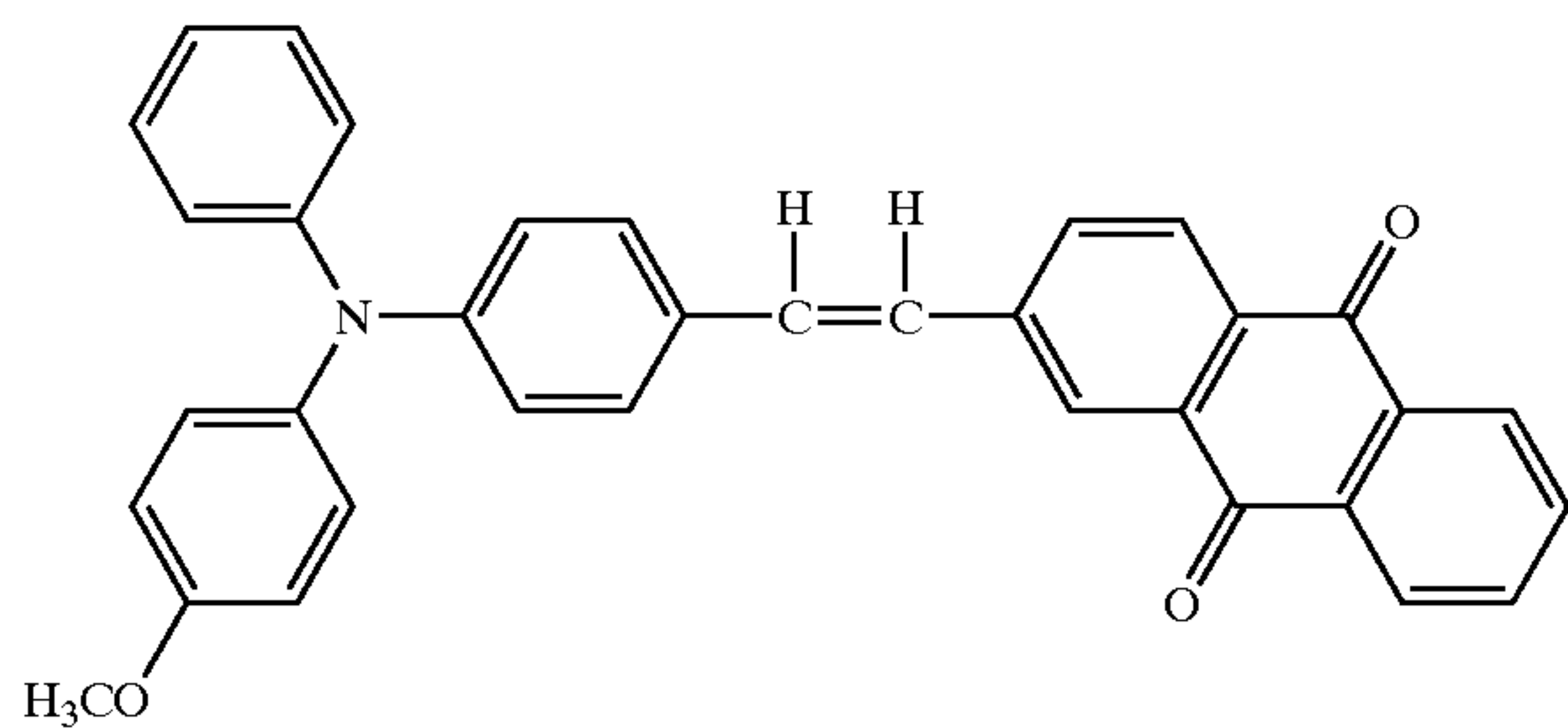
Structural Formula (20)-20:
