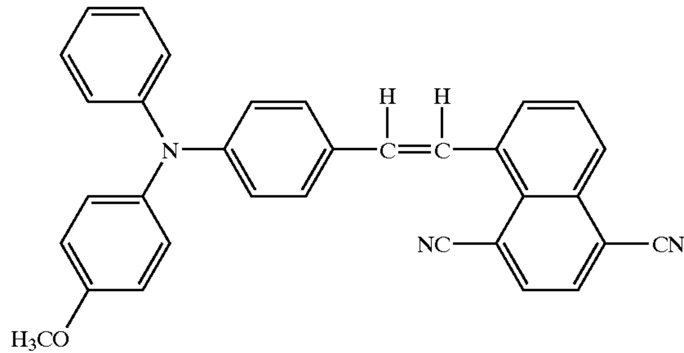
Structural Formula (20)-9:
