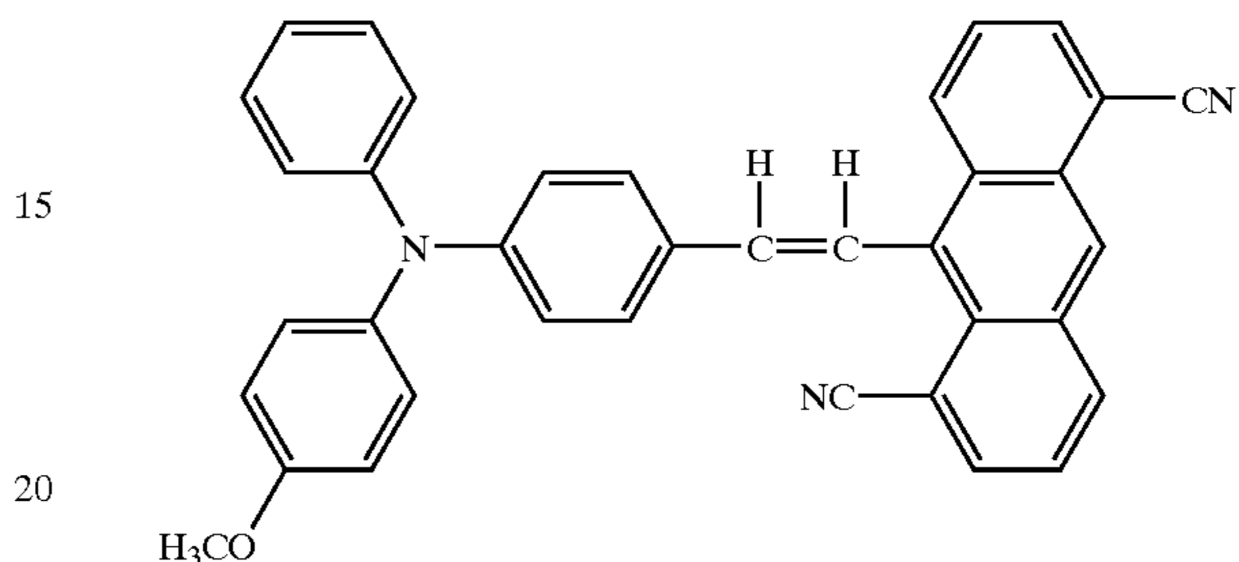
Structural Formula (20)-11:
