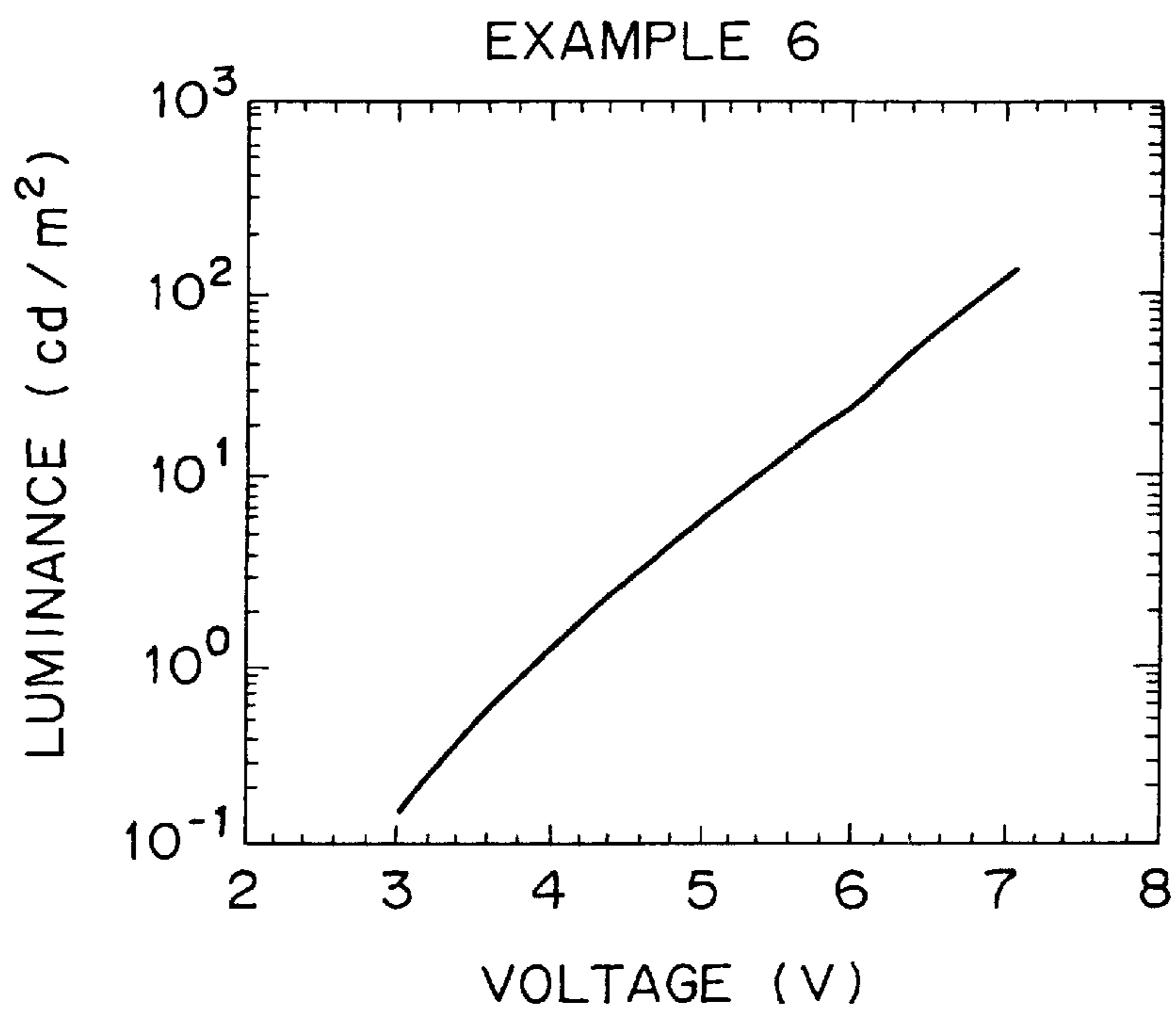
VOLTAGE-LUMINANCE CHARACTERISTIC
