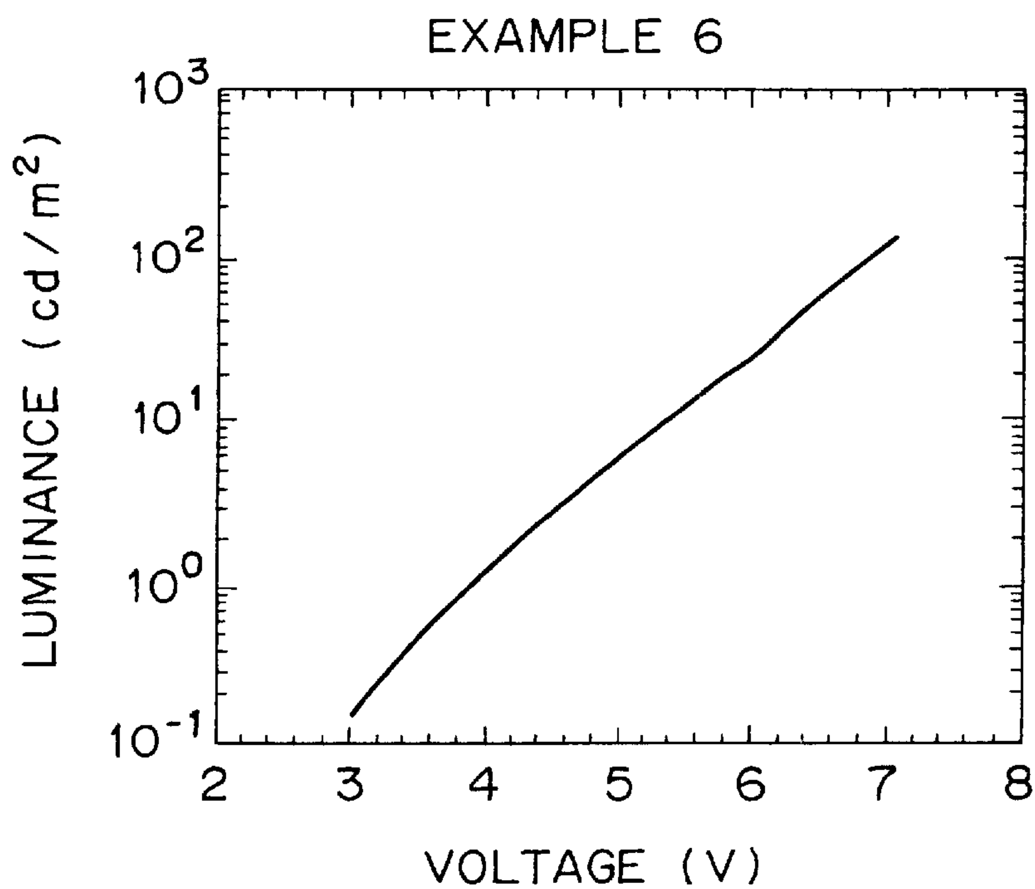
VOLTAGE-LUMINANCE CHARACTERISTIC
