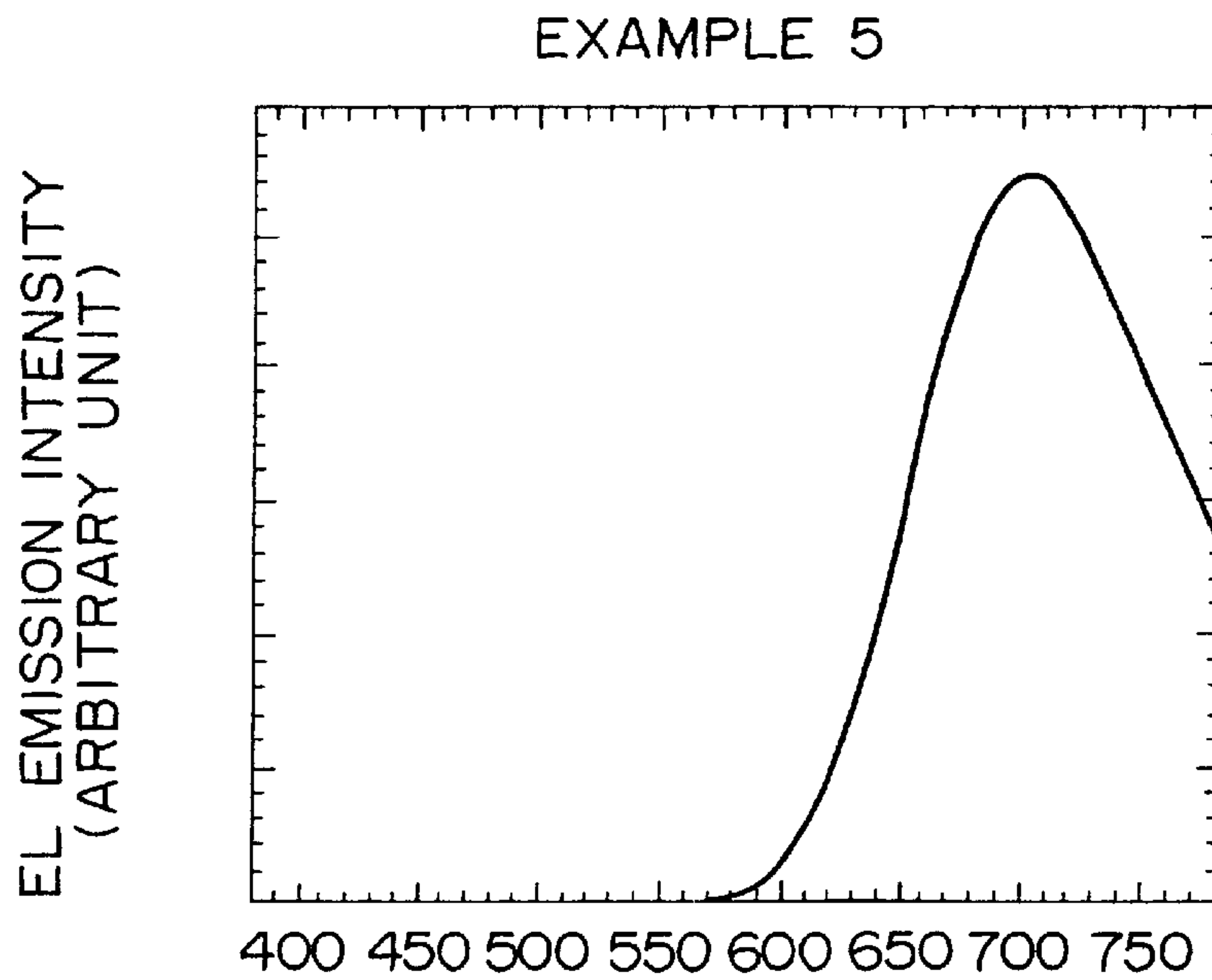
WAVELENGTH (nm) EL EMISSION SPECTRUM
