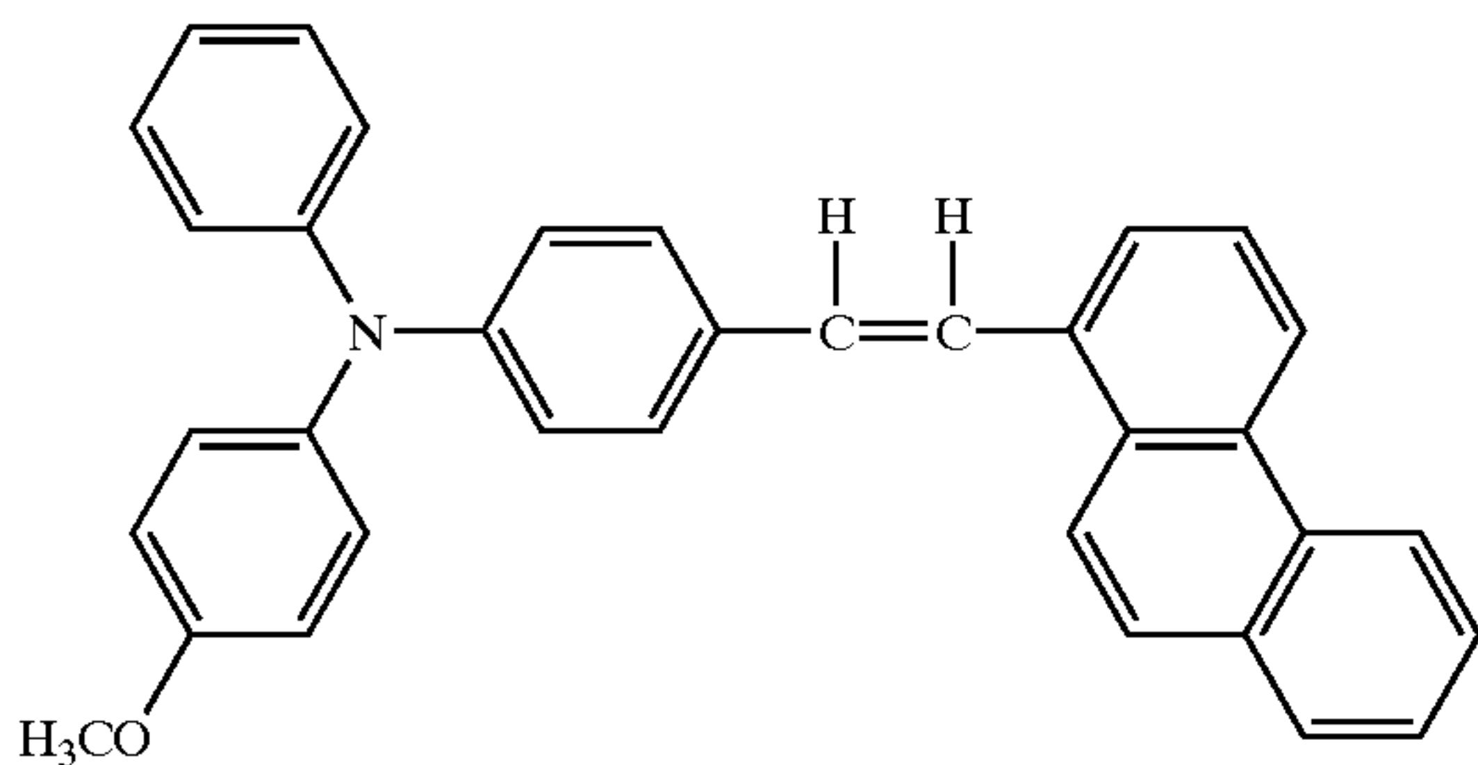
Structural Formula (20)-15:
