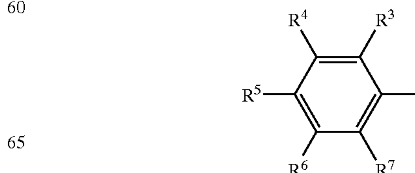
General Formula (2):
