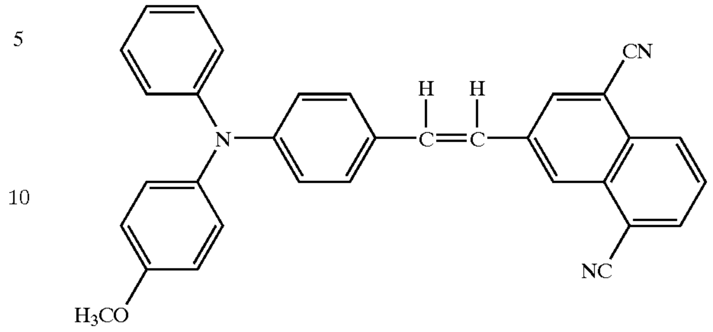
15 Structural Formula (20)-9:
