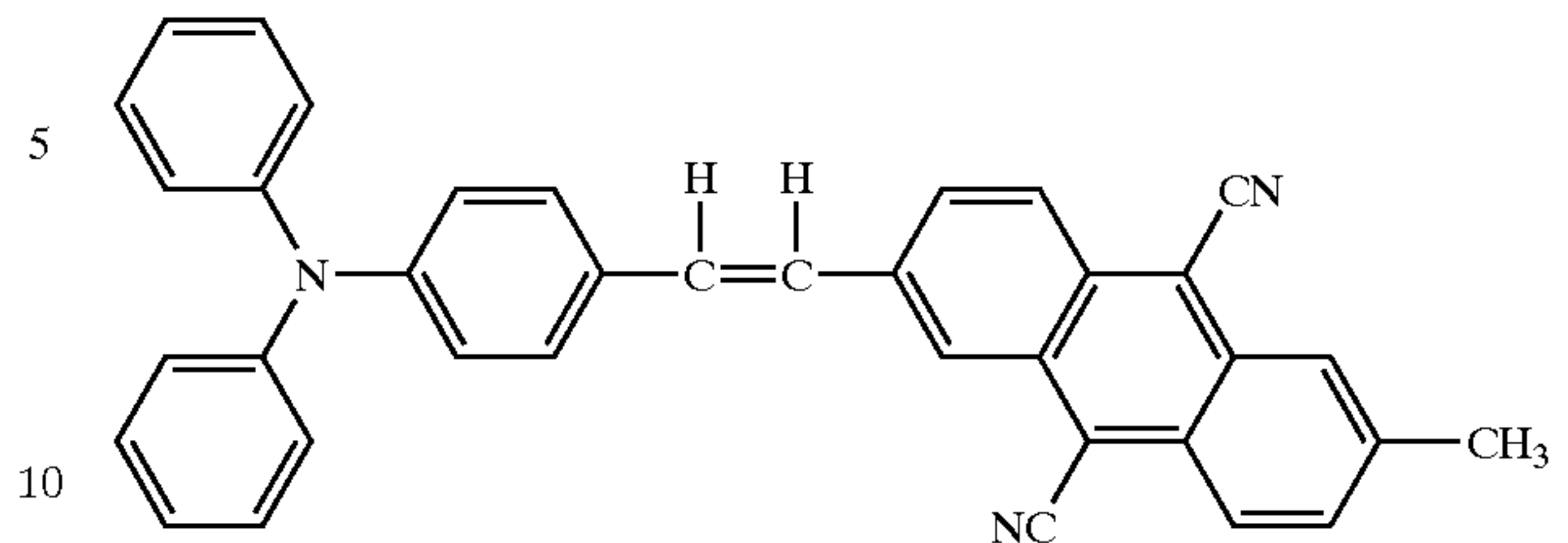
Structural Formula (20)-6:
