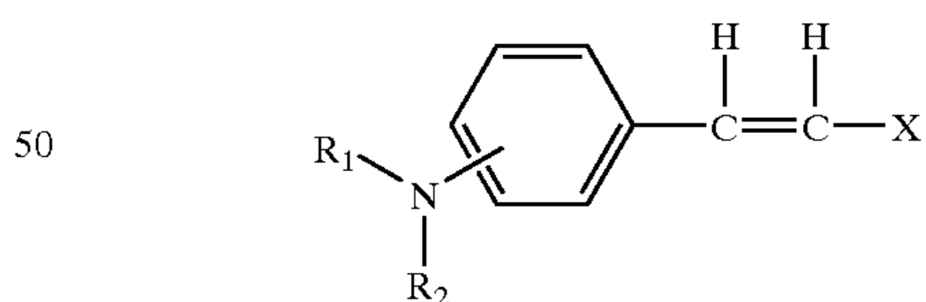
General Formula (1):
