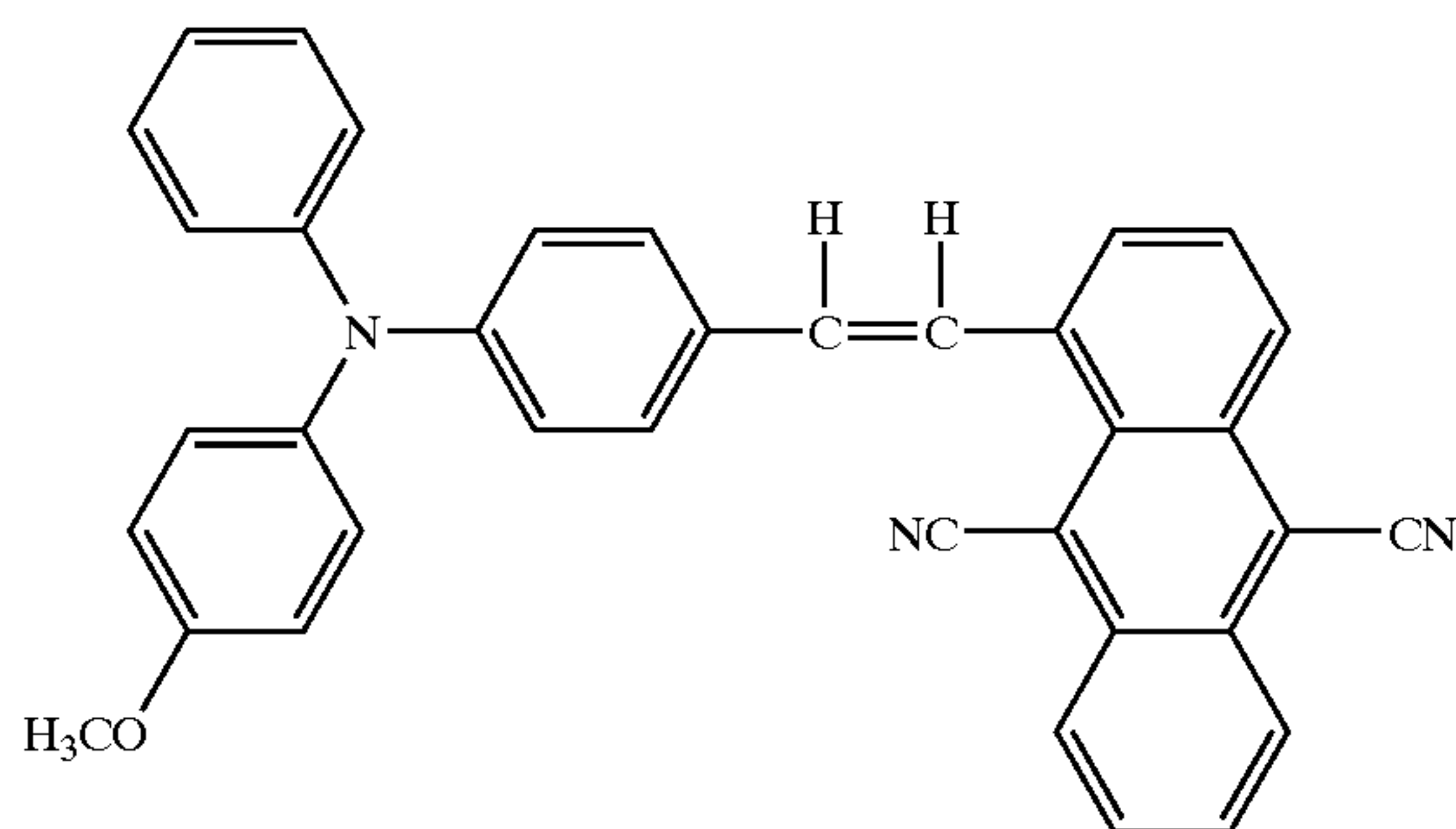
Structural Formula (20)-10:
