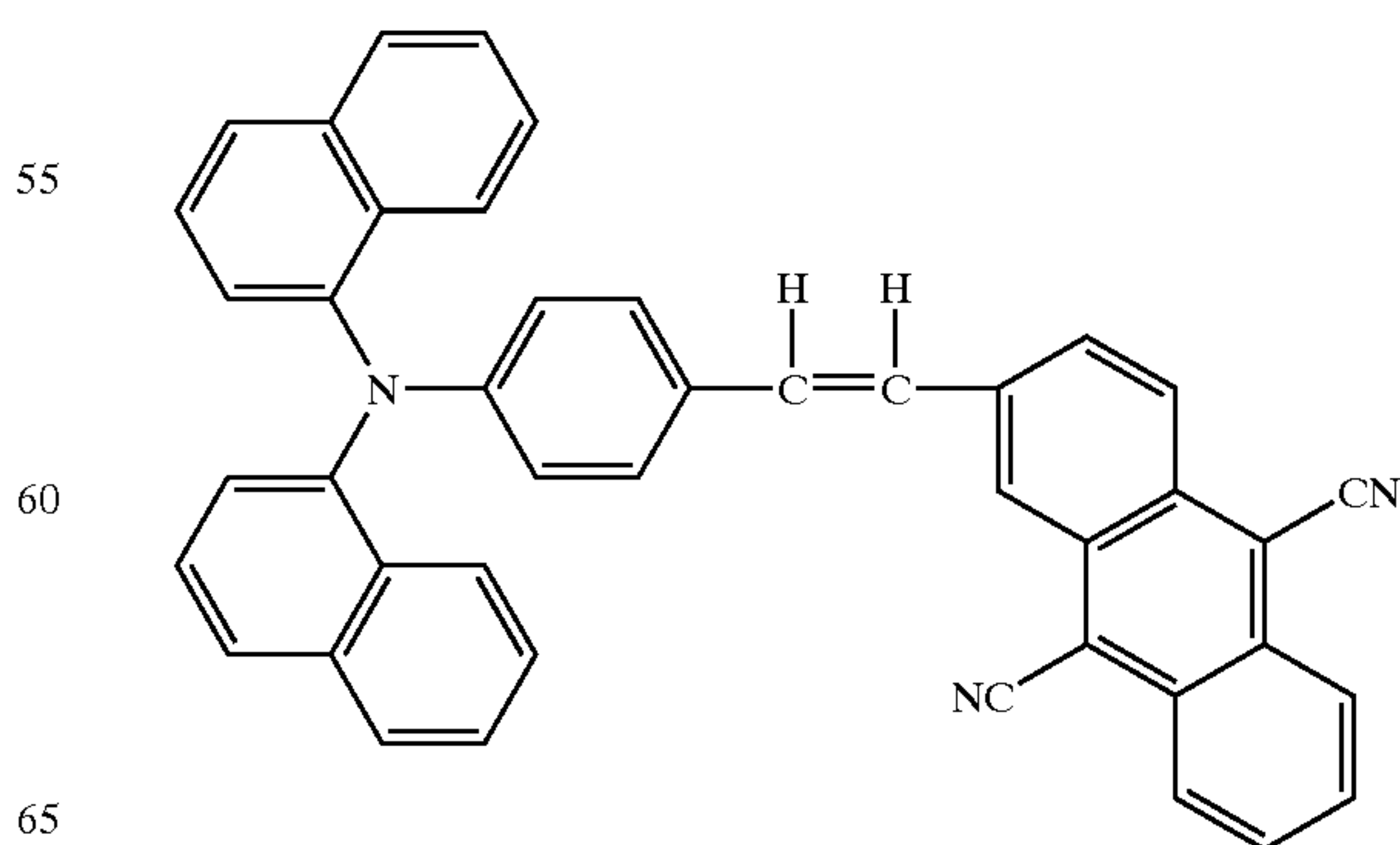
Structural Formula (20)-4:
