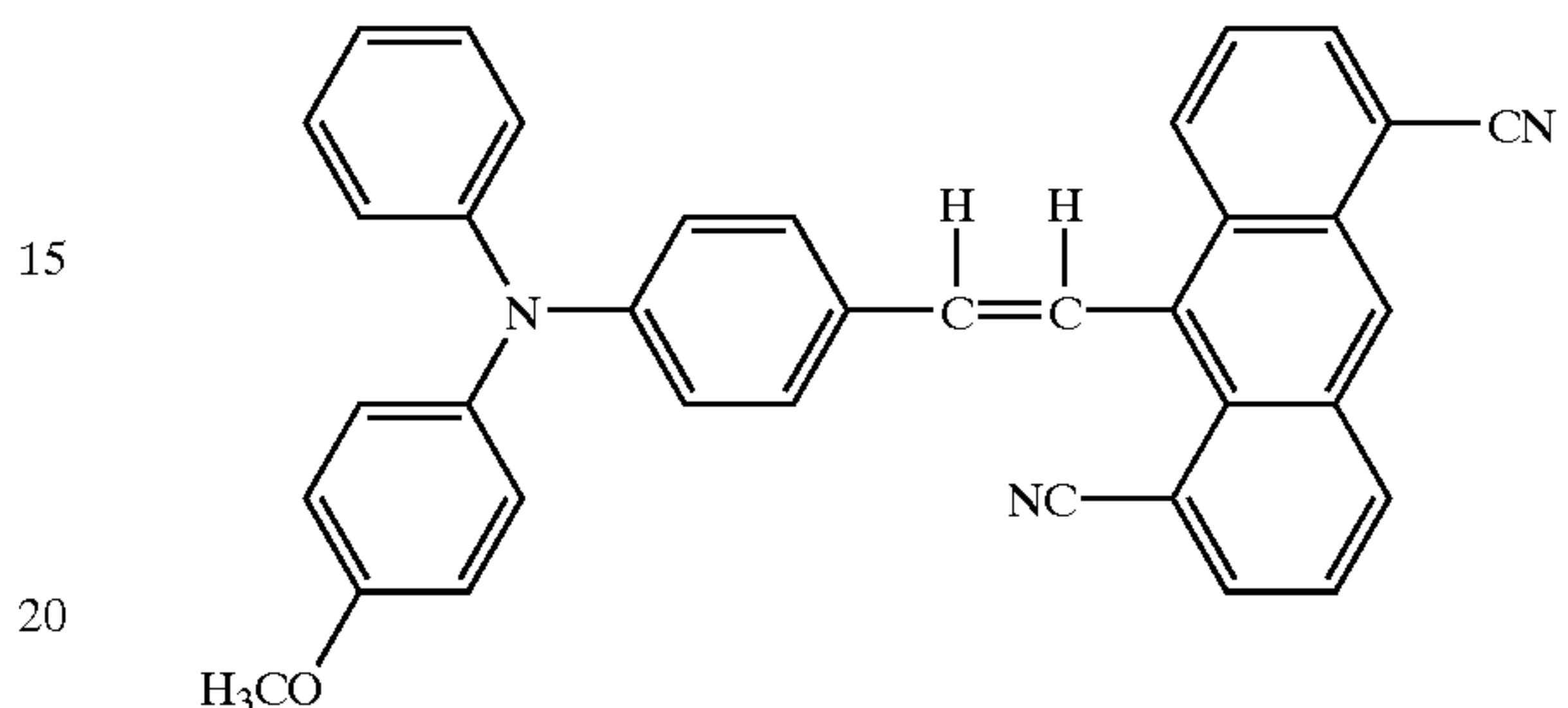
Structural Formula (20)-11:
