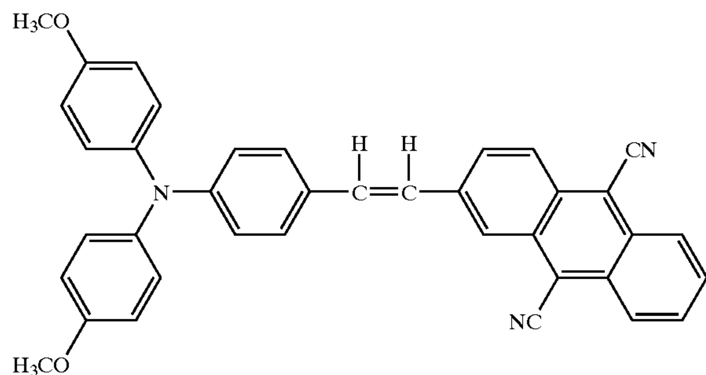
Structural Formula (20)-5:
