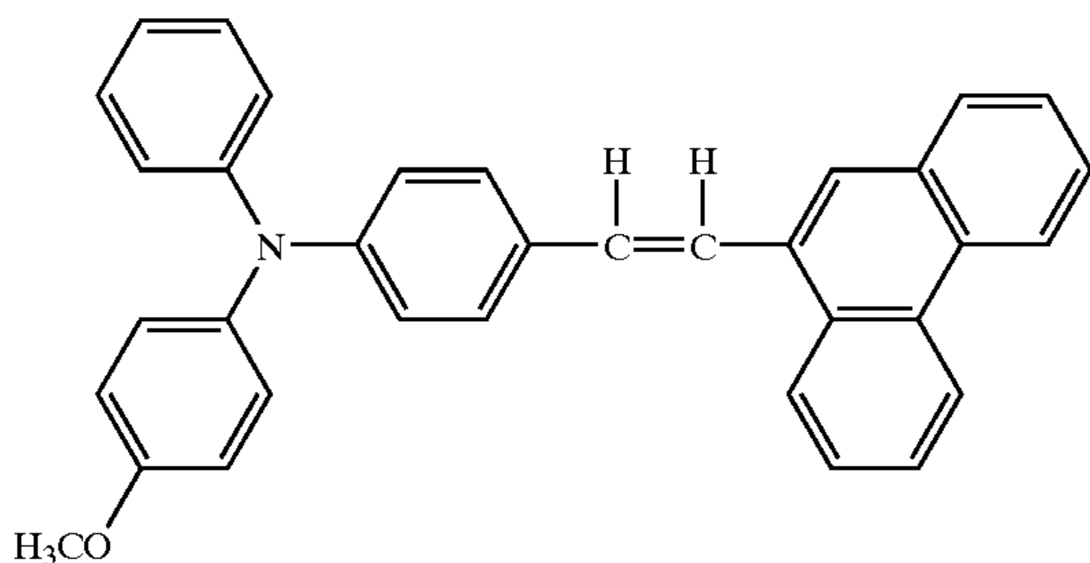
Structural Formula (20)-16:
