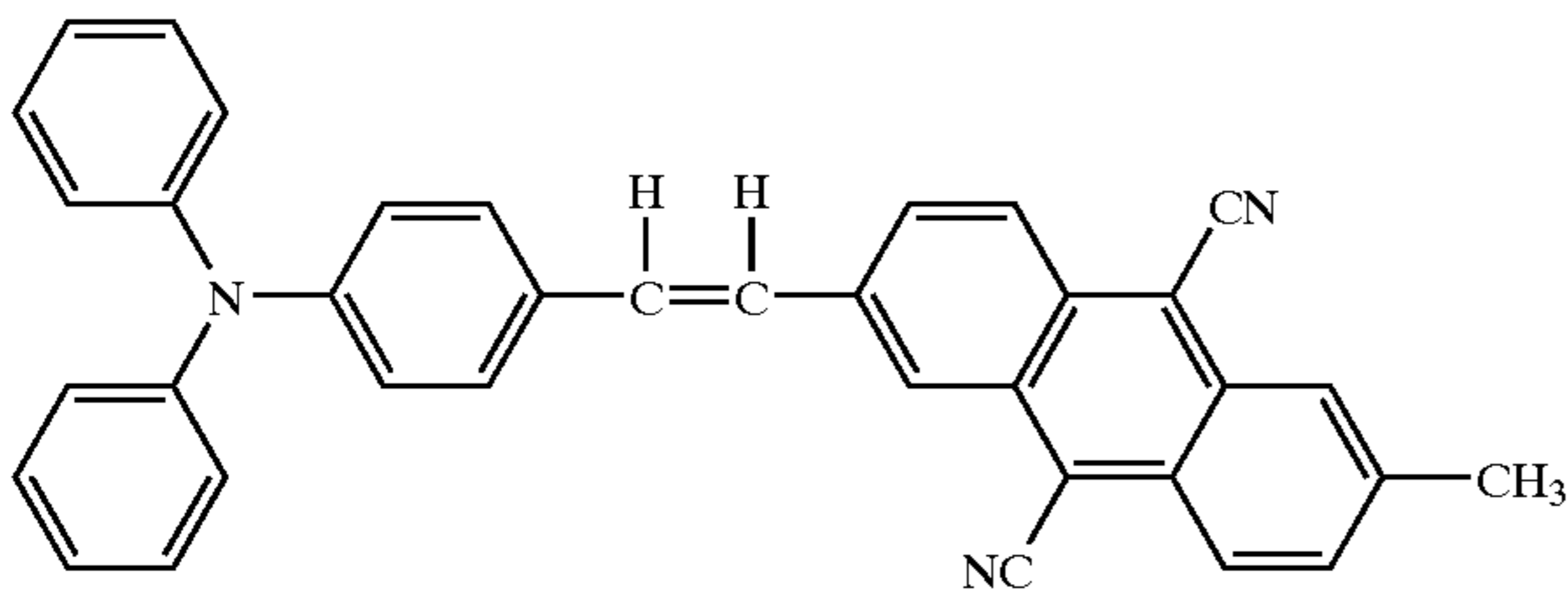
Structural Formula (20)-7:
