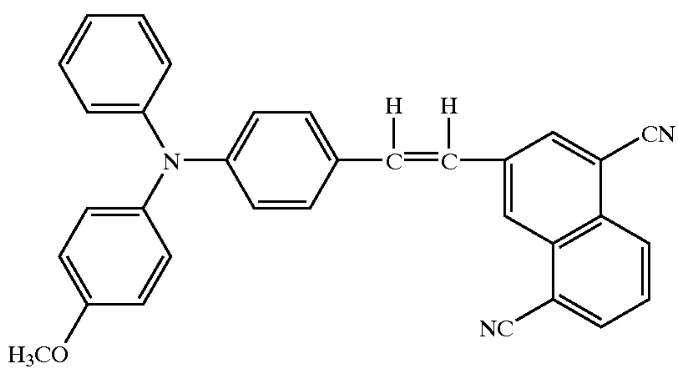
Structural Formula (20)-9:
