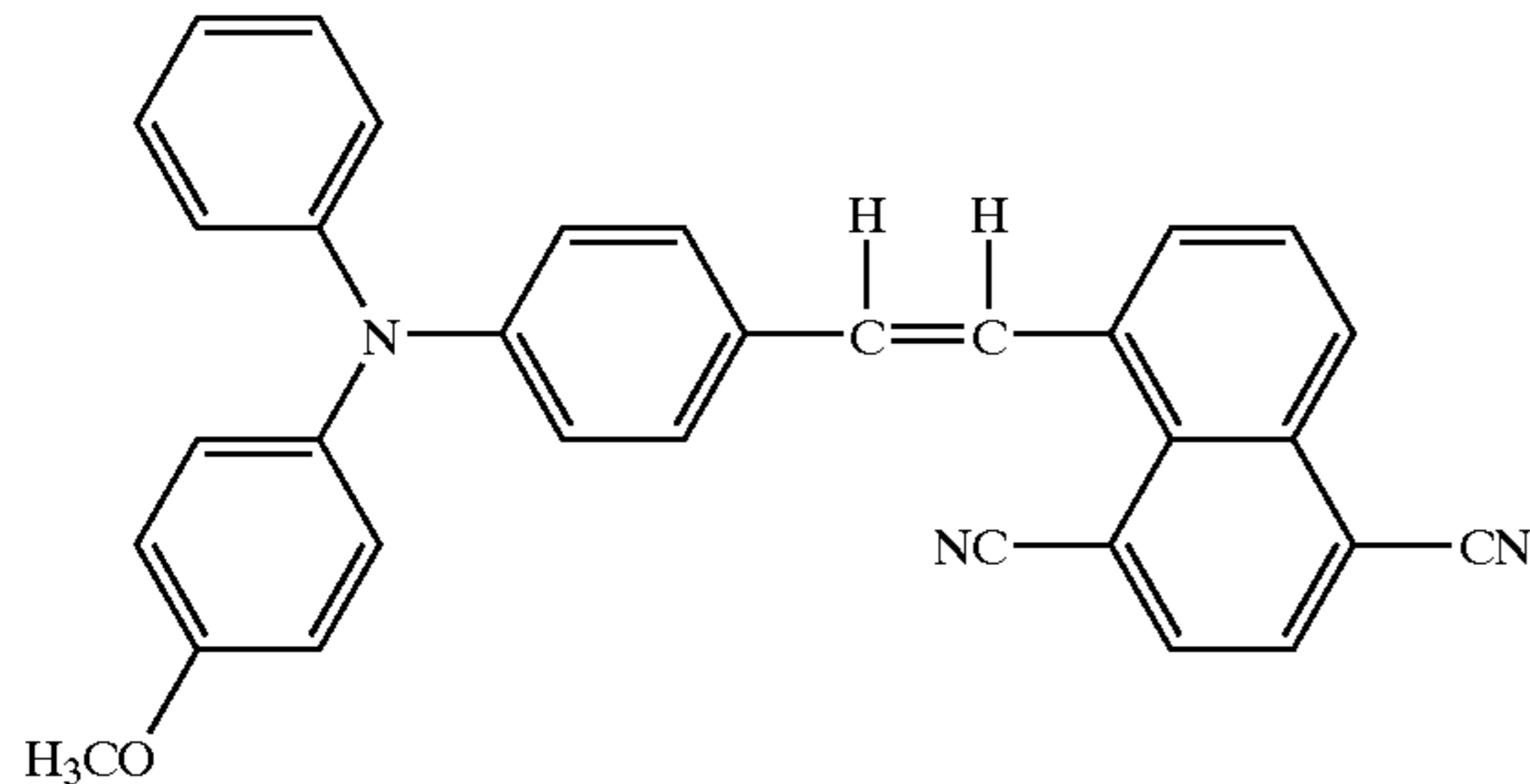
Structural Formula (20)-9:
