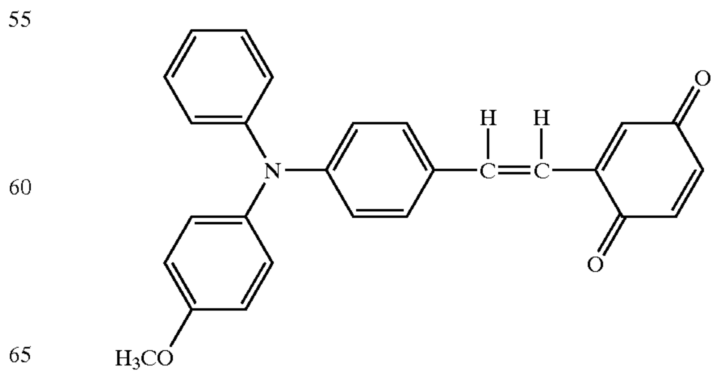
Structural Formula (20)-18:
