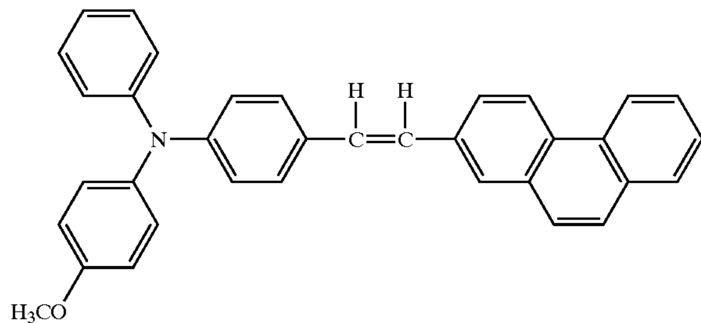
Structural Formula (20)-13:
