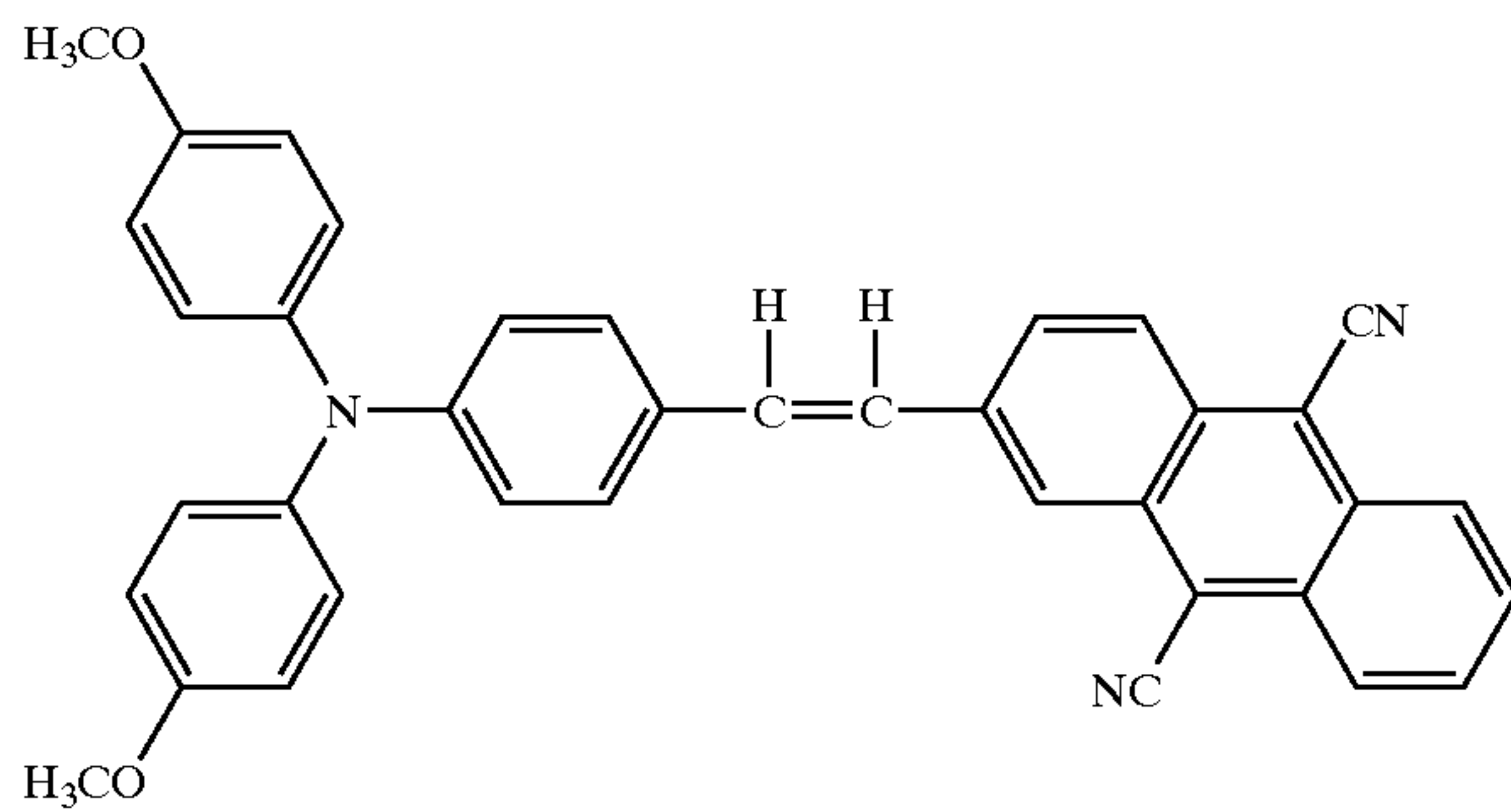
Structural Formula (20)-6:
