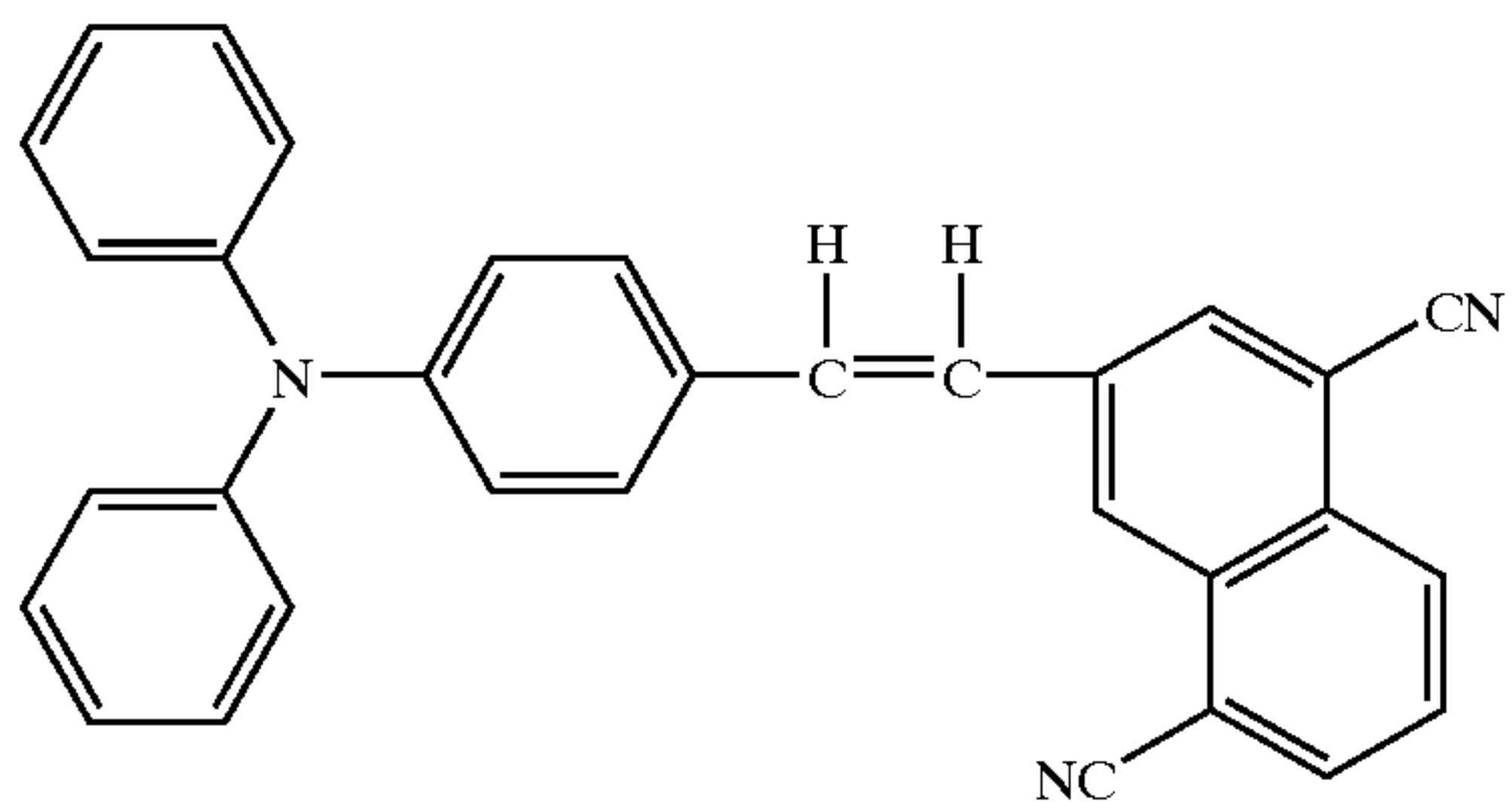
Structural Formula (20)-8:
