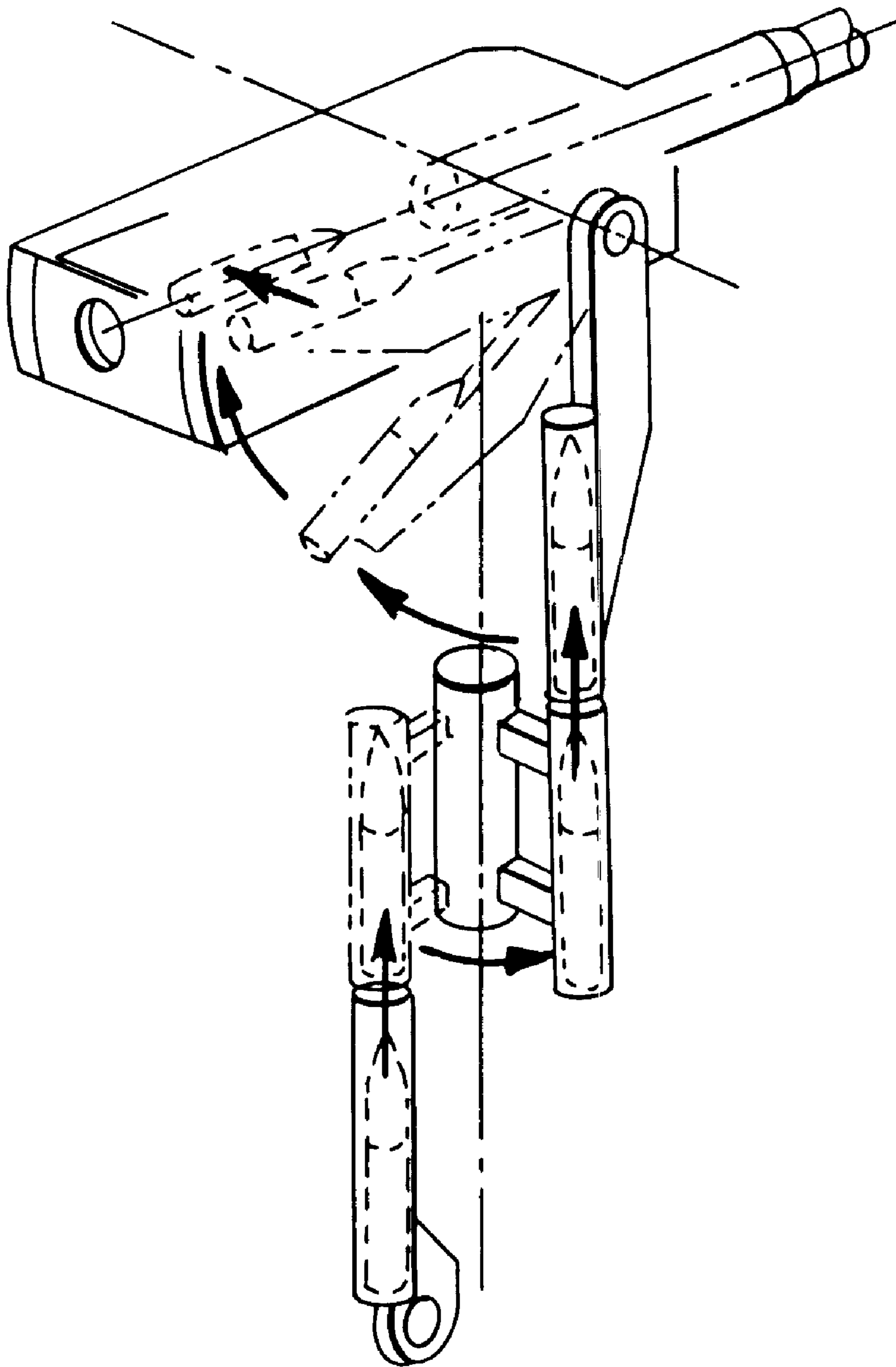
Fig. 7 PRIOR ART
