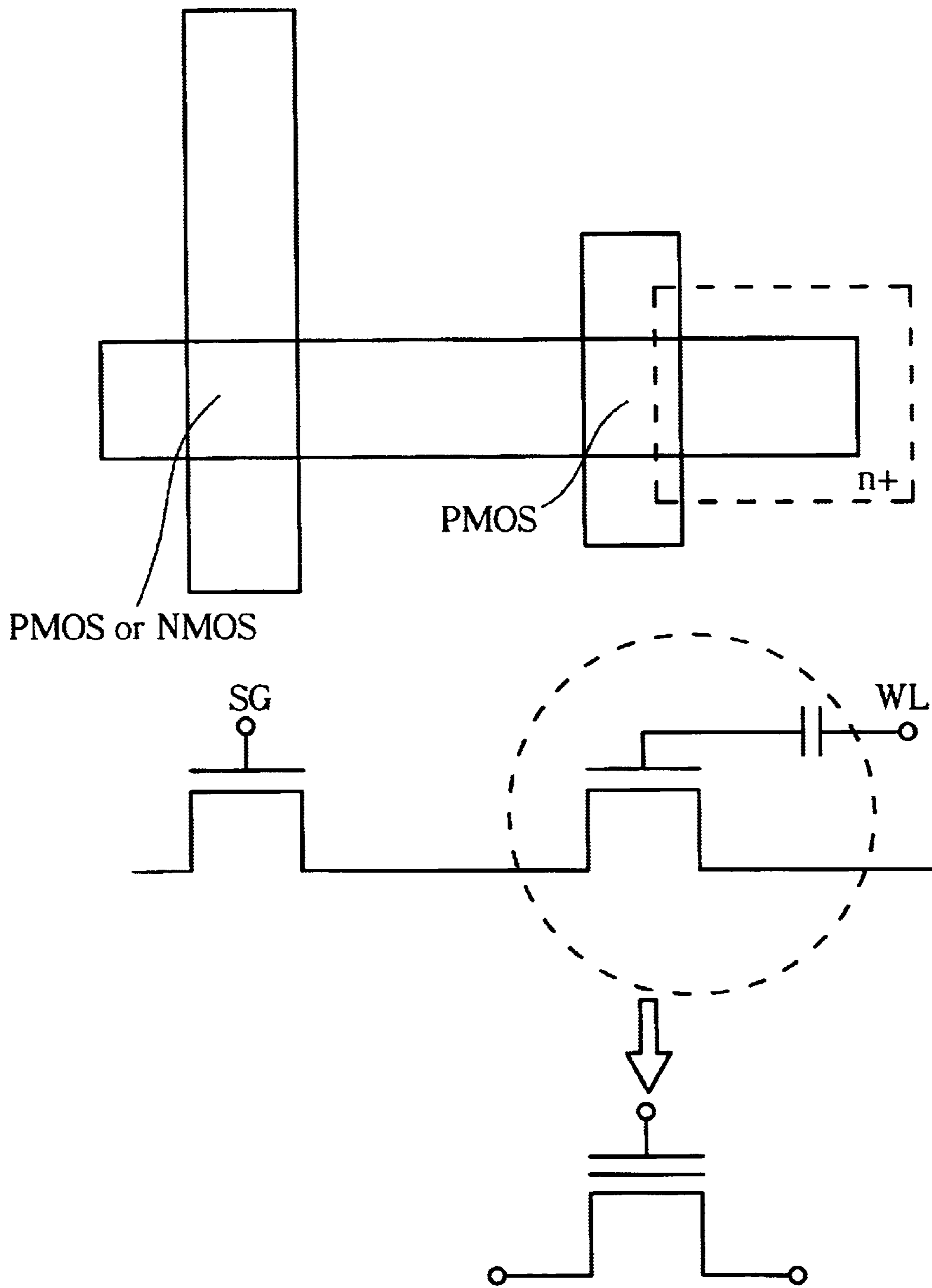
Fig. 2 Prior Art
