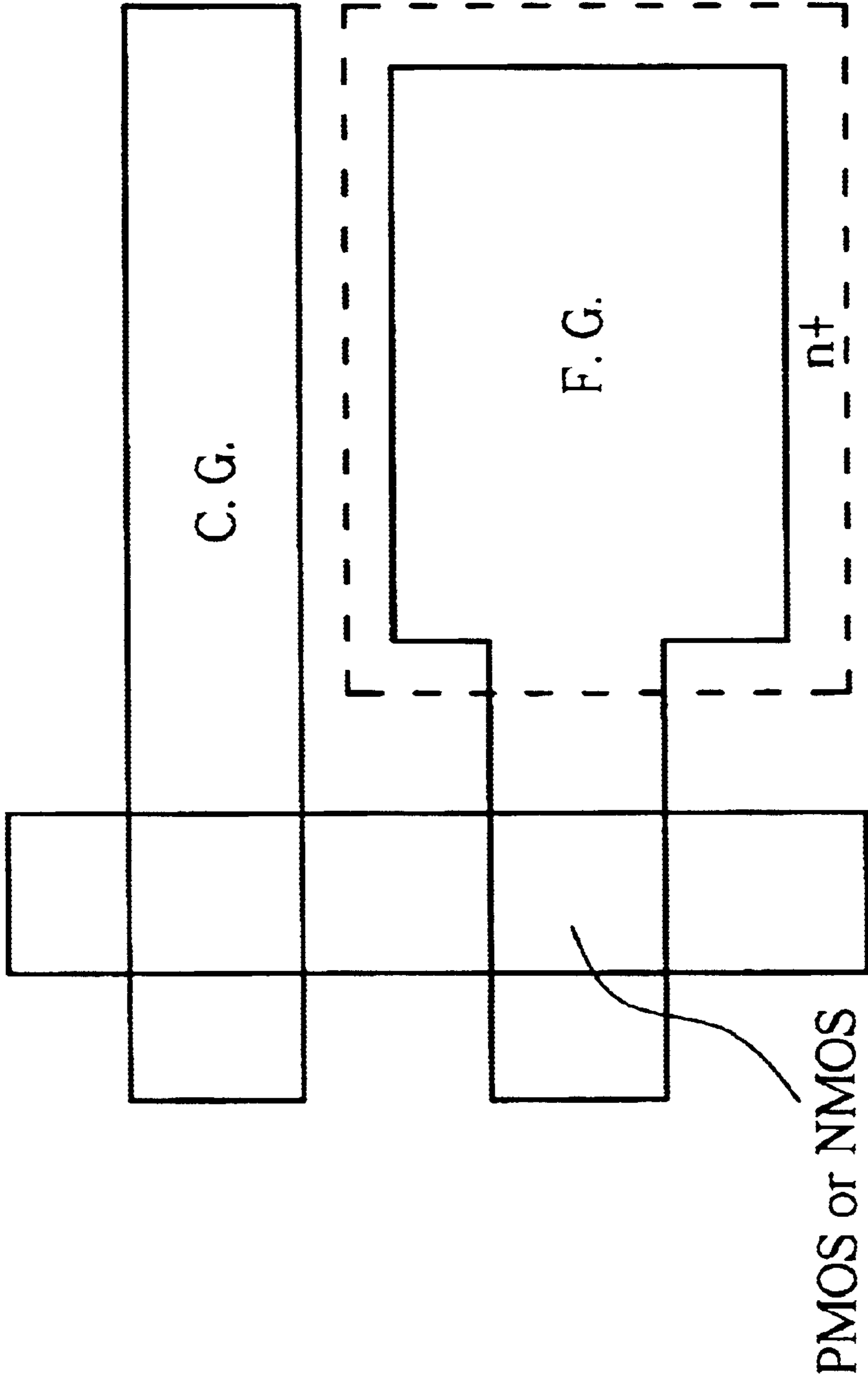
Fig. 1 Prior Art
