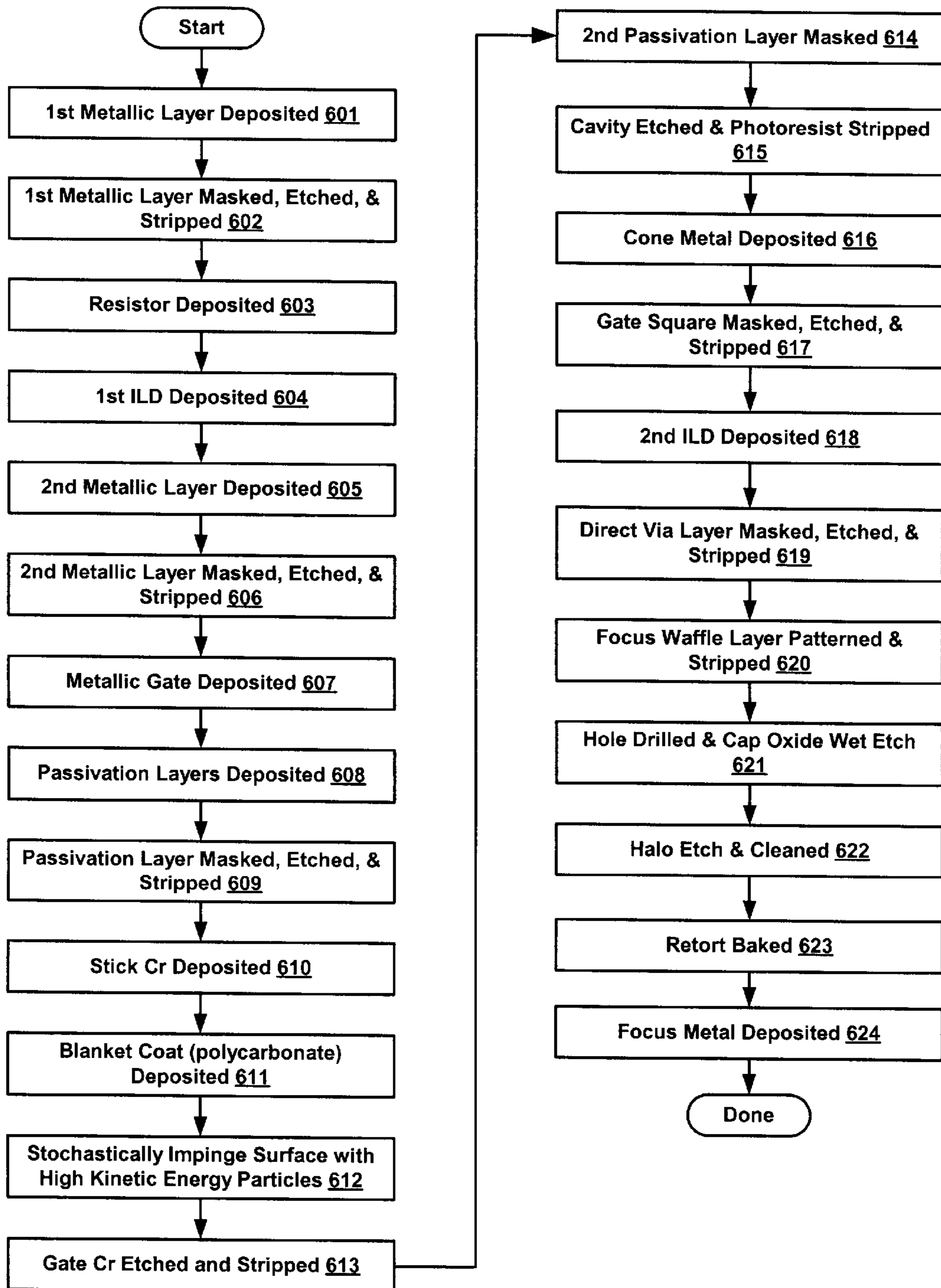
FIG. 6 (CONVENTIONAL ART)
