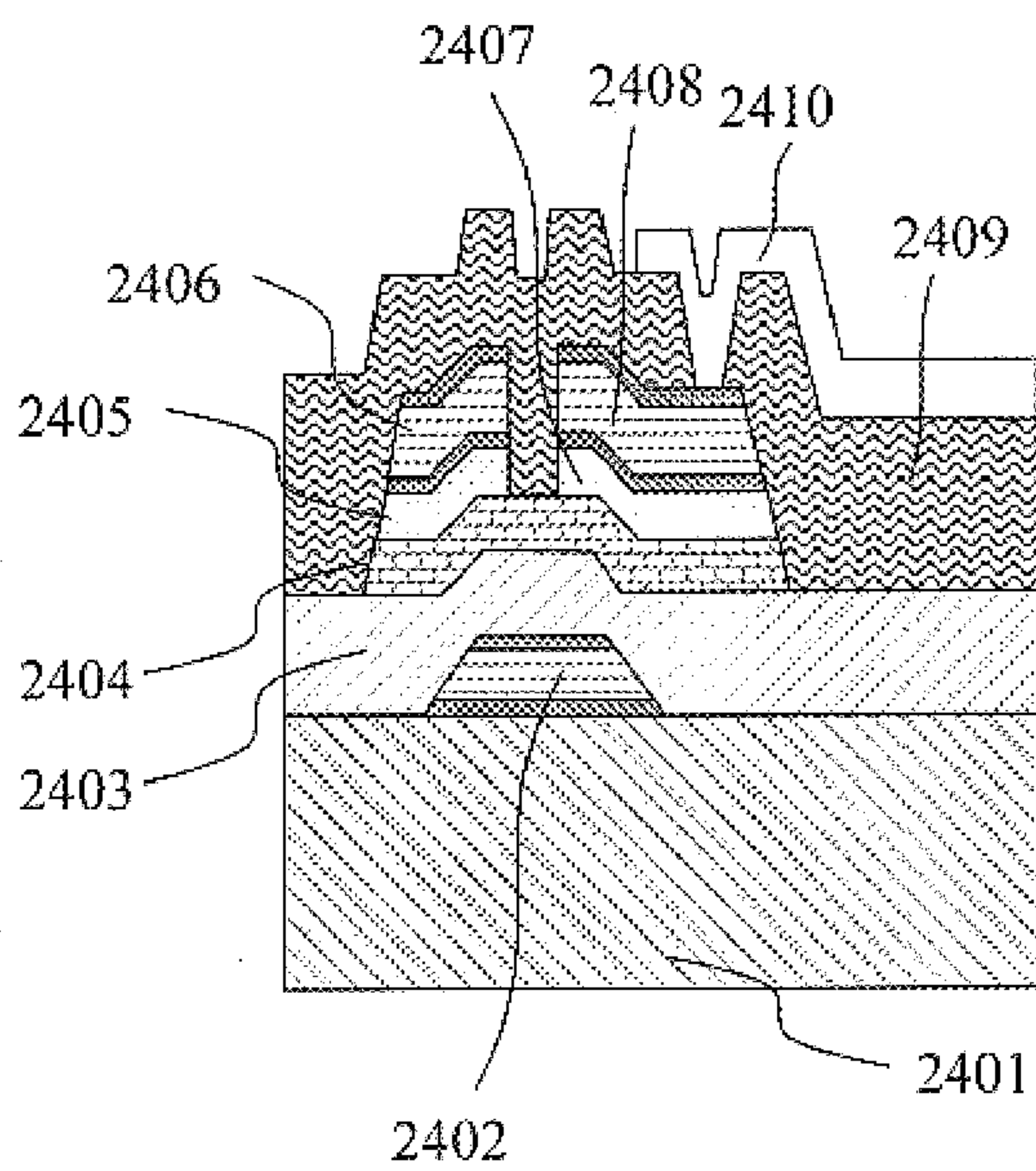
CONVENTIONAL DEVICE STRUCTURE
