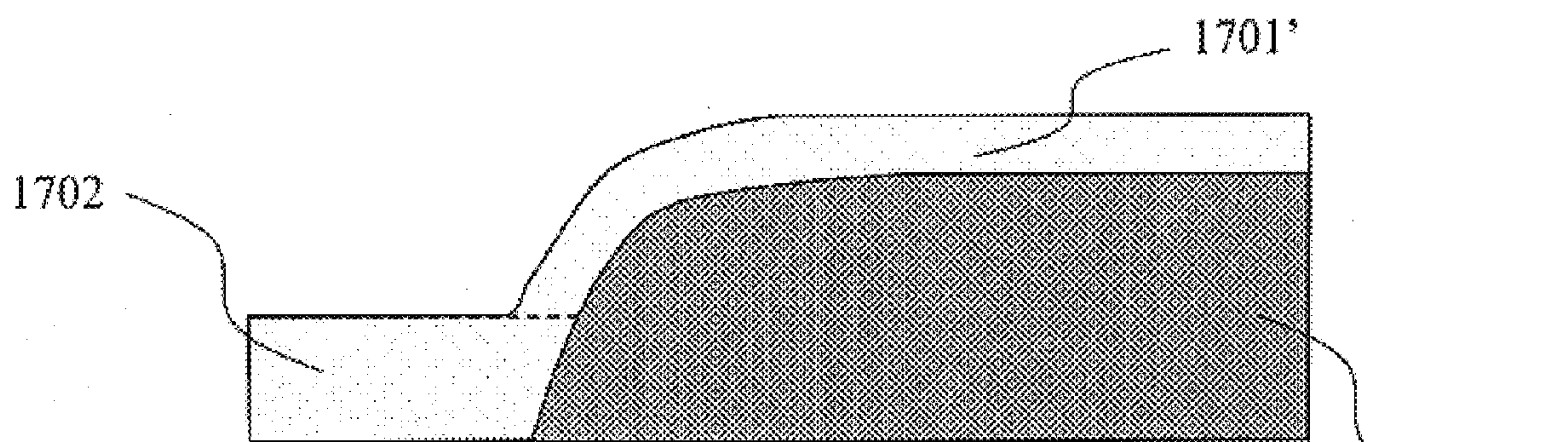
THIS INVENTION (PLASMA OXIDATION USING Kr)
