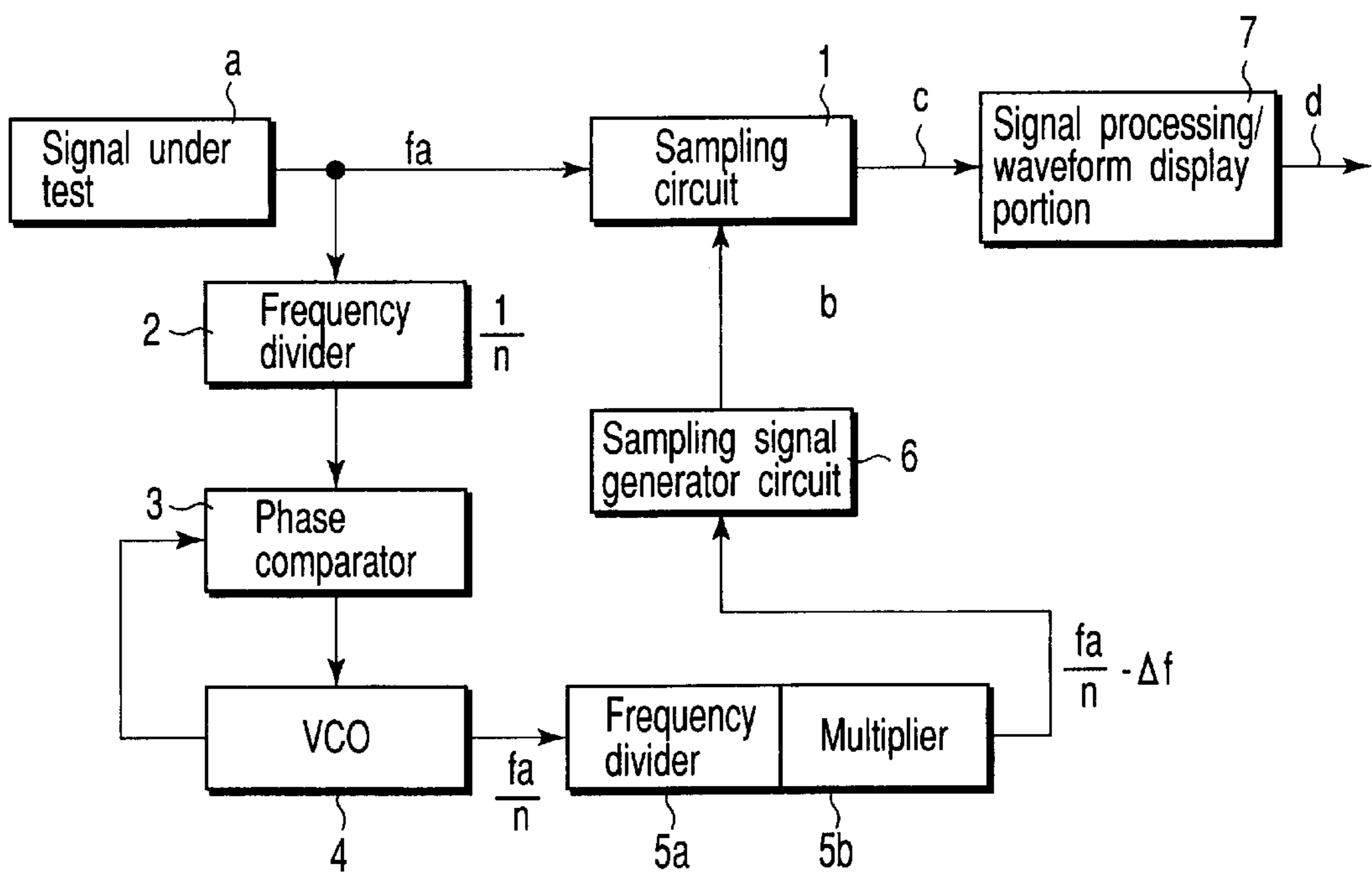
FIG. 8 PRIOR ART
