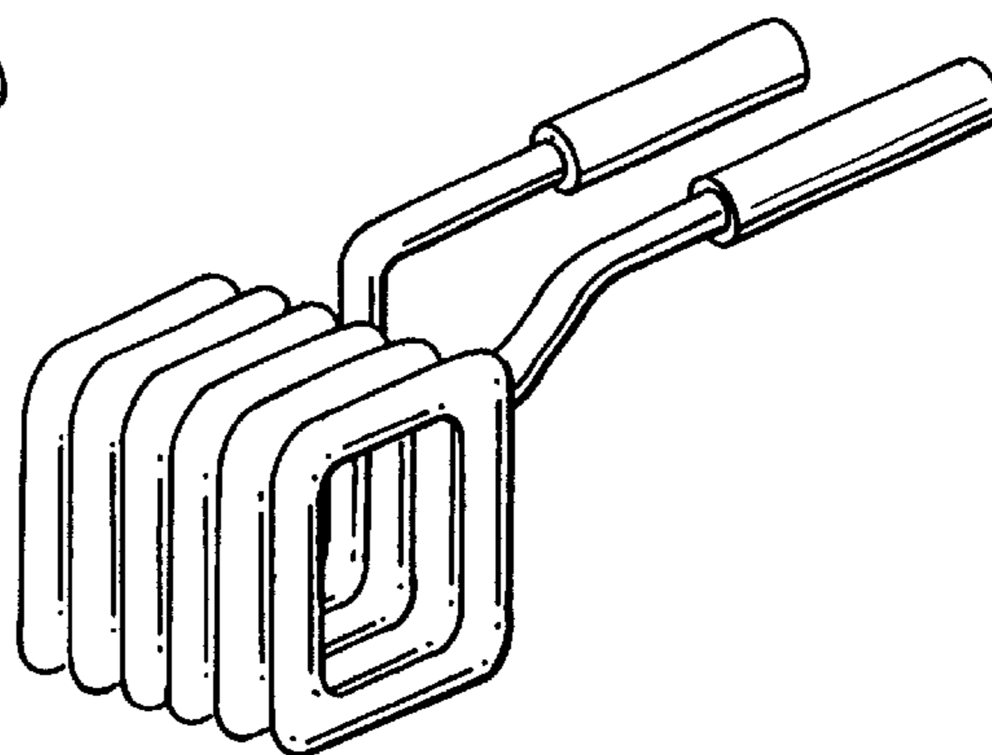
RECTANGULAR FIG.2b
