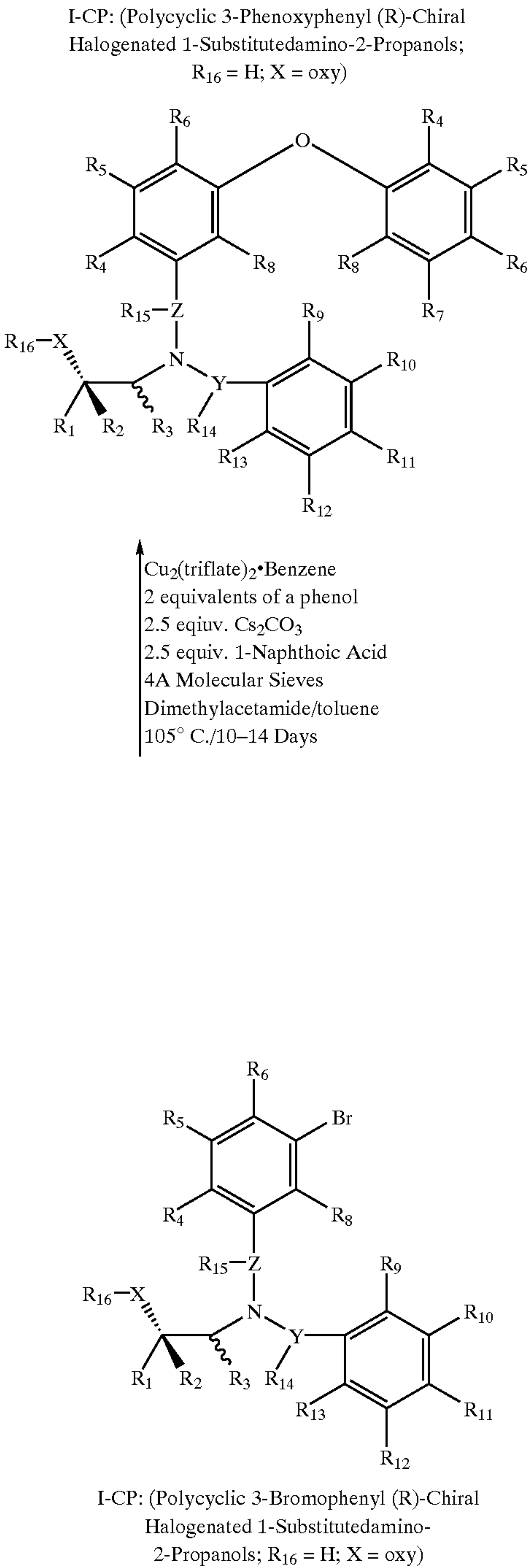
Scheme 8
