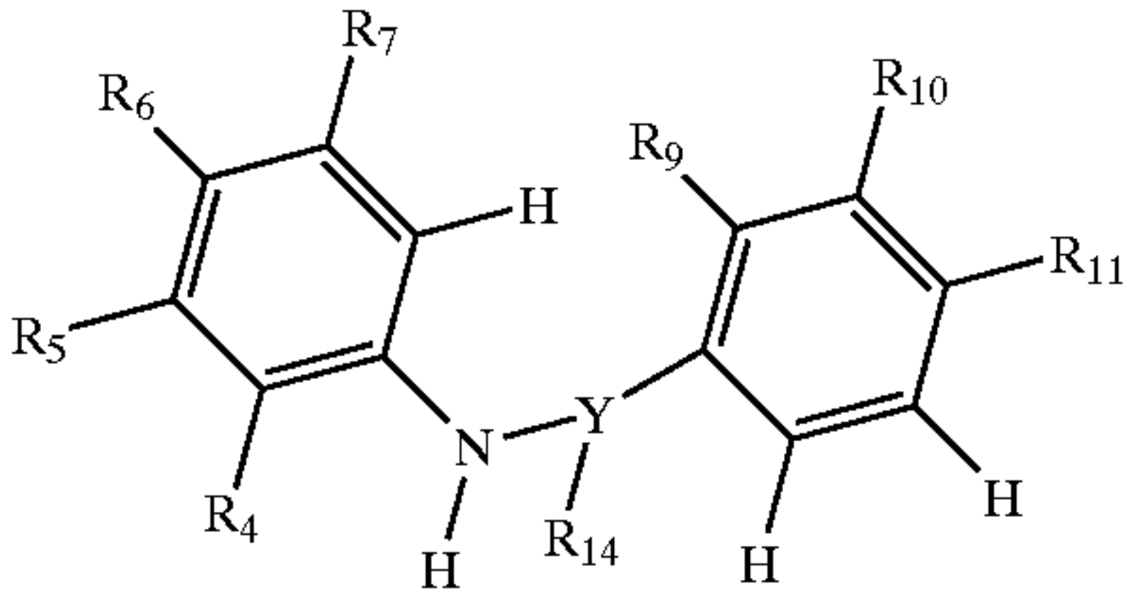
Secondary Phenyl Amine (XIIIA)
