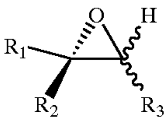
Structure of (R)-Chiral Oxirane Reagents.
