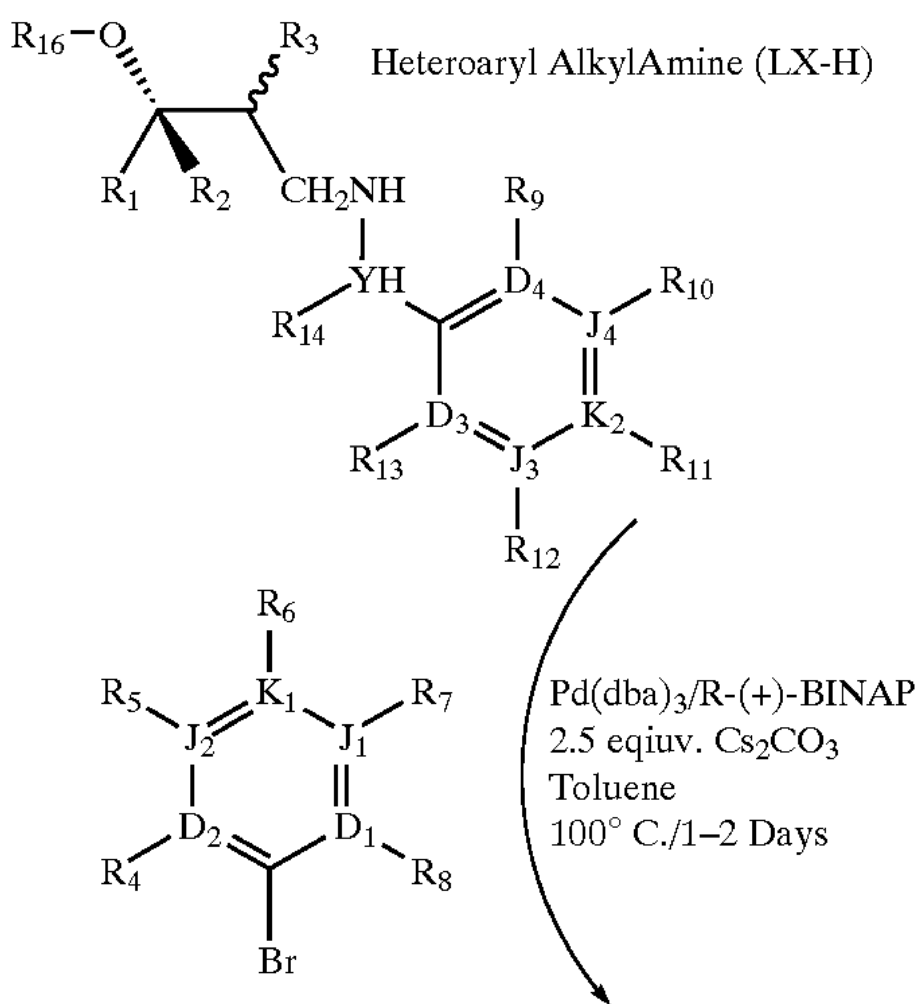
Scheme 32
