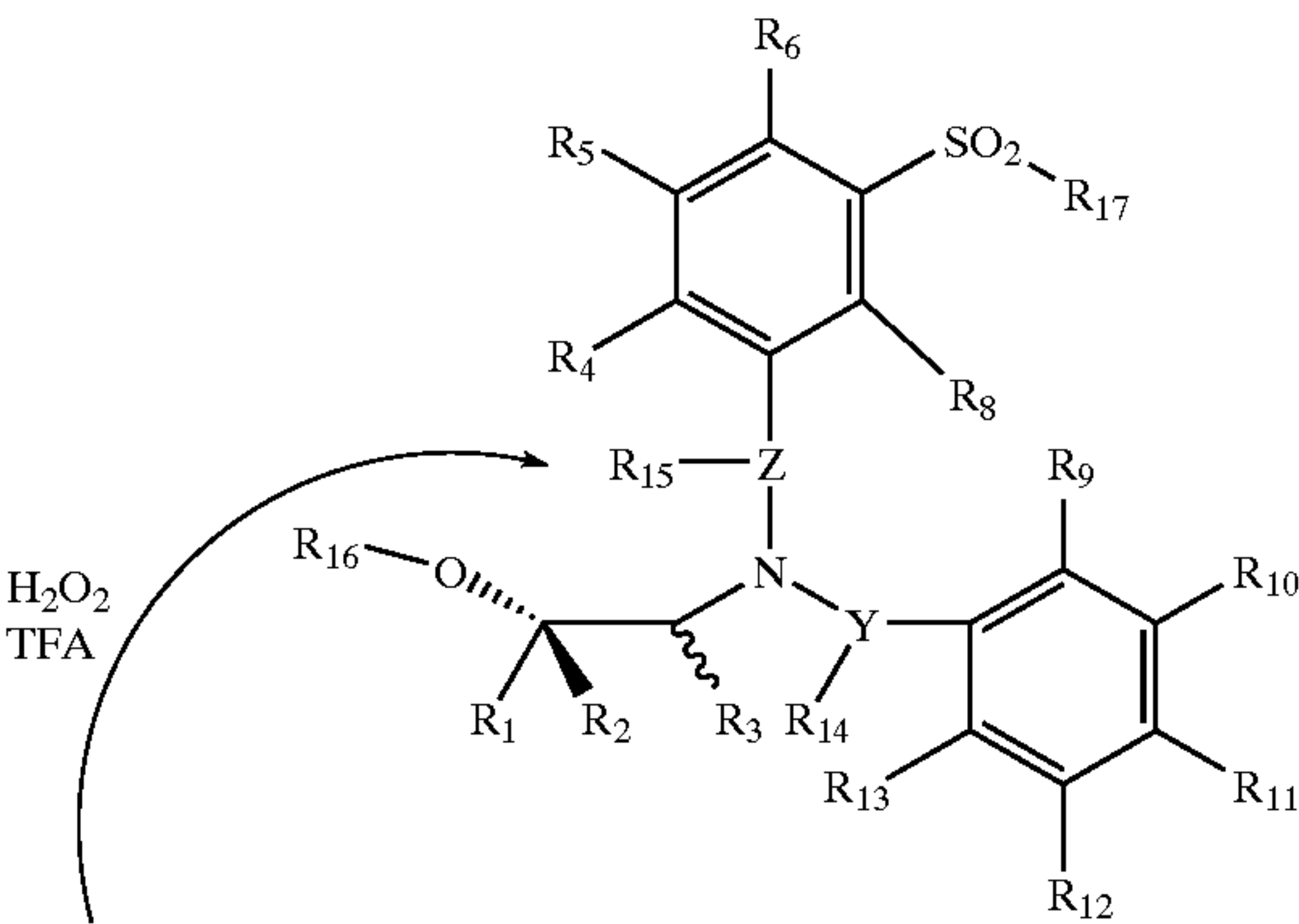
Scheme 19
