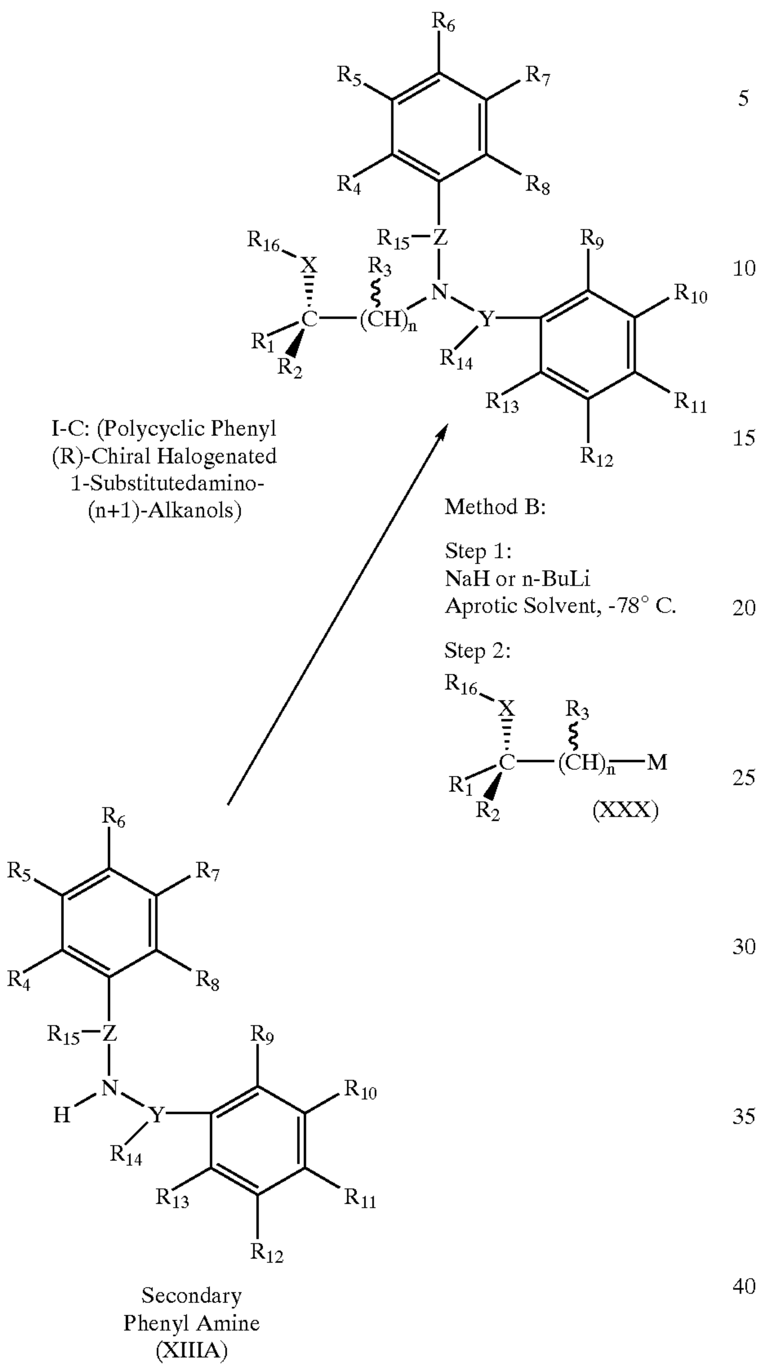
Scheme 5
