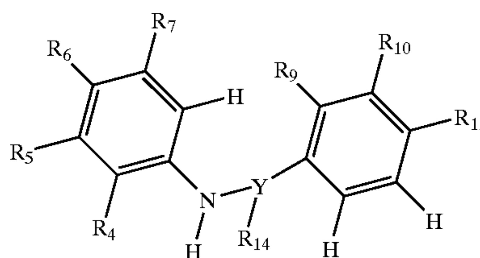
Secondary Phenyl Amine (XIIIA)
