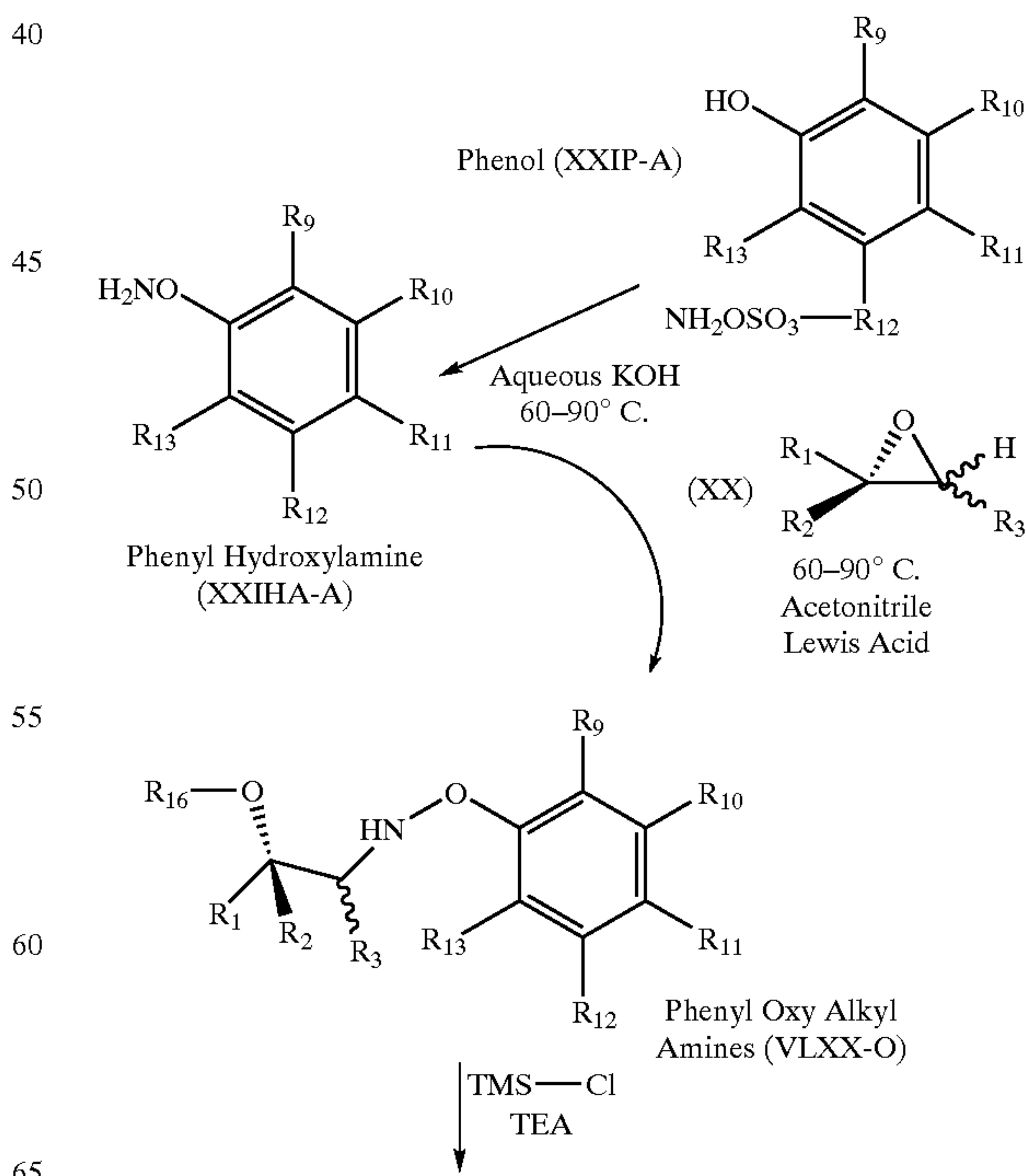
Scheme 58
