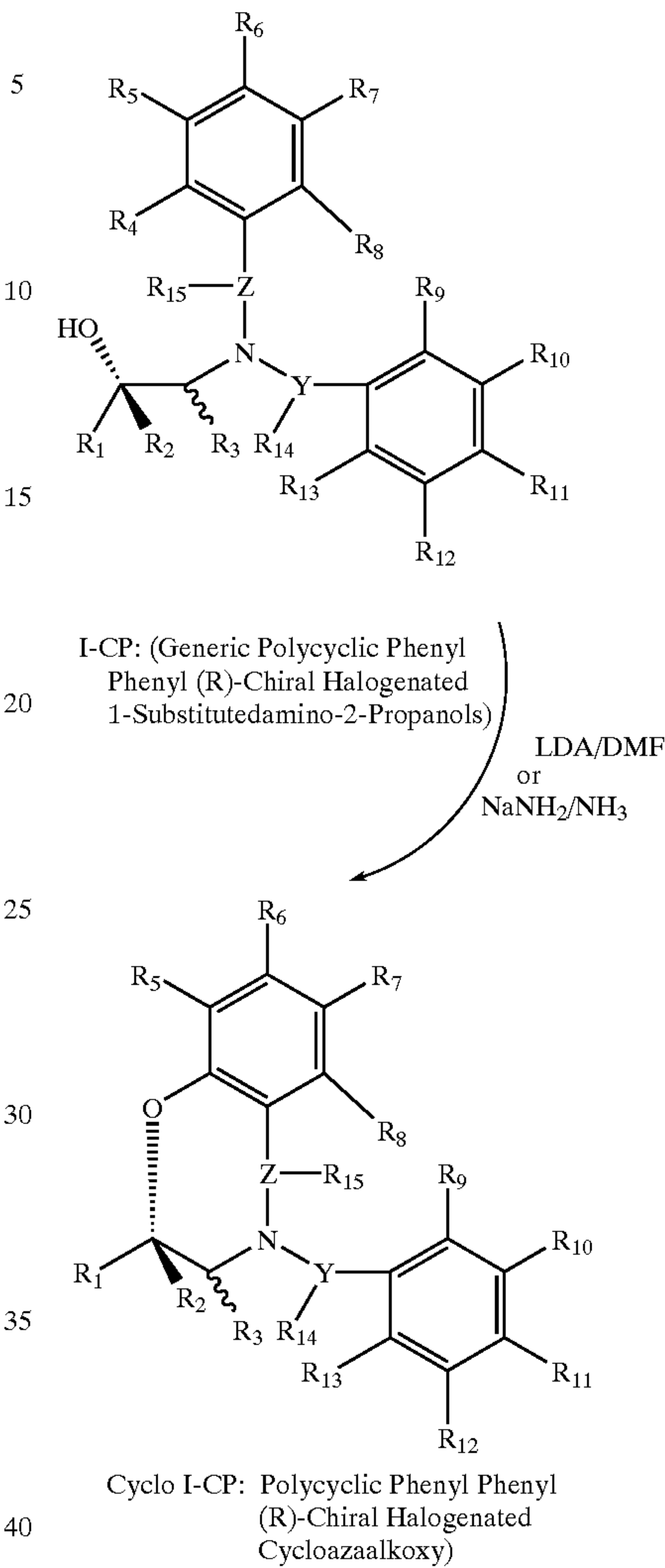
Scheme 18
