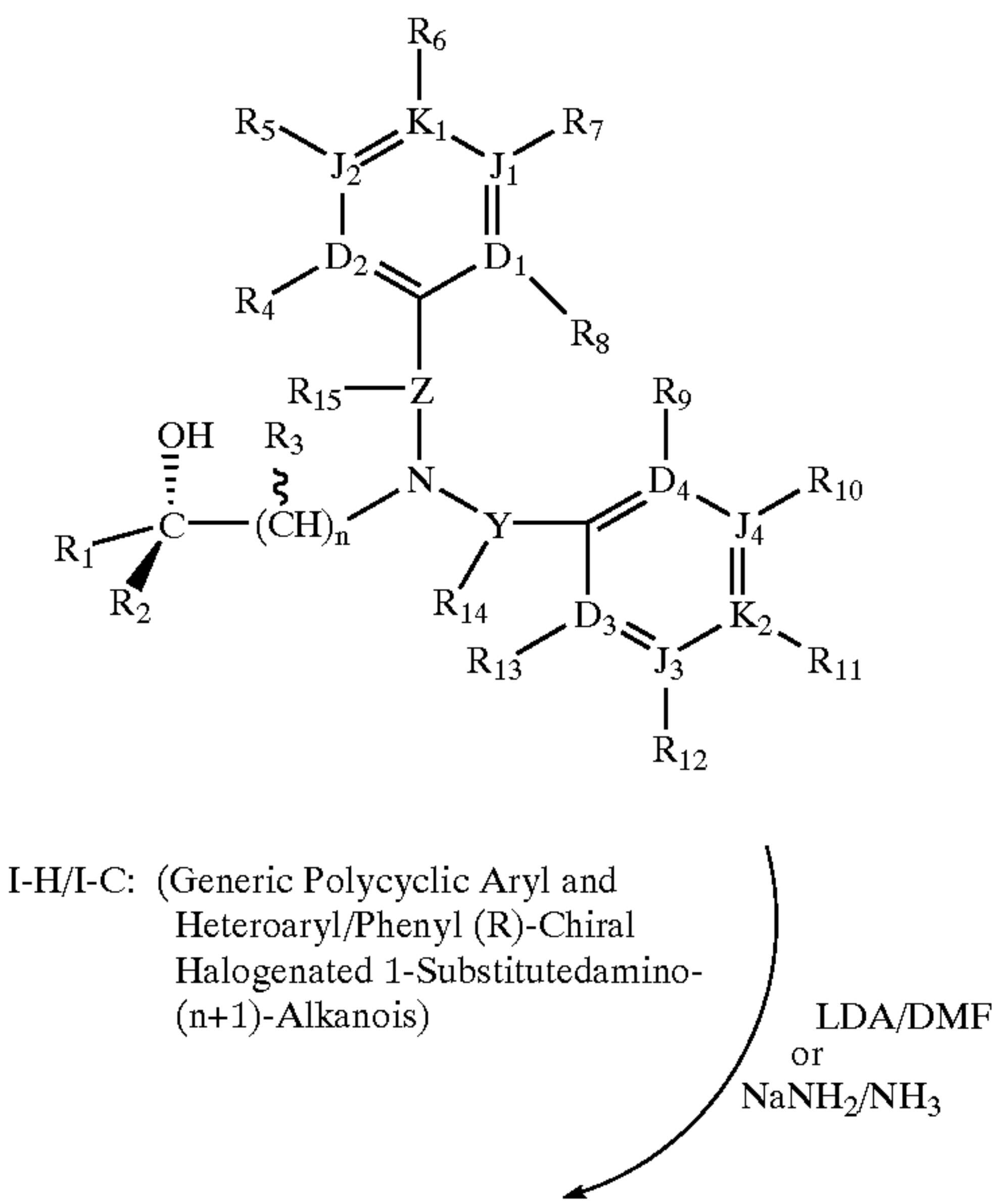
Scheme 17
