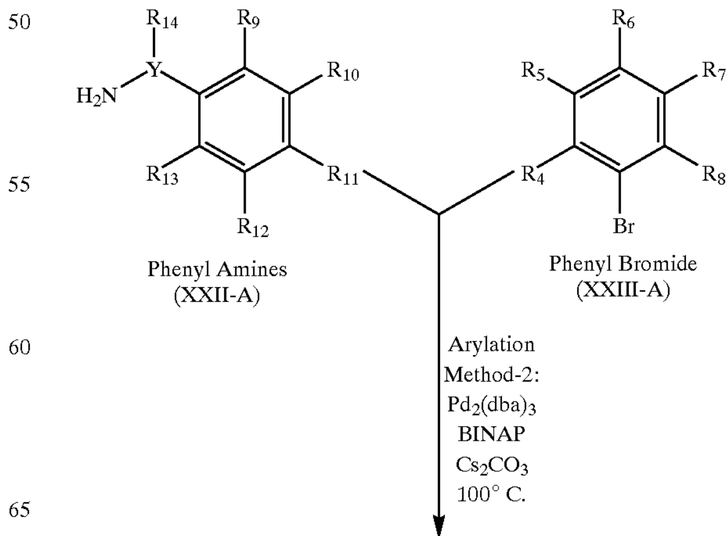
Scheme 10
