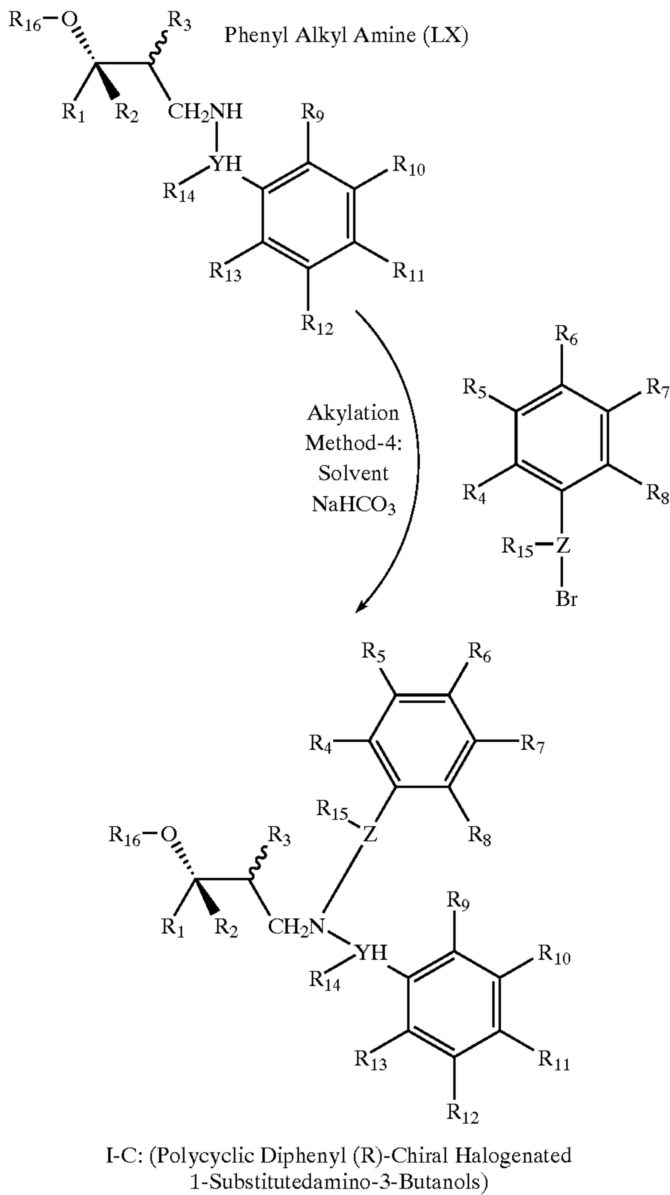
Scheme 34
