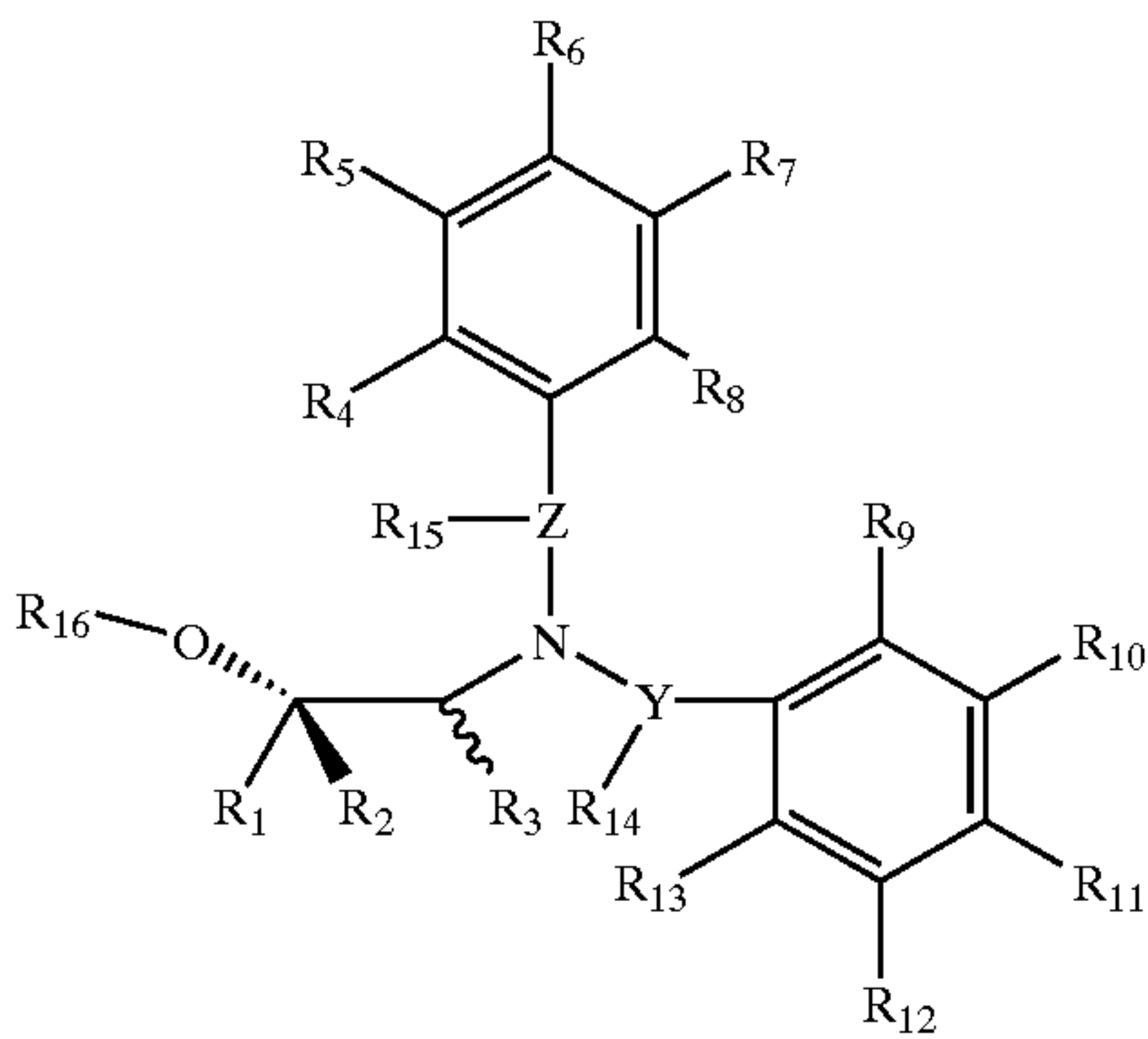
I-CP: (Polycyclic Phenyl (R)-Chiral Halogenated 1-Substitutedamino-2-Propanol; R 16 = H)
