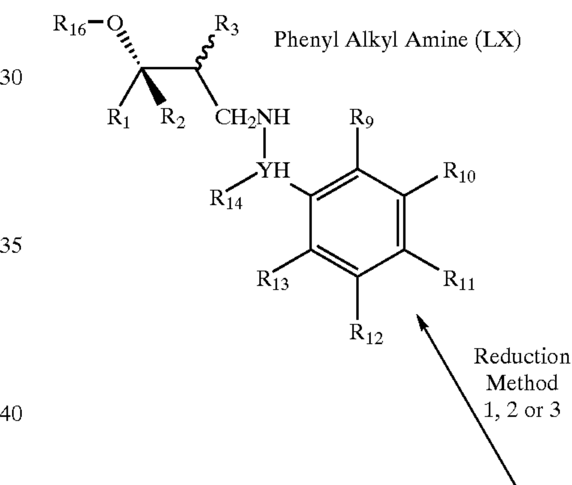
Scheme 33
