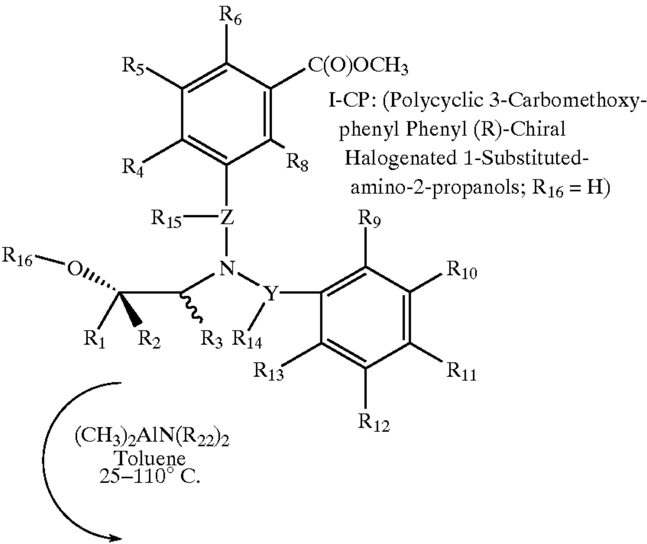
Scheme 27
