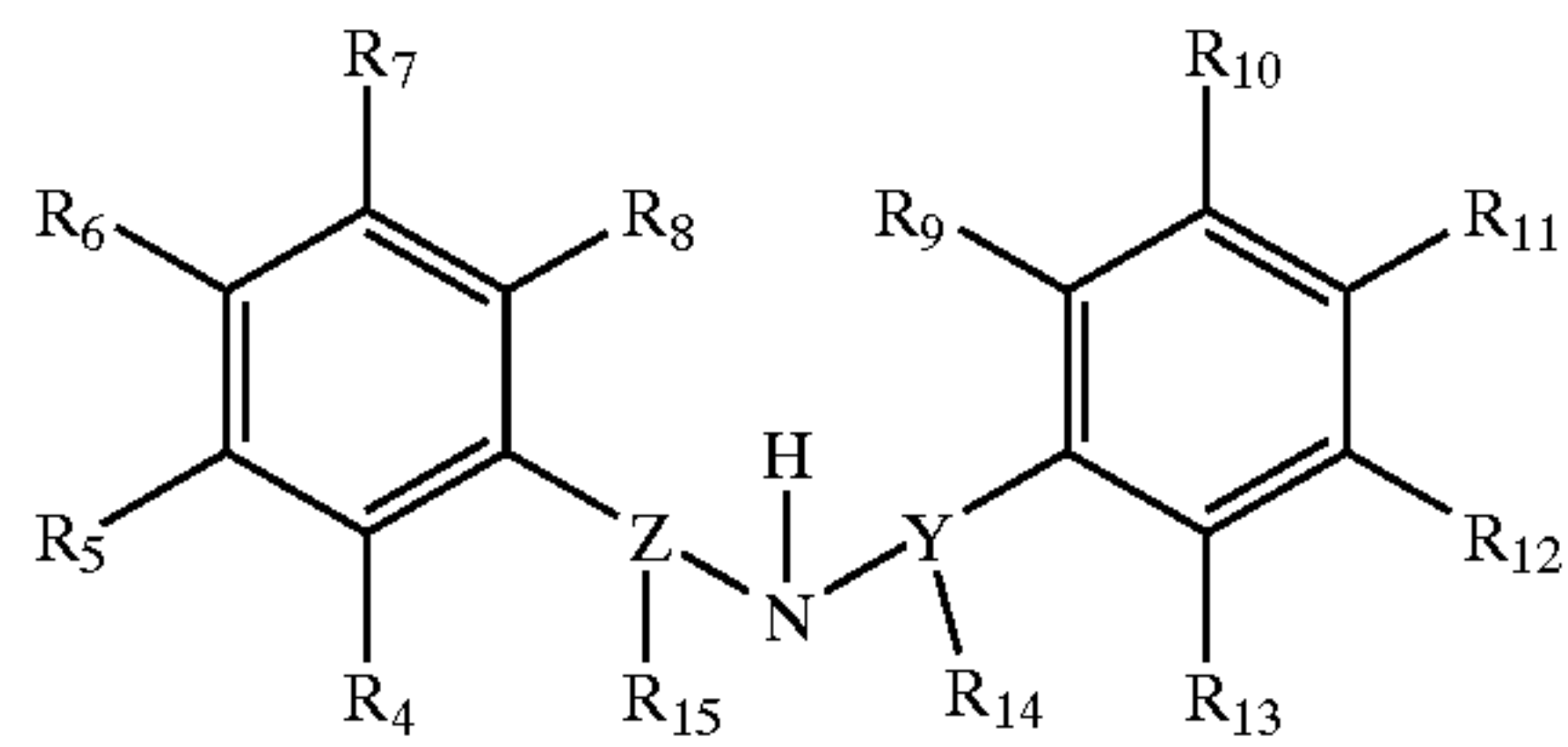
Structure of “Secondary Phenyl Amine” Reagents (Z is covalent bond; there is no R 15 substituent; R 4 and R 13 equal H).
