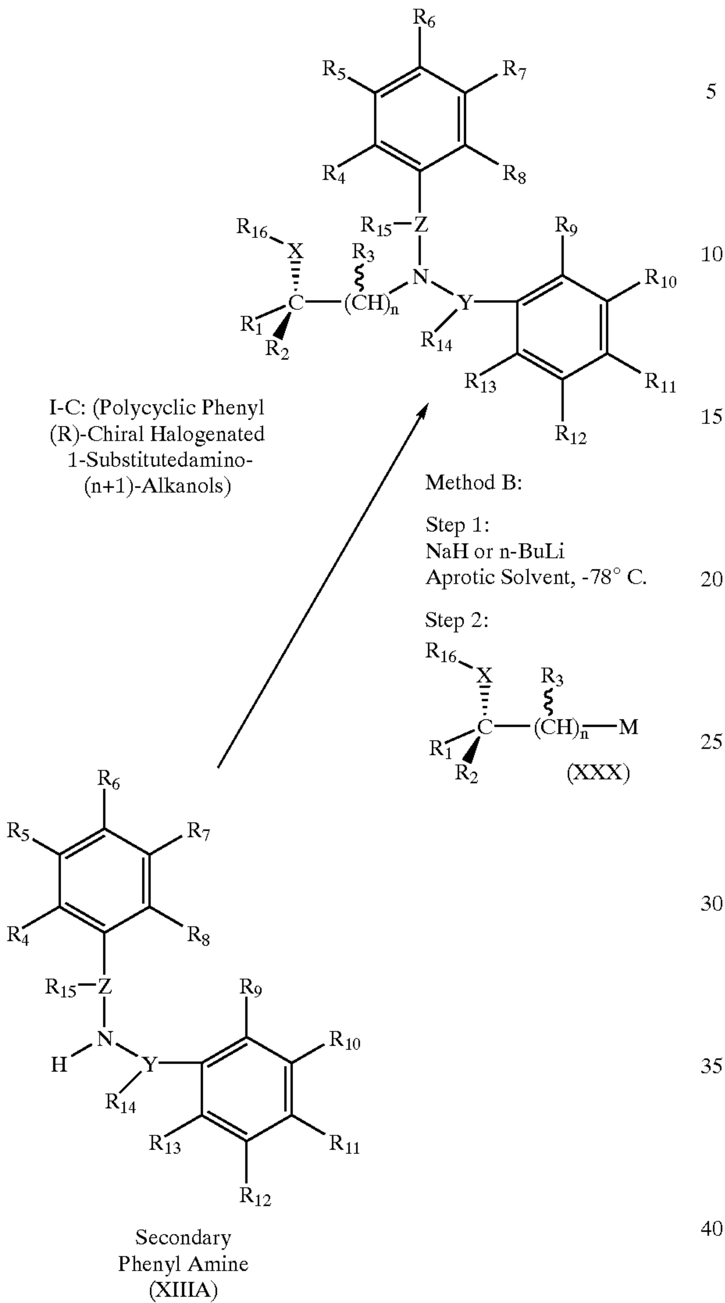
Scheme 5
