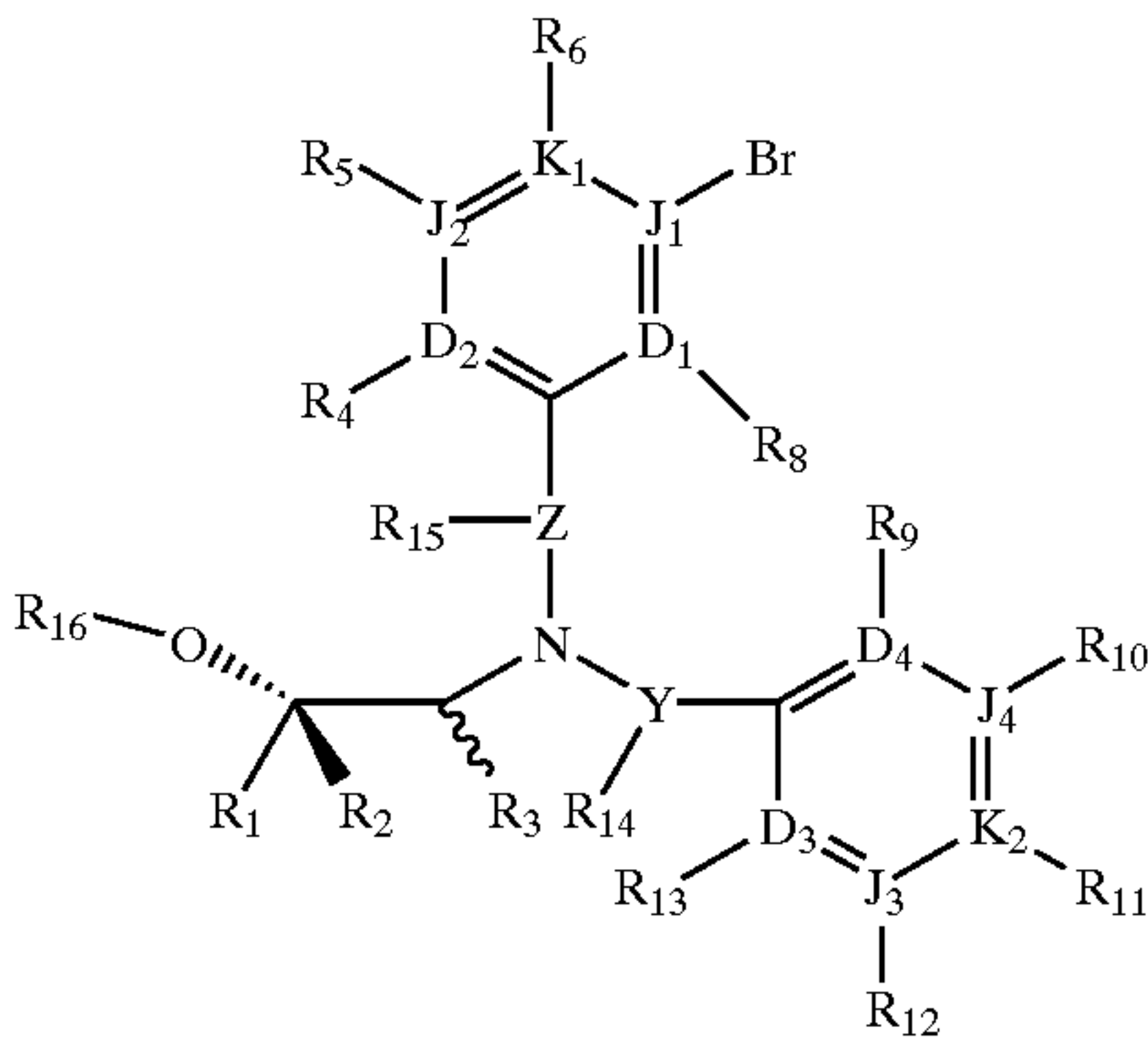
I-HP/I-HPC: (Generic Polycyclic 3-Bromo Aryl and Heteroaryl/Aryl-Heteroaryl (R)-Chiral Halogenated 1-Substitutedamino-2-Propanols)
