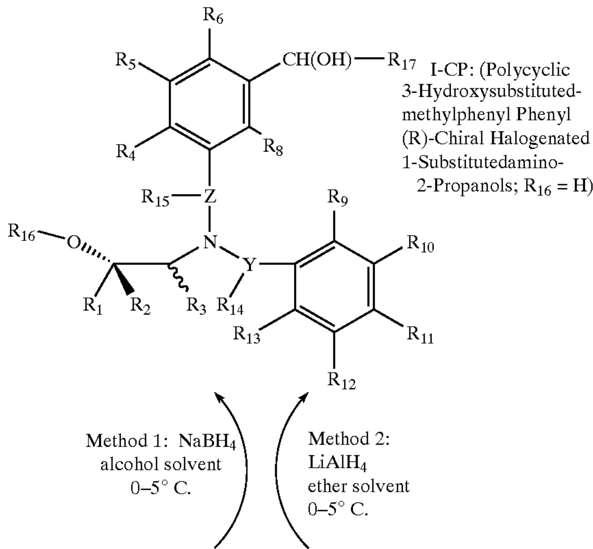
Scheme 29
