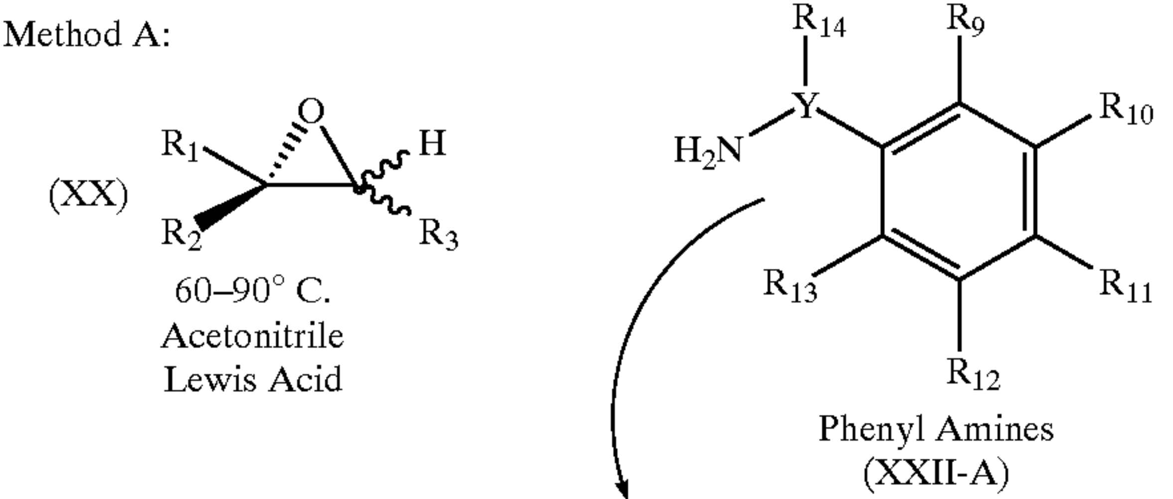
Scheme 57
