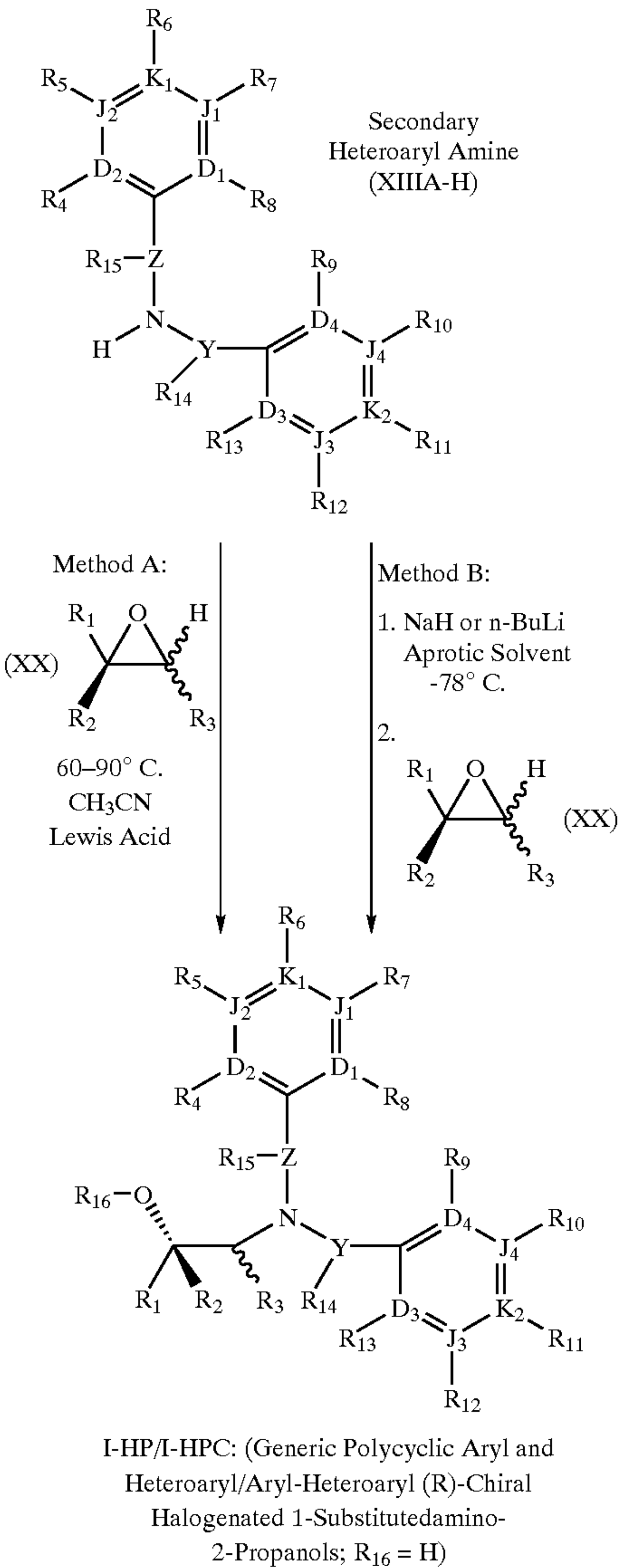
Scheme 7
