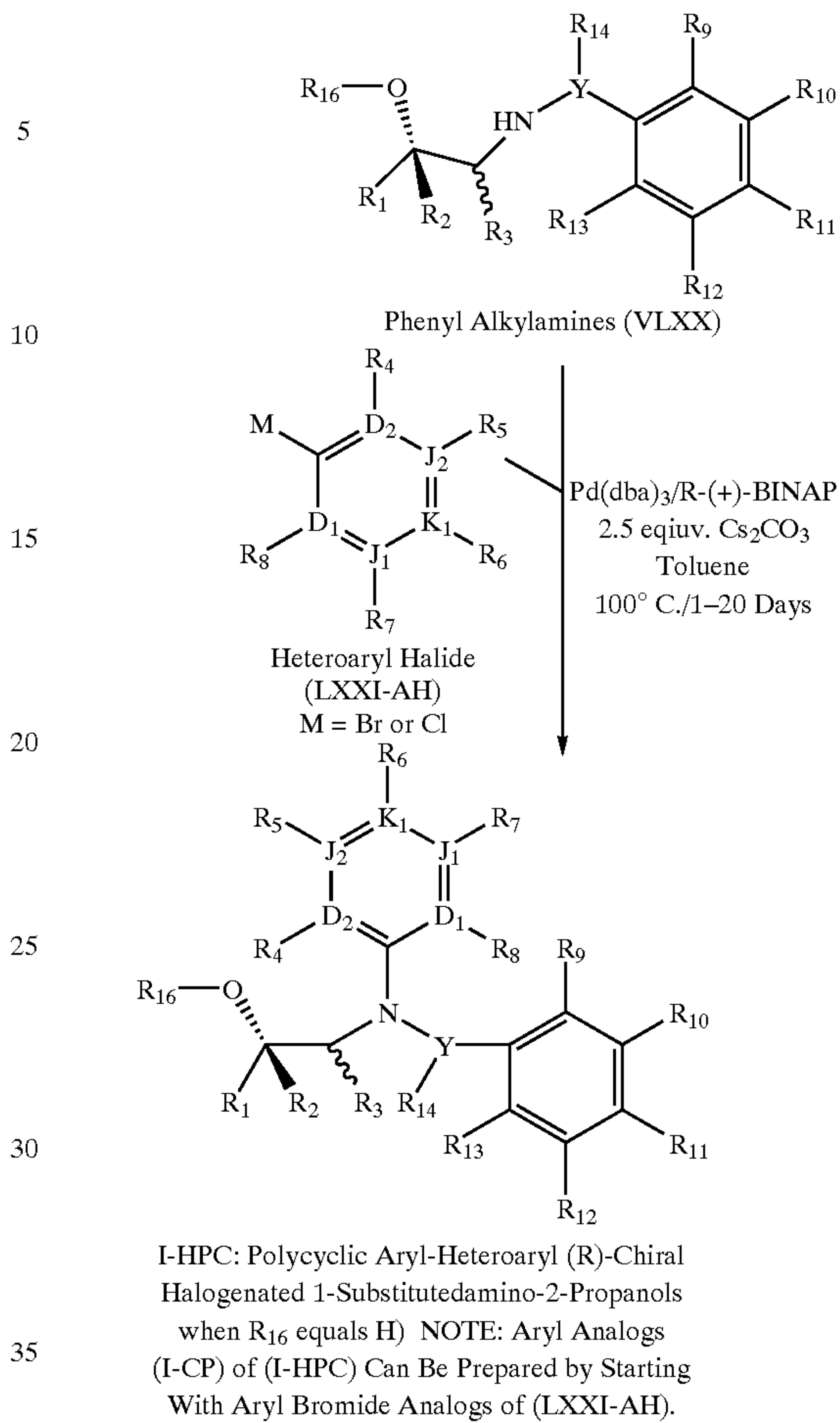
Scheme 58
