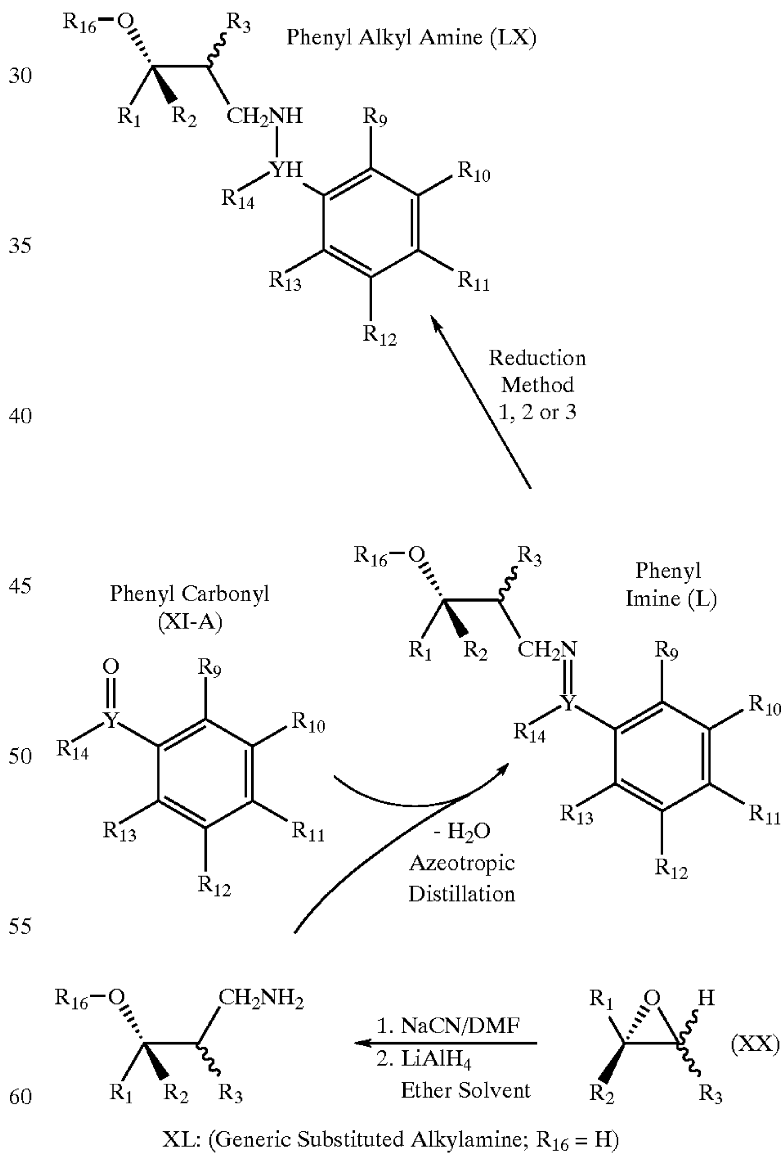
Scheme 33
