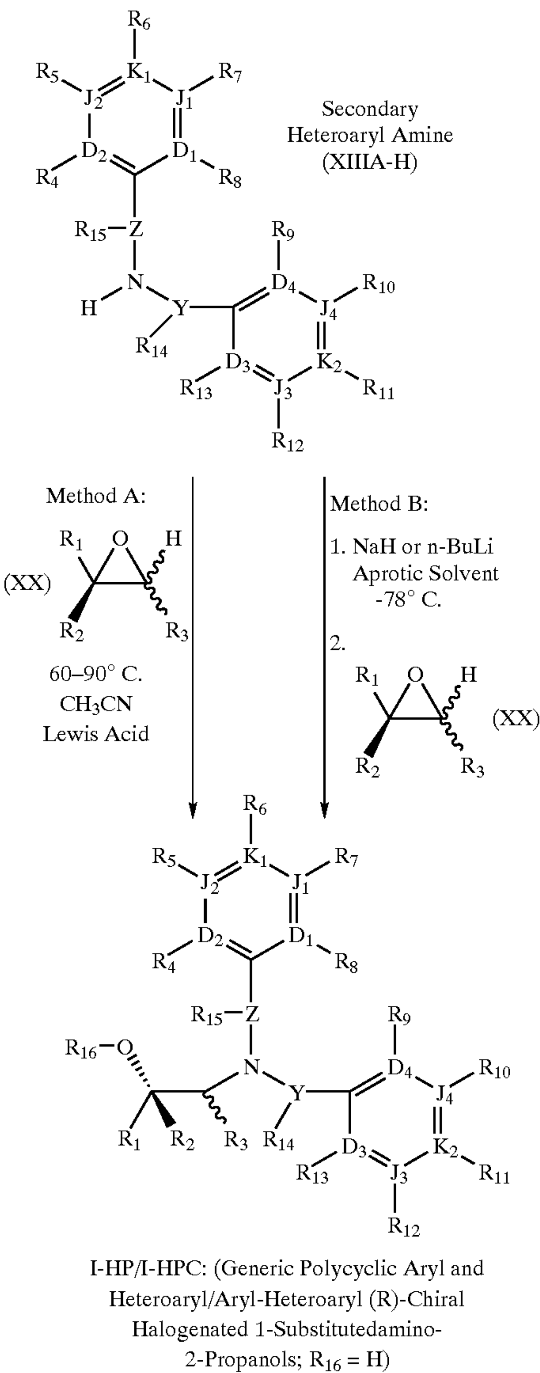
Scheme 7
