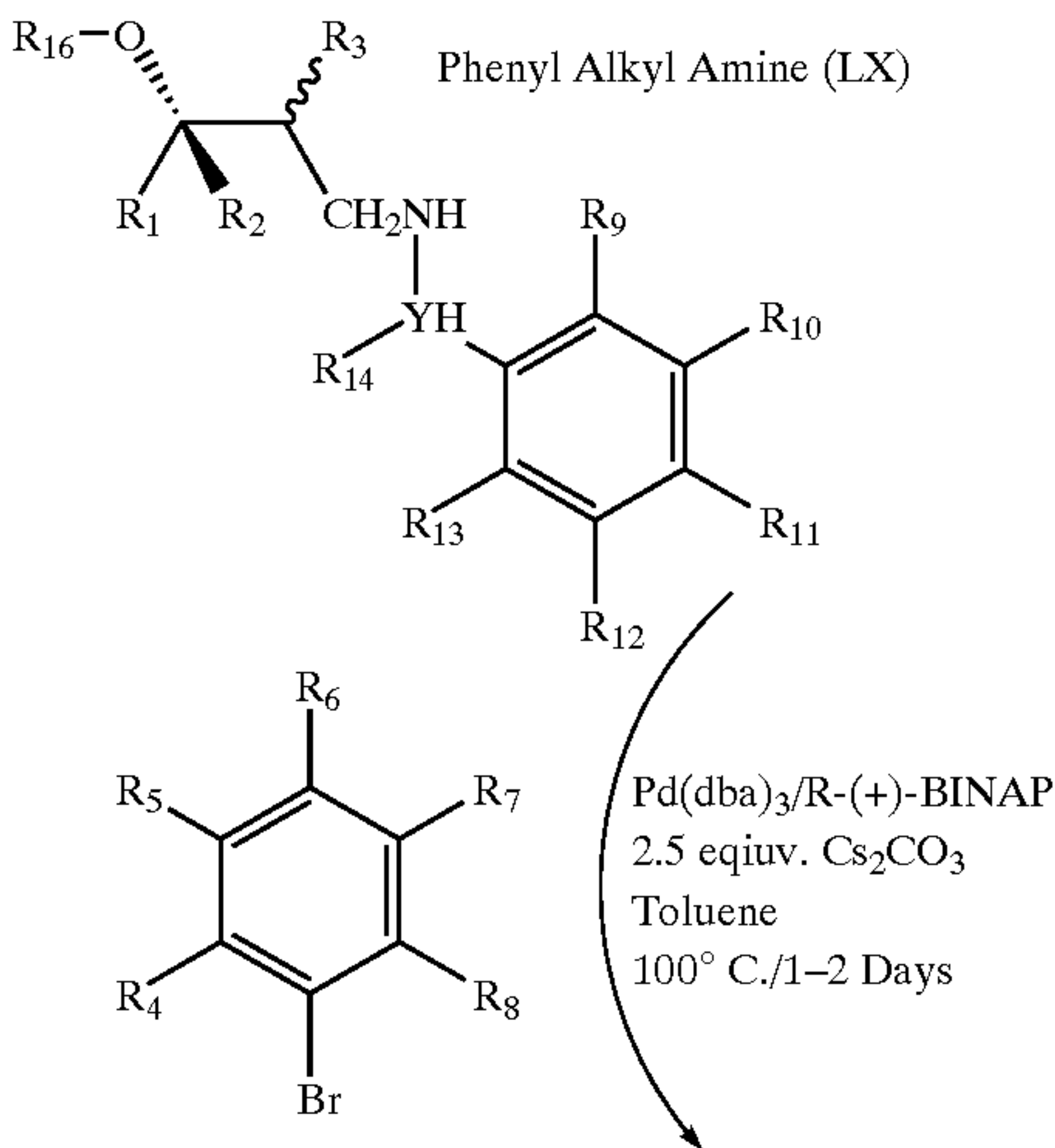
Scheme 35
