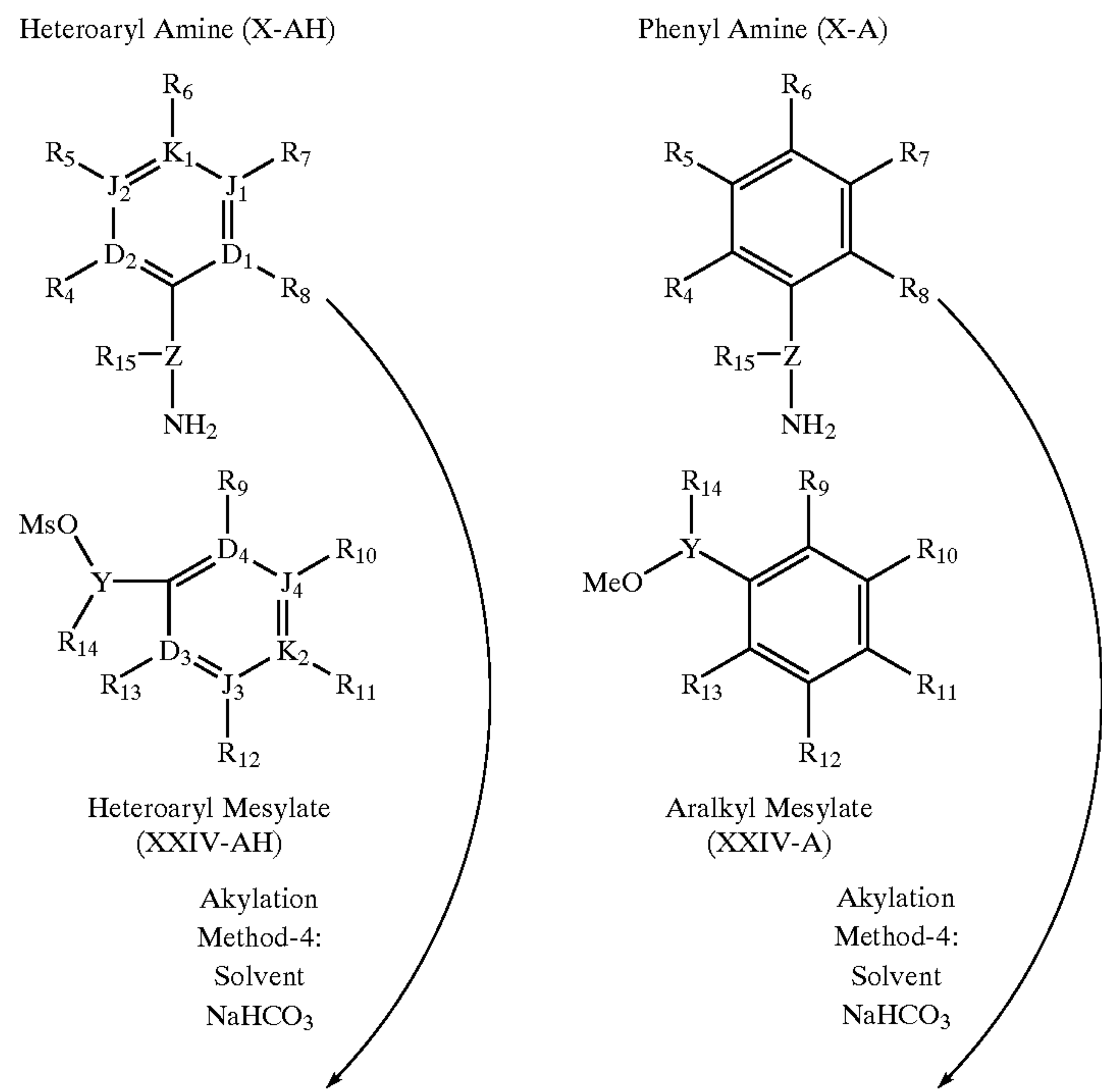
Scheme 4
