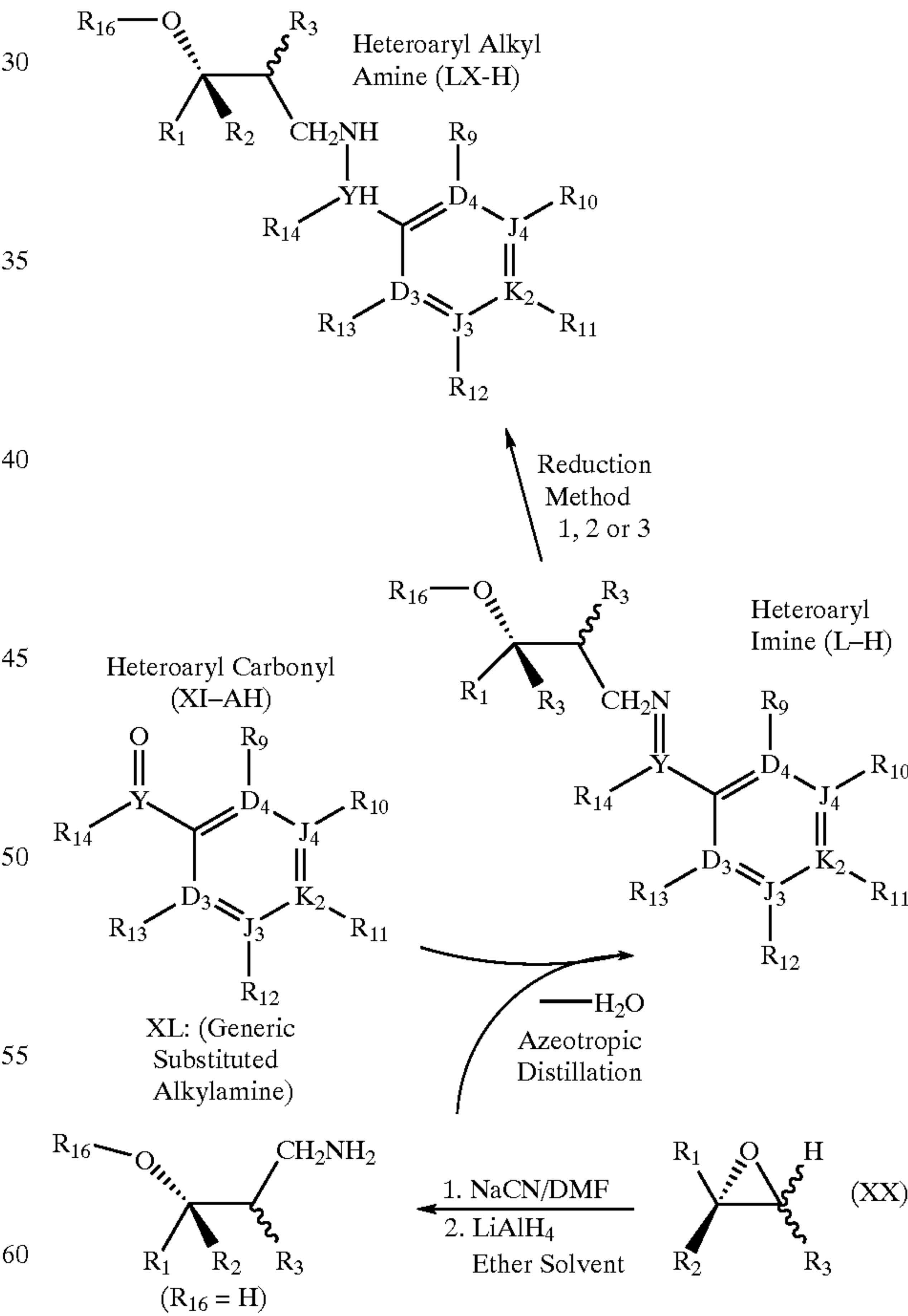
Scheme 30
