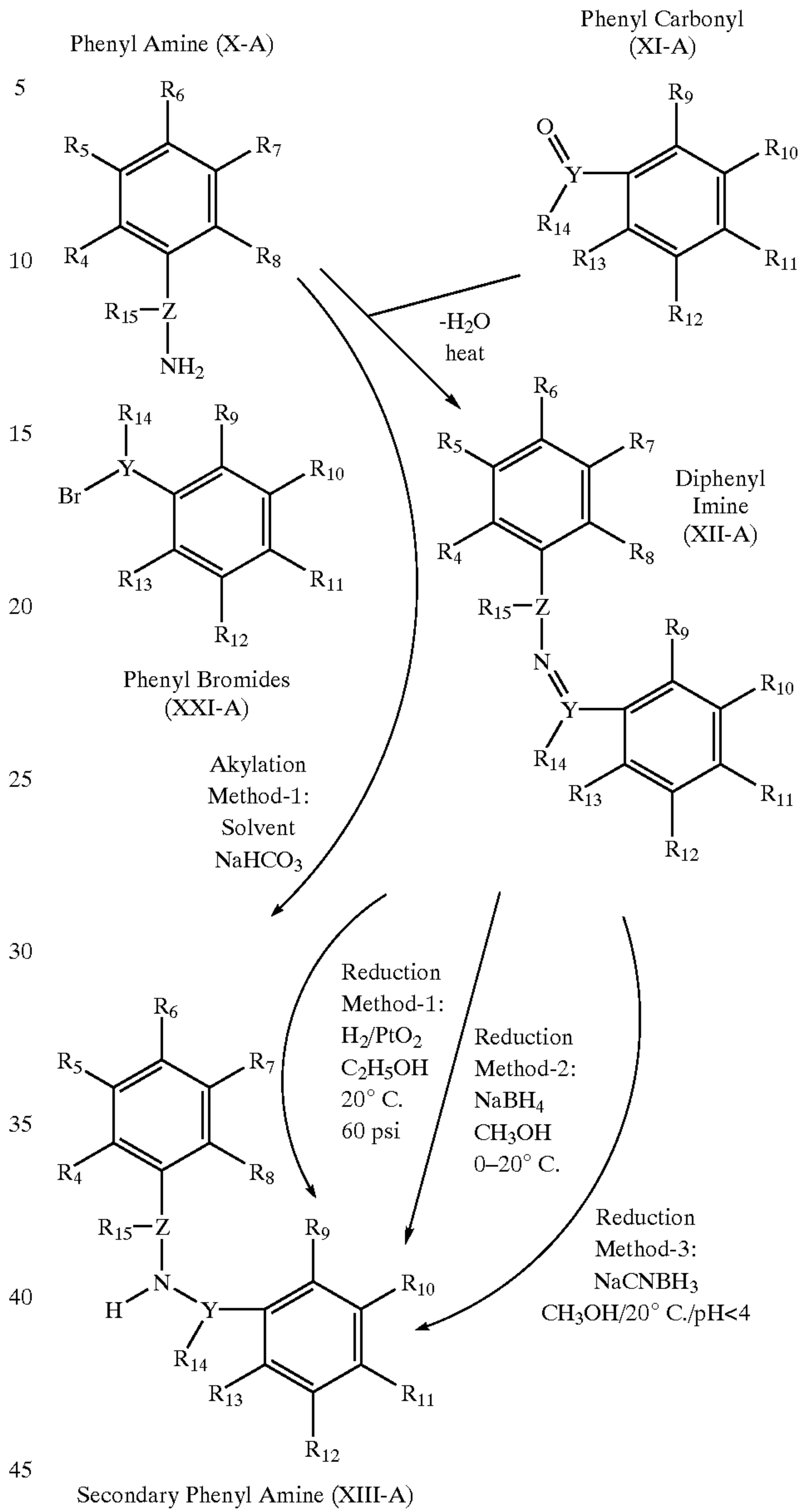
Scheme 9
