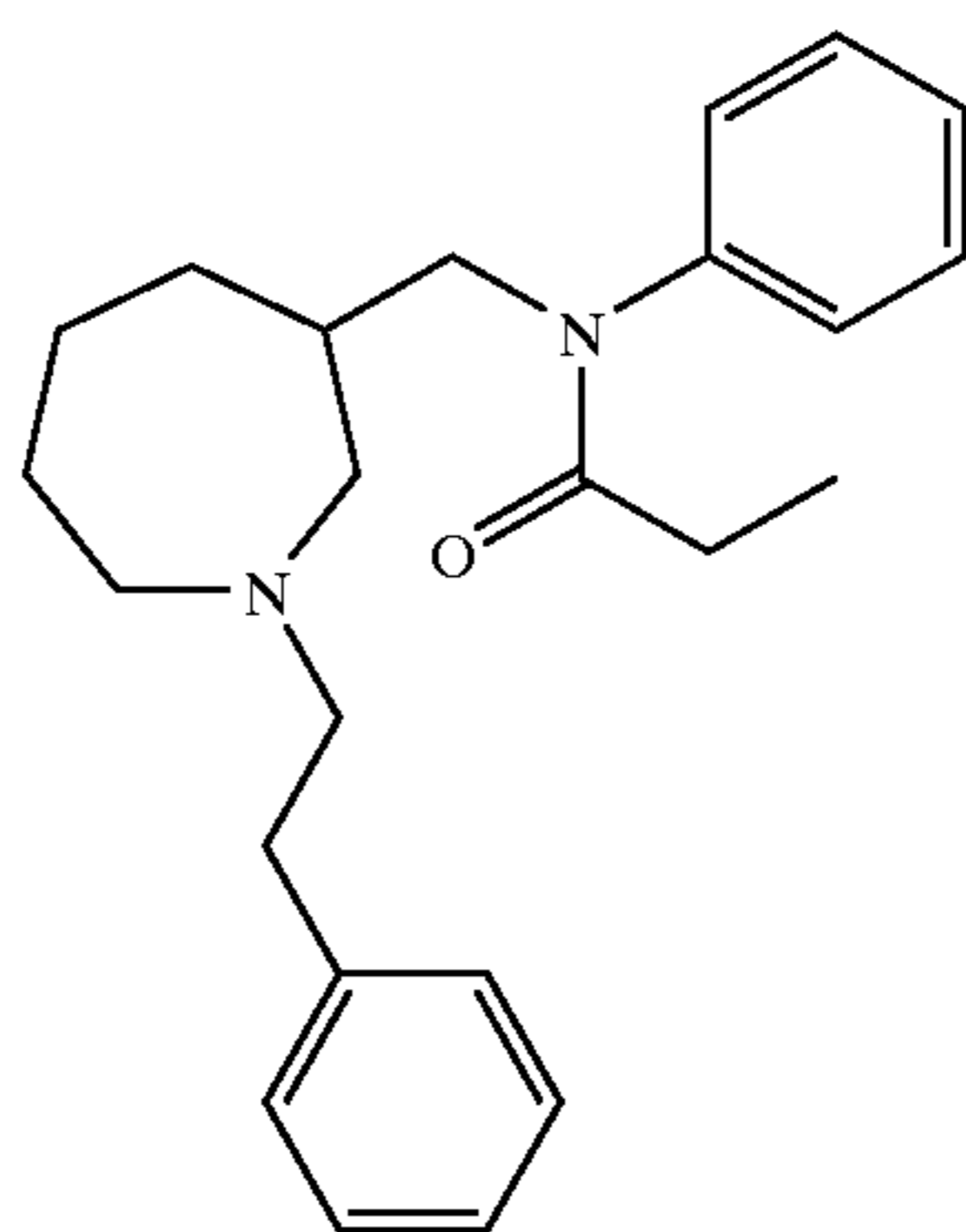
N-(1-Phenethyl-azepan-3-ylmethyl)-N-phenyl-propionamide 150
