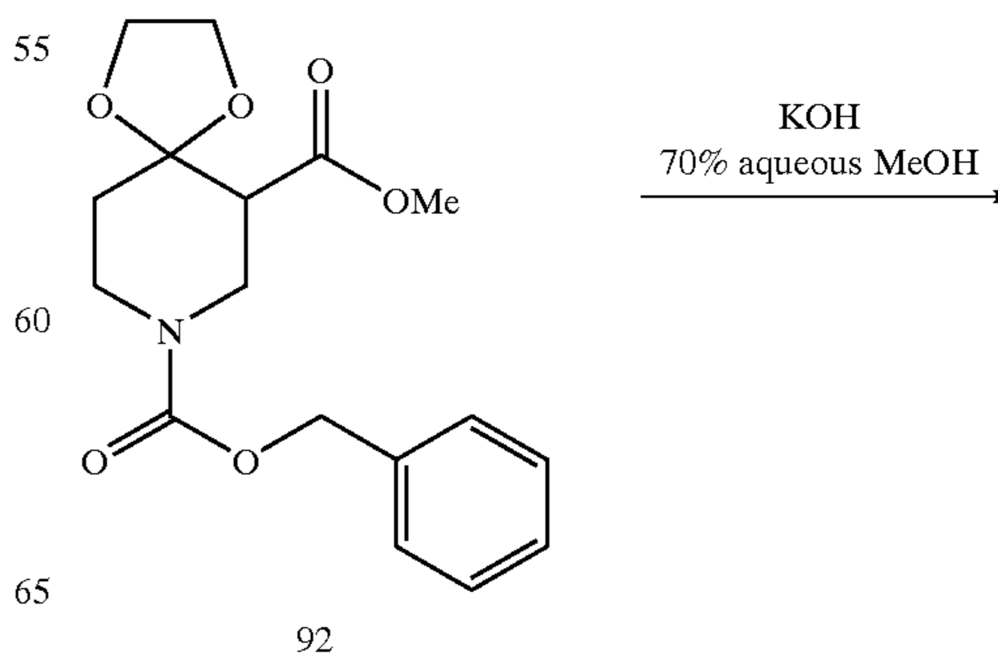
8-Benzyloxycarbonyl-1,4-dioxo-8-aza-spiro[4.5]decane-6-carboxylic Acid 93
