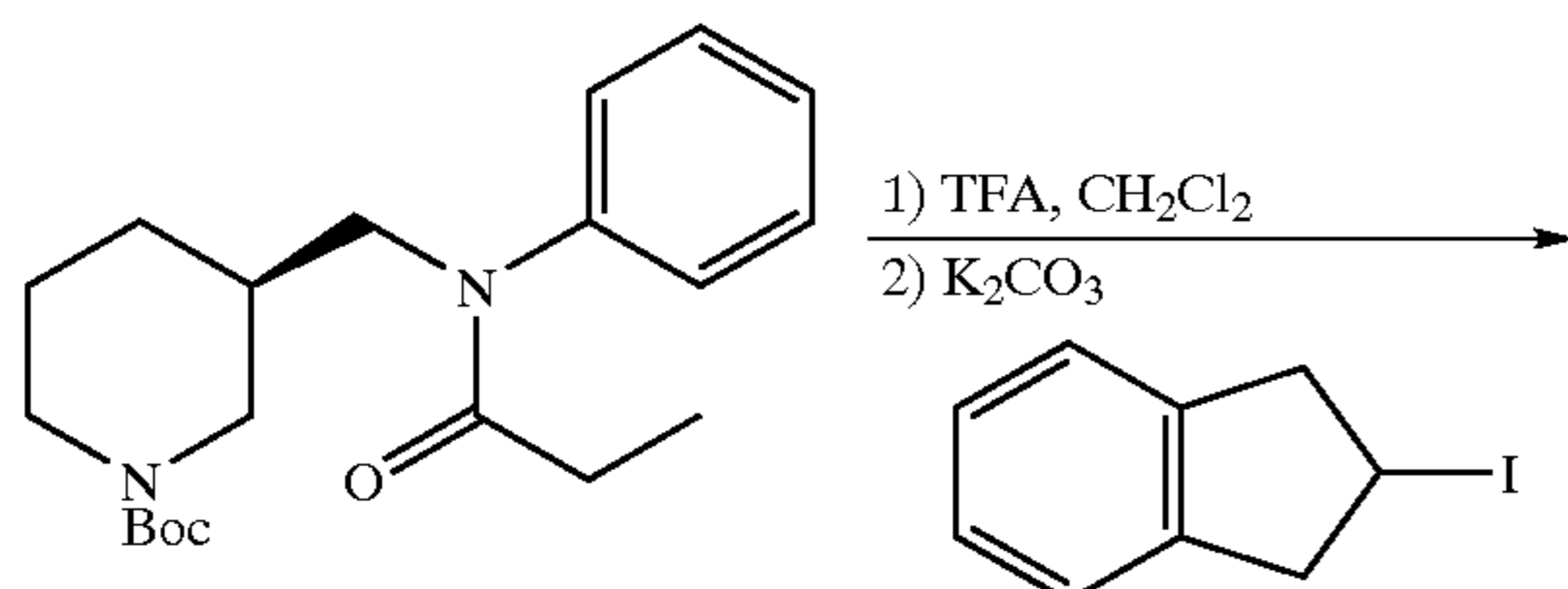
N-(1-Indan-2-yl-piperidin-3-ylmethyl)-N-phenylpropionamide (199)
