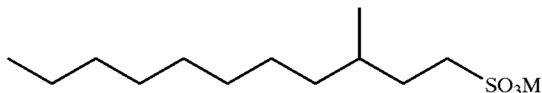
3-Methyltridecyl sulfate:
