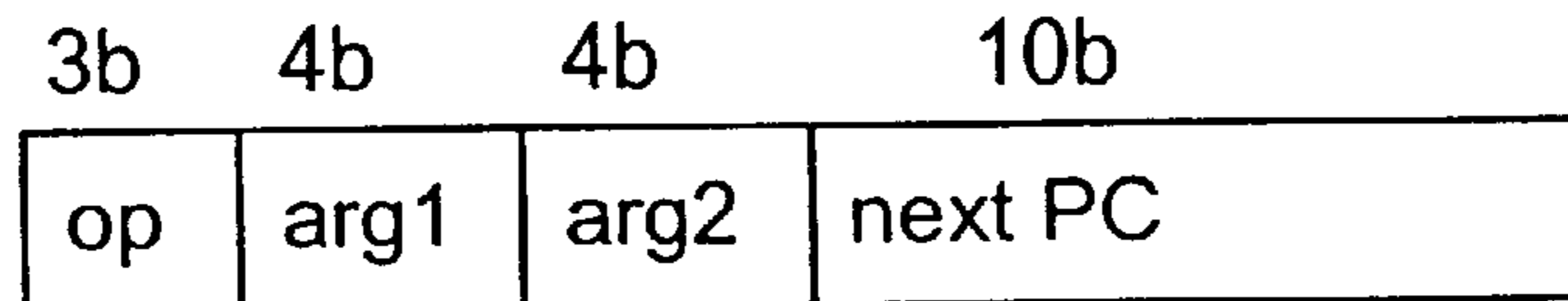
Microcode Instruction Format
