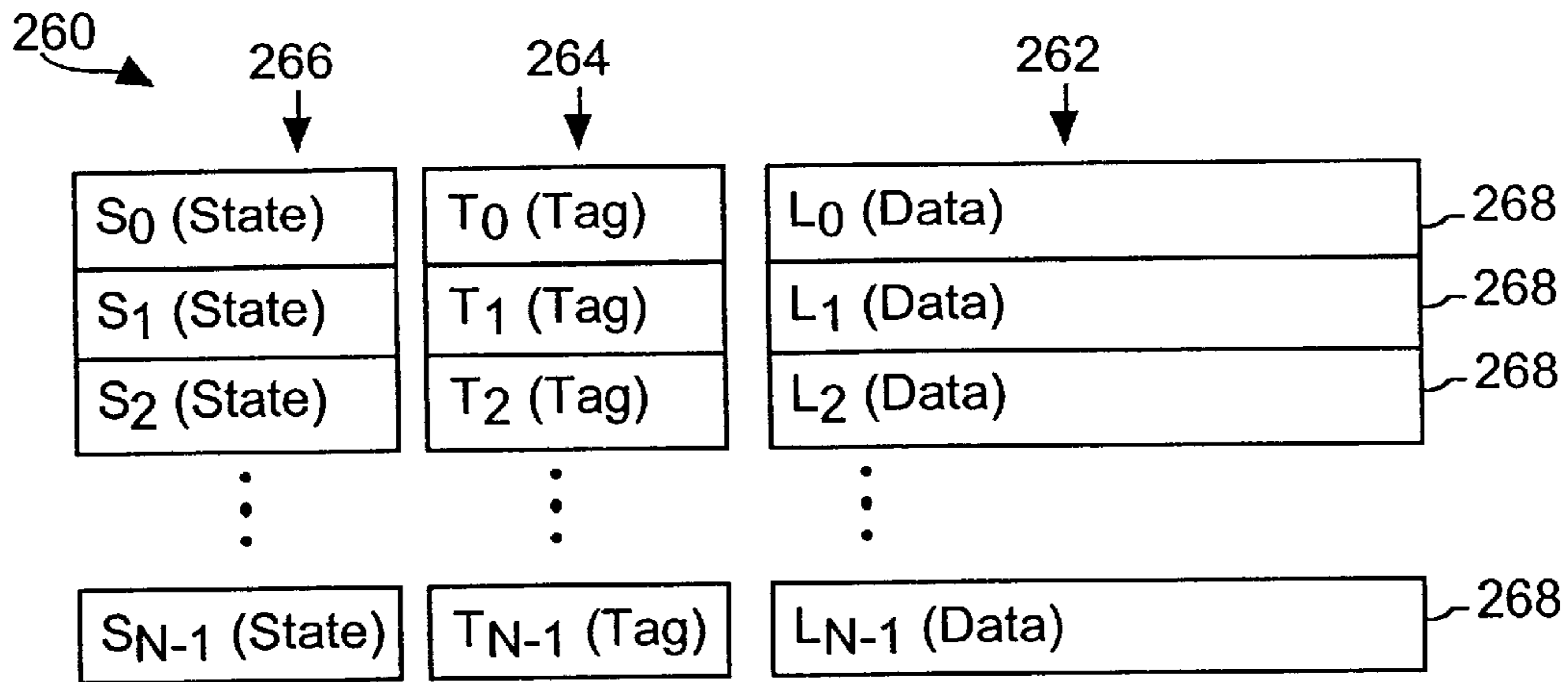
L1 Cache (Direct Mapped)
