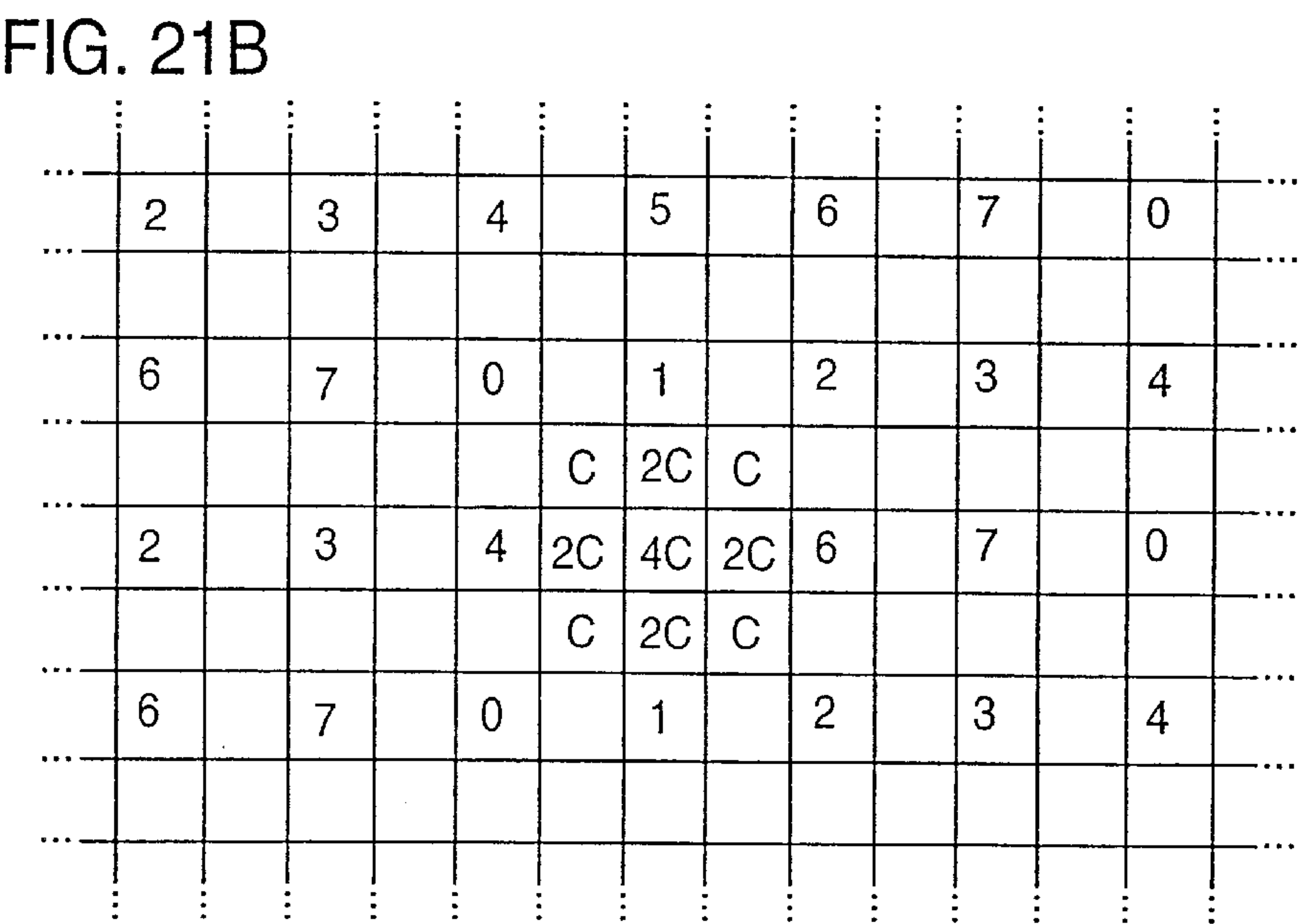
EXAMPLE OF HOW MANY ELEMENTARY BUMPS, 900, WOULD BE ASSIGNED LOCATIONS IN AN IMAGE, AND THOSE LOCATIONS WOULD BE ASSOCIATED WITH A CORRESPONDING BIT PLANE IN THE N-BIT WORD, HERE TAKEN AS N=8 WITH INDEXES OF 0-7. ONE LOCATION, ASSOCIATED WITH BIT PLANE "5", HAS THE OVERLAY OF THE BUMP PROFILE DEPICTED.
