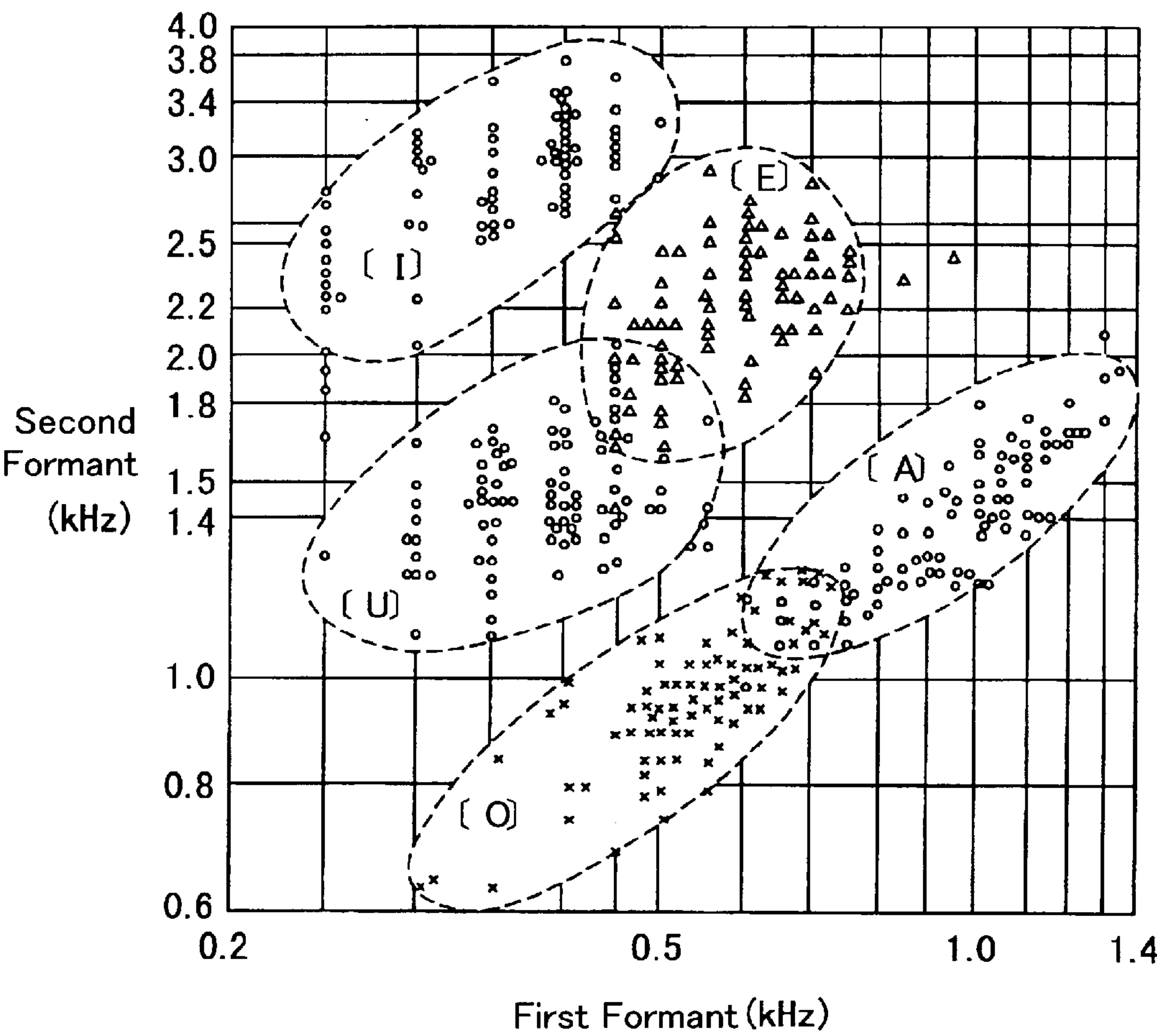
Formants of Japanese Vowels
