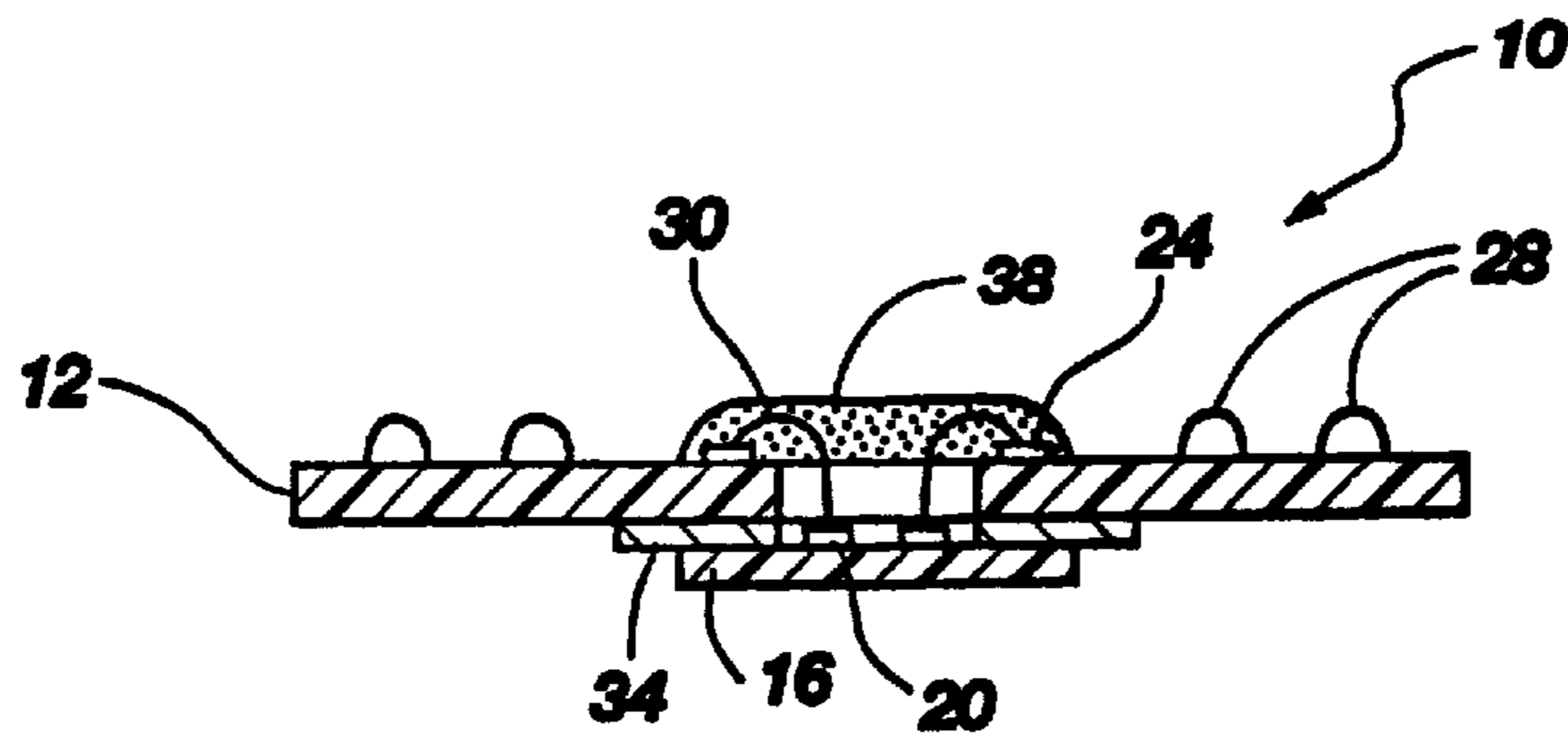
Fig. 3 (PRIOR ART)
