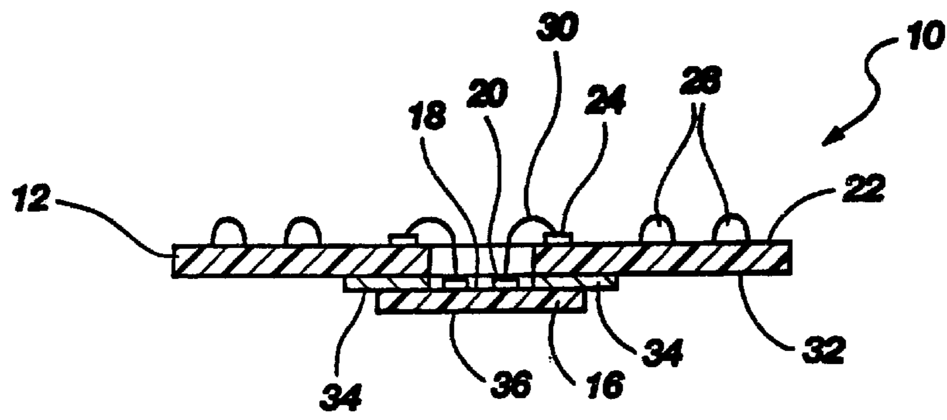
Fig. 2 (PRIOR ART)
