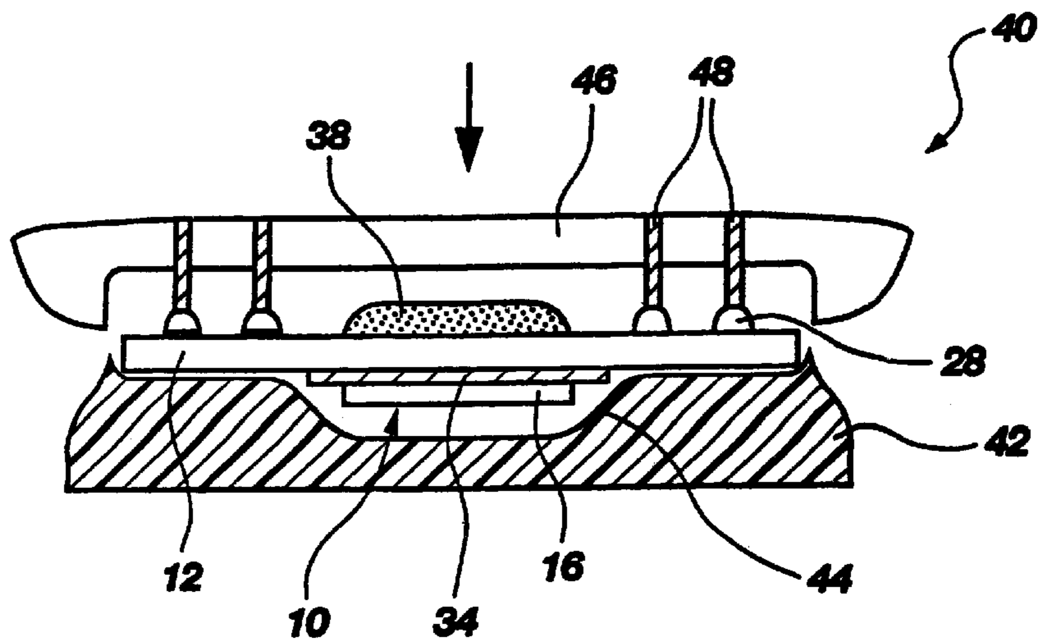
Fig. 4 (PRIOR ART)
