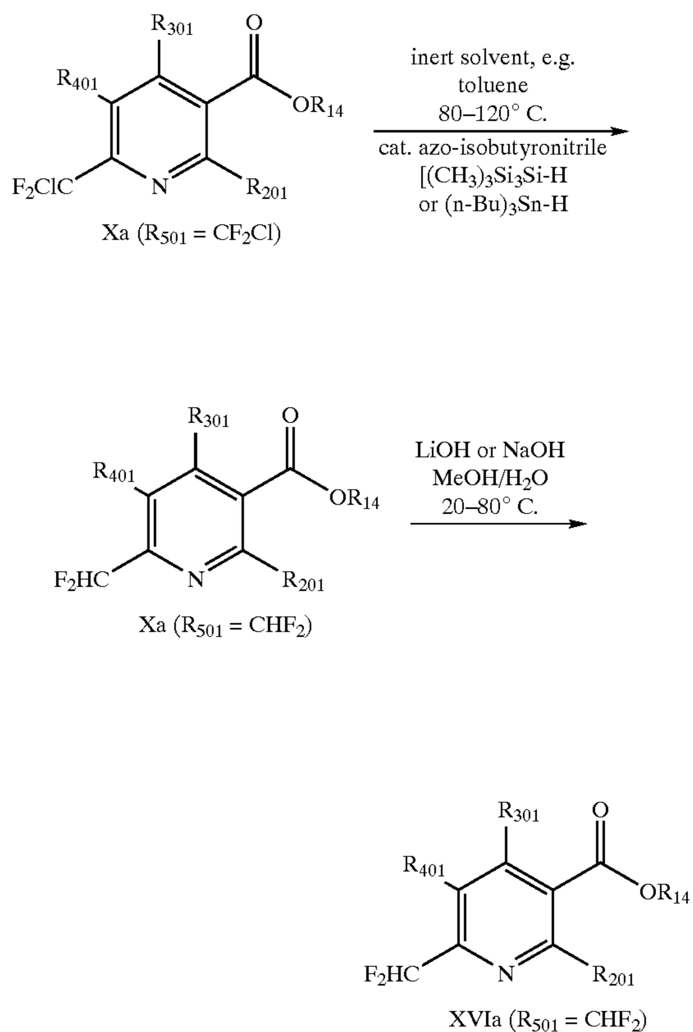
Reaction Scheme 6
