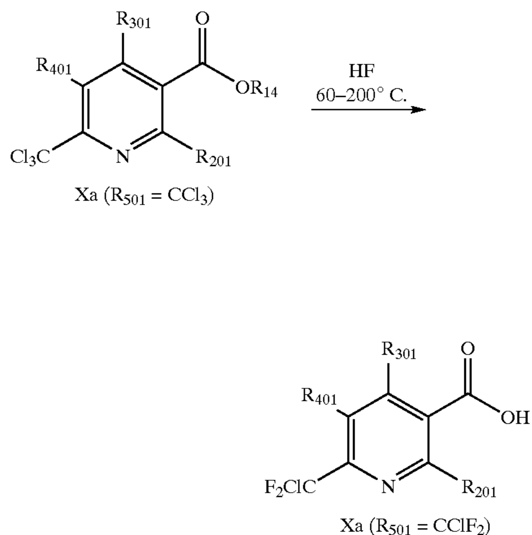
Reaction Scheme 5
