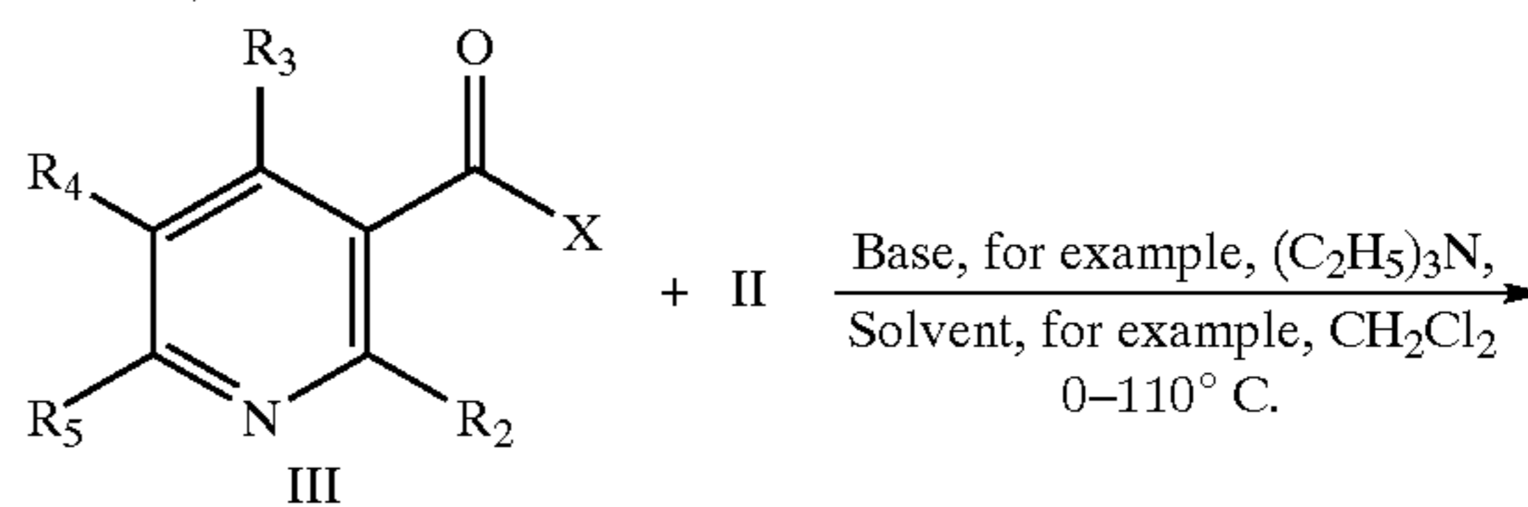
Reaction scheme 1
