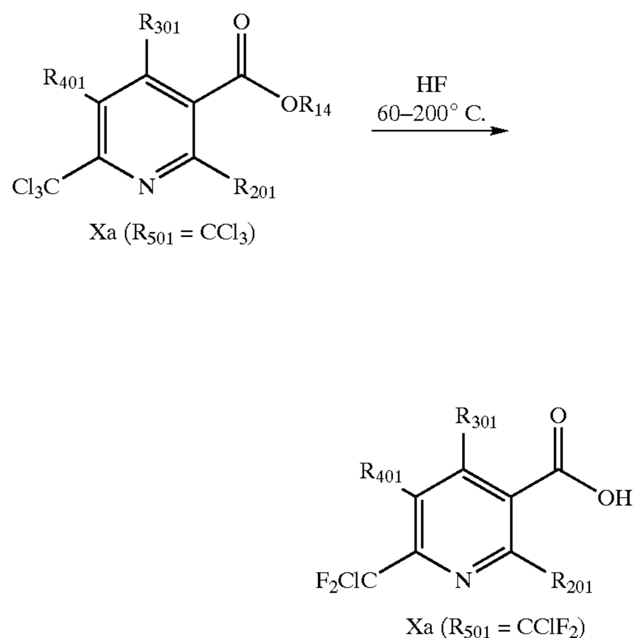
Reaction Scheme 5
