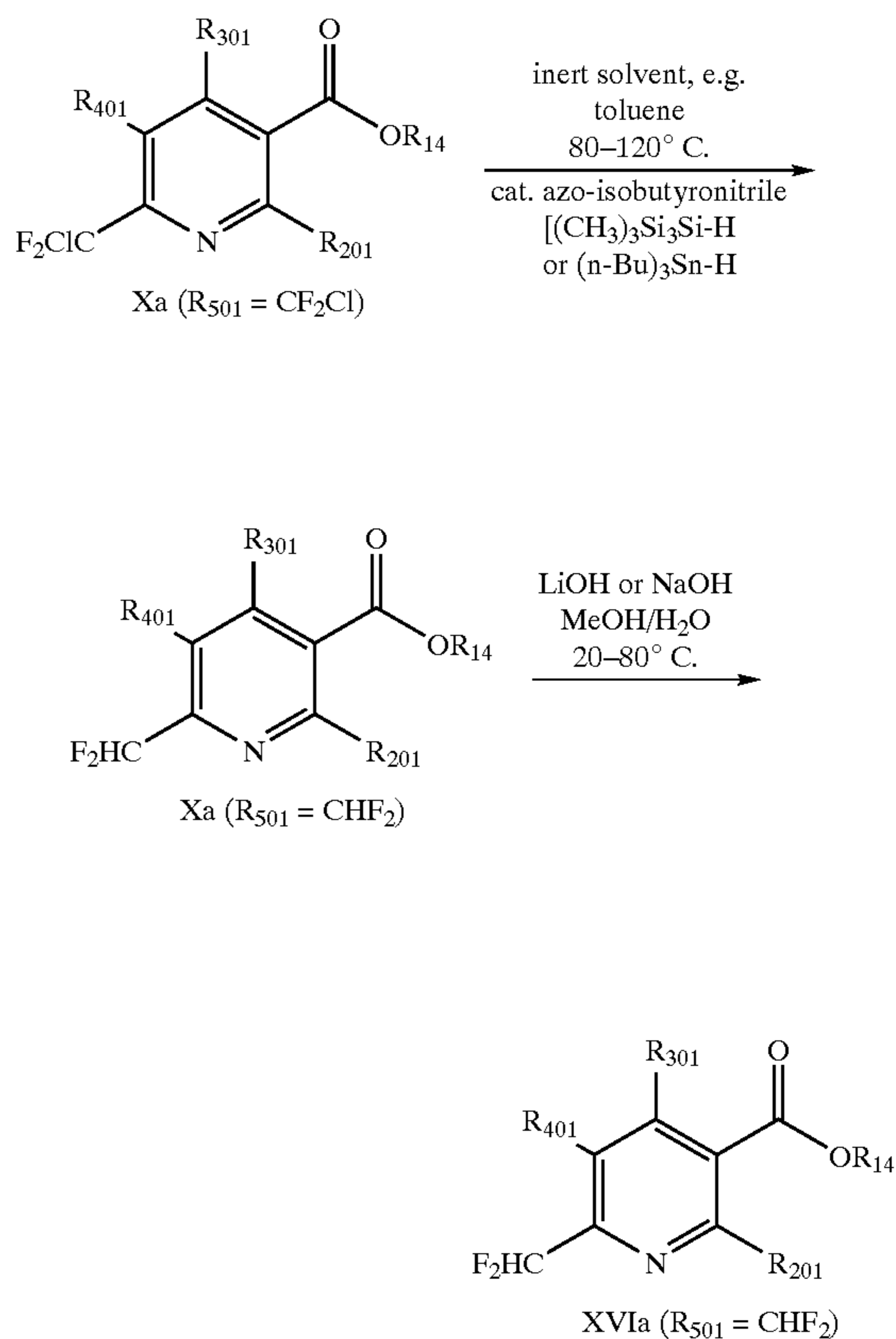
Reaction Scheme 6
