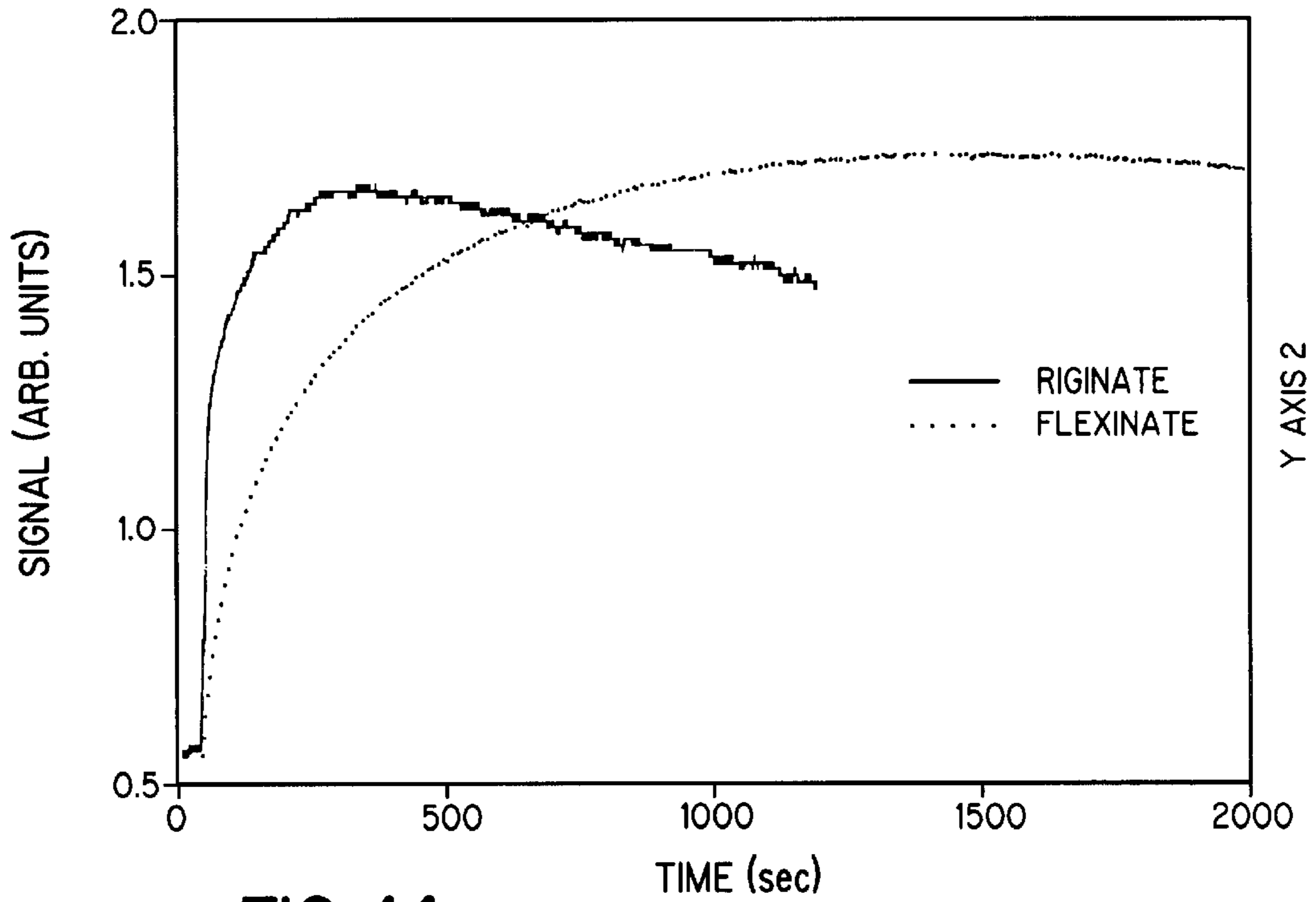
BLOOD CLEARANCE PROFILE OF CYANINETETRASULFONATES
