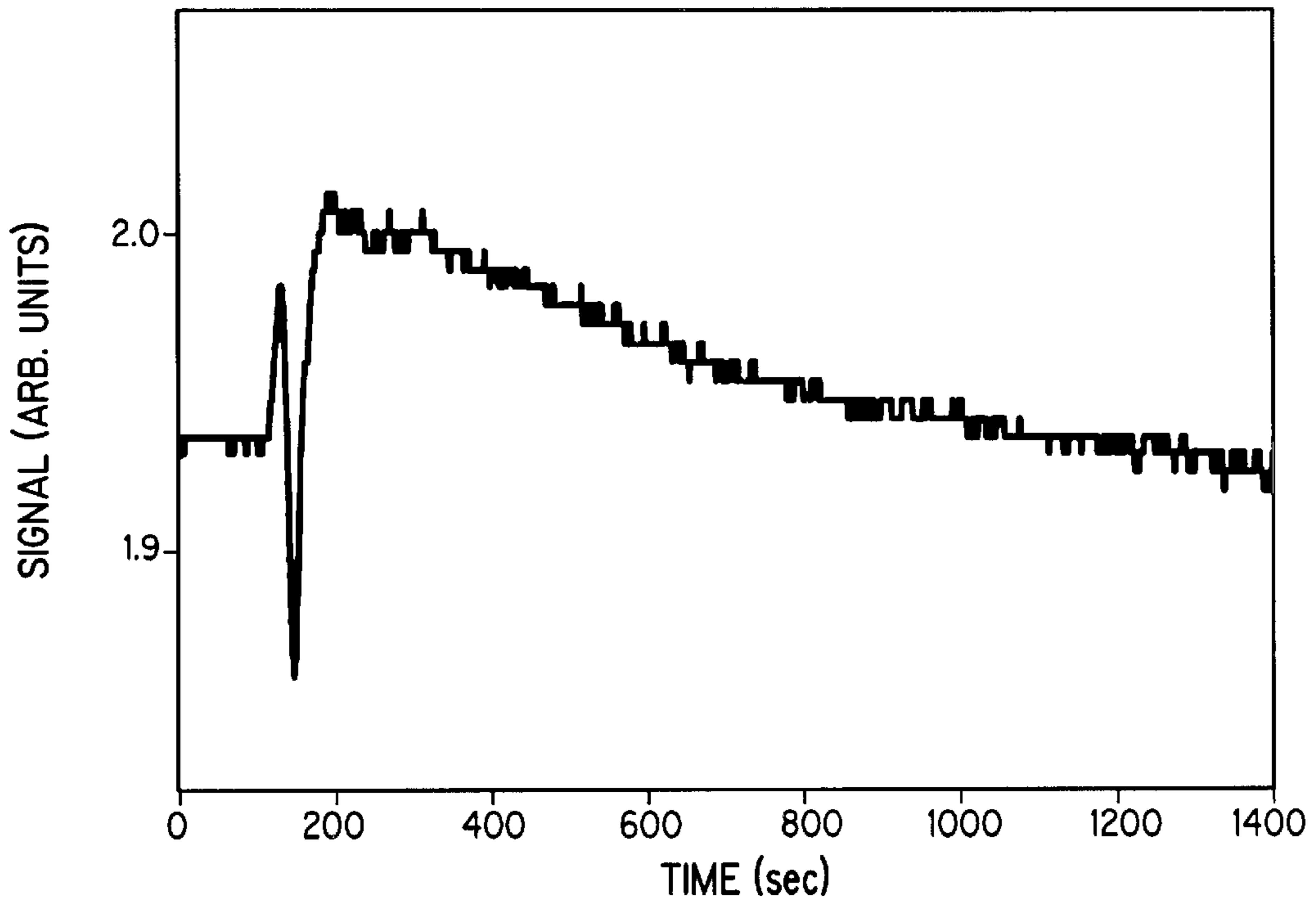
BLOOD CLEARANCE PROFILE OF INDOLE DISULFINATE
