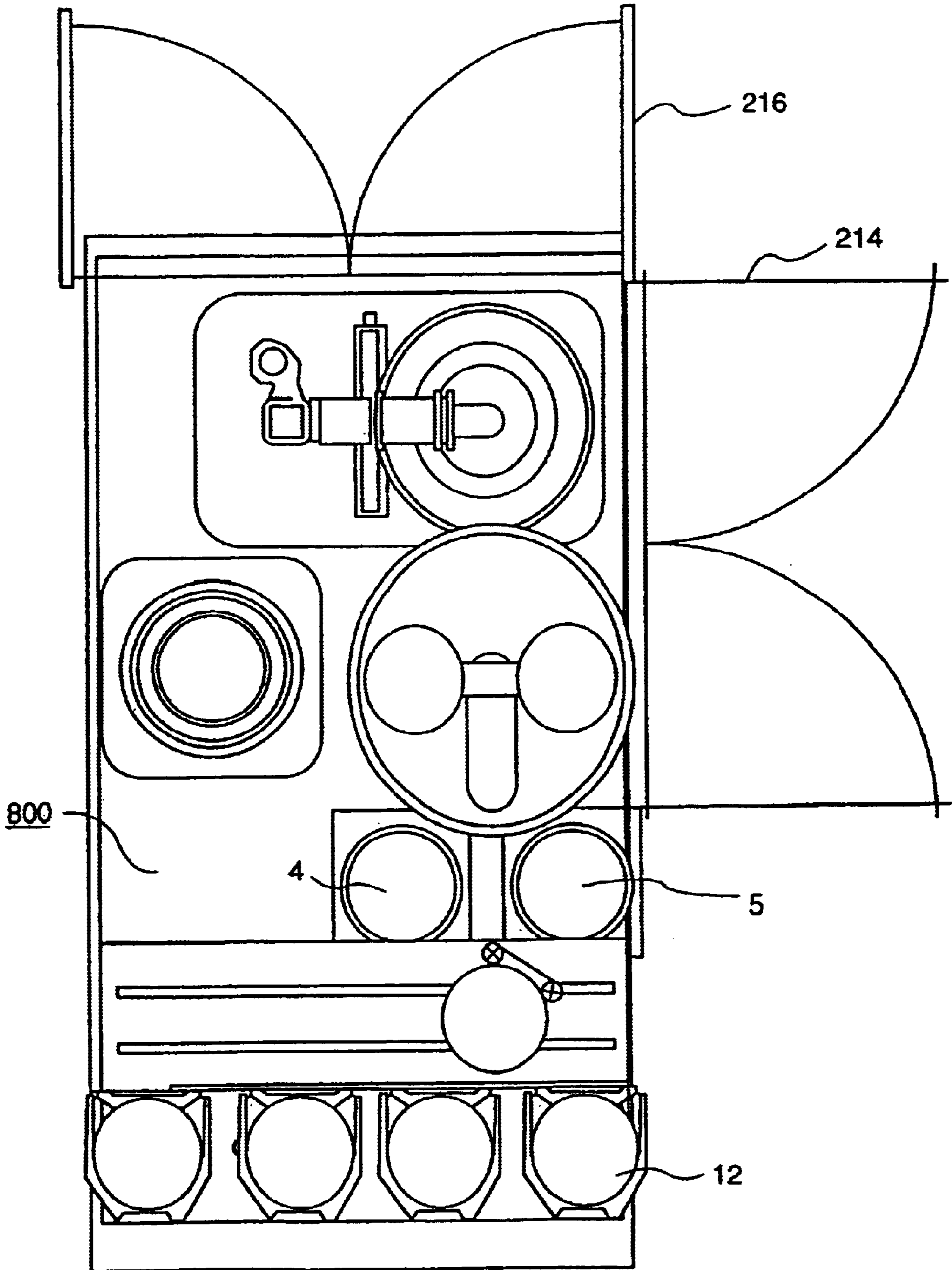
FIG. 9 PRIOR ART
