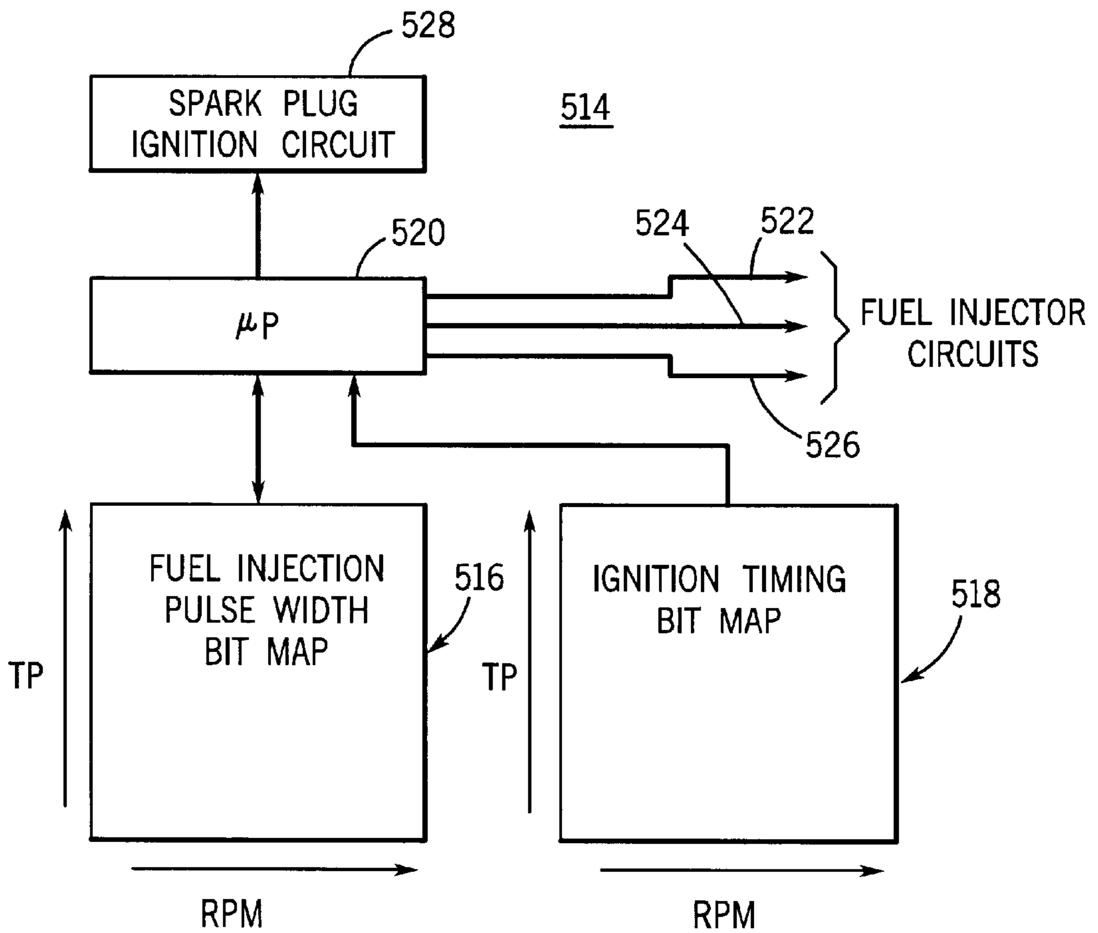
FIG. 7 (PRIOR ART)
