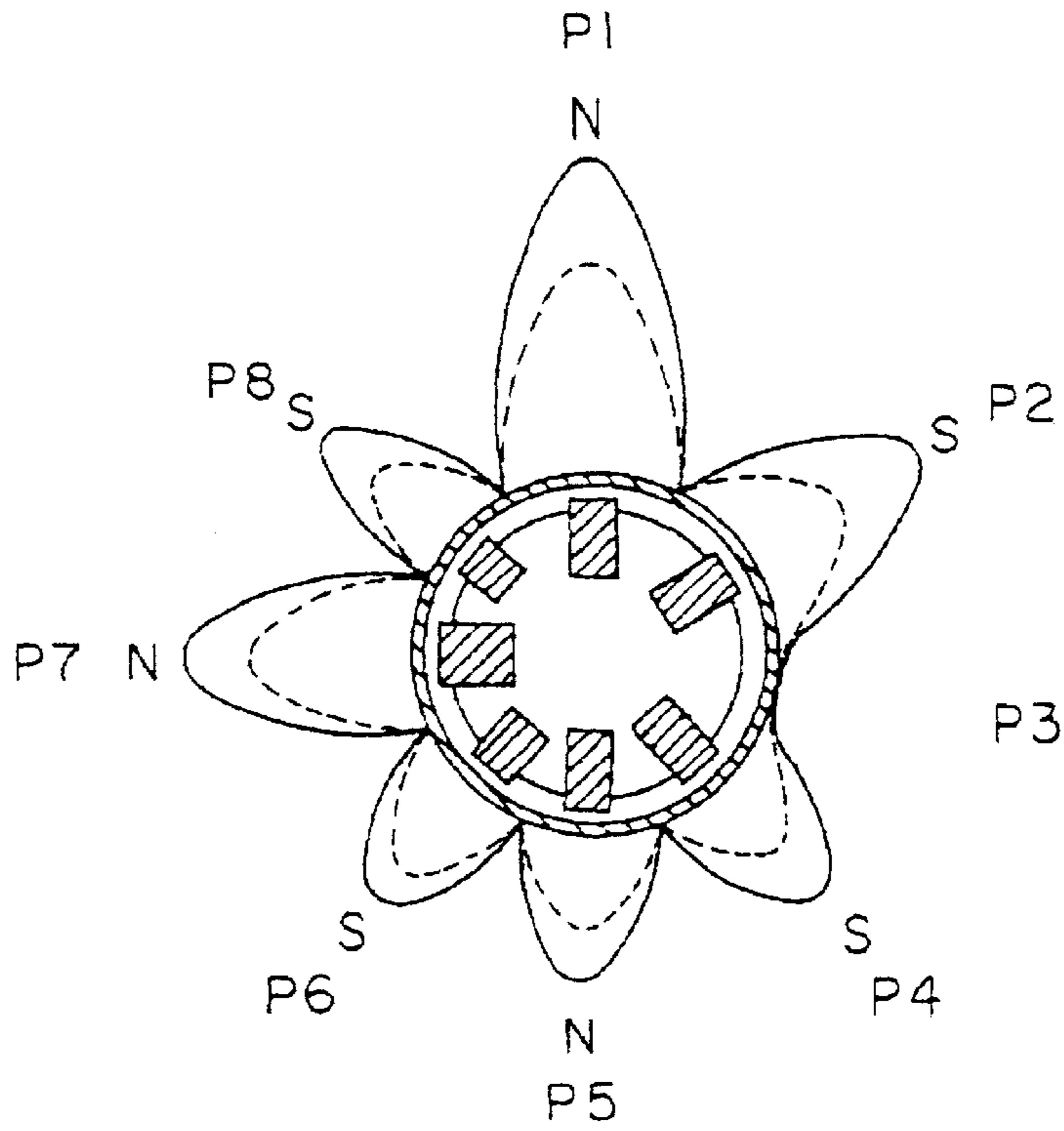
FIG. 5 PRIOR ART
