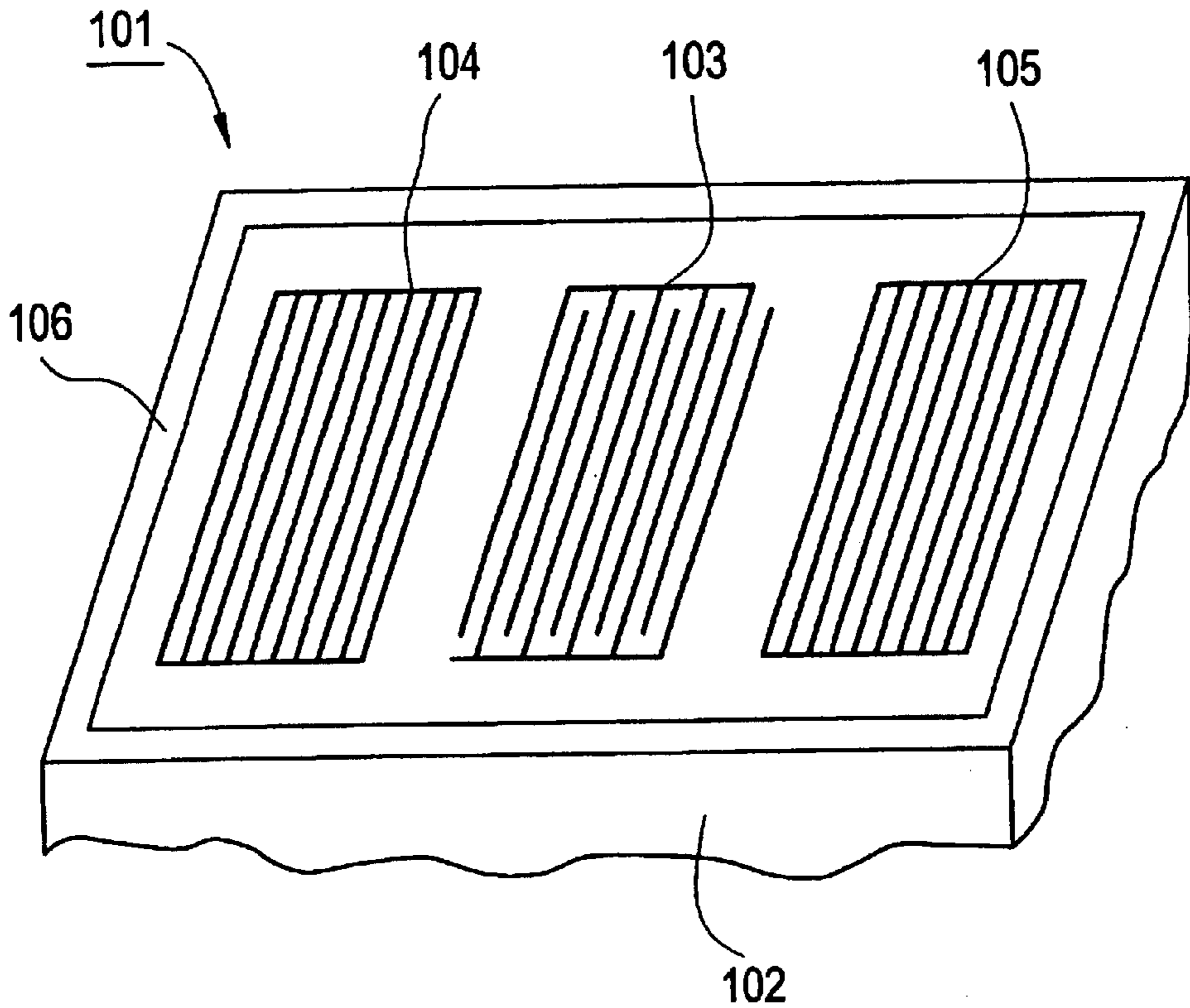
FIG. 4 PRIOR ART
