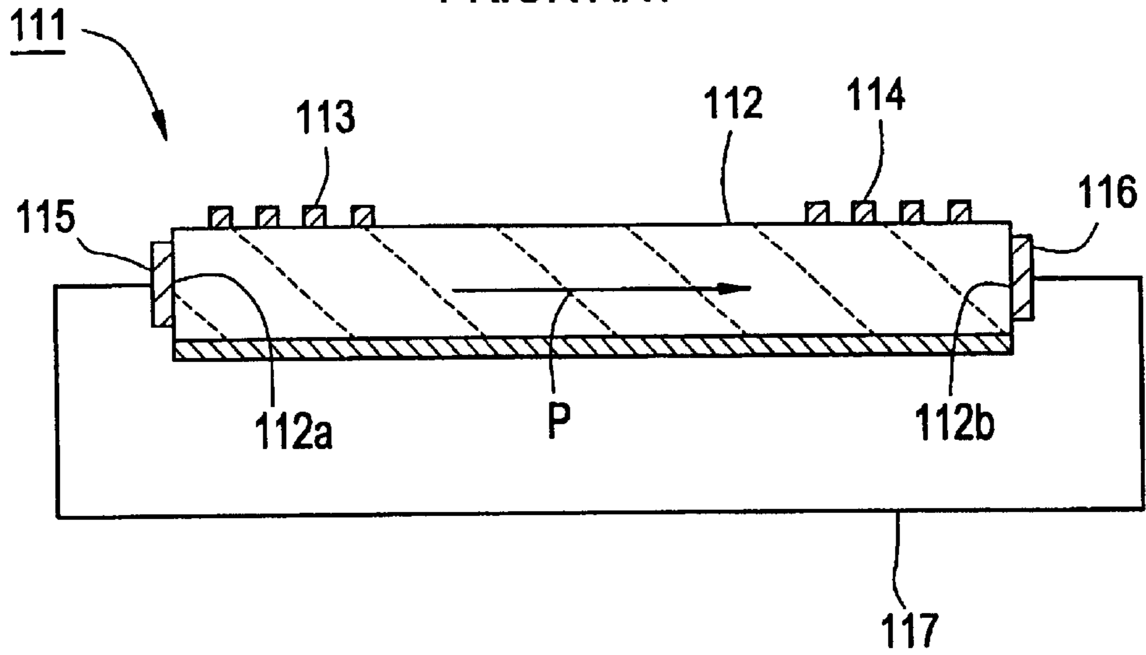
FIG. 5 PRIOR ART
