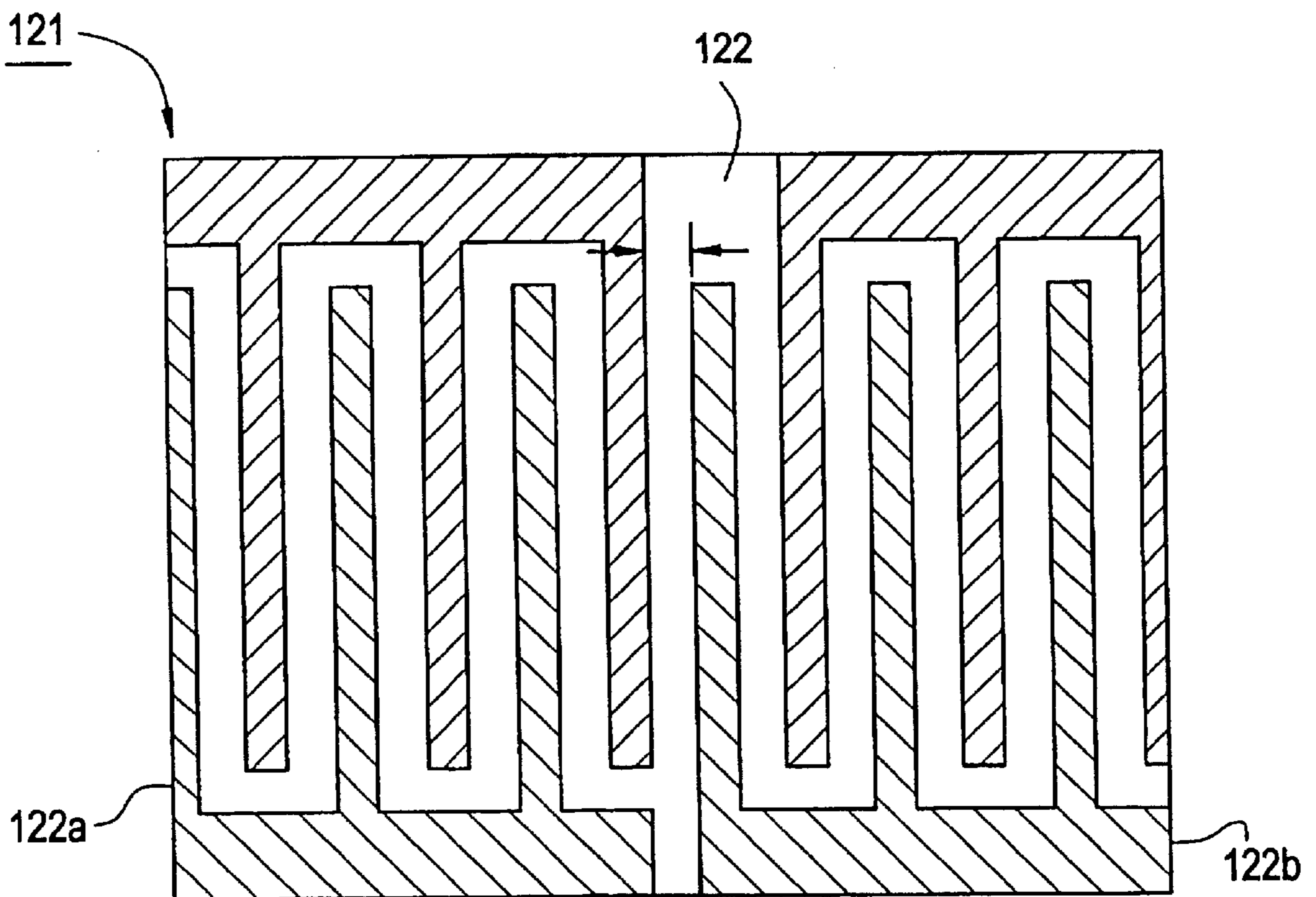
FIG. 6 PRIOR ART
