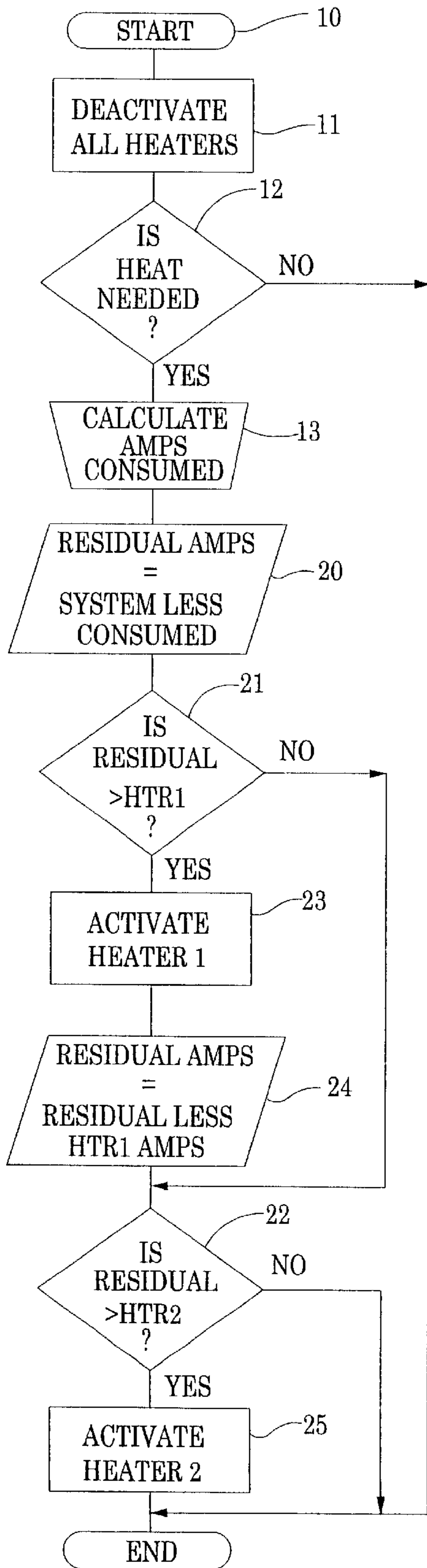
ROUTINE TO CALCULATE TOTAL CONSUMED CURRENT BASED ON ACTIVATED DEVICES IN THE SYSTEM
