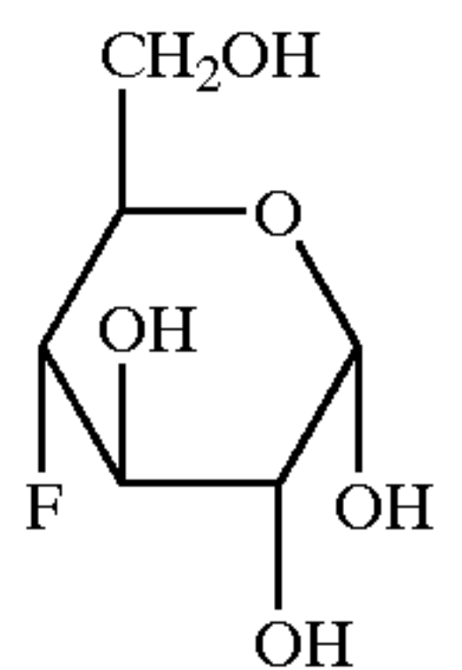
10 - 4-Fluoro-D-glucose
