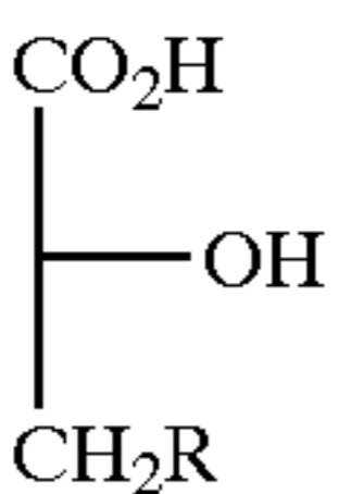
21 - R = I 22 - R = F 23 - R = SH 24 - R = CO 2 H
