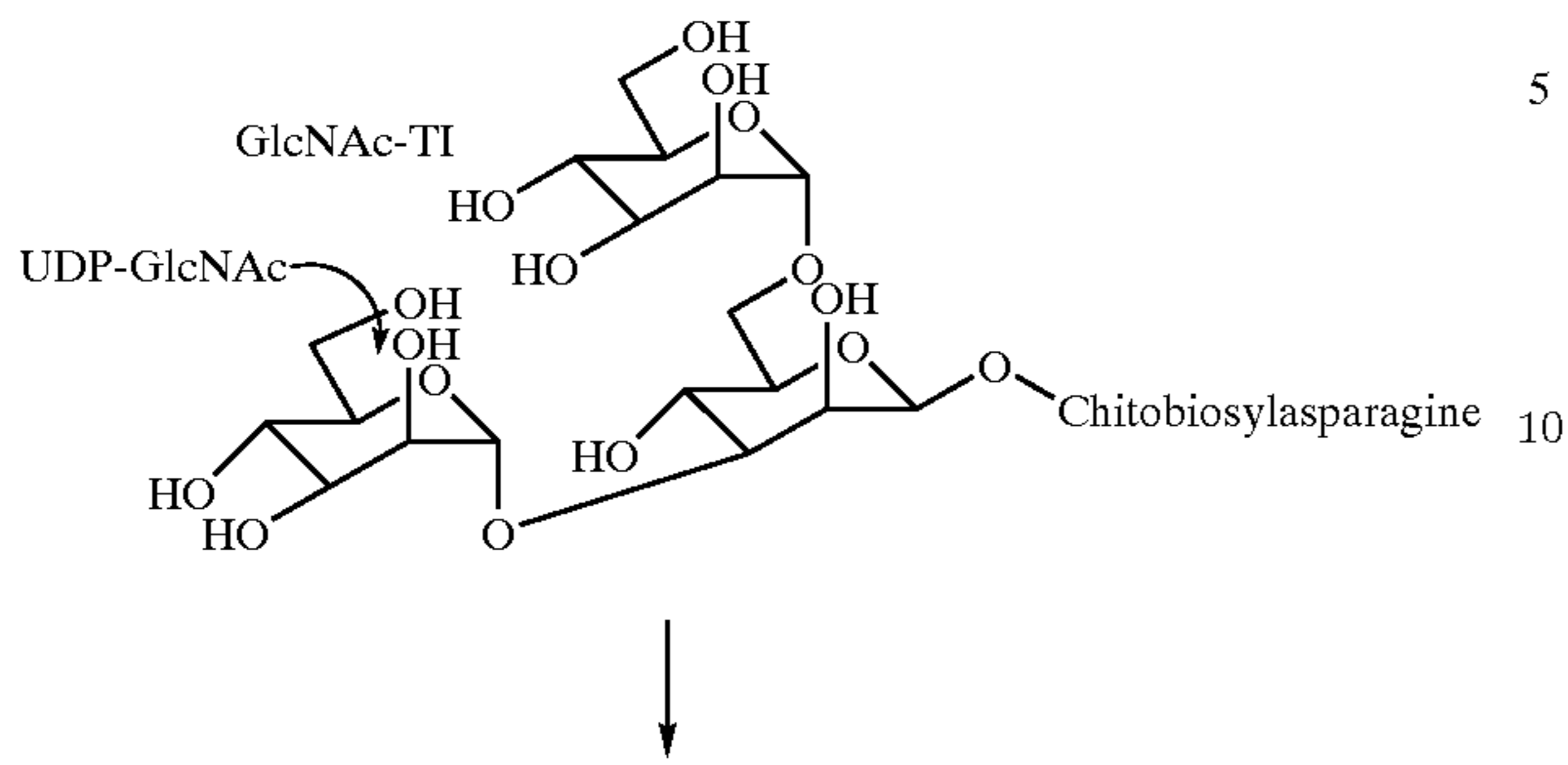
Scheme 10
