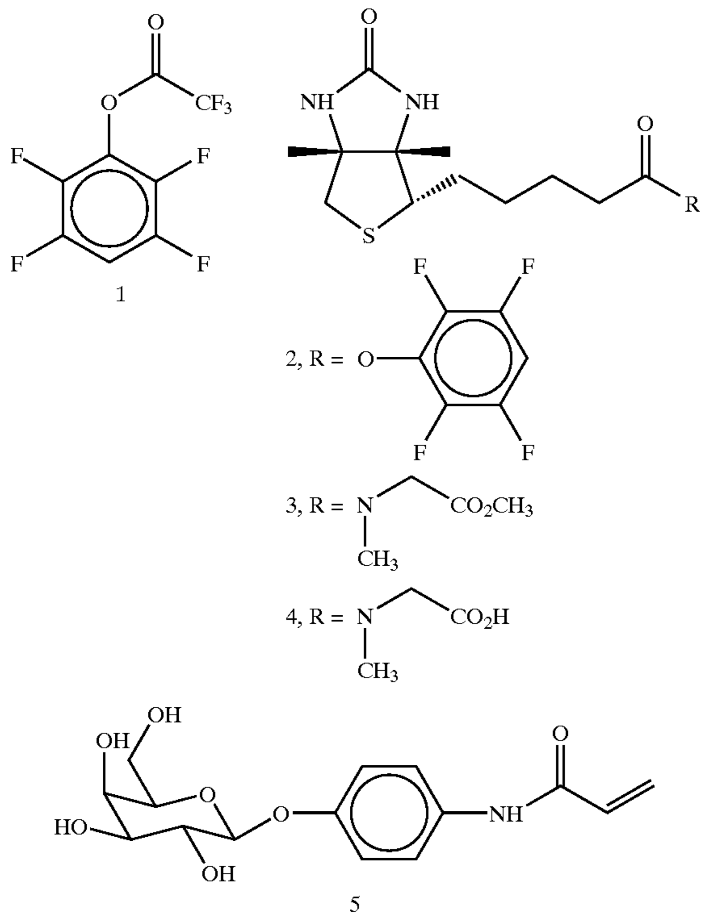
Scheme 14
