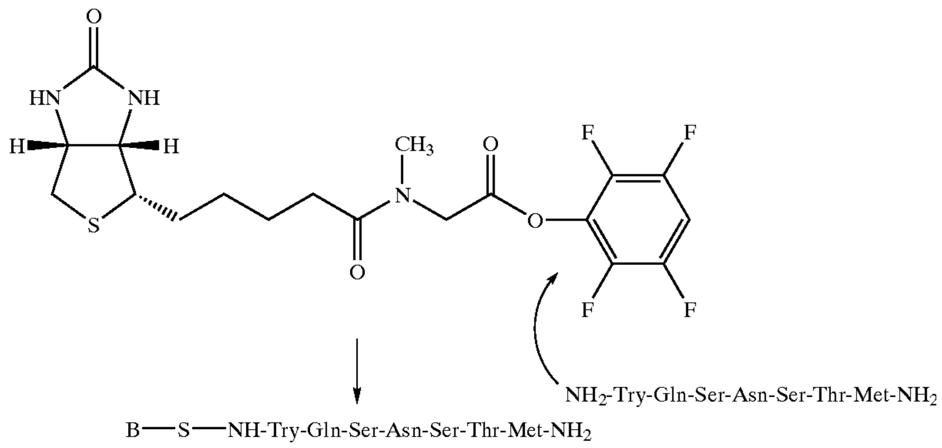
Scheme 13
