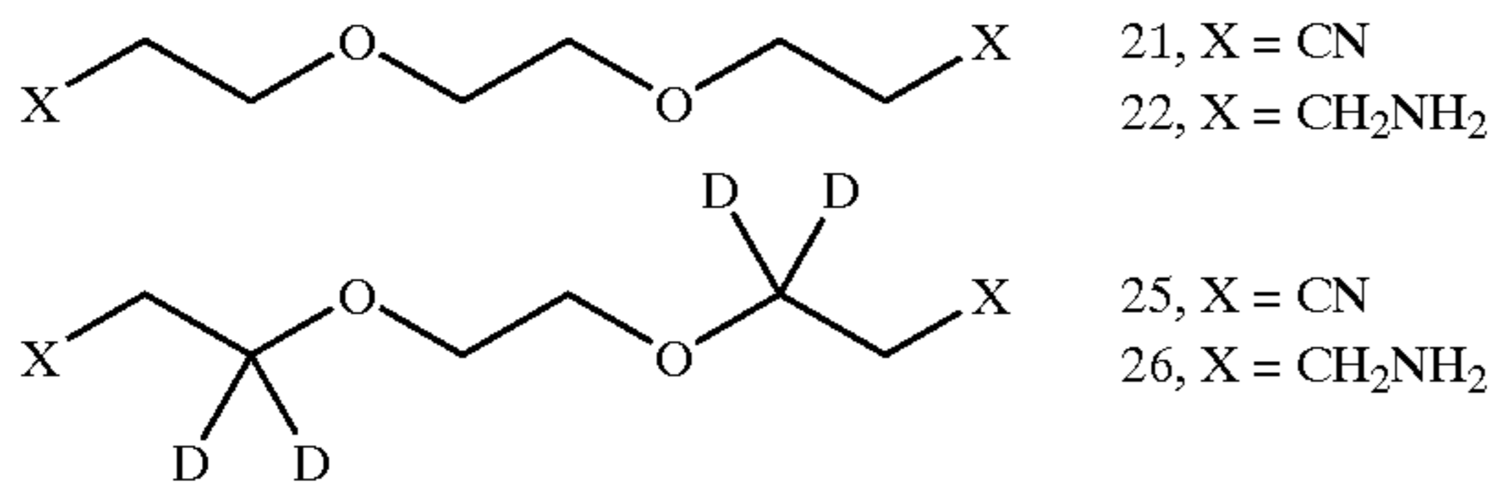
Scheme 19
