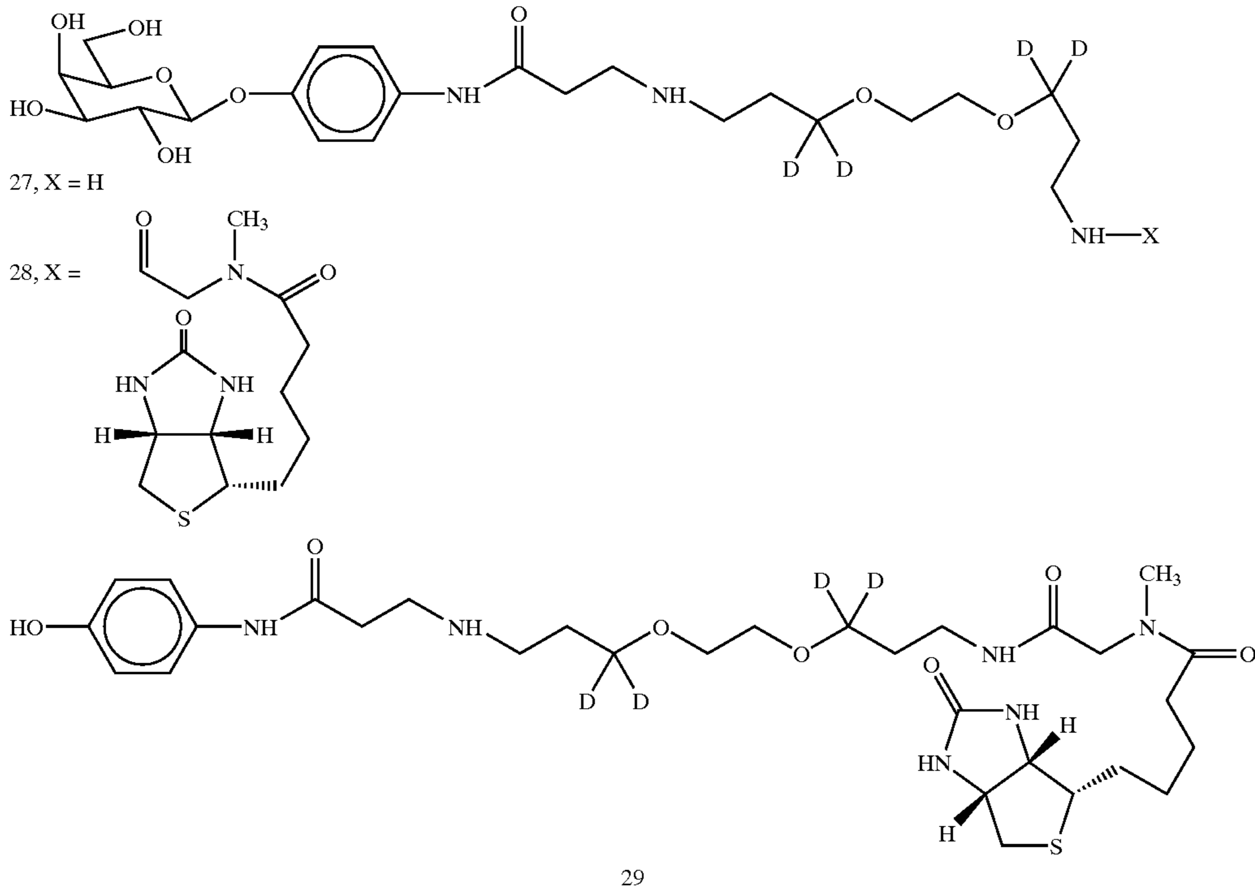
Scheme 19
