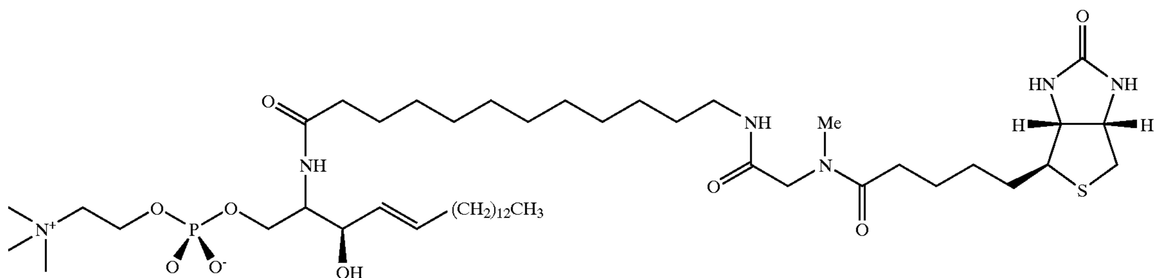
Scheme 7
