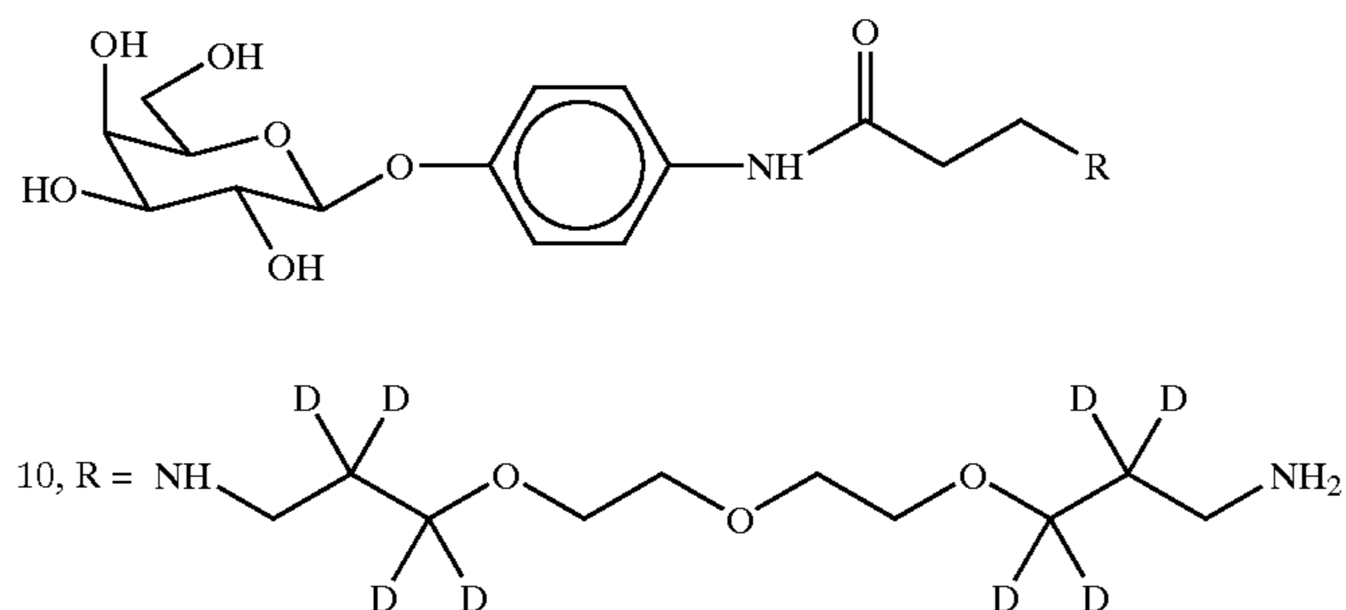
Scheme 16
