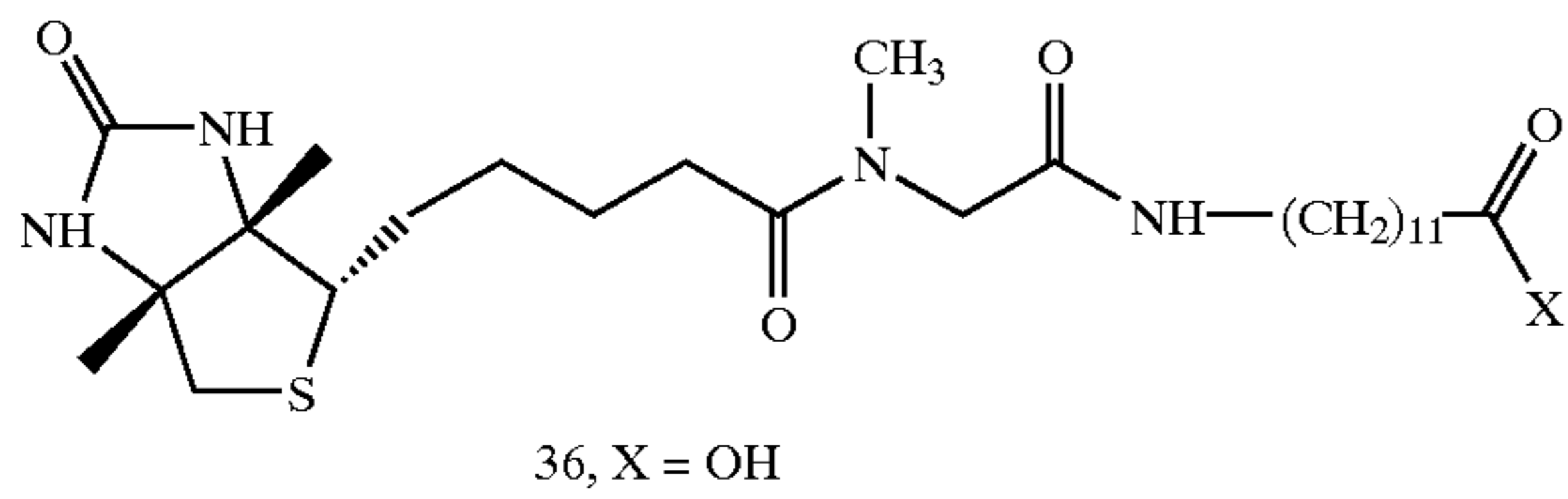
Scheme 22
