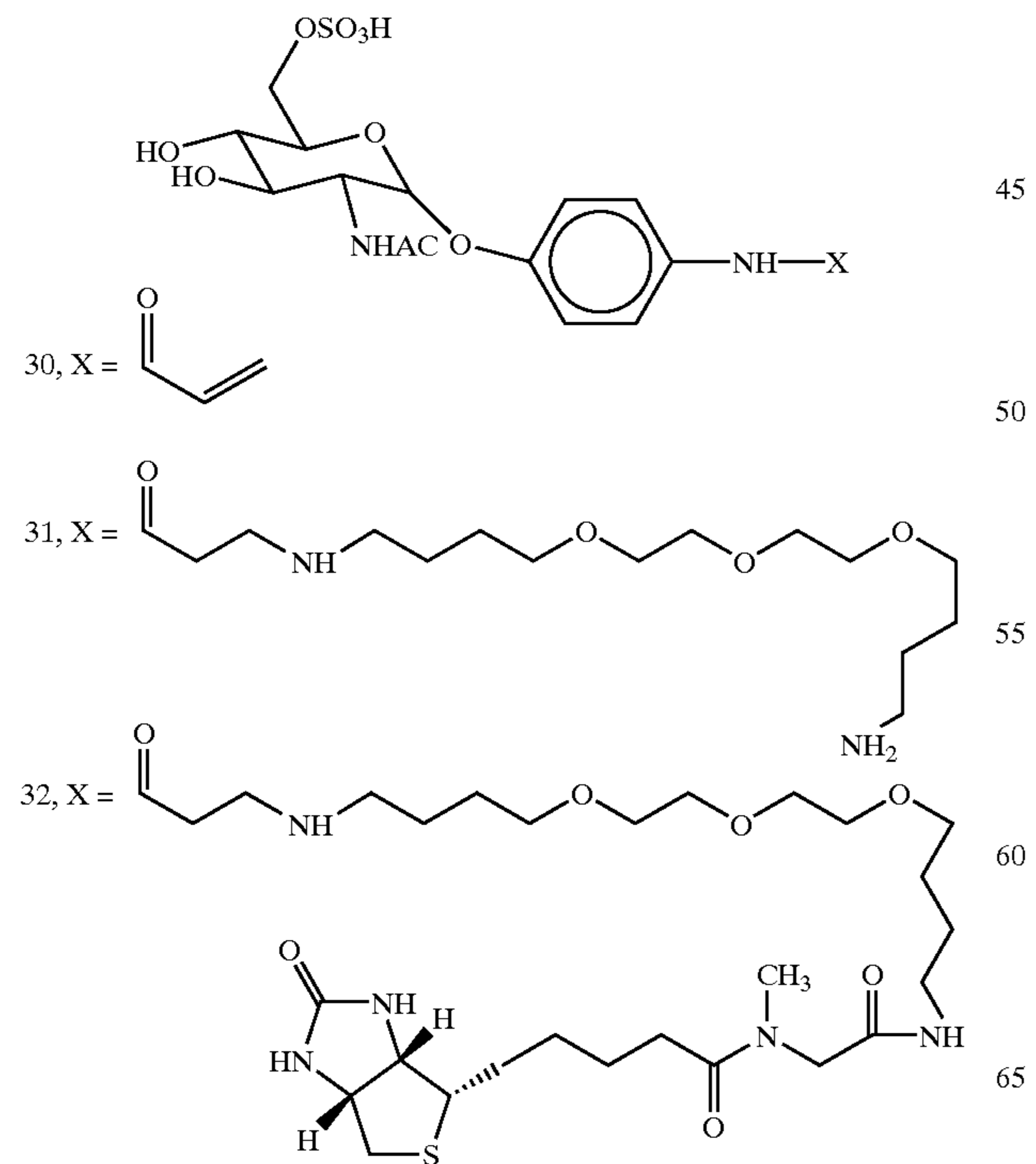
Scheme 20
