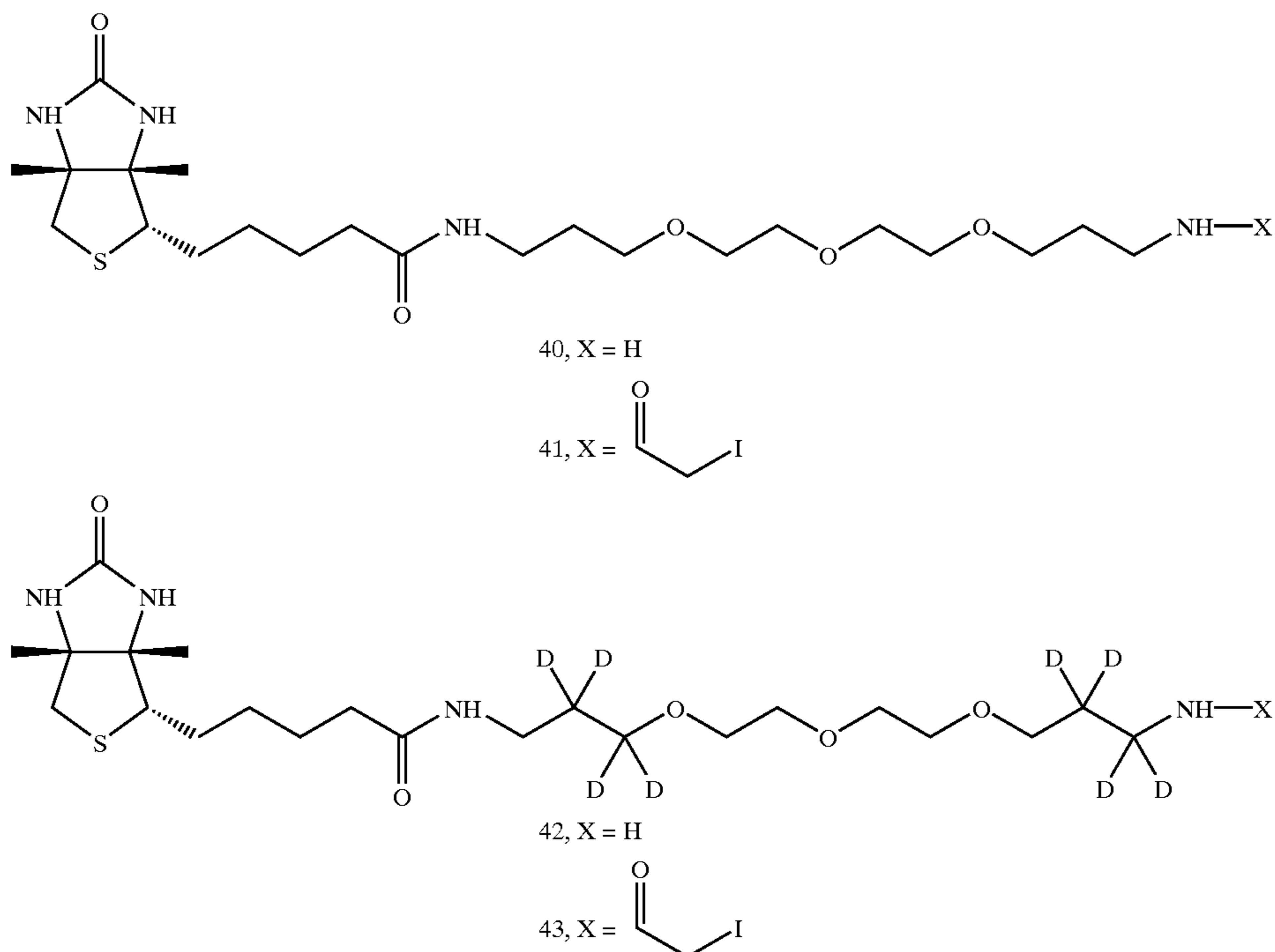
Scheme 23
