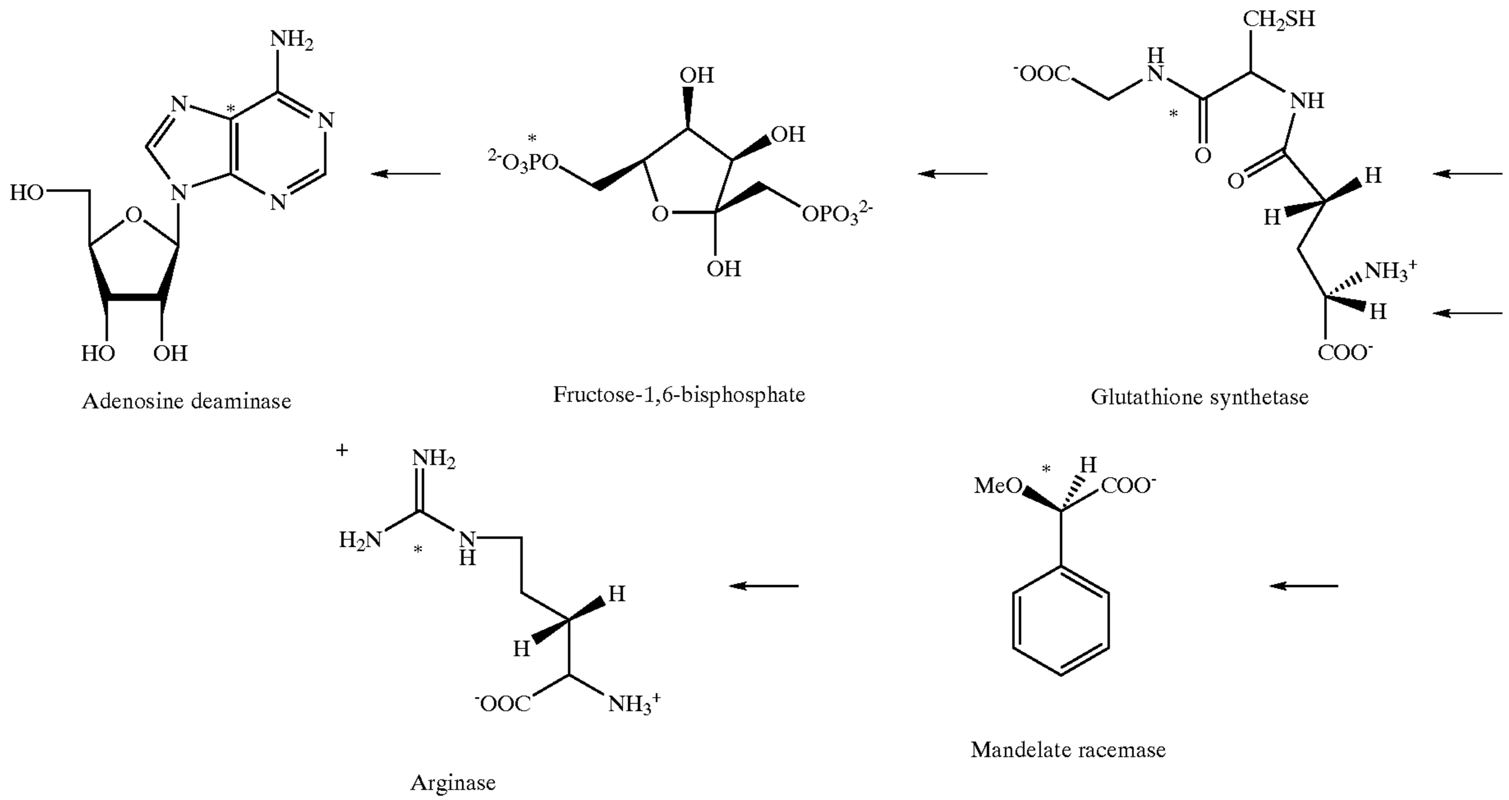
Scheme 6
