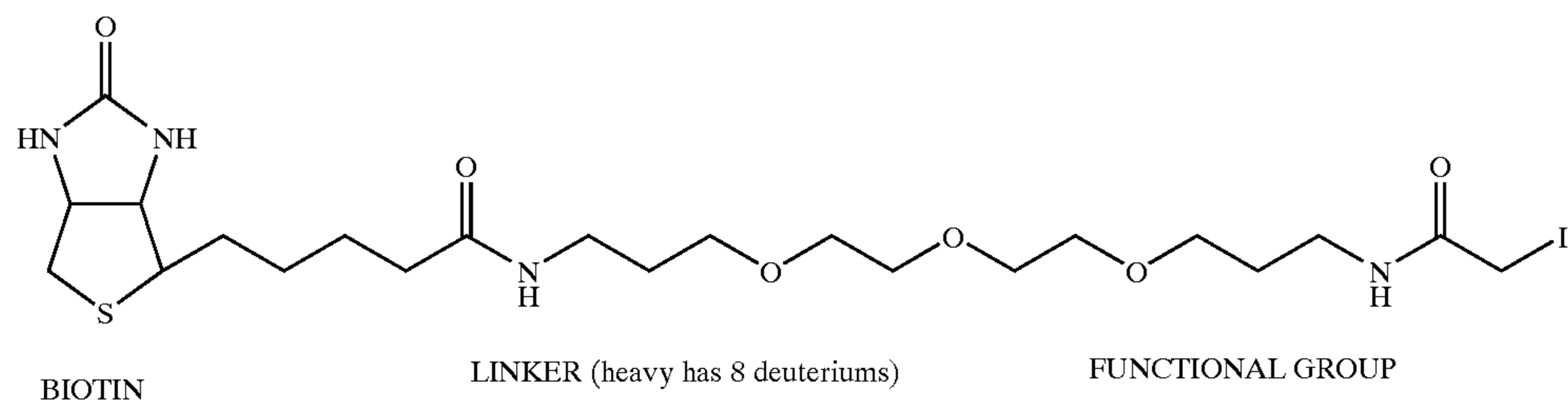
Scheme 1
