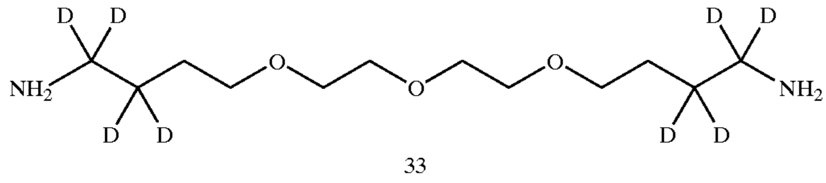
Scheme 21
