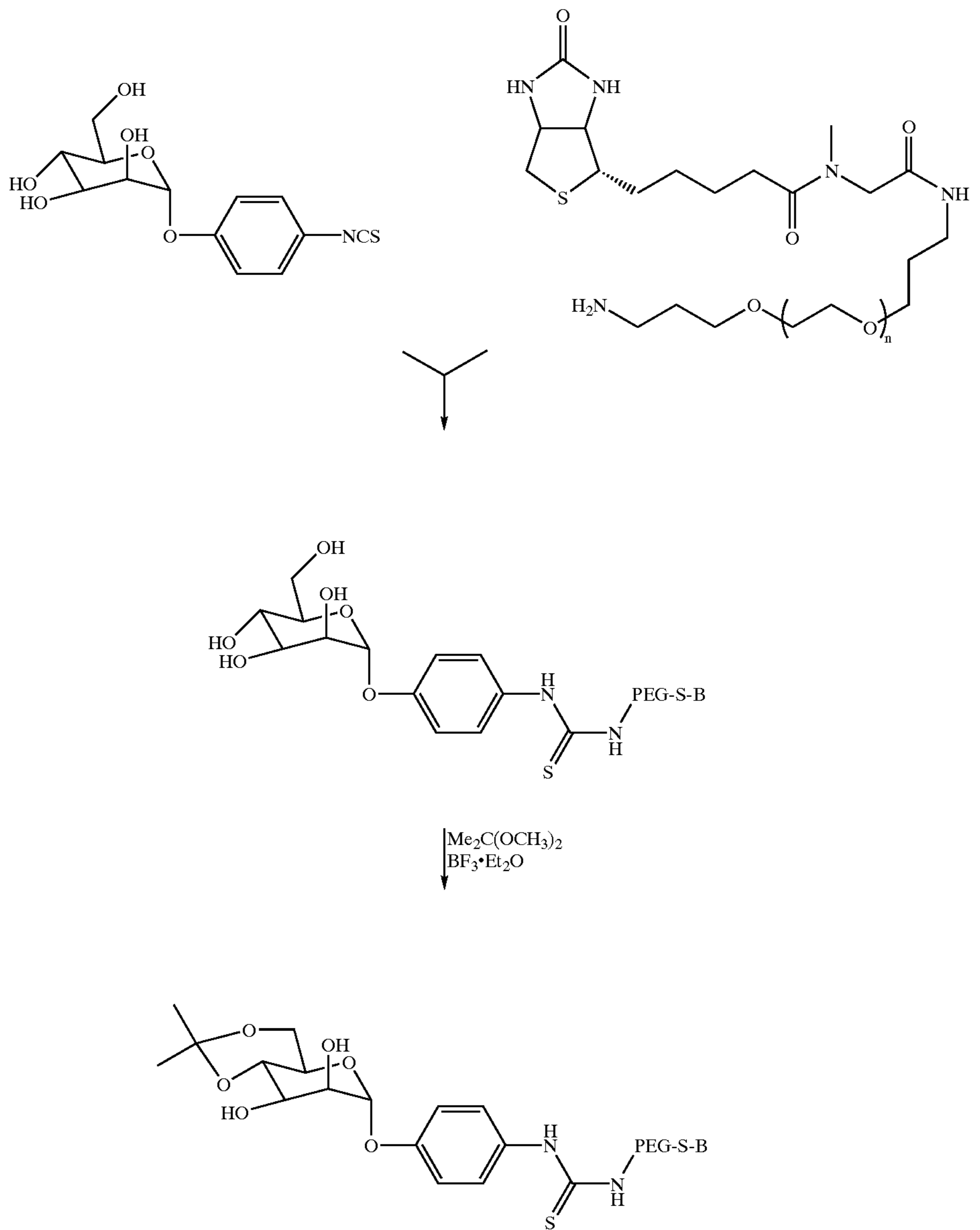
Scheme 11
