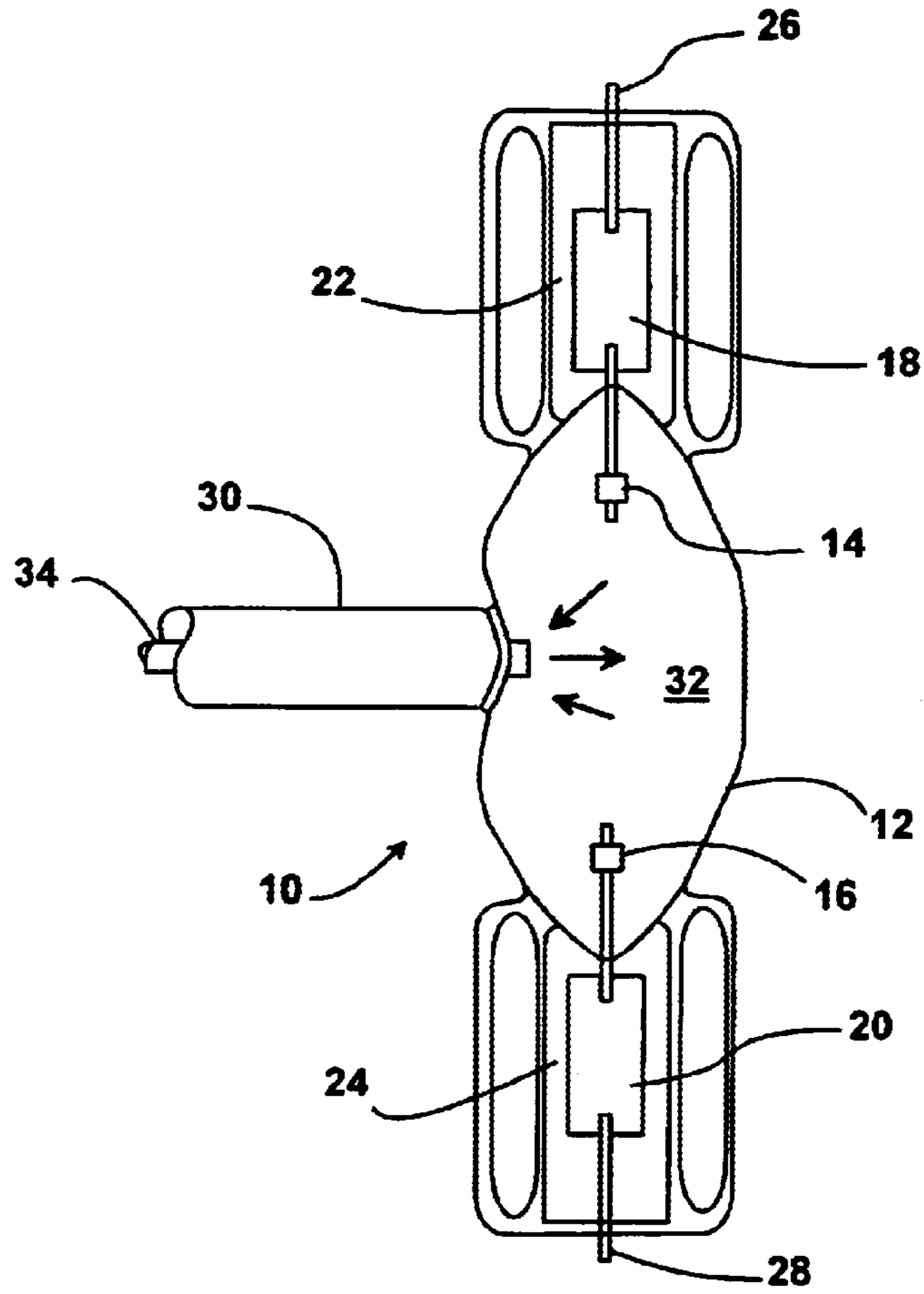
Fig. 1 (Prior Art)
