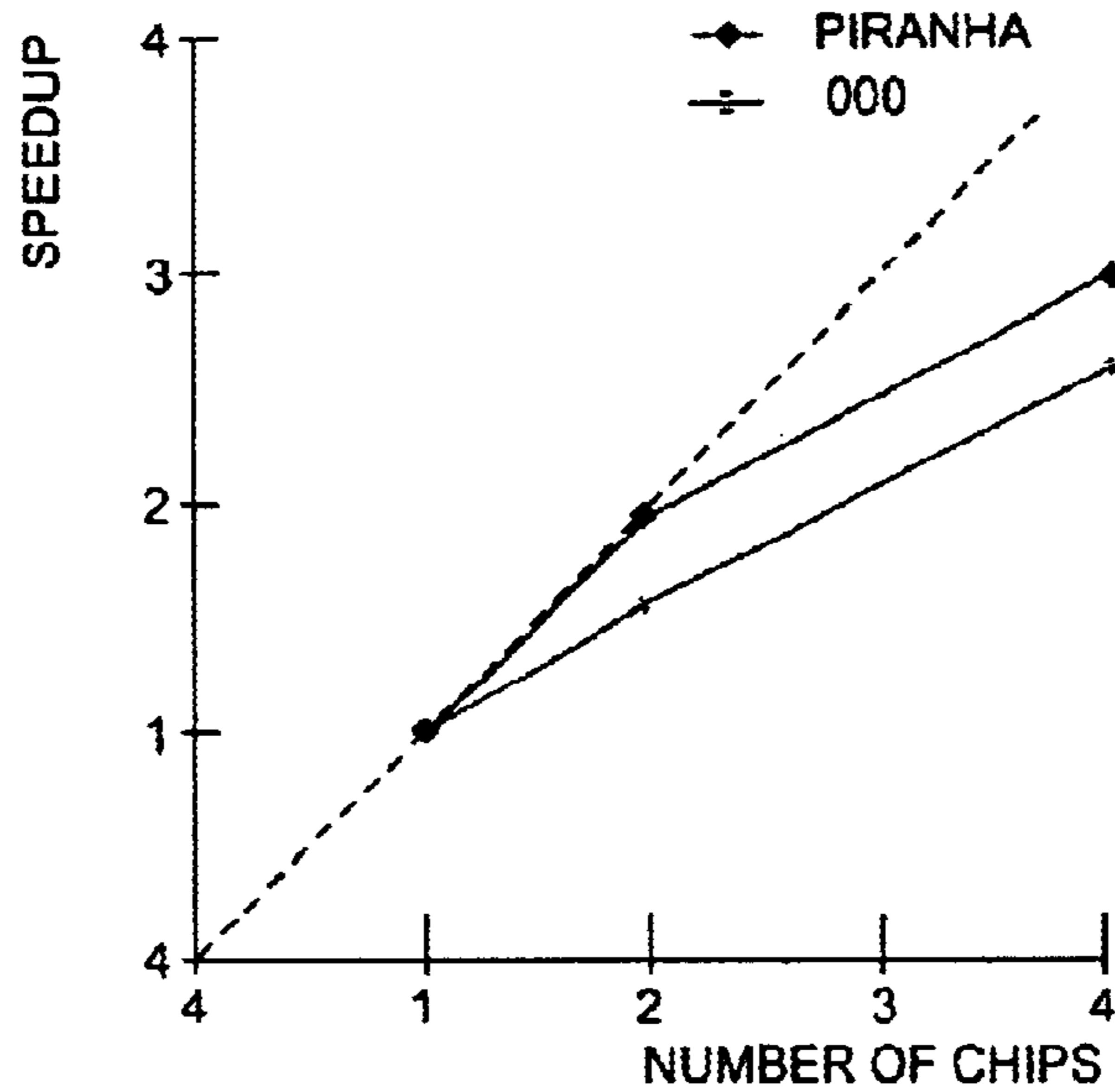
SPEEDUP OF OLTP IN MULTI-CHIP SYSTEMS WITH 500 Mhz 4-CPU PIRANHA CHIPS VERSUS 1 GHz OUT-OF-ORDER CHIPS. (A SINGLE-CHIP 4-CPU PIRANHA IS APPROXIMATELY 1.5x FASTER THAN THE SINGLE-CHIP 000)
