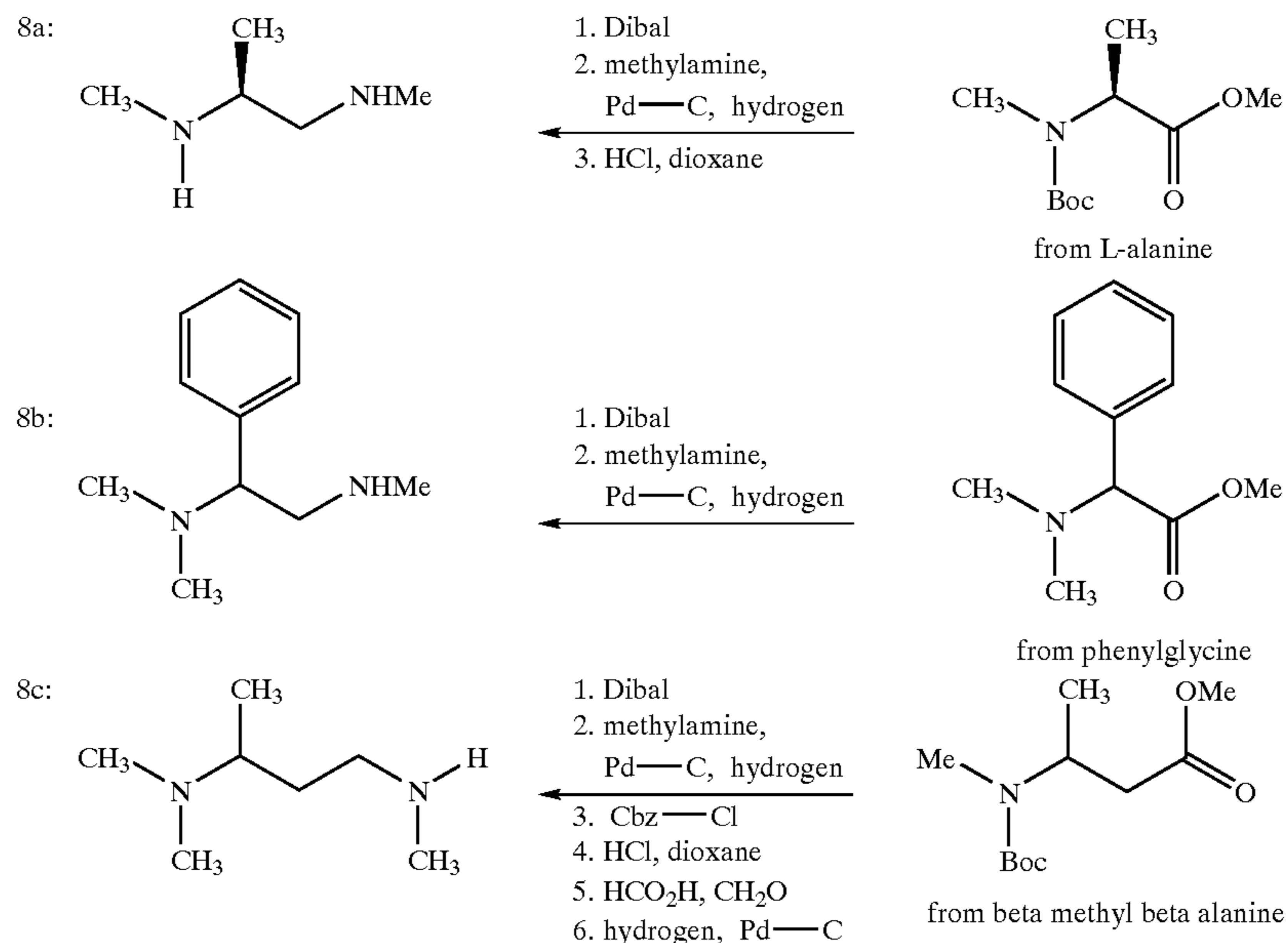
Synthetic Scheme 3
