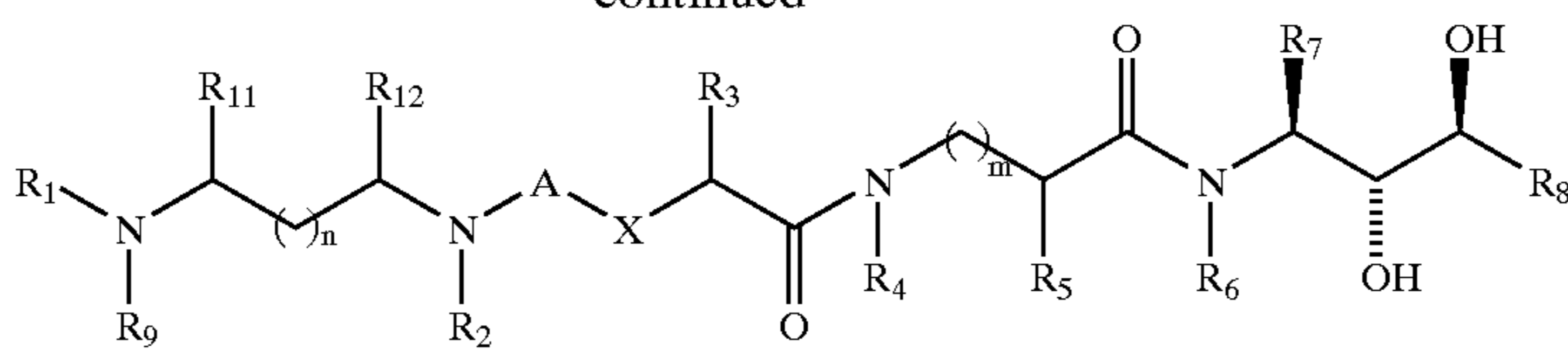
Formula I
