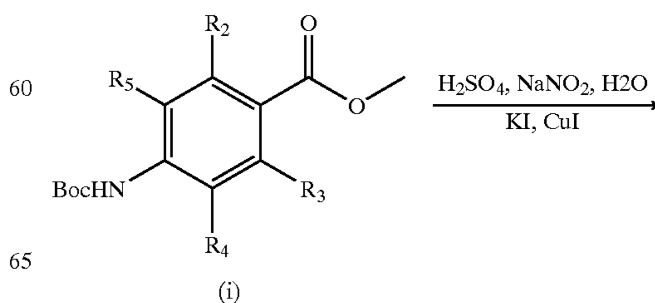
Scheme 4
