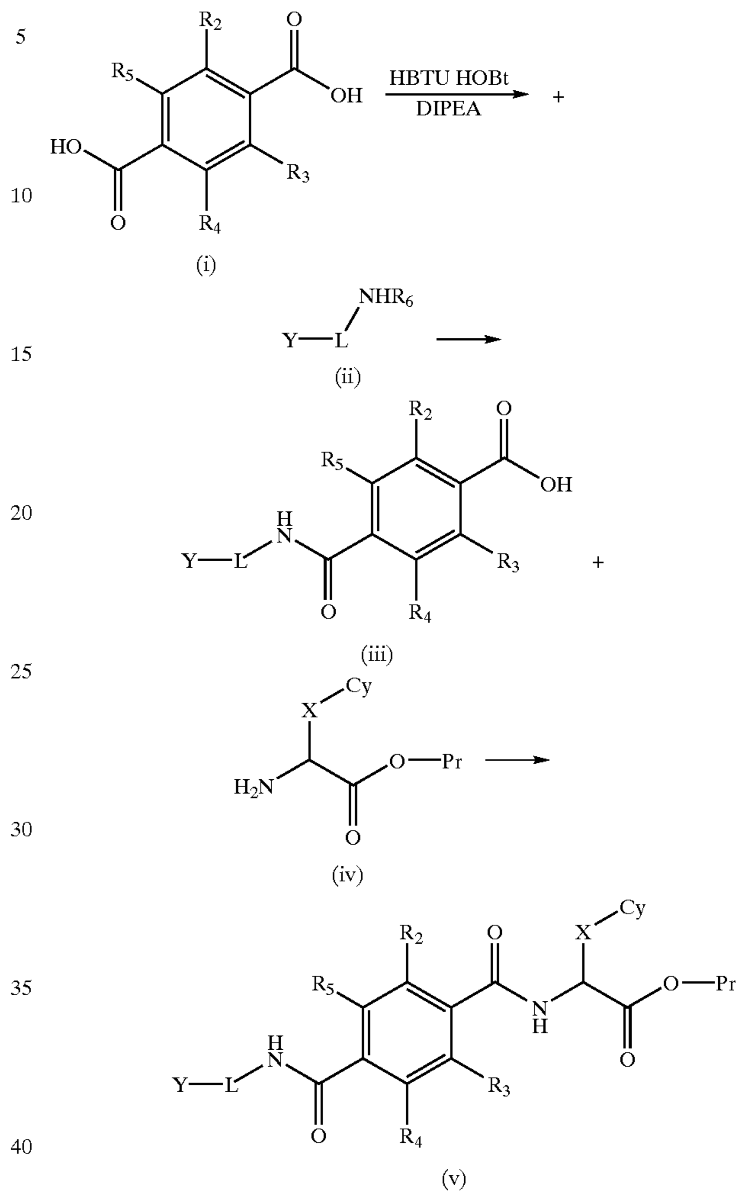
Scheme 3
