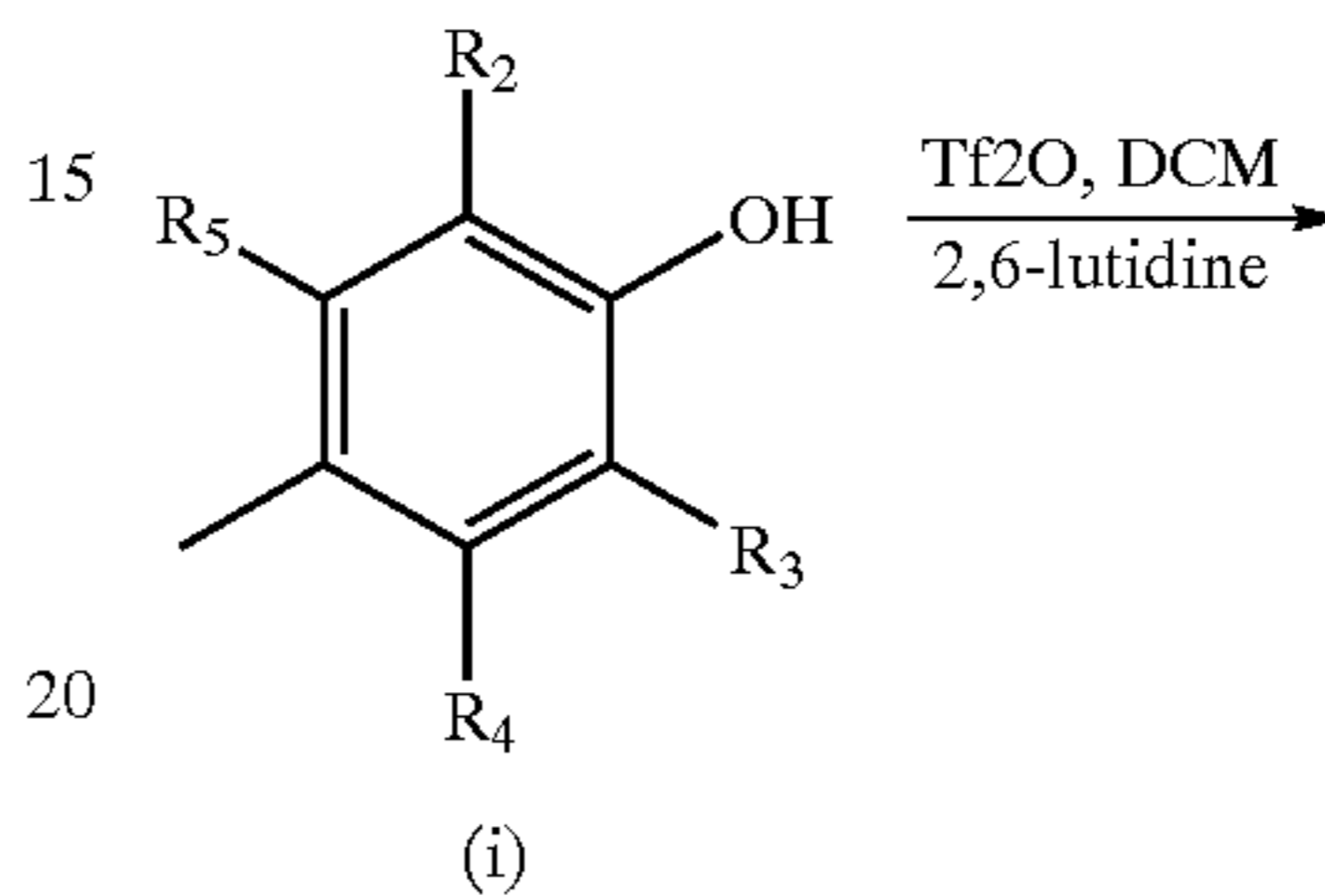
Scheme 5
