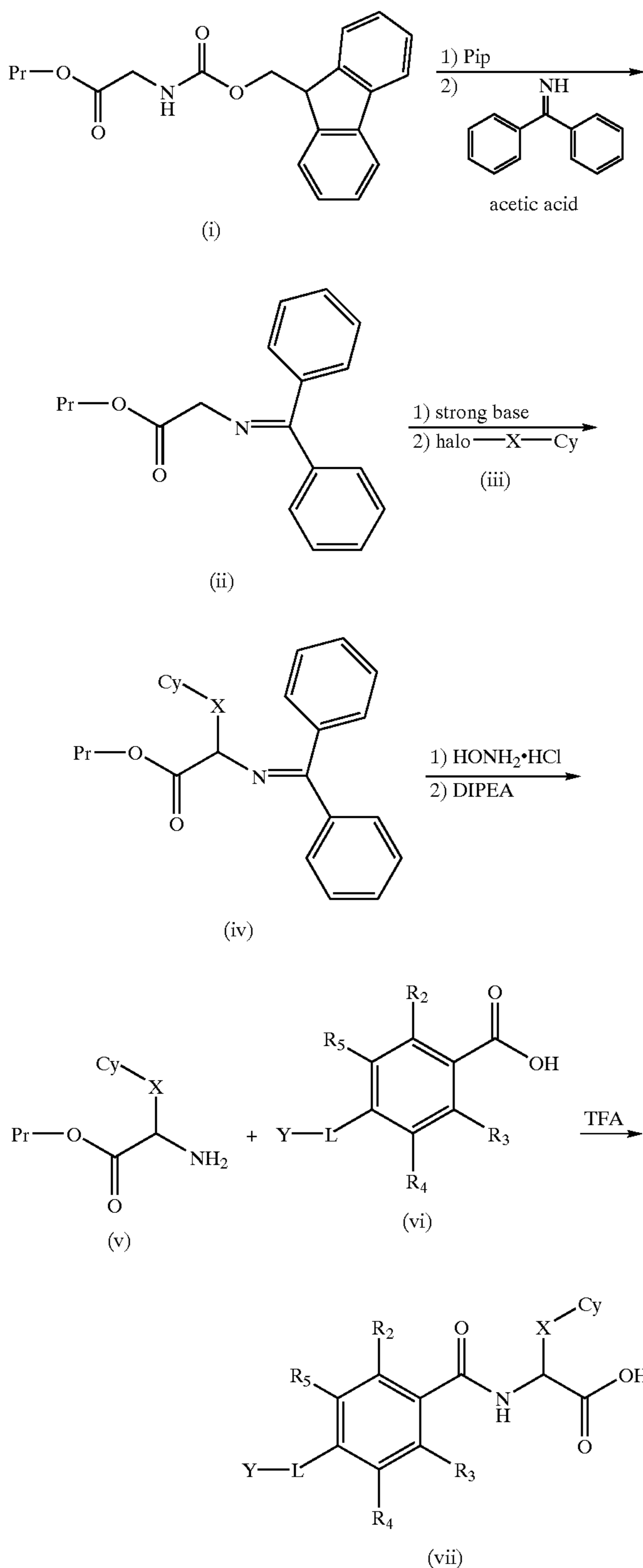
Scheme 1
