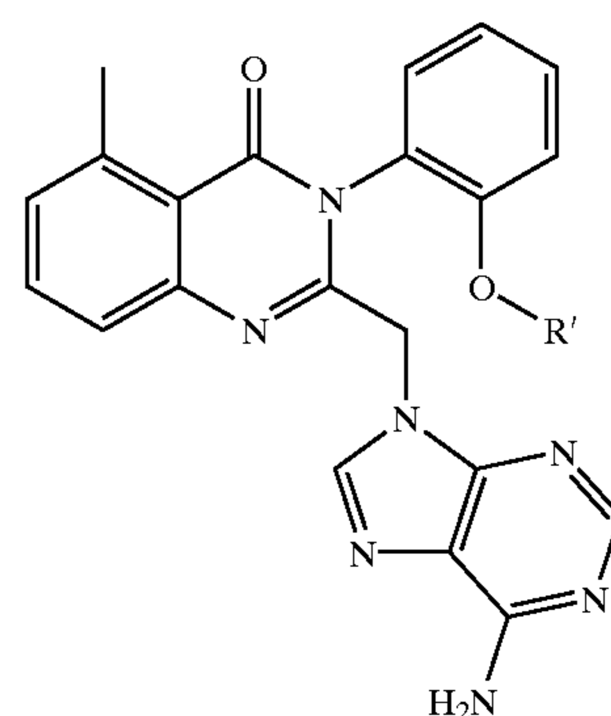
2-(6-Aminopurin-9-ylmethyl)-5-methyl-3-{2-(2-(1-methylpyrrolidin-2-yl)ethoxy)-phenyl}-3H-quinazolin-4-one (D-070C)
