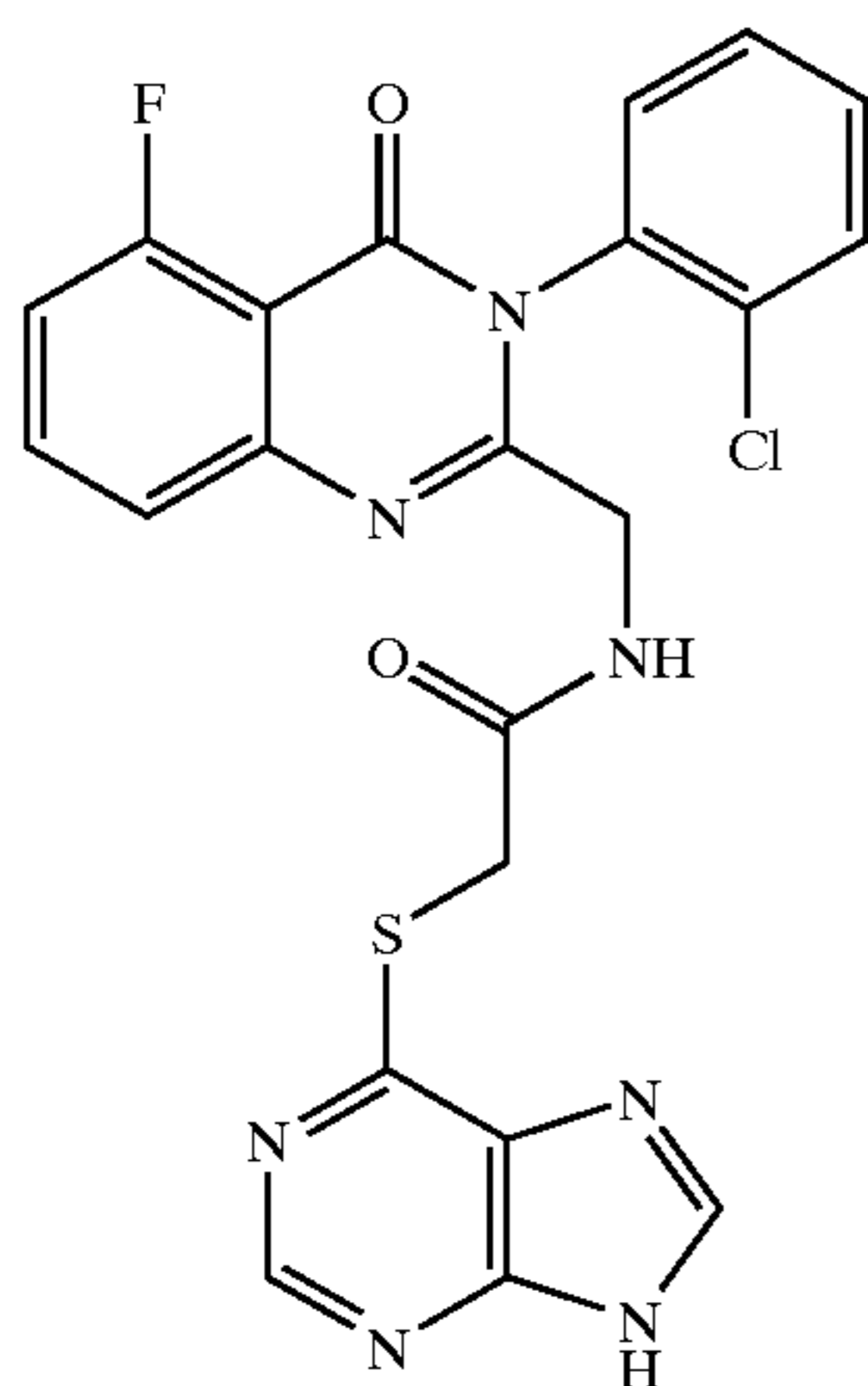
N-[3-(2-Chlorophenyl)-5-fluoro-4-oxo-3,4-dihydroquinazolin-2-ylmethyl]-2-(9H-purin-6-ylsulfanyl)-acetamide (D-077)
