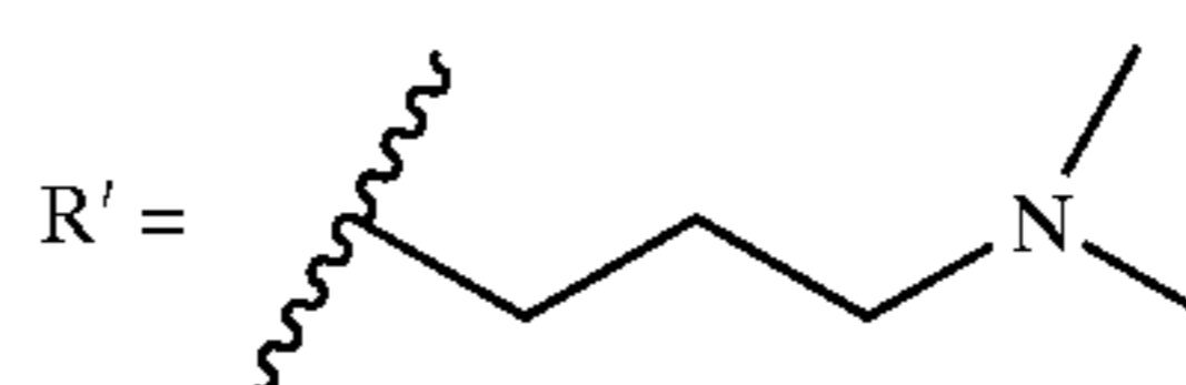
2-(6-Aminopurin-9-ylmethyl)-3-(2-(3-dimethylamino-propoxy)-phenyl)-5-methyl-3H-quinazolin-4-one (D-070D)
