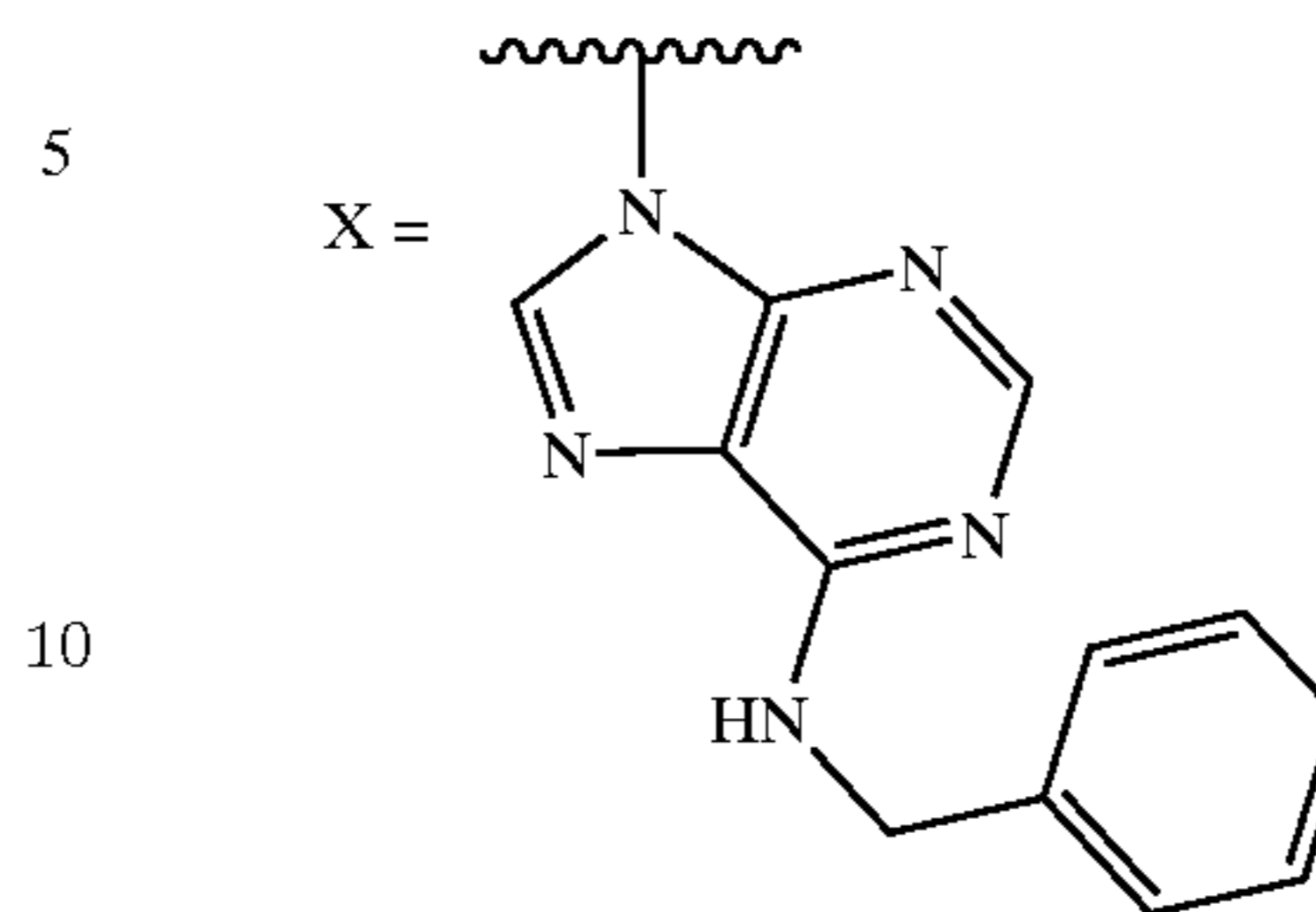
2-(6-Benzylaminopurin-9-ylmethyl)-5-methyl-3-o-tolyl-3H-quinazolin-4-one (D-108)
