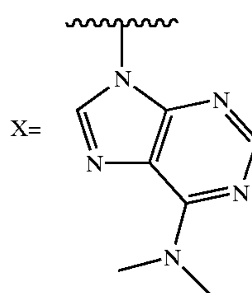
2-(6-Dimethylaminopurin-9-ylmethyl)-5-methyl-3-o-tolyl-3H-quinazolin-4-one (D-082)
