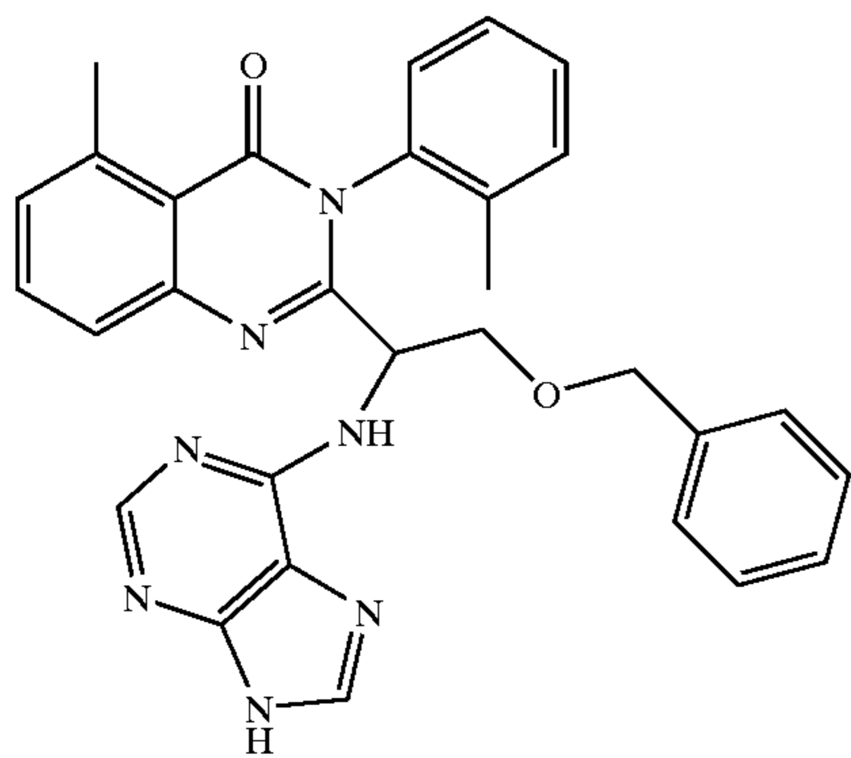
2-[2-Benzyloxy-1-(9H-purin-6-ylamino)ethyl]-5-methyl-3-o-tolyl-3H-quinazolin-4-one (D-081e)
