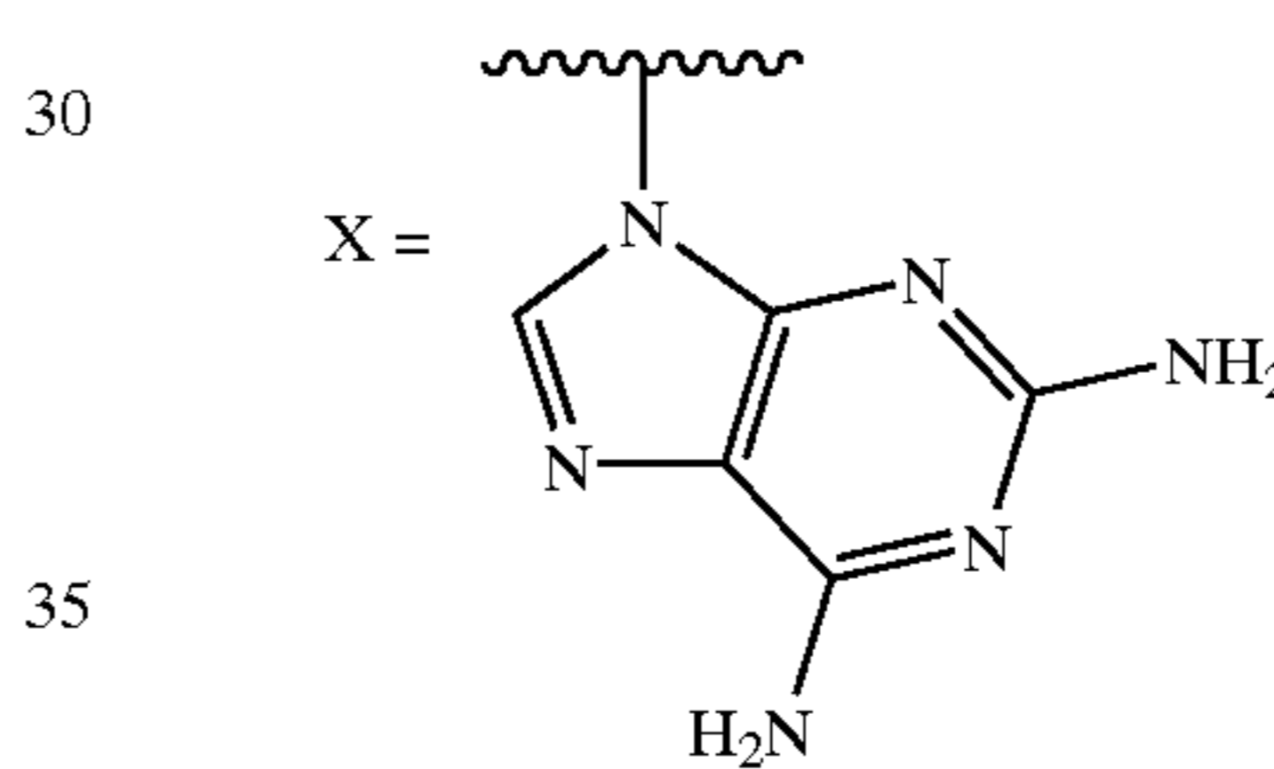
2-(2,6-Diaminopurin-9-ylmethyl)-5-methyl-3-o-tolyl-3H-quinazolin-4-one (D-109)
