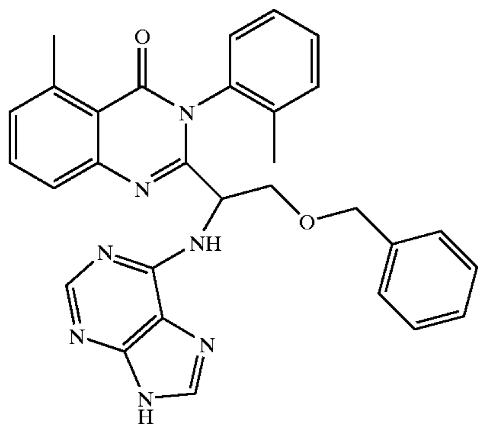
2-[2-Benzyloxy-1-(9H-purin-6-ylamino)ethyl]-5-methyl-3-o-tolyl-3H-quinazolin-4-one (D-081e)
