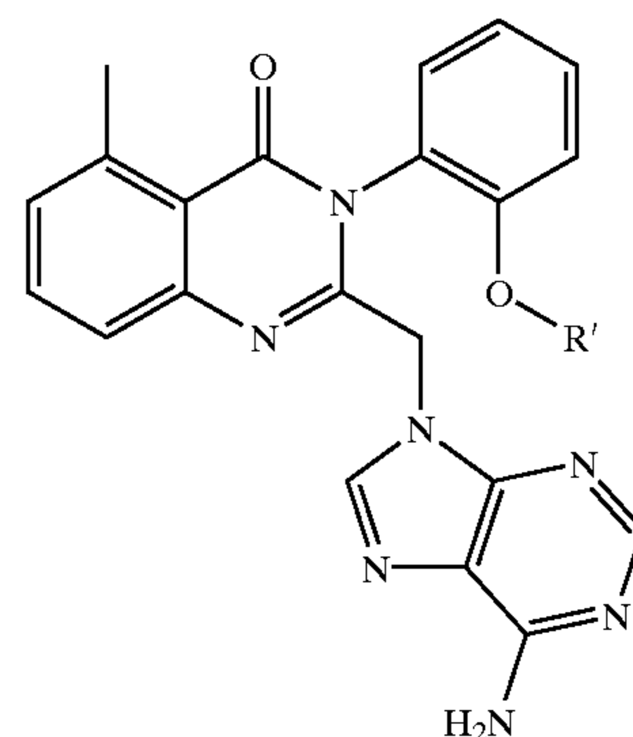
2-(6-Aminopurin-9-ylmethyl)-5-methyl-3-{2-(2-(1-methylpyrrolidin-2-yl)ethoxy)-phenyl}-3H-quinazolin-4-one (D-070C)
