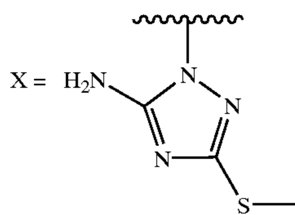
2-(5-Amino-3-methylsulfanyl-1,2,4-triazol-1-ylmethyl)-5-methyl-3-o-tolyl-3H-quinazolin-4-one (D-106)
