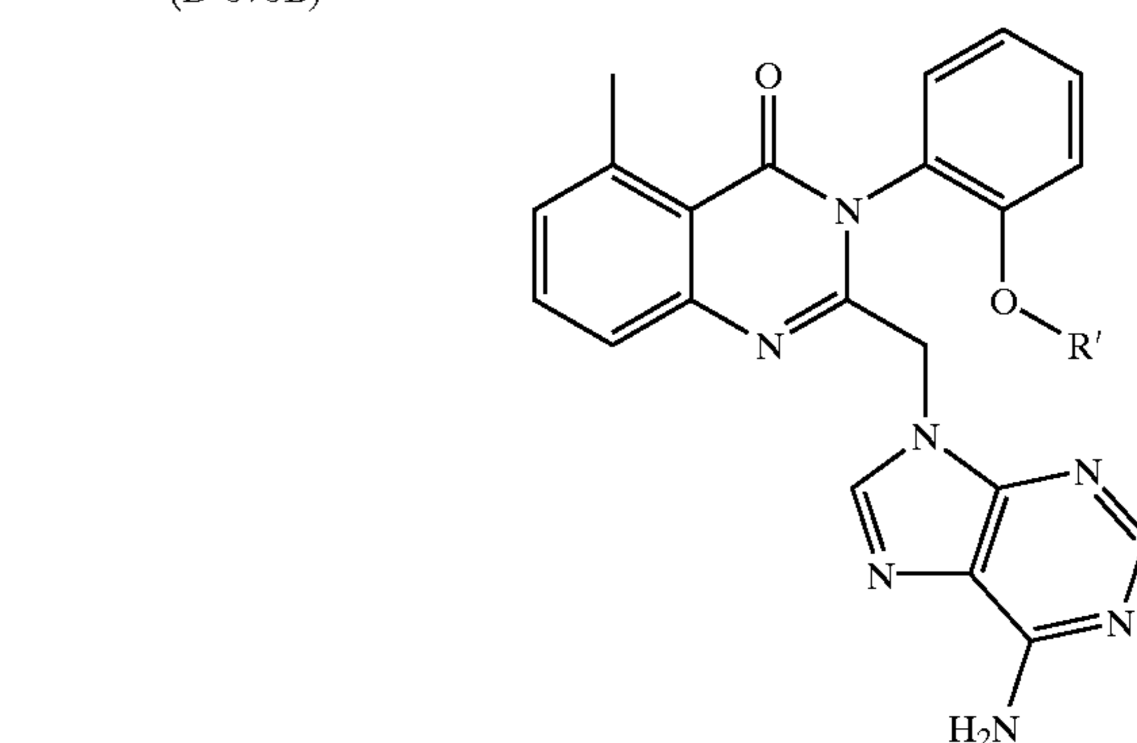
2-(6-Aminopurin-9-ylmethyl)-5-methyl-3-{2-(2-(1-methylpyrrolidin-2-yl)-ethoxy)-phenyl}-3H-quinazolin-4-one (D-070C)
