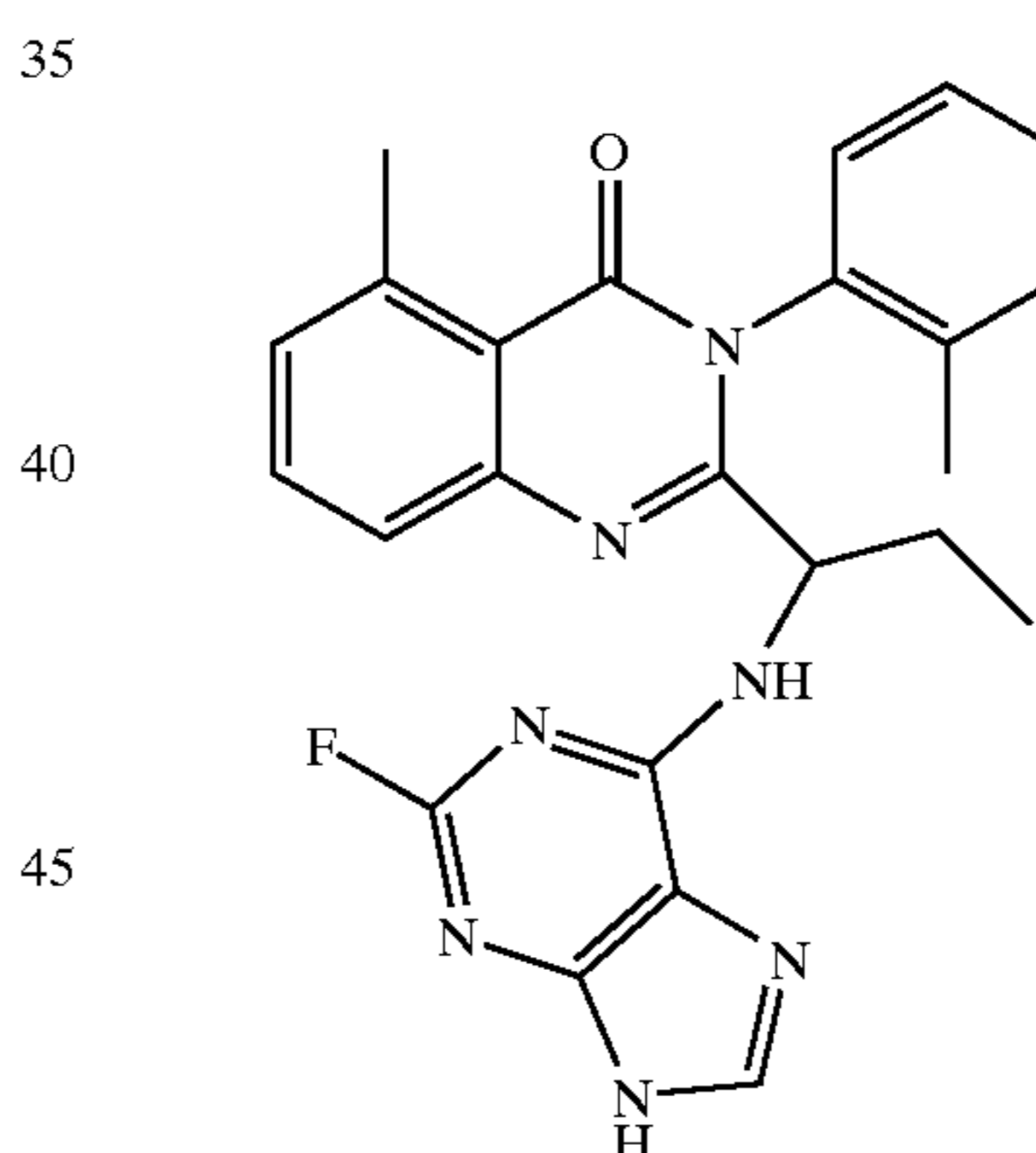
2-(1-(2-Amino-9H-purin-6-ylamino)ethyl)-5-methyl-3-o-tolyl-3H-quinazolin-4-one (D-081a)
