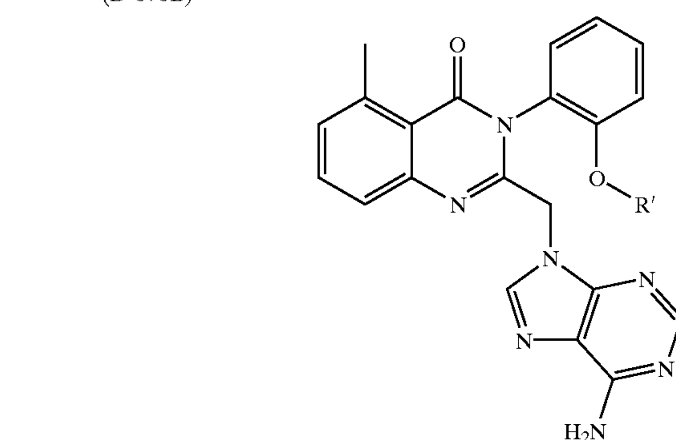
2-(6-Aminopurin-9-ylmethyl)-5-methyl-3-{2-(2-(1-methylpyrrolidin-2-yl)-ethoxy)-phenyl}-3H-quinazolin-4-one (D-070C)
