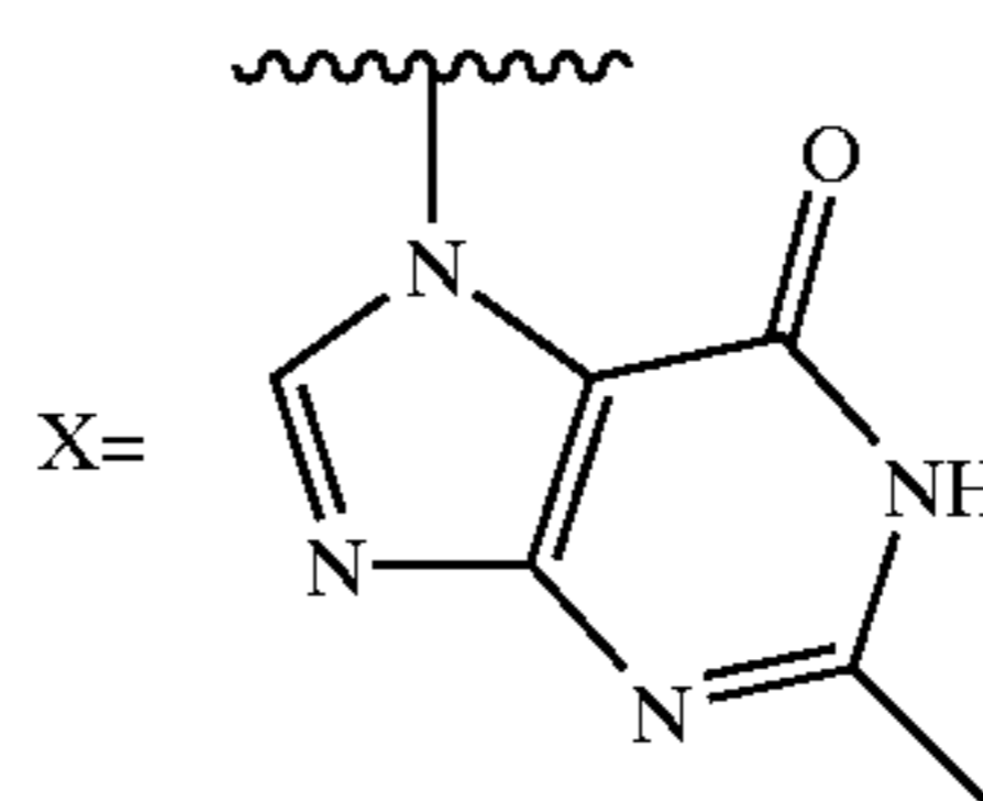
5-Methyl-2-(2-methyl-6-oxo-1,6-dihydro-purin-7-ylmethyl)-3-o-tolyl-3H-quinazolin-4-one (D-083)
