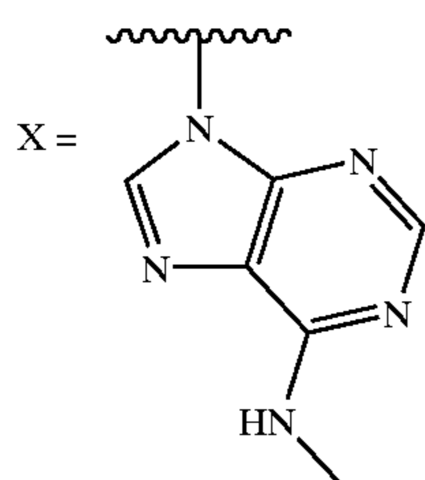
5-Methyl-2-(6-methylaminopurin-9-ylmethyl)-3-o-tolyl-3H-quinazolin-4-one (D-107)
