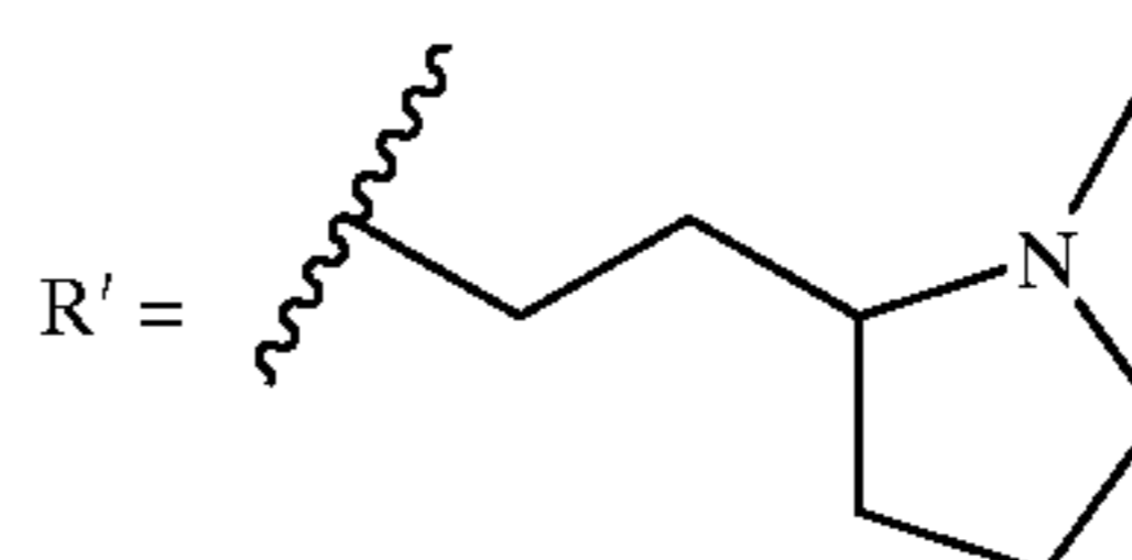
2-(6-Aminopurin-9-ylmethyl)-5-methyl-3-{2-(2-(1-methylpyrrolidin-2-yl)-ethoxy)-phenyl}-3H-quinazolin-4-one (D-070C)
