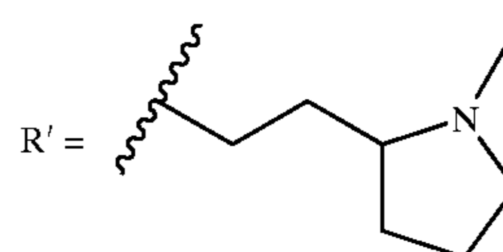
2-(6-Aminopurin-9-ylmethyl)-5-methyl-3-{2-(2-(1-methylpyrrolidin-2-yl)ethoxy)-phenyl}-3H-quinazolin-4-one (D-070C)
