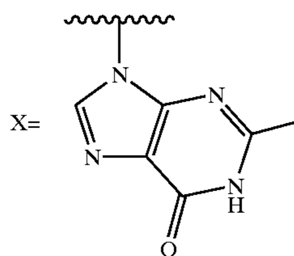
5-Methyl-2-(2-methyl-6-oxo-1,6-dihydro-purin-9-ylmethyl)-3-o-tolyl-3H-quinazolin-4-one (D-084)
