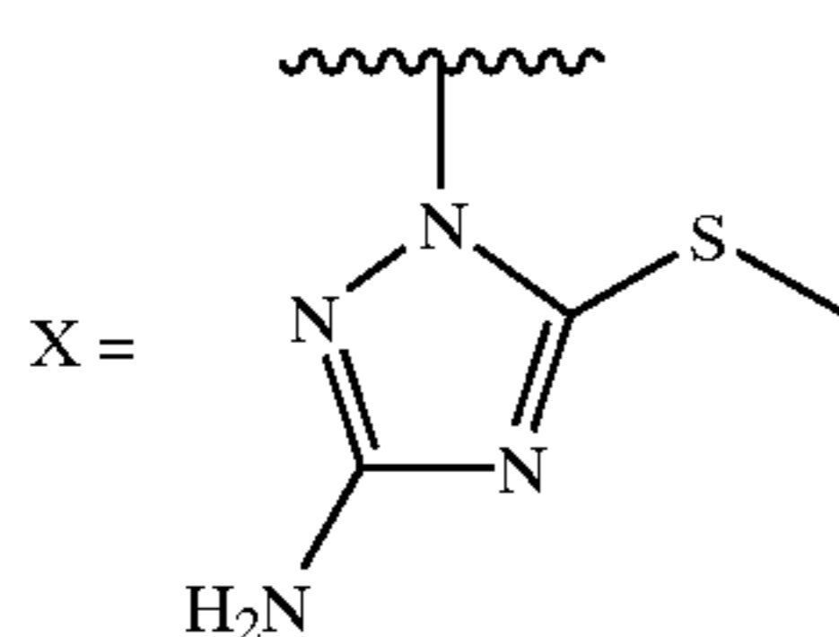
2-(3-Amino-5-methylsulfanyl-1,2,4-triazol-1-ylmethyl)-5-methyl-3-o-tolyl-3H-quinazolin-4-one (D-105)
