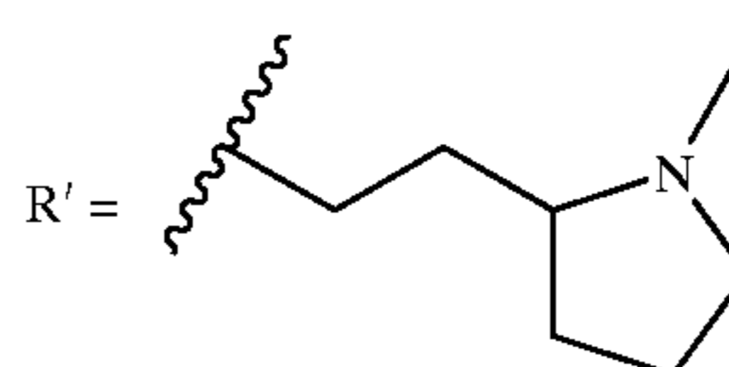
2-(6-Aminopurin-9-ylmethyl)-5-methyl-3-{2-(2-(1-methylpyrrolidin-2-yl)ethoxy)-phenyl}-3H-quinazolin-4-one (D-070C)
