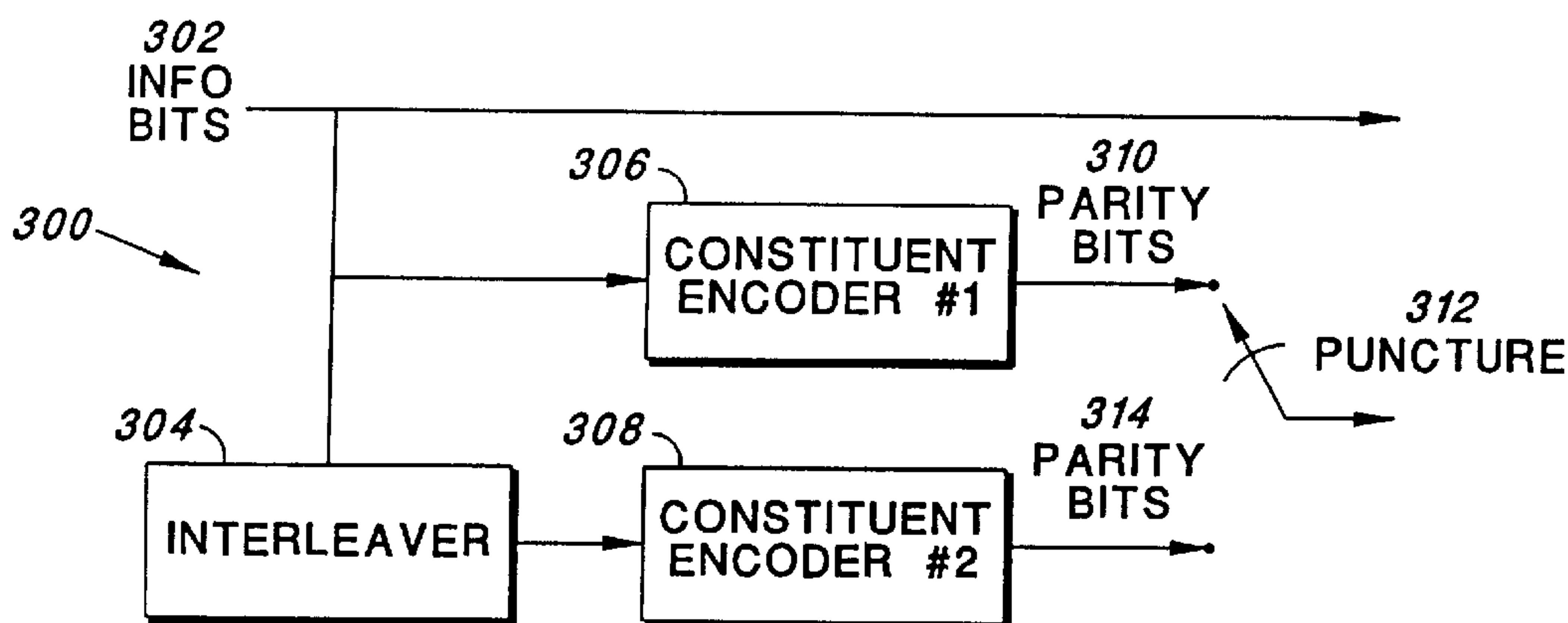
GENERIC TURBO CODE ENCODER BLOCK DIAGRAM
