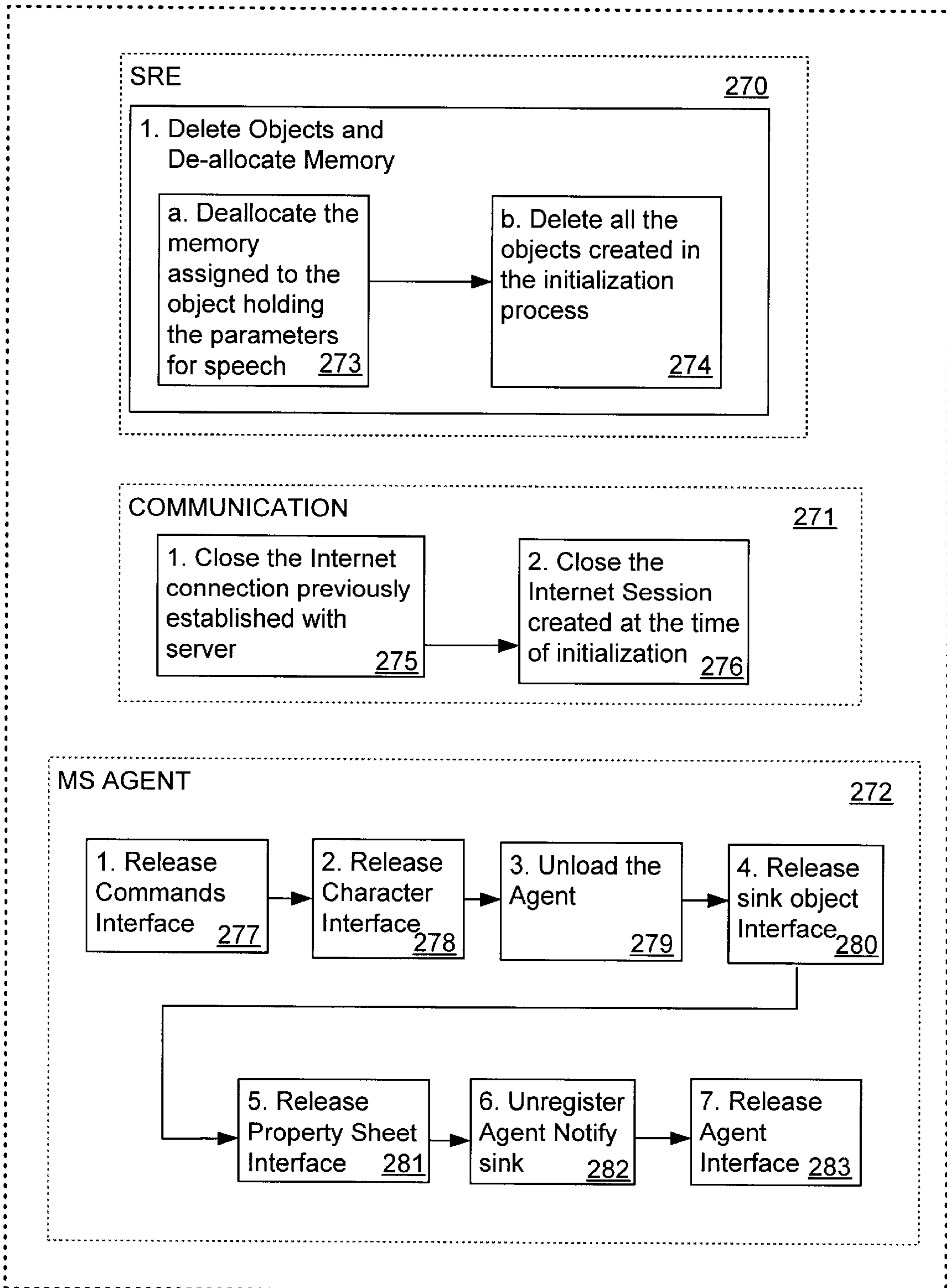
Fig. 4 Client-side Un-Initialization
