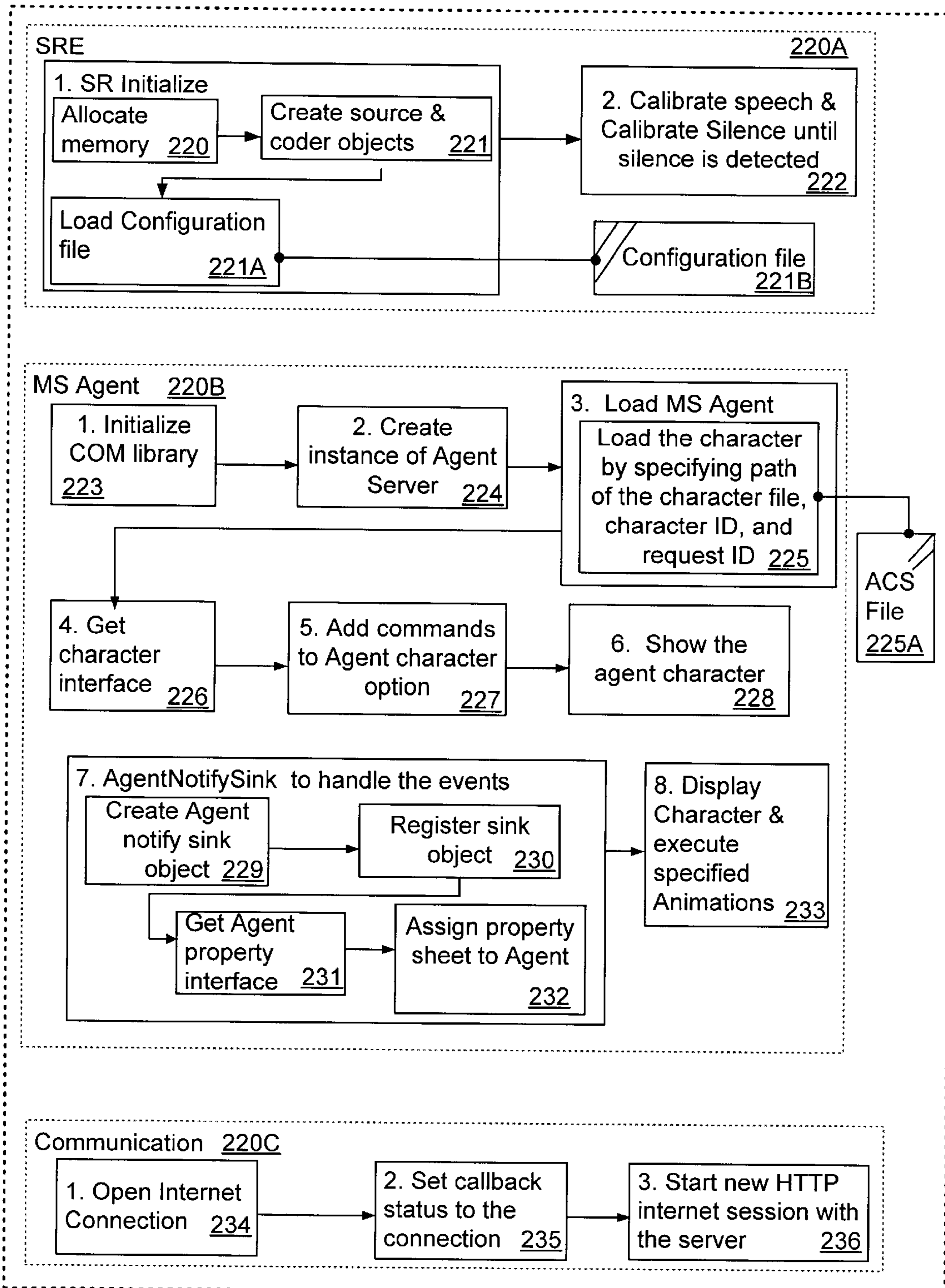
Fig. 2-2 Client-side Initialization
