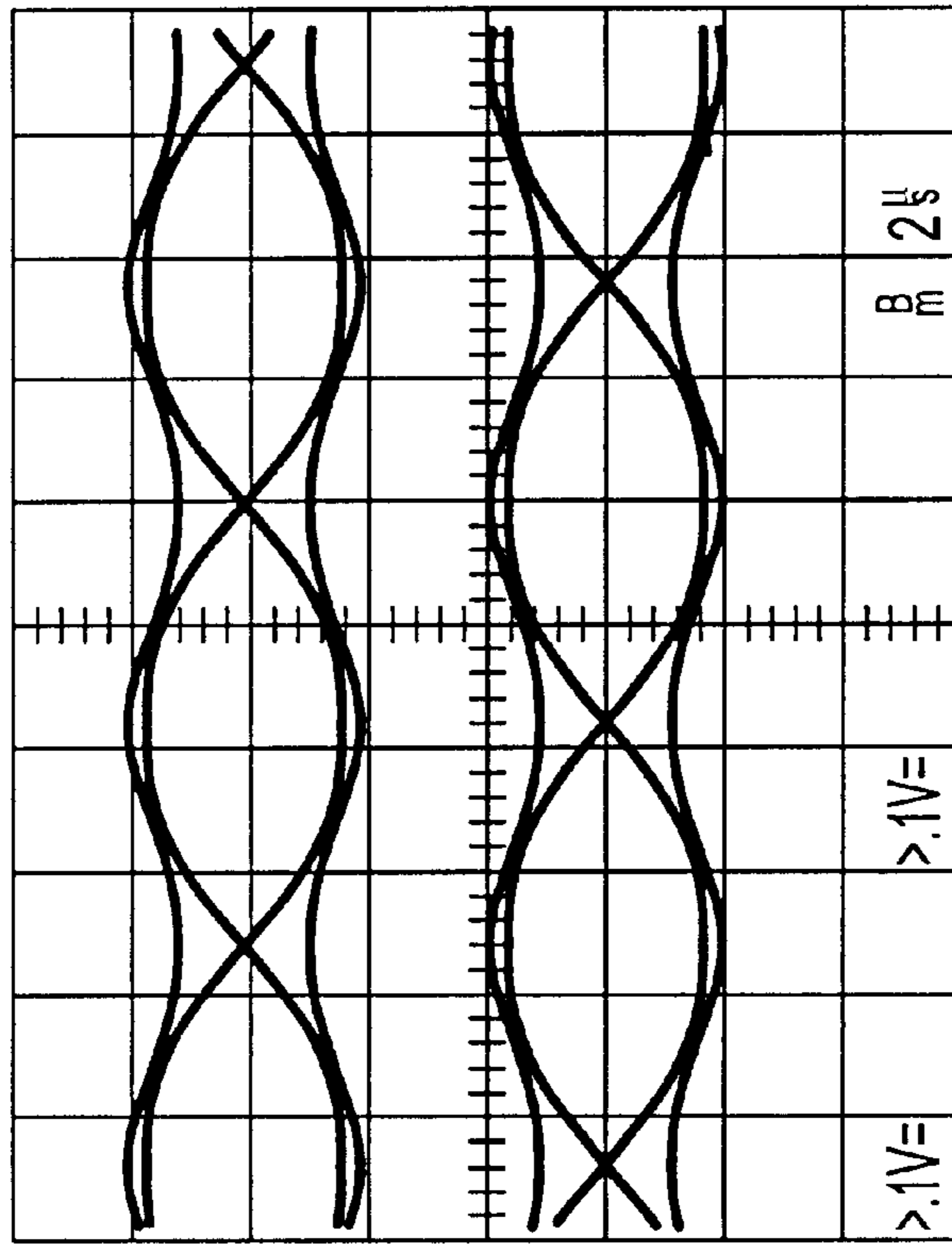
FGMSK (BTb=0.3)
