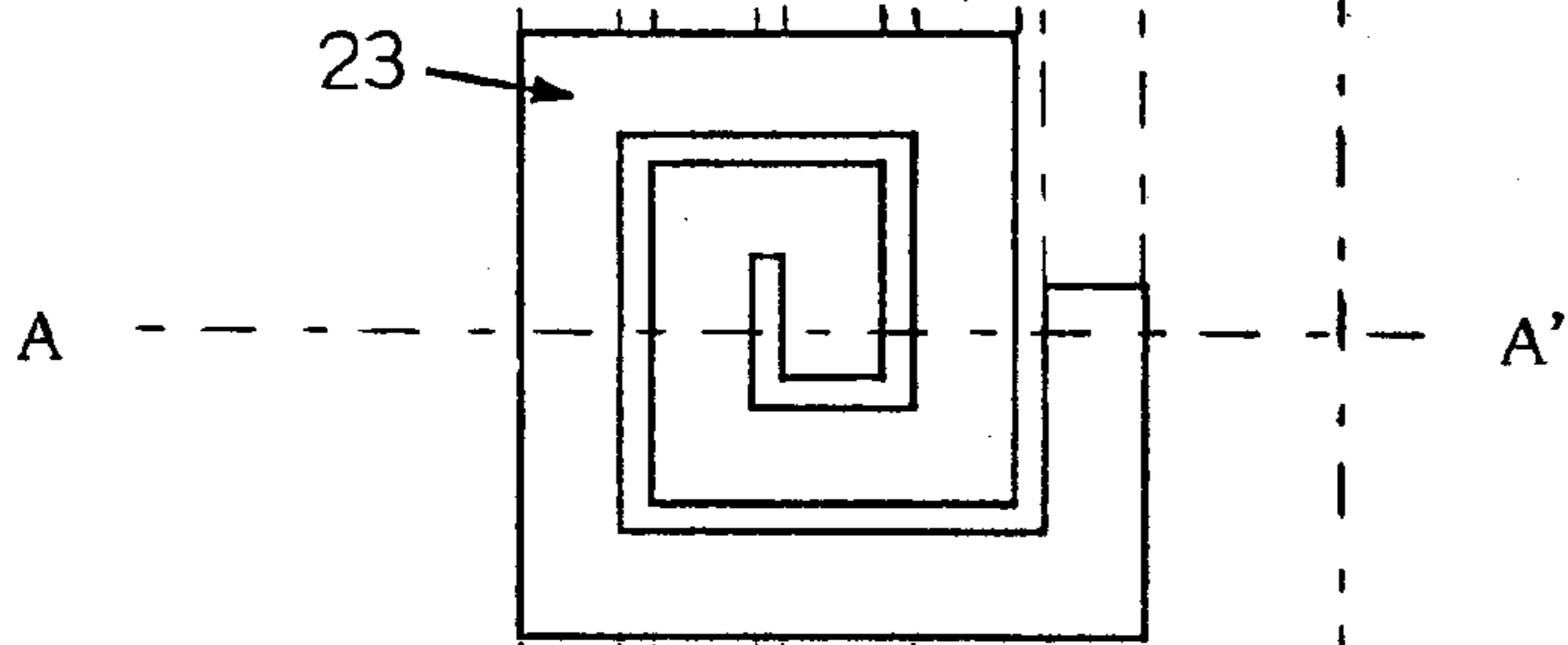
Fig. 2 (b) Top view of the second layer
