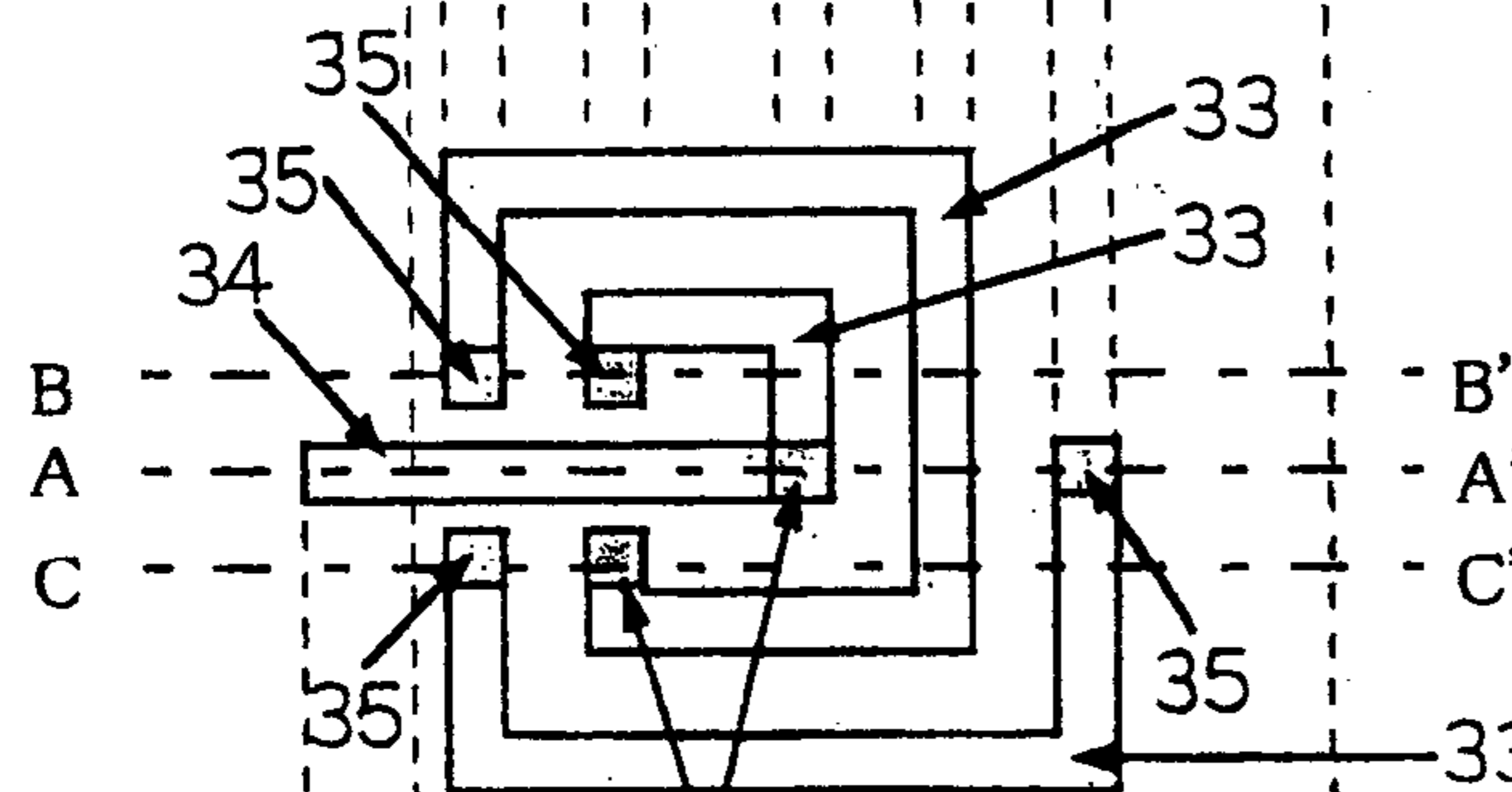
Fig. 3 (b) Top view of the second layer
