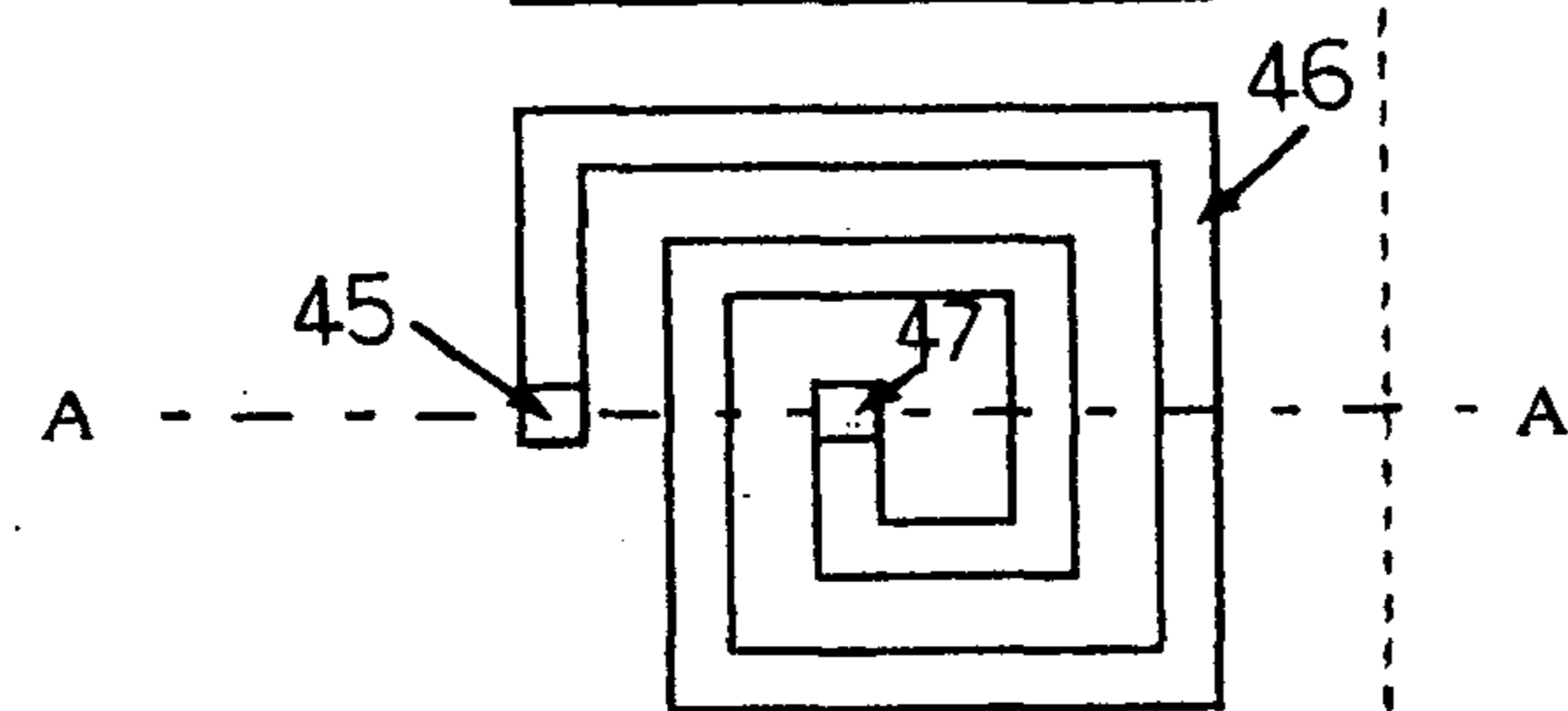
Fig. 4 (c) Top view of the third layer
