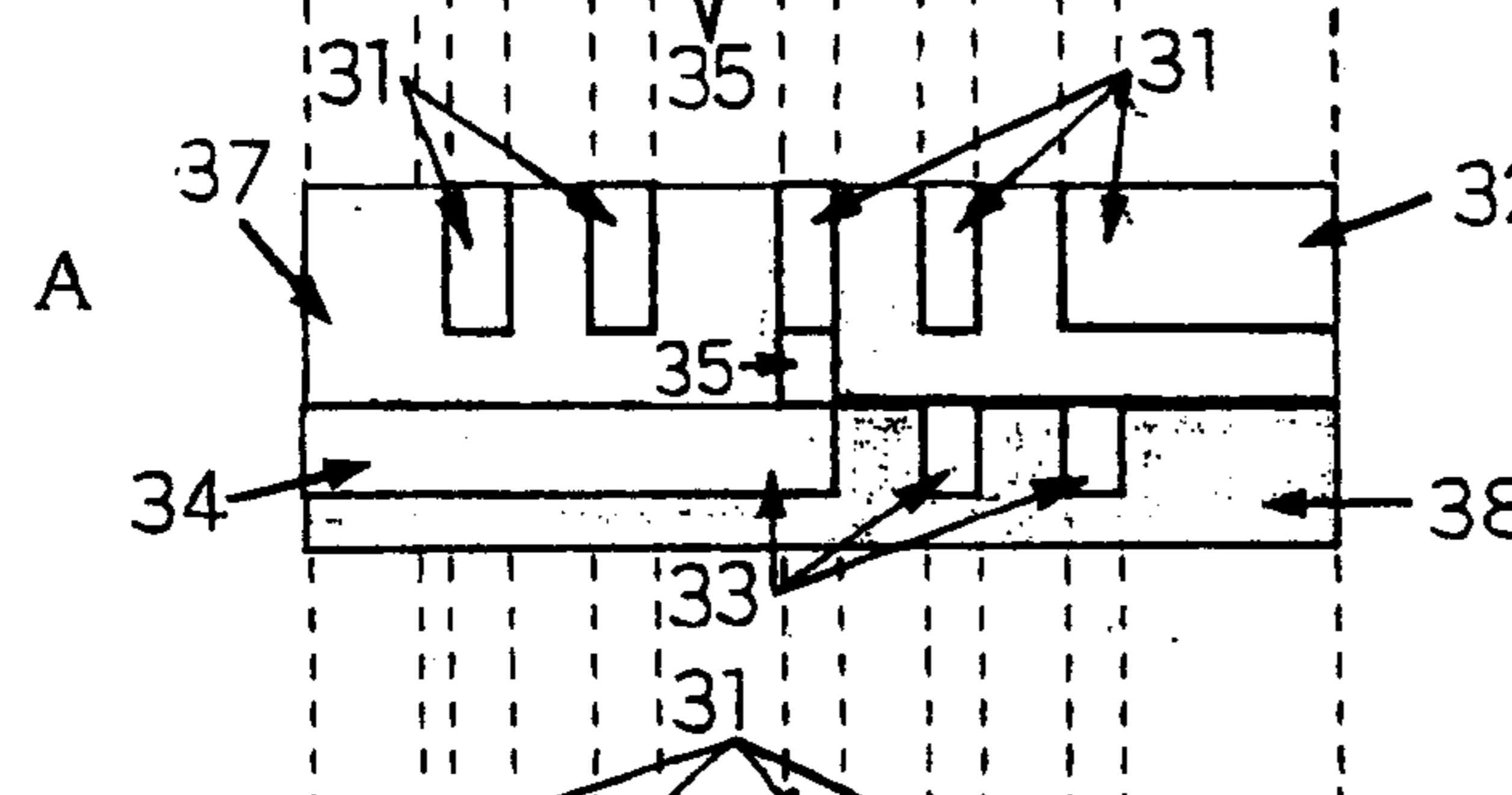
Fig. 3 (c) A-A' cross section
