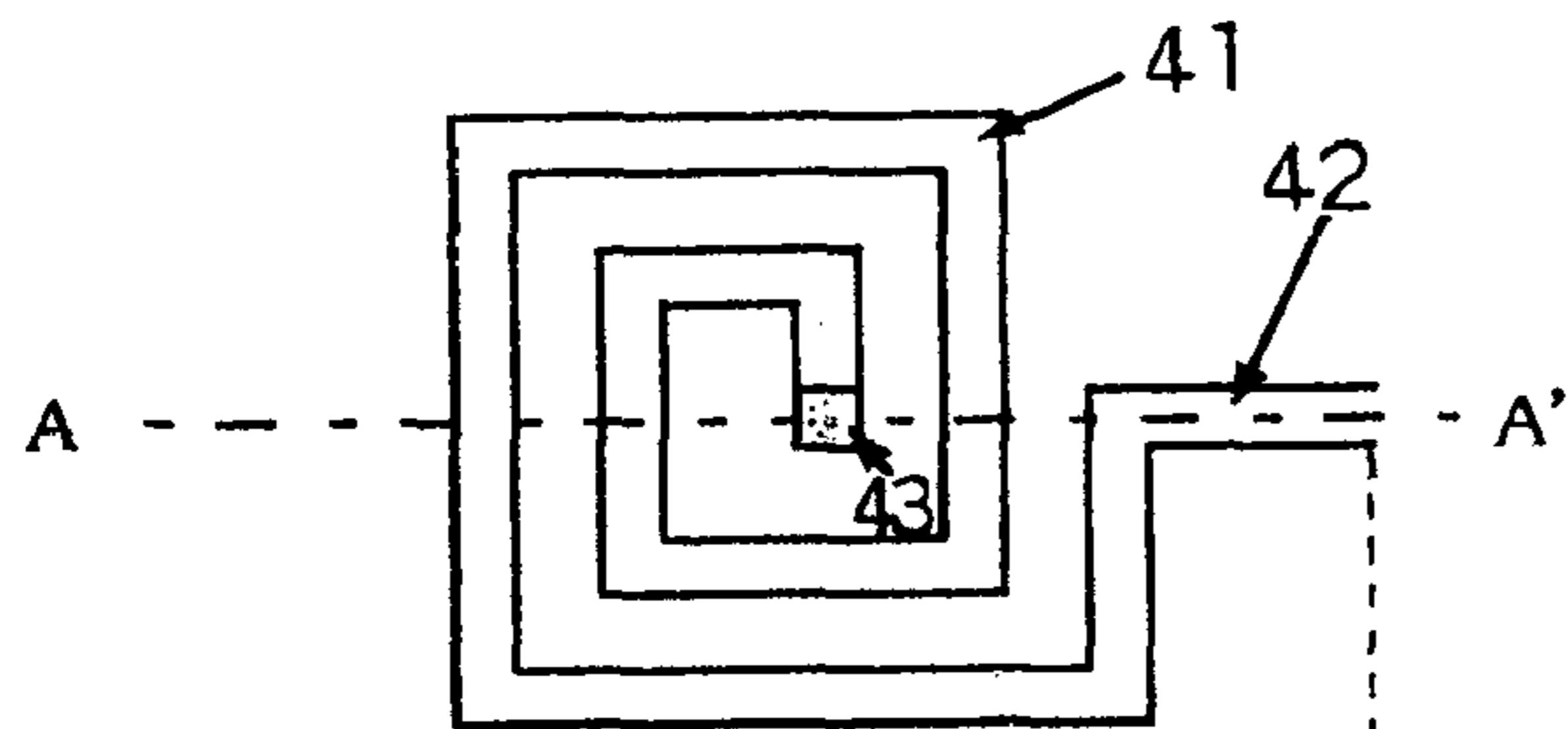
Fig. 4 (a) Top view of the first layer
