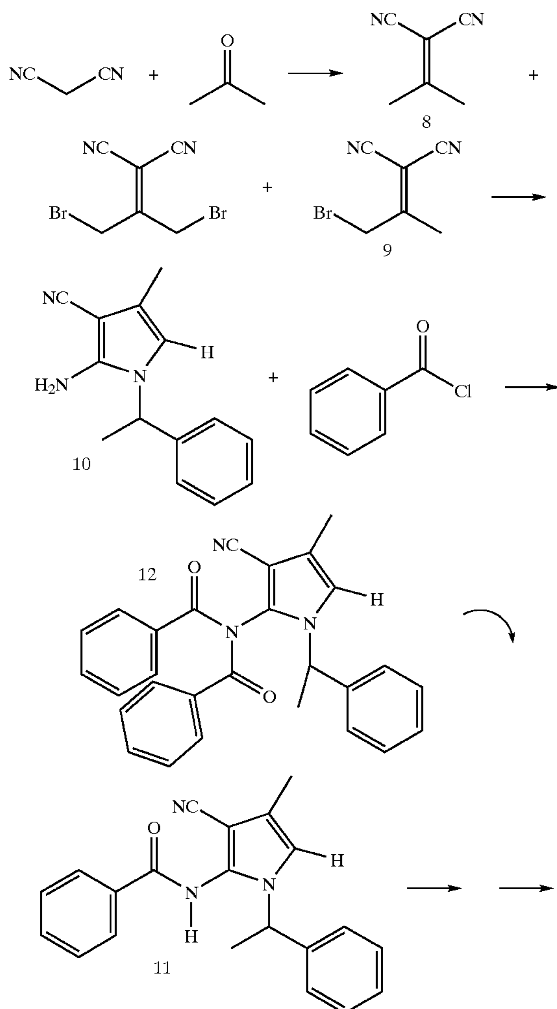
Scheme V
