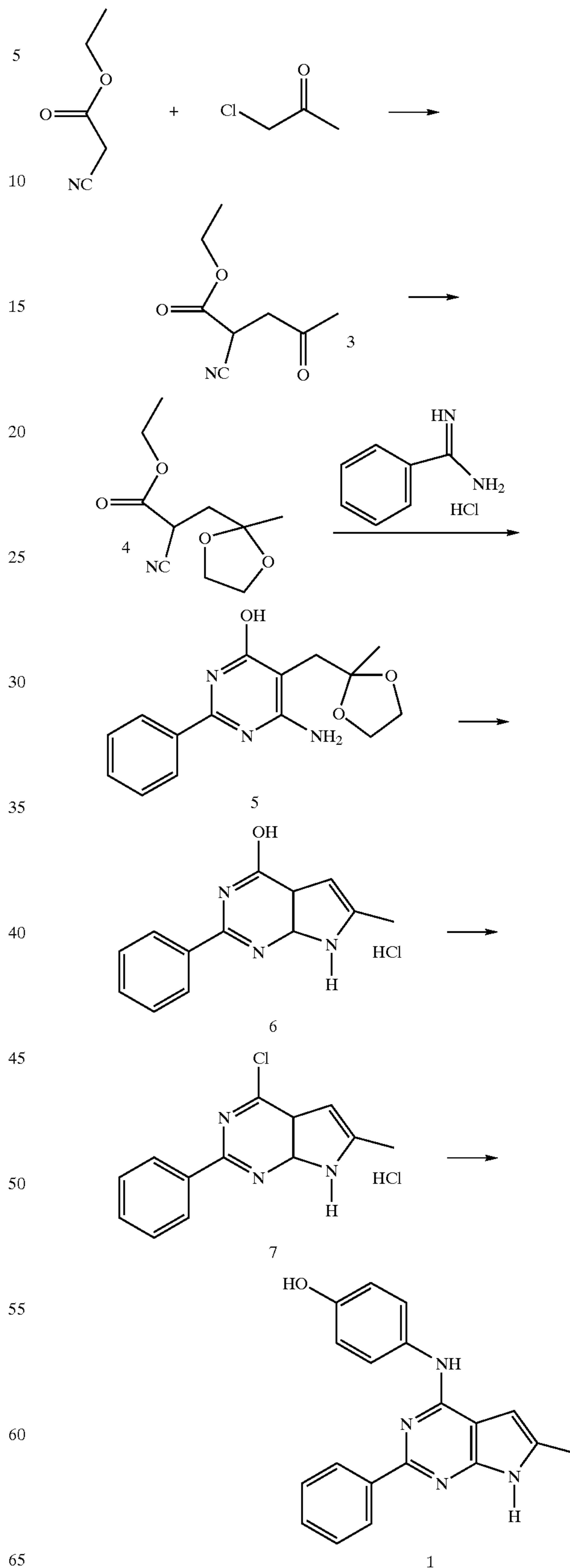
Scheme IV
