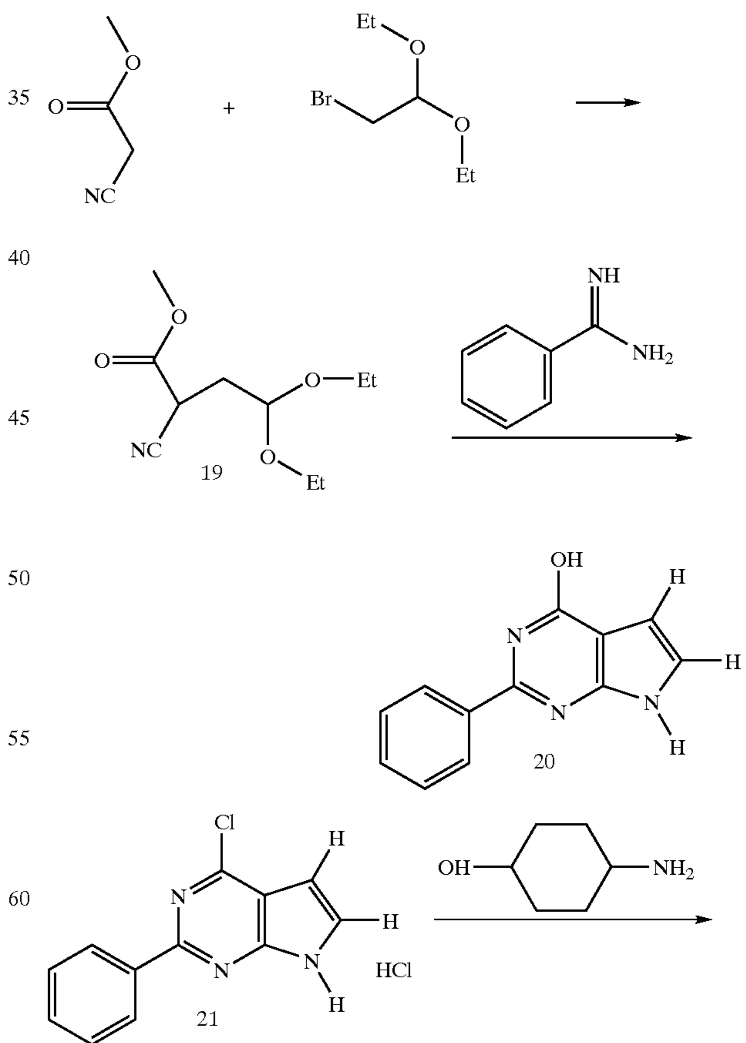
Scheme VIII
