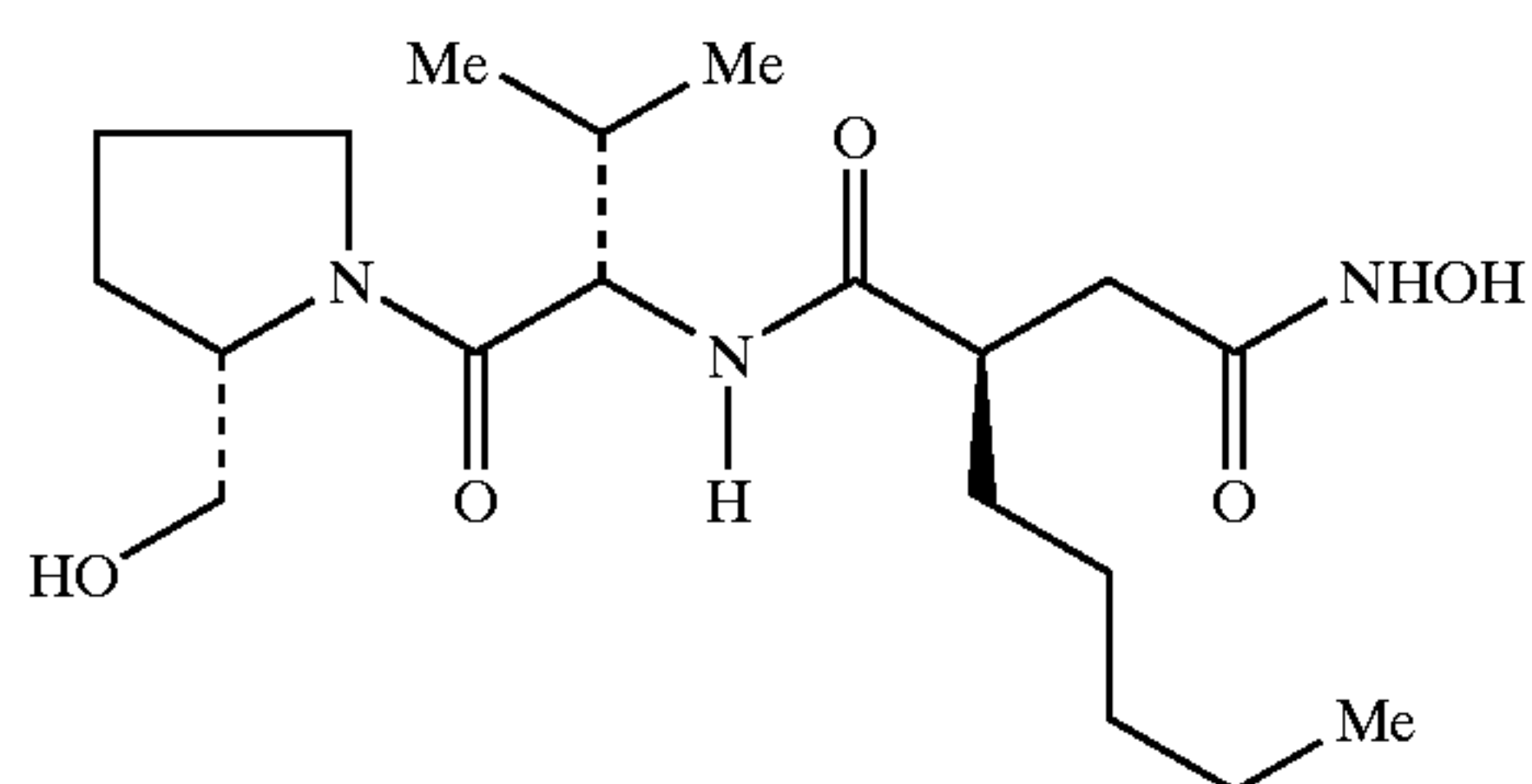
Actinonin
