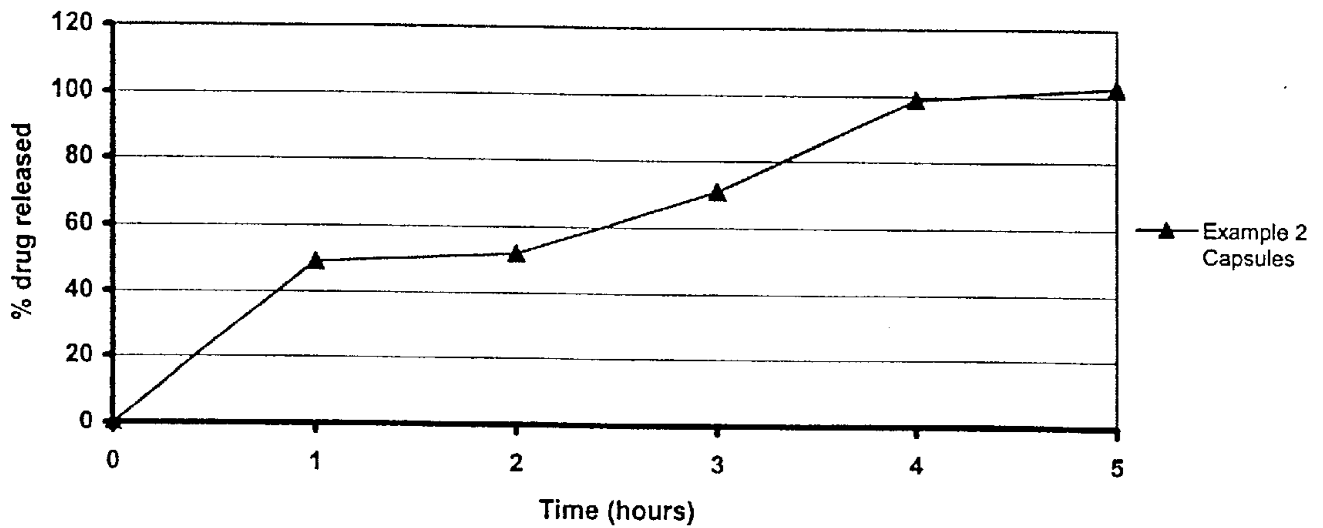
Drug Release Profile for Nizatidine CRR Capsules, 150 mg (75 mg IR + 75 mg TPR) of Example 2
