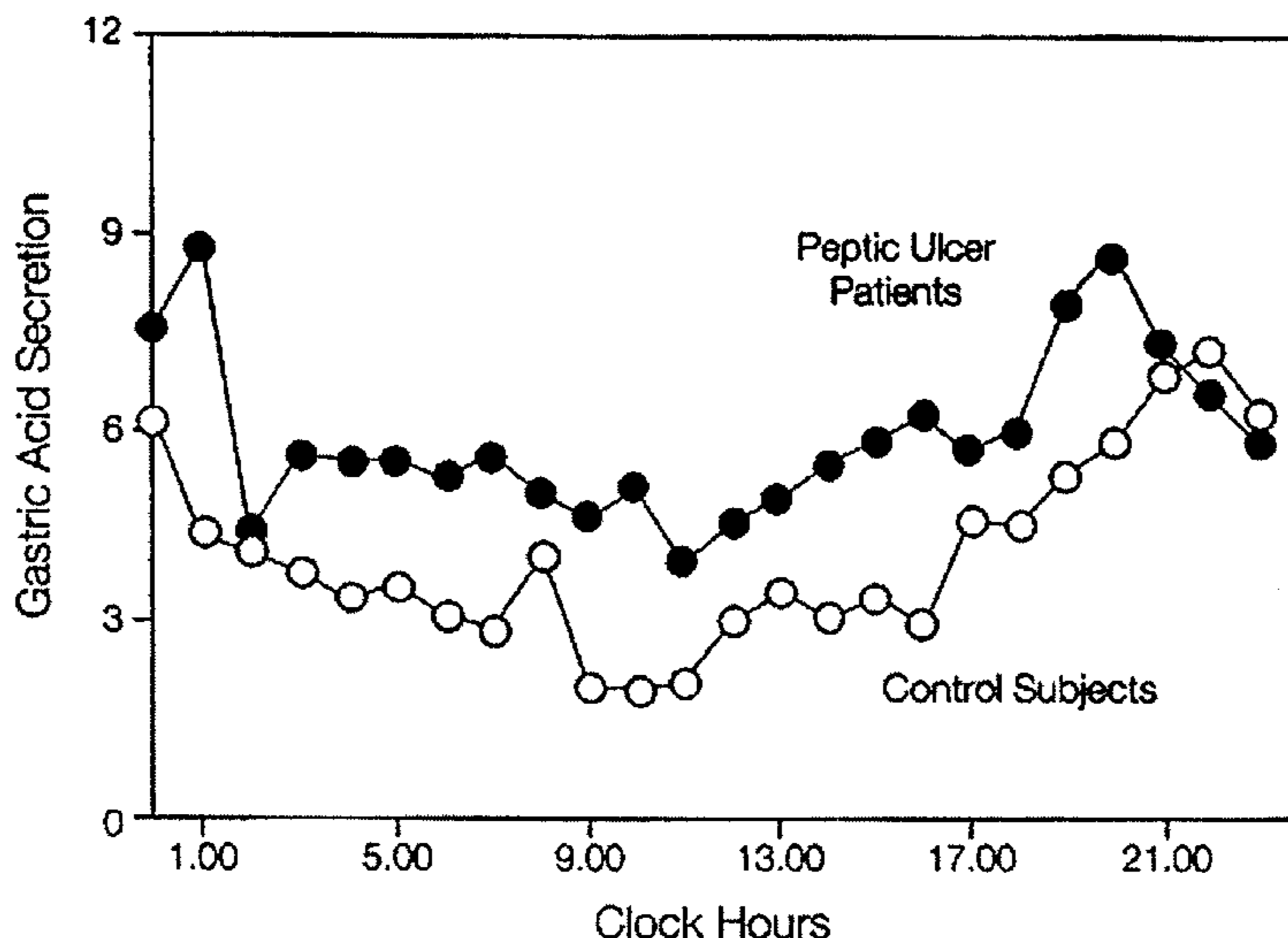
Circadian Variations in Gastric Acid Secretion
