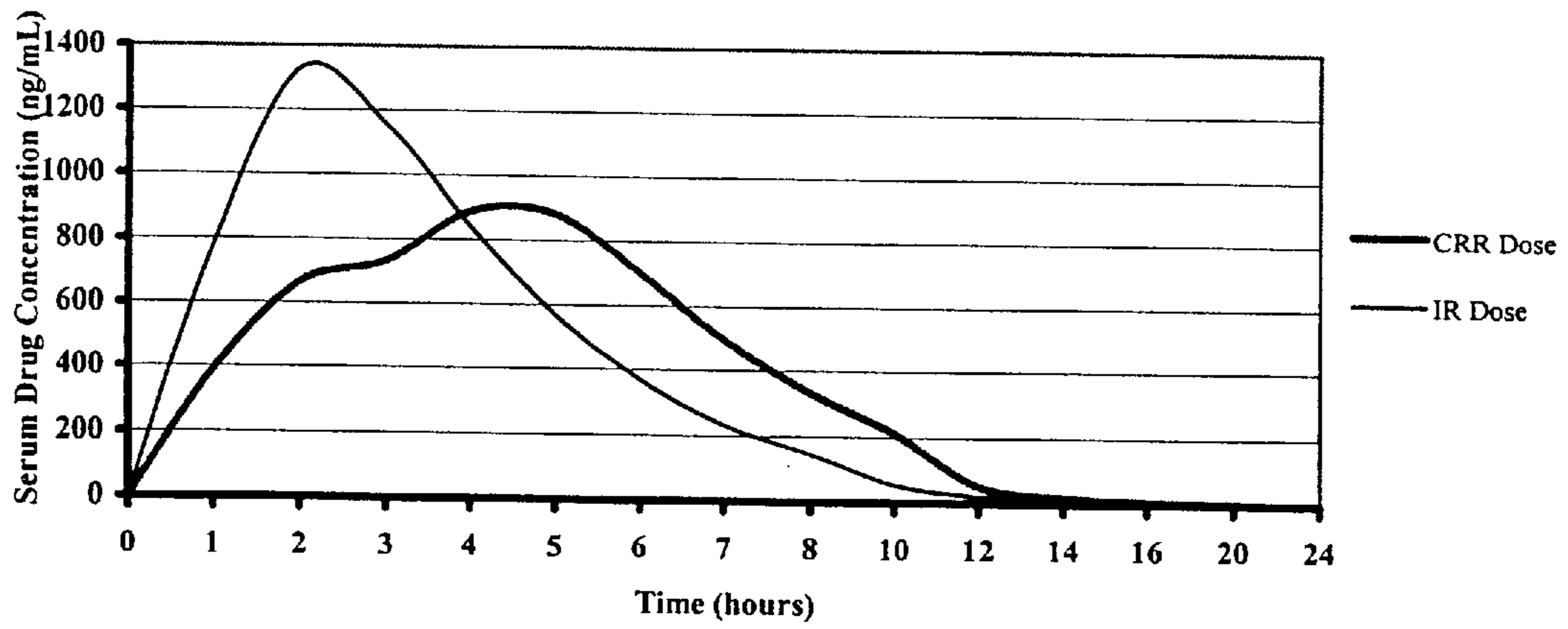
Simulated Serum Levels for Nizatidine 300 mg Night Time Dosing (IR Vs CRR)
