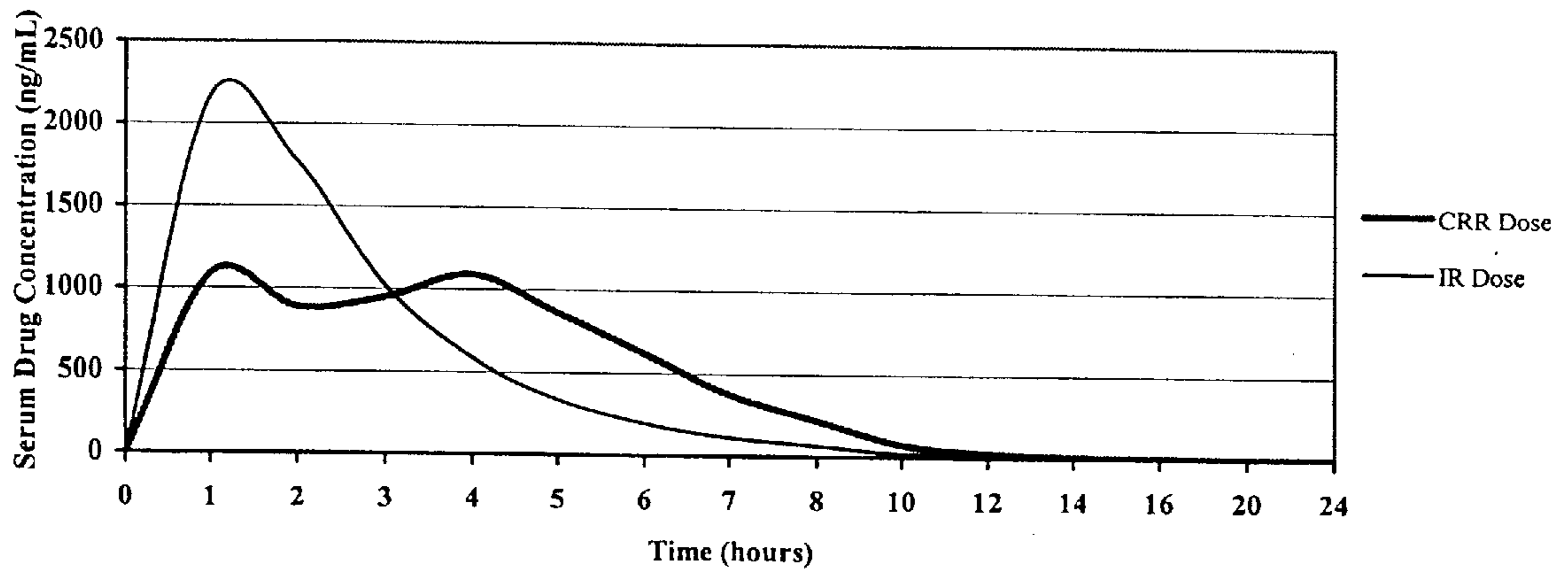
Simulated Serum Levels for Nizatidine 300 mg Day Time Dosing (IR Vs CRR)
