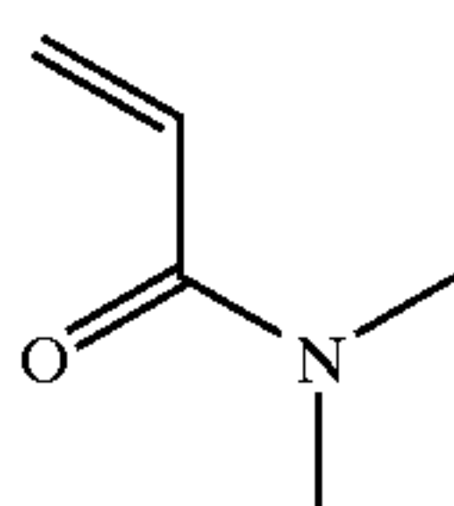
N,N-dimethylacrylamide (DMA)
