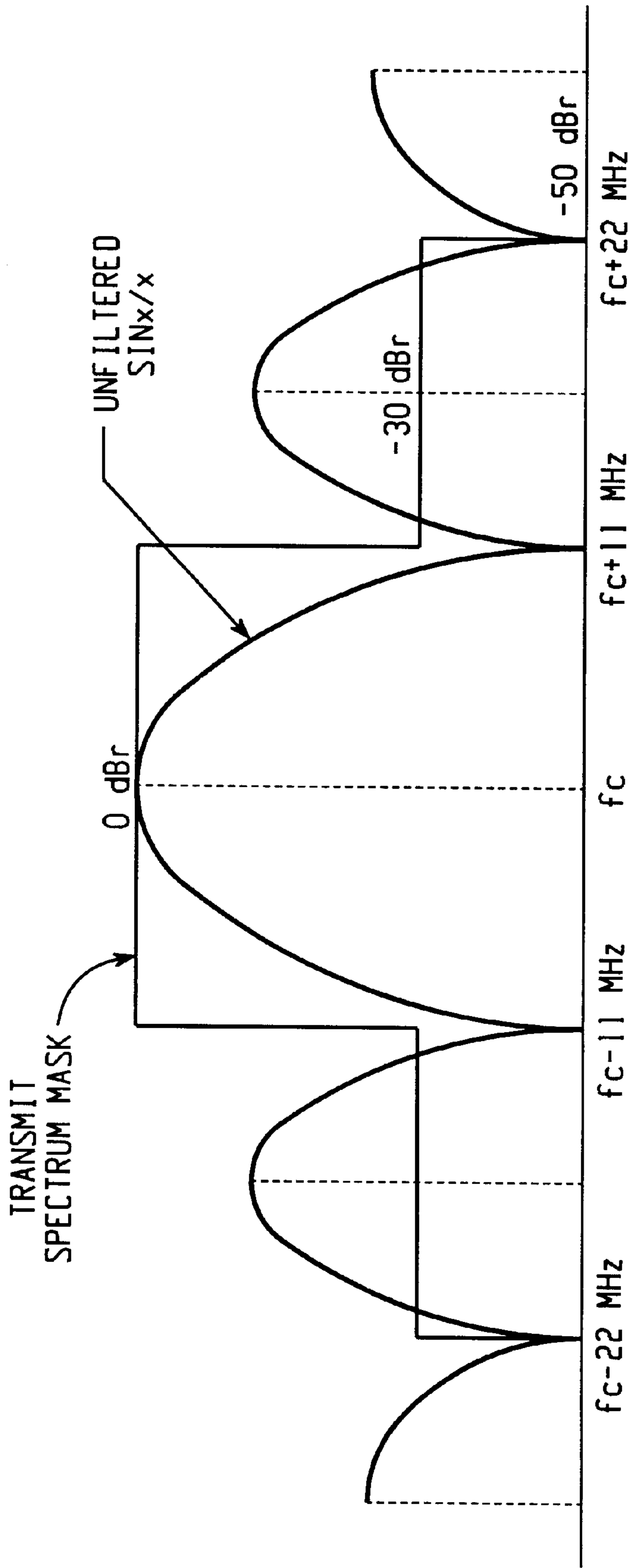
TRANSMIT SPECTRUM MASK
