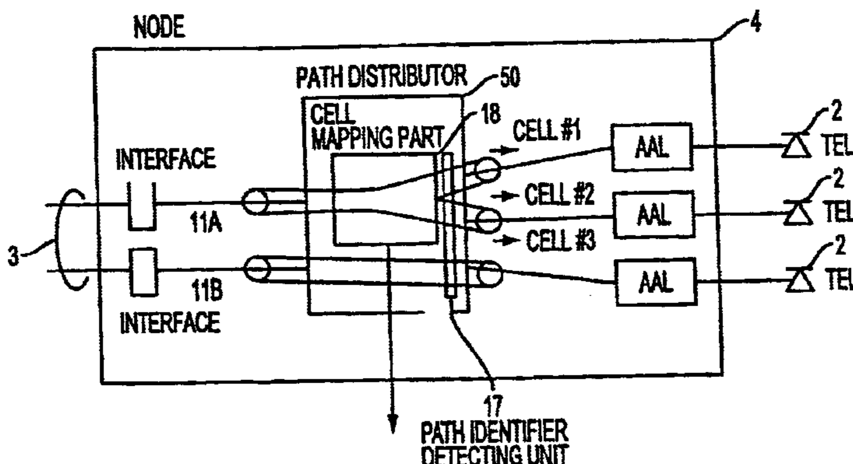
VIEW ILLUSTRATING OVERALL SYSTEM CONFIGURATION OF SECOND EMBODIMENT OF INVENTION
