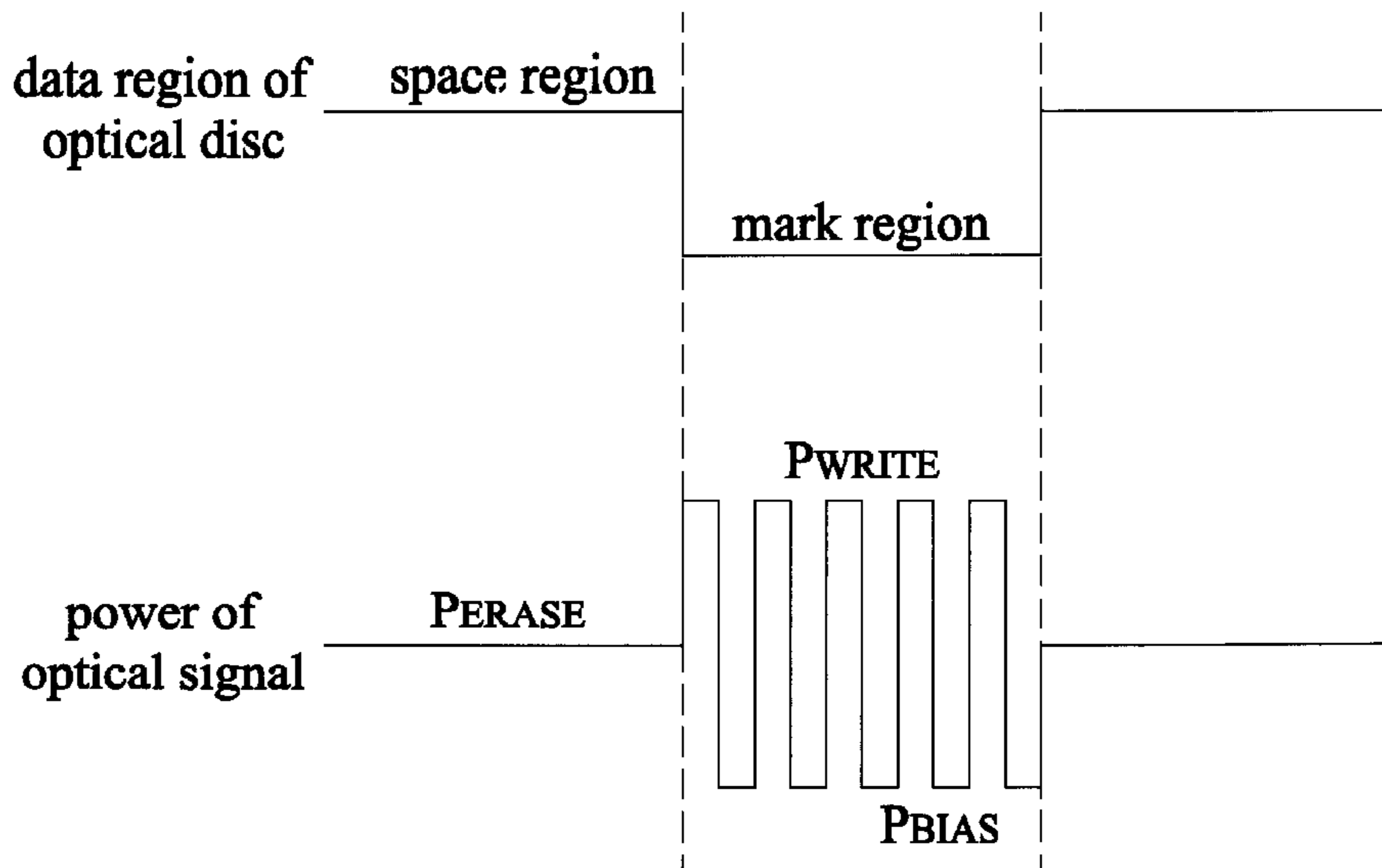
FIG. 1 (PRIOR ART)
