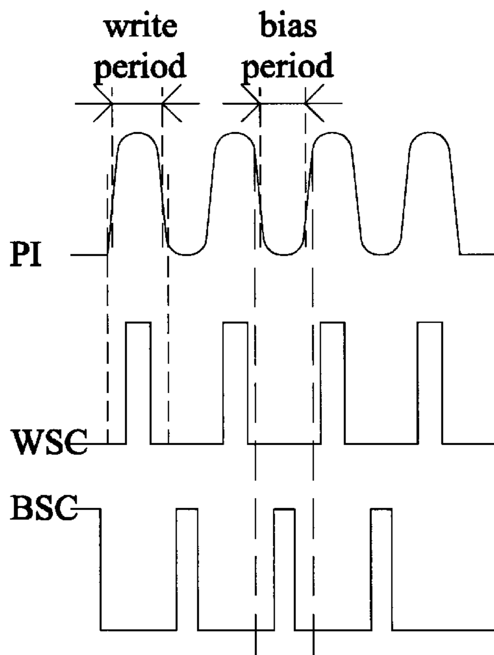
FIG. 4 (PRIOR ART)
