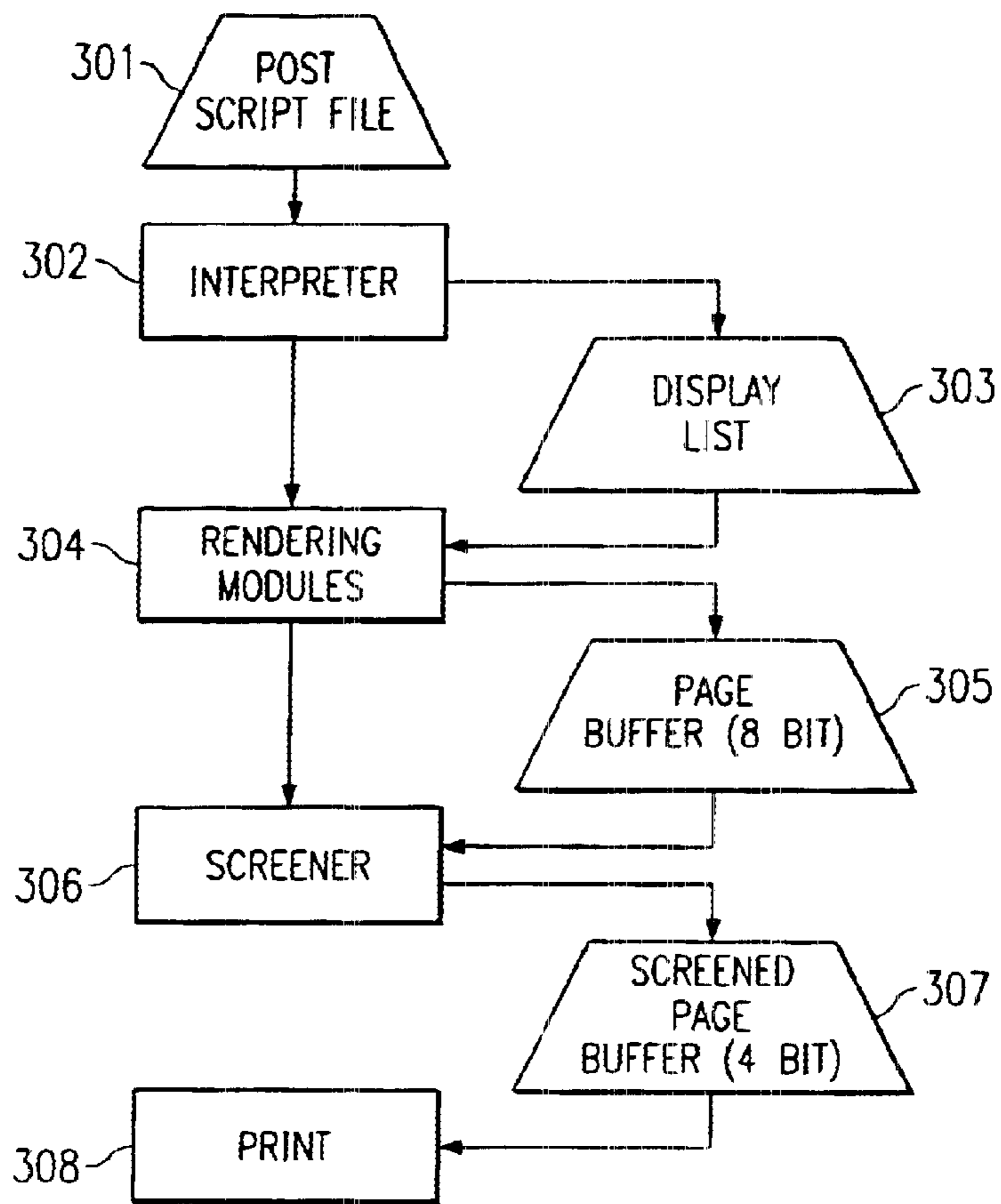
FIG. 8 (PRIOR ART)
