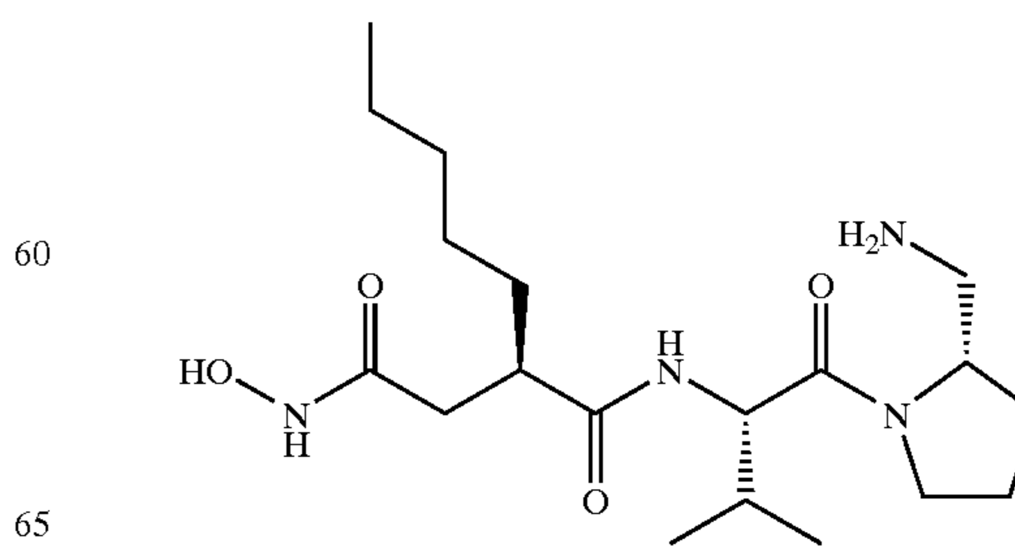
N4-hydroxy-N1-(1-(2-methylamine-pyrrolidine-1-carbonyl)-2-methyl-propyl)-2-pentyl-succinamide (53)
