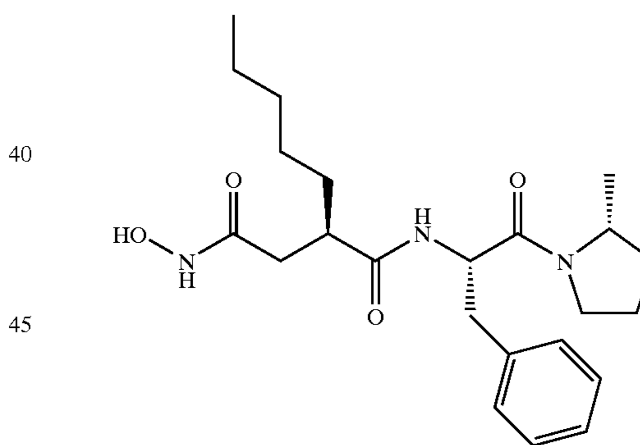
N4-hydroxy-N1-(1-benzyl-2-(2-methyl-pyrrolidin-1-yl)-2-oxo-ethyl)-2-pentyl-succinamide (52)
