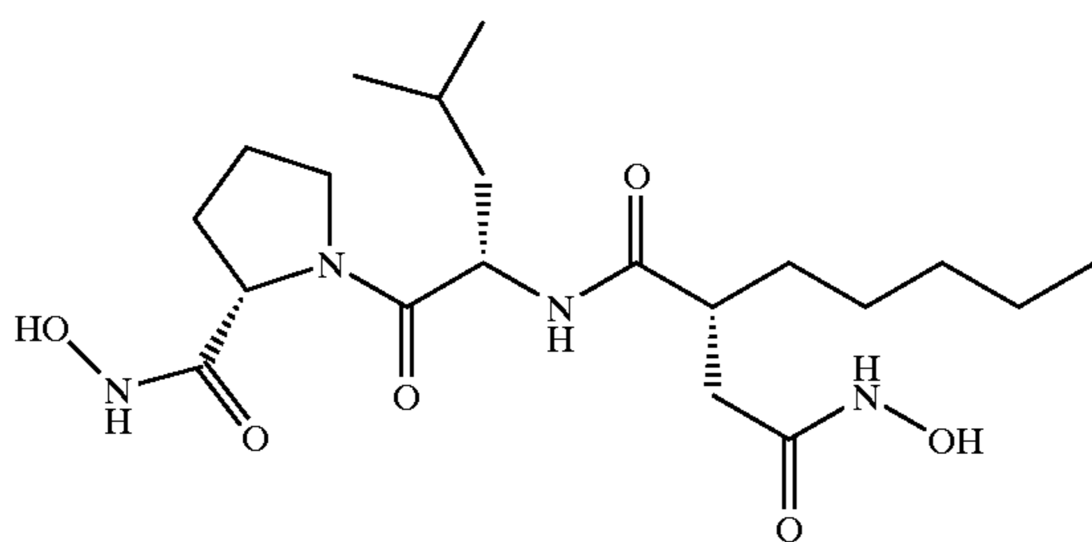
N4-hydroxy-N1-(1-(2-hydroxycarbamoyl-pyrrolidine-1-carbonyl)-3-methyl-butyl)-2-pentyl succinamide (47)
