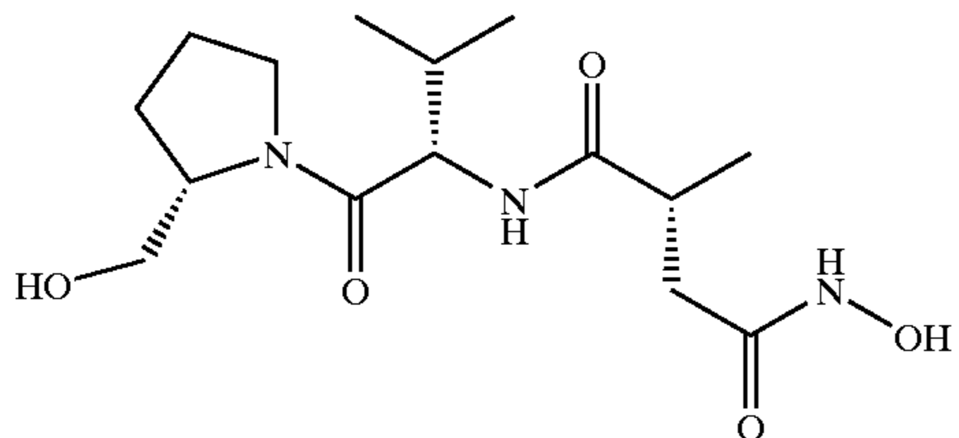
N4-hydroxy-N1-(1-(2-hydroxymethyl-pyrrolidine-1-carbonyl)-2-methyl-propyl)-2-methyl-succinamide (48)
