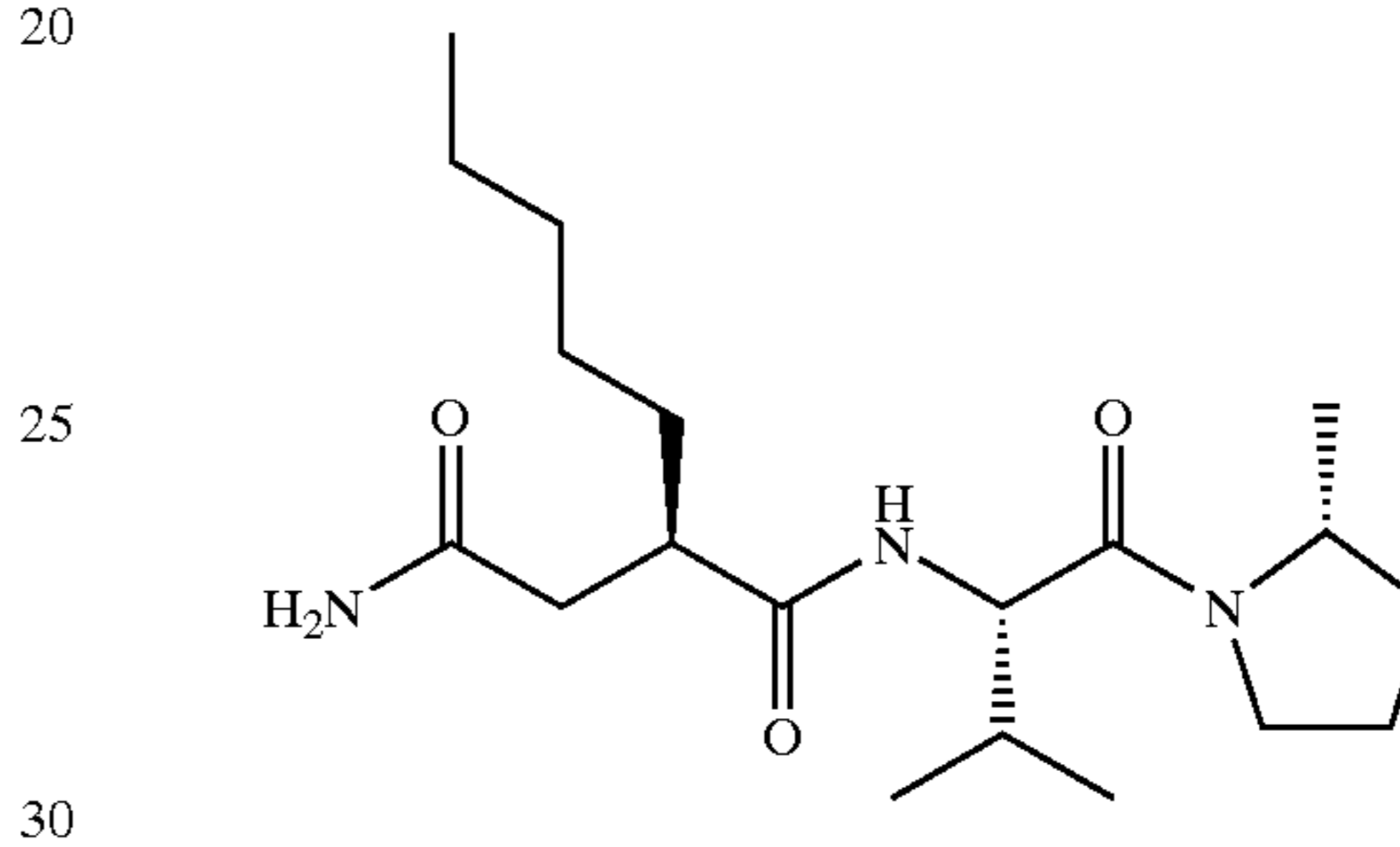
N1-(1-(2-methyl-pyrrolidine-1-carbonyl)-2-methyl-propyl)-2-pentyl-succinamide (51)
