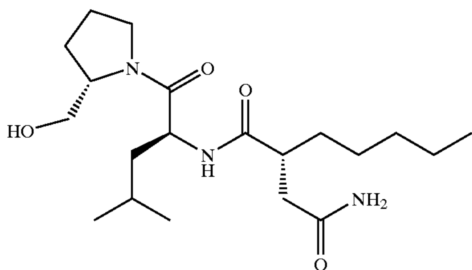
N1-(1-(2-hydroxymethyl-pyrrolidine-1-carbonyl)-3-methyl-butyl)-2-pentyl-succinamide (49)
