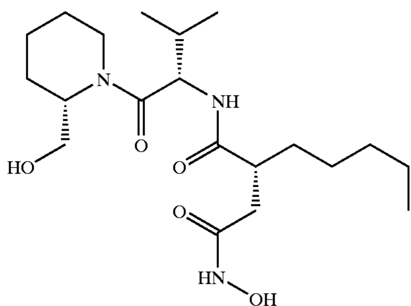
N4-hydroxy-N1-(1-(2-hydroxymethyl-piperidine-1-carbonyl)-2-methyl-propyl)-2-pentyl-succinamide (46)
