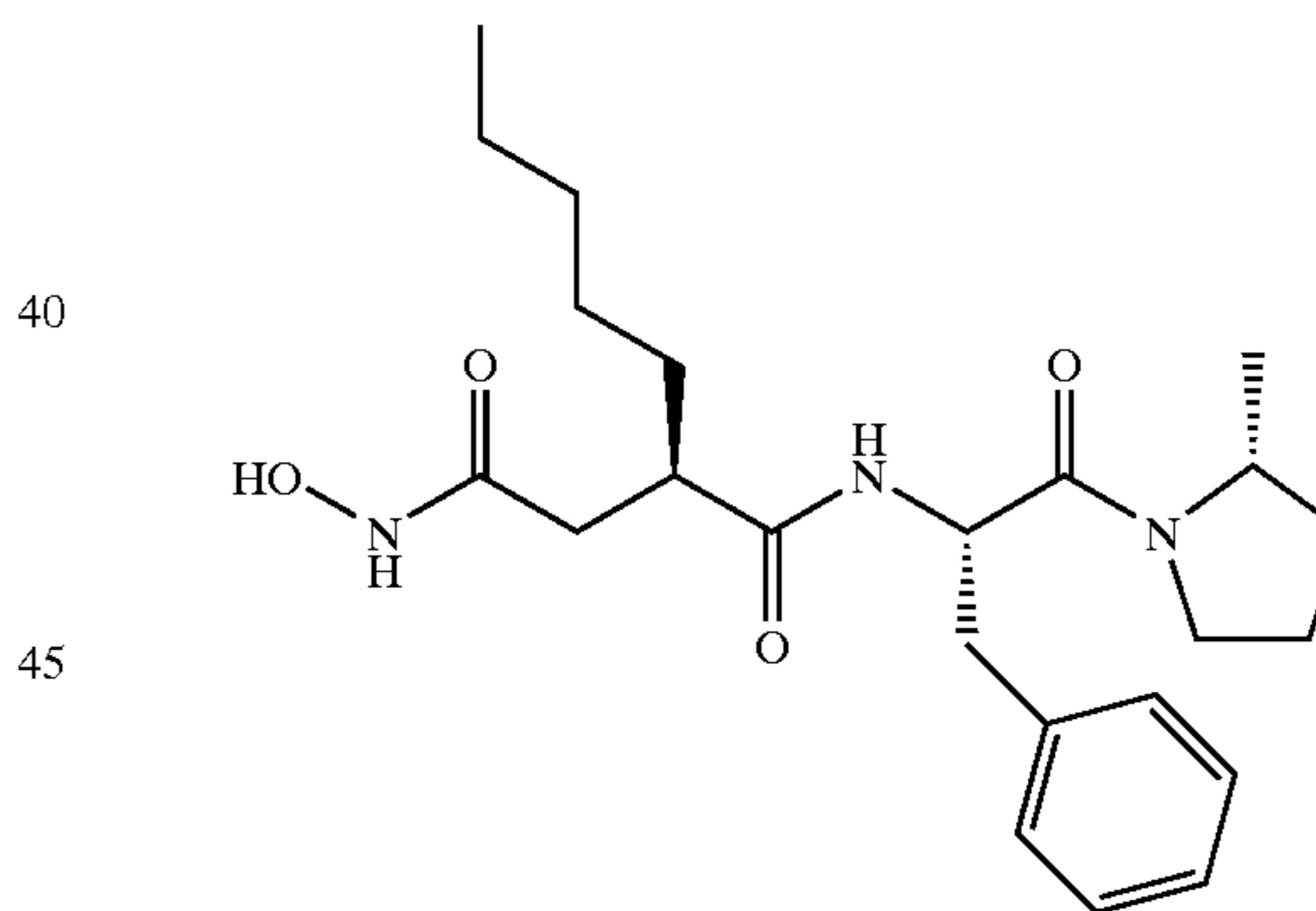
N4-hydroxy-N1-(1-benzyl-2-(2-methyl-pyrrolidin-1-yl)-2-oxo-ethyl)-2-pentyl-succinamide (52)
