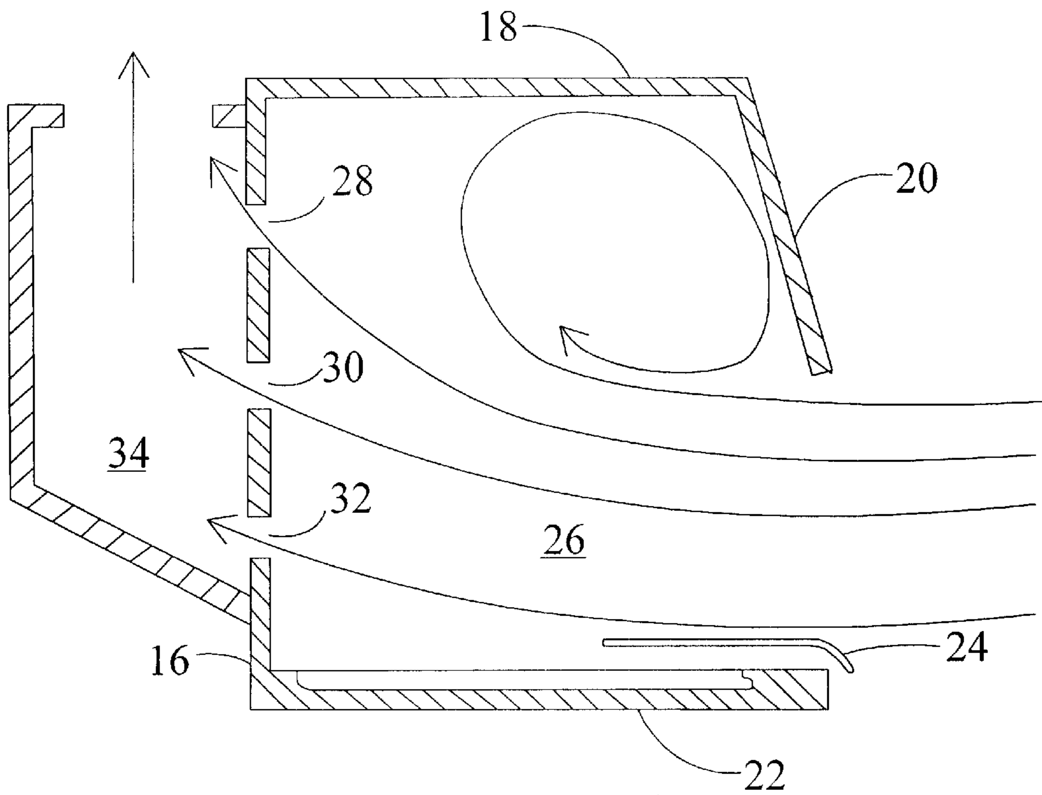
FIG. 2 (Prior Art)
