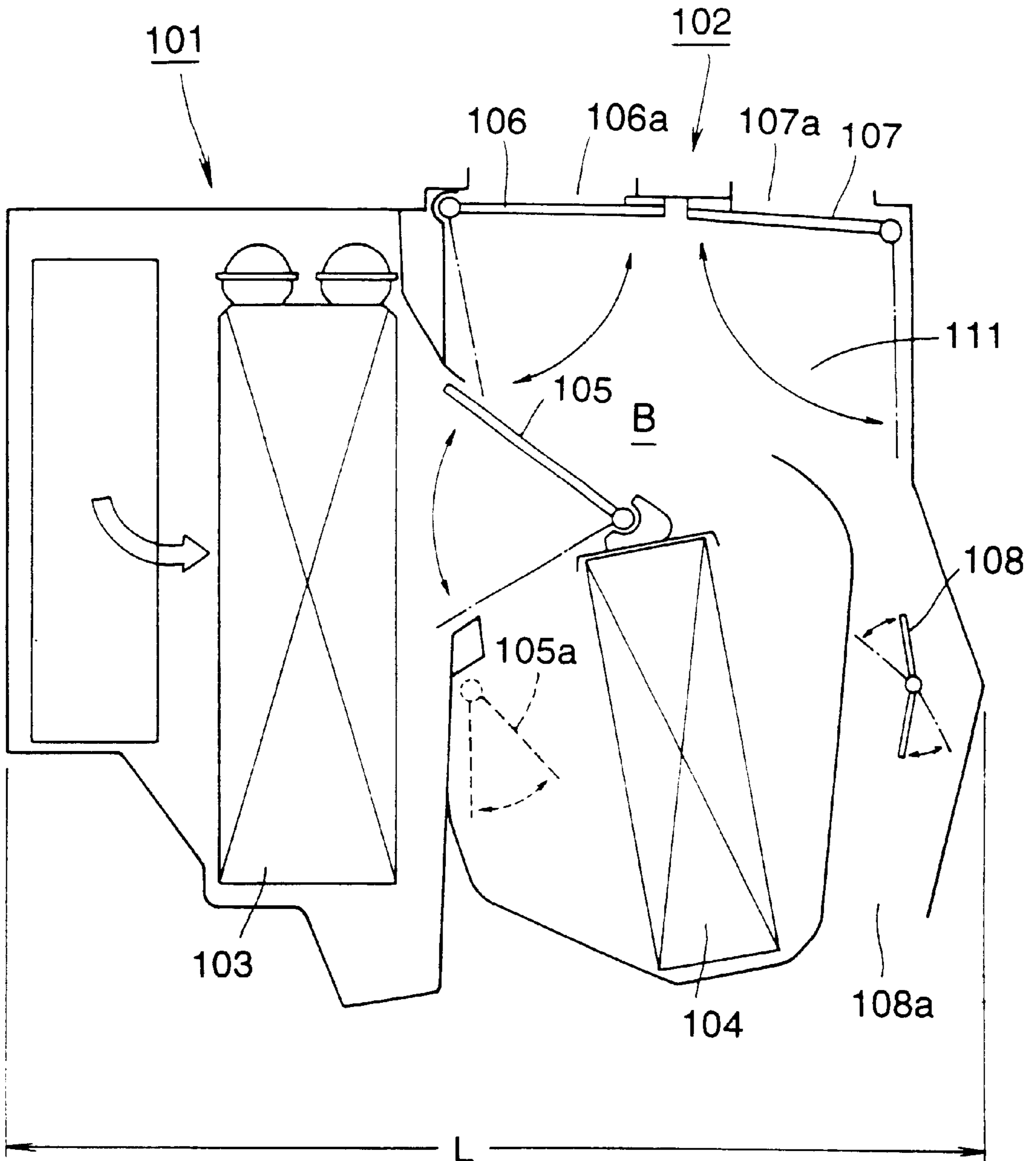
(PRIOR ART) FIG. 16
