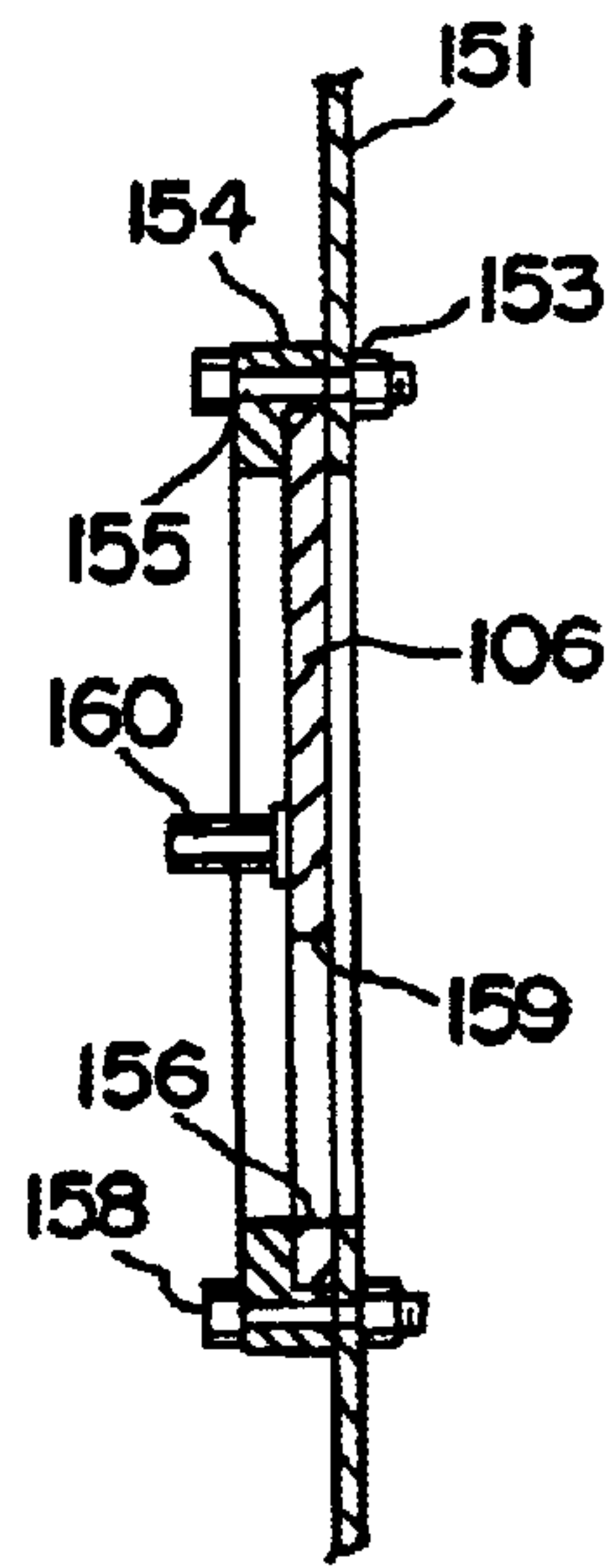
FIG. 11 PRIOR ART
