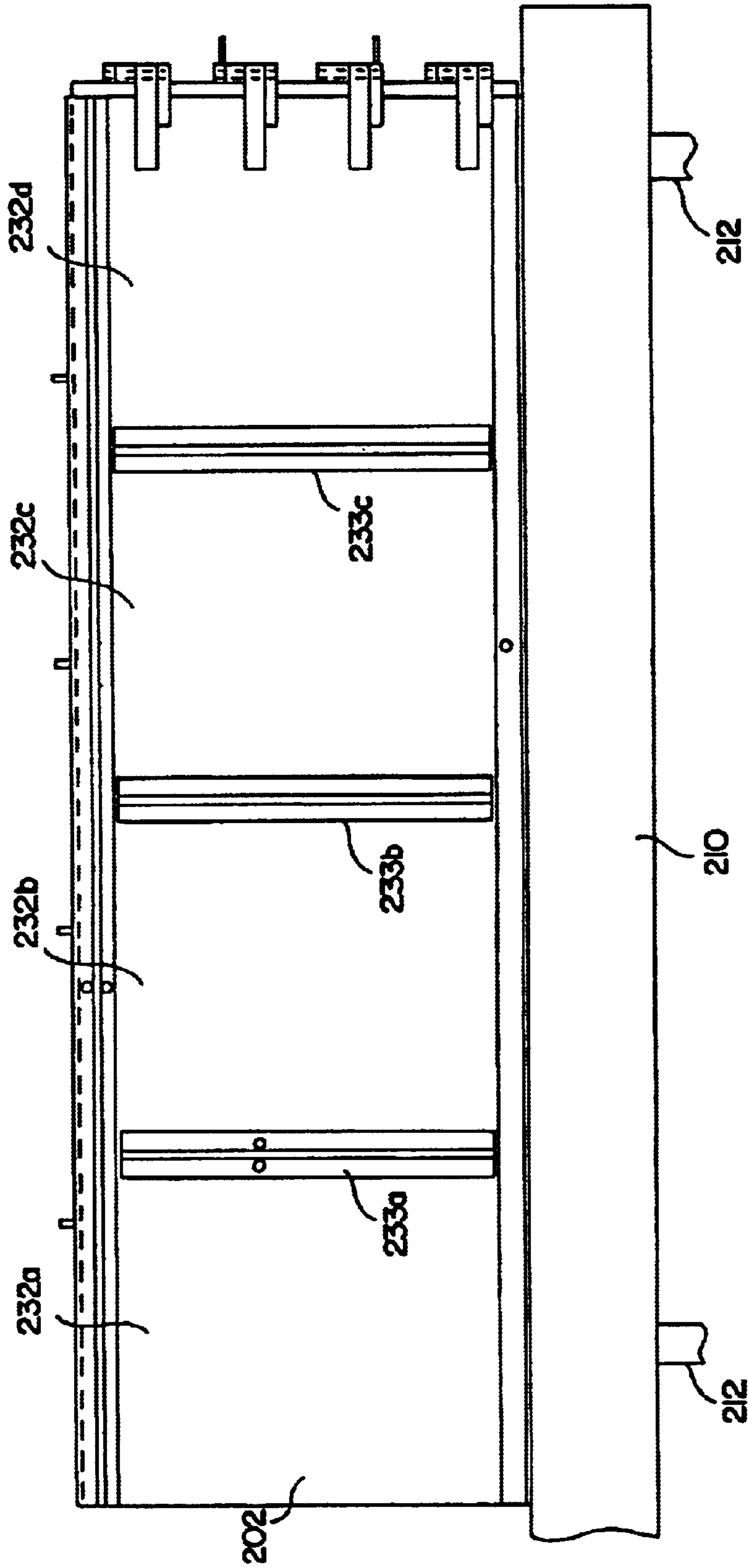
FIG. 22 PRIOR ART
