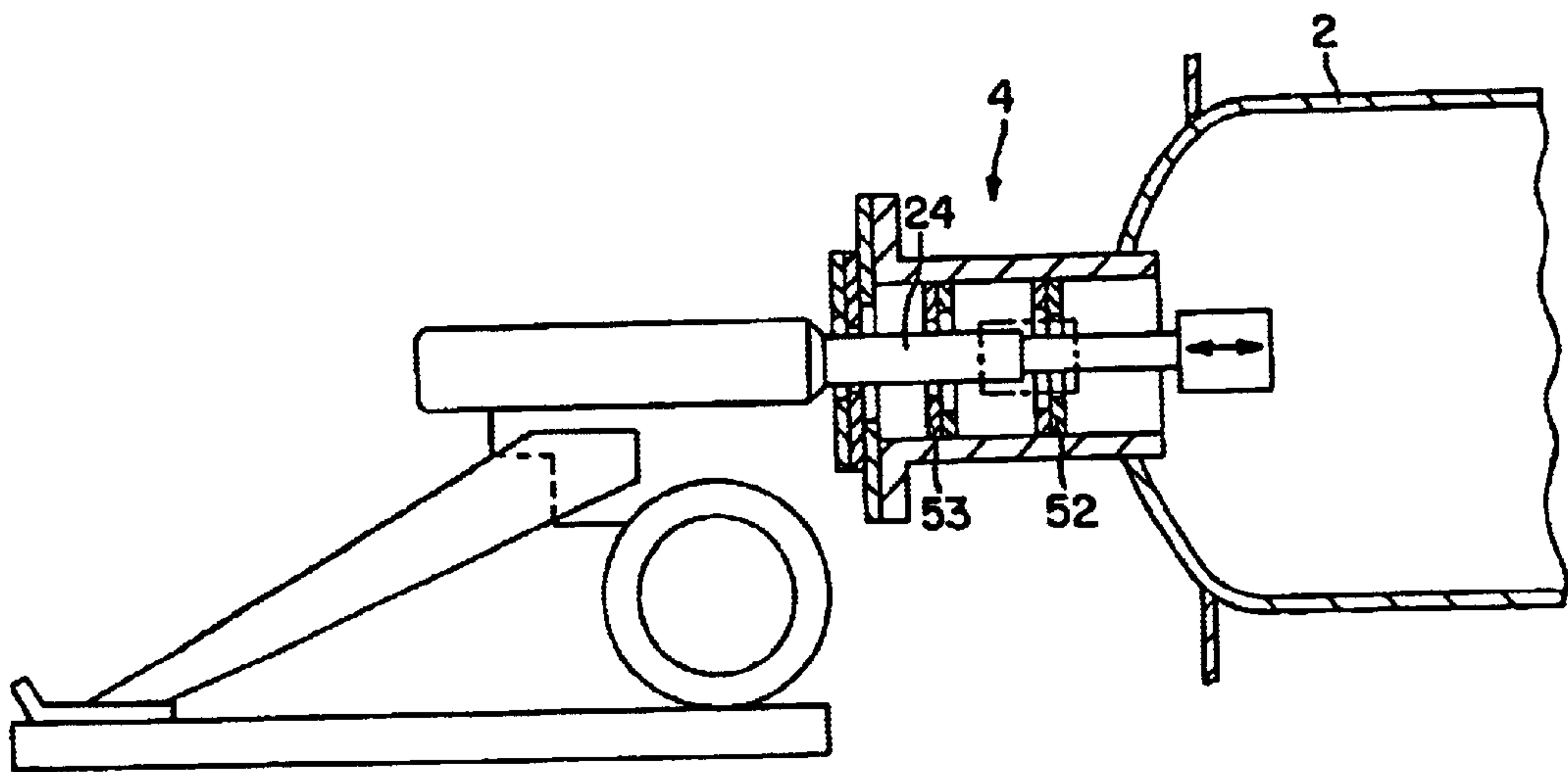
FIG. 5 PRIOR ART
