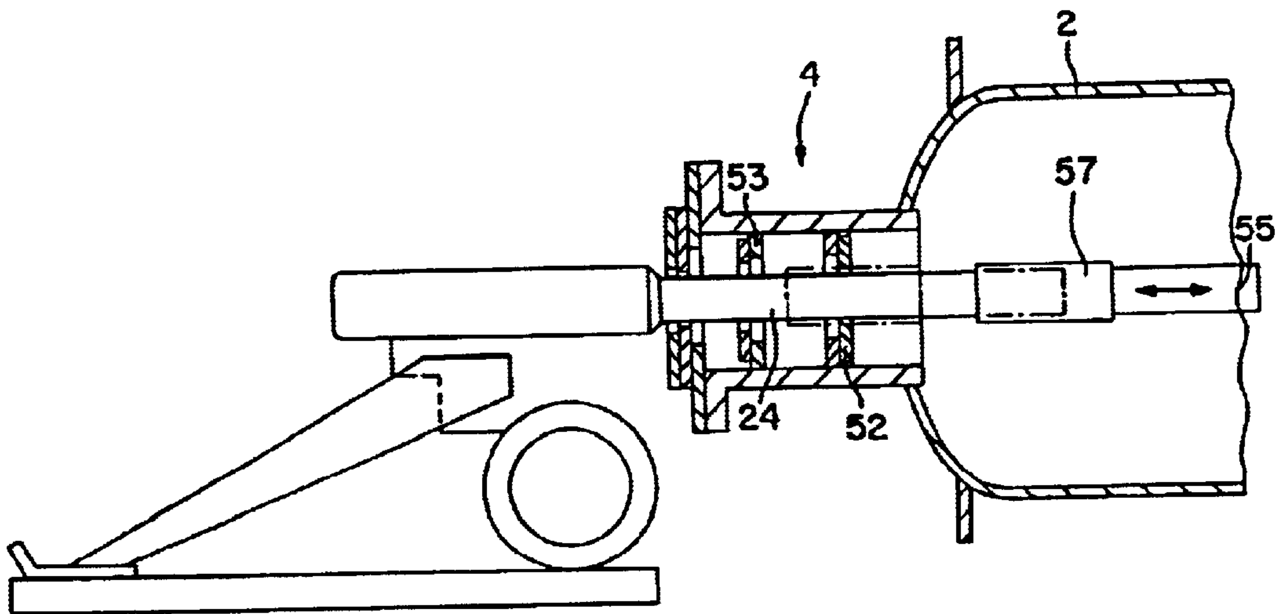
FIG. 6 PRIOR ART
