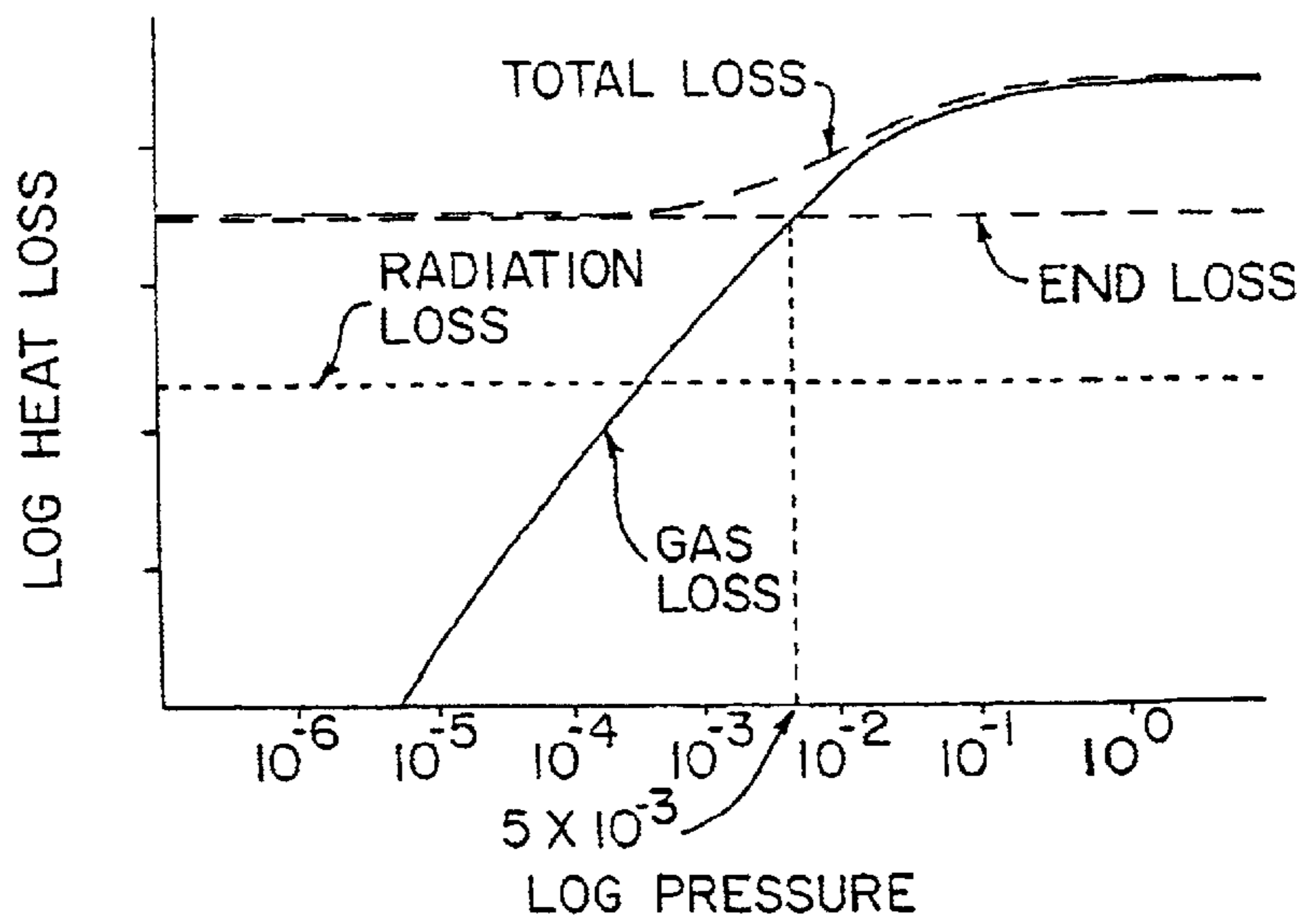
FIG. 2 PRIOR ART
