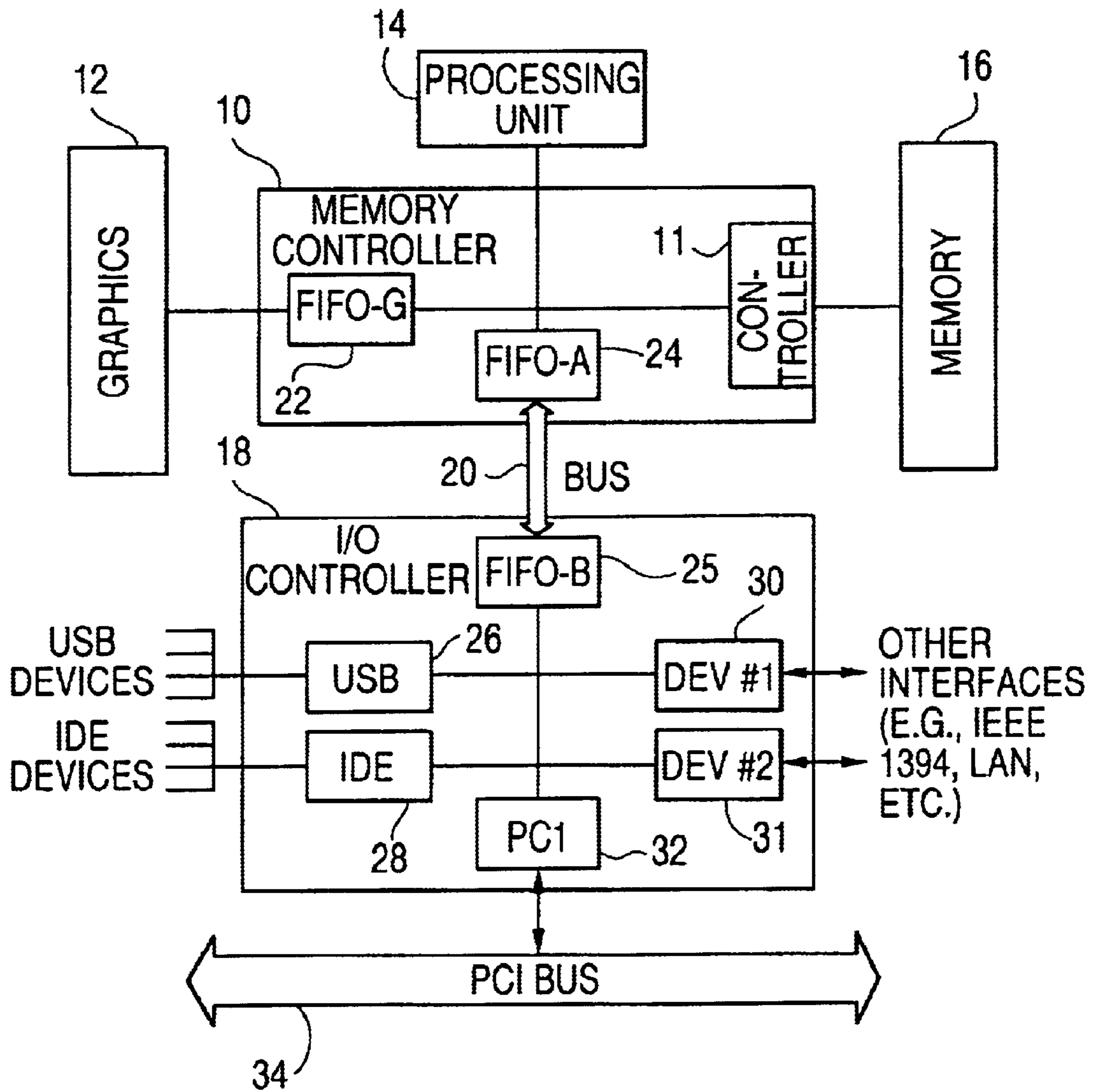
FIG. 1 (PRIOR ART)
