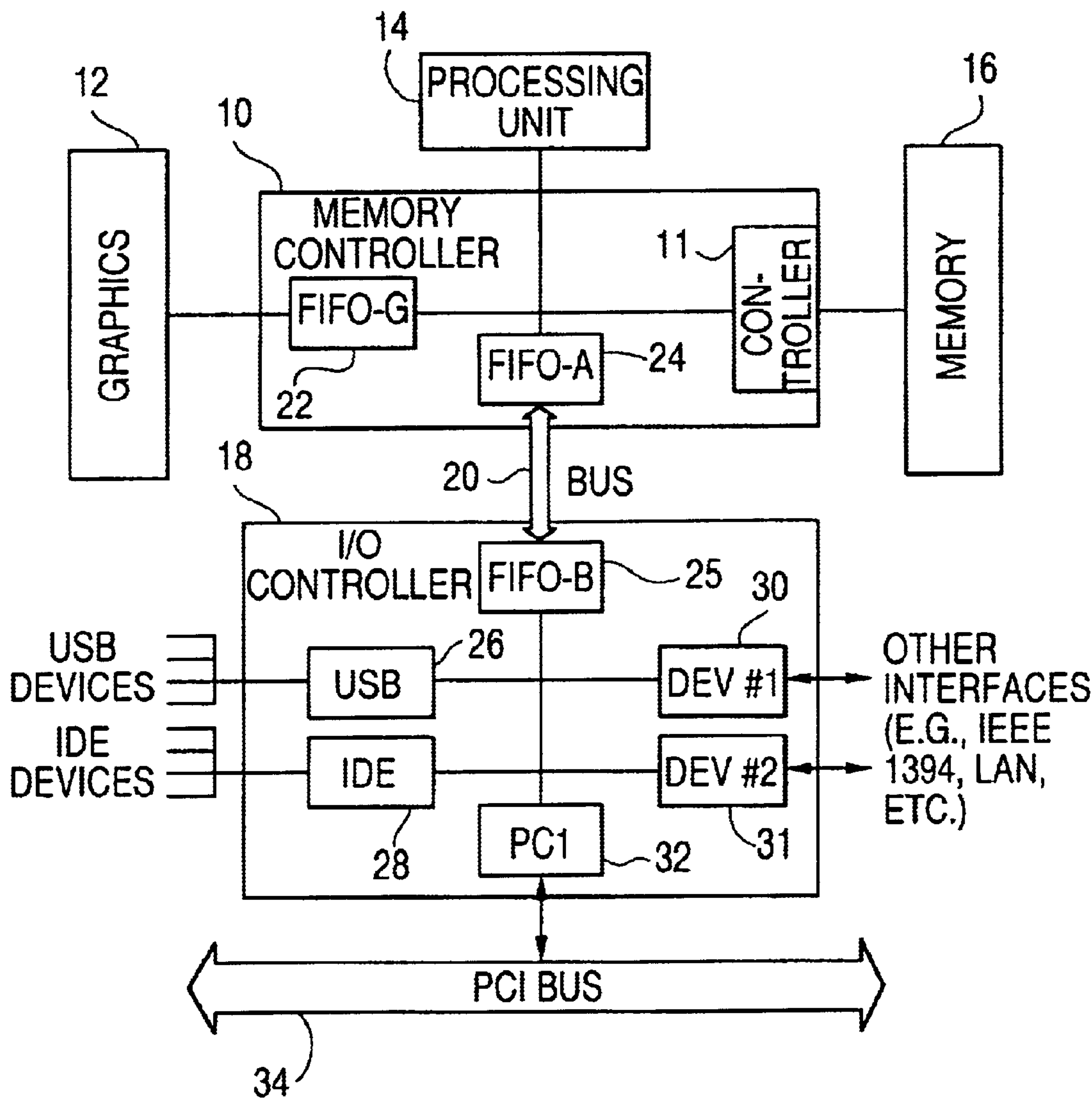
FIG. 1 (PRIOR ART)
