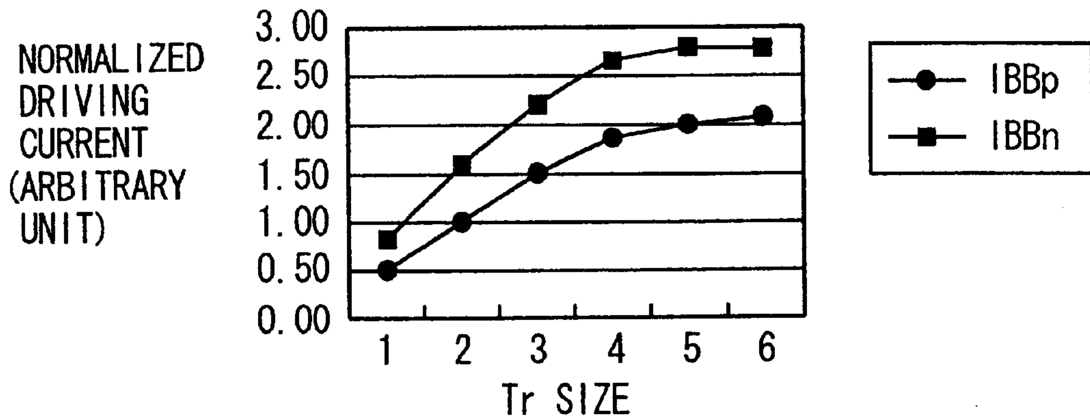
( G_{wp}/G_{wn} = 30/40, 75/100, 150/200, 300/400, 450/600, 600/800 ) Tr SIZE DEPENDENCY OF DRIVING CURRENT
