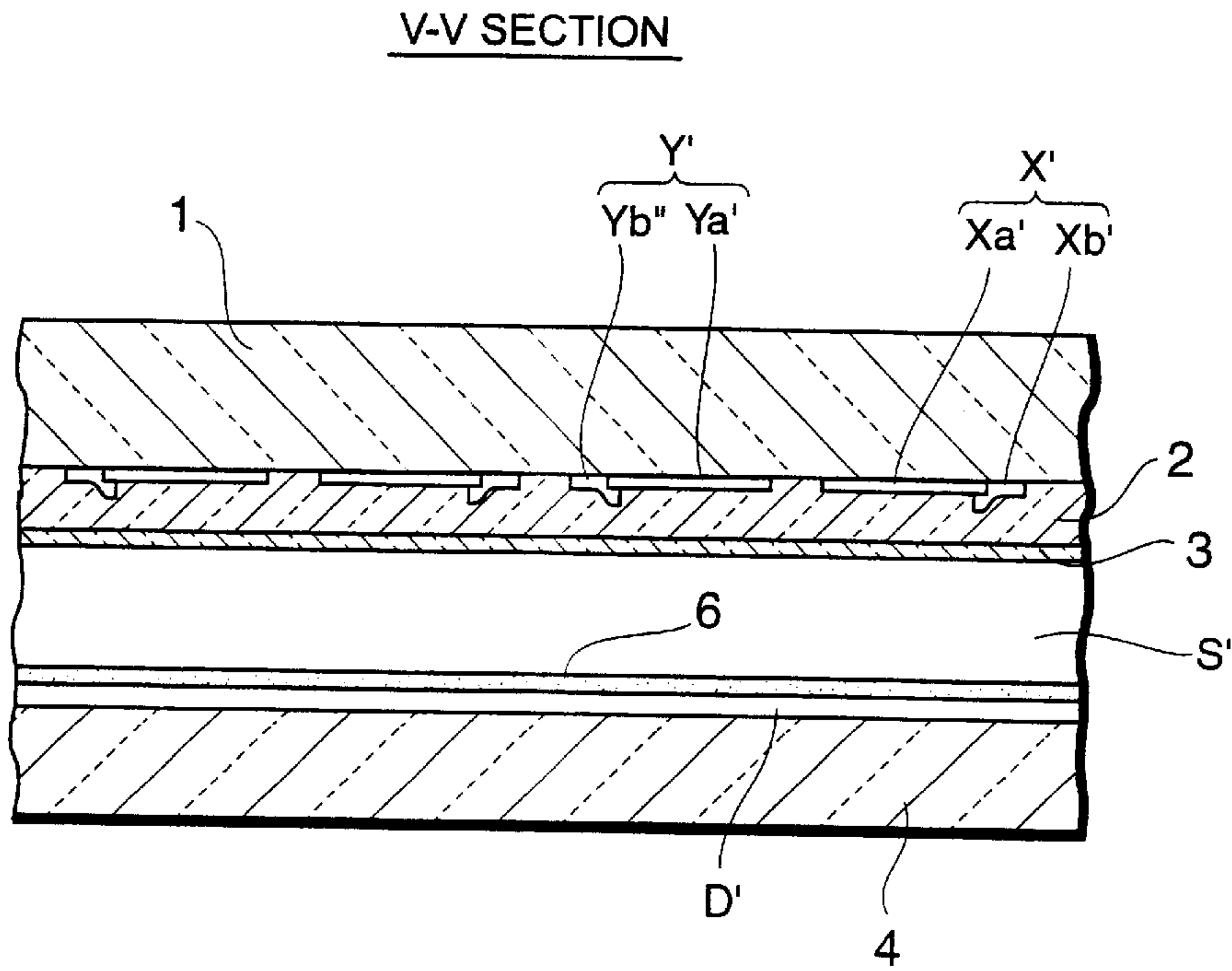
Fig.49 (PRIOR ART)
