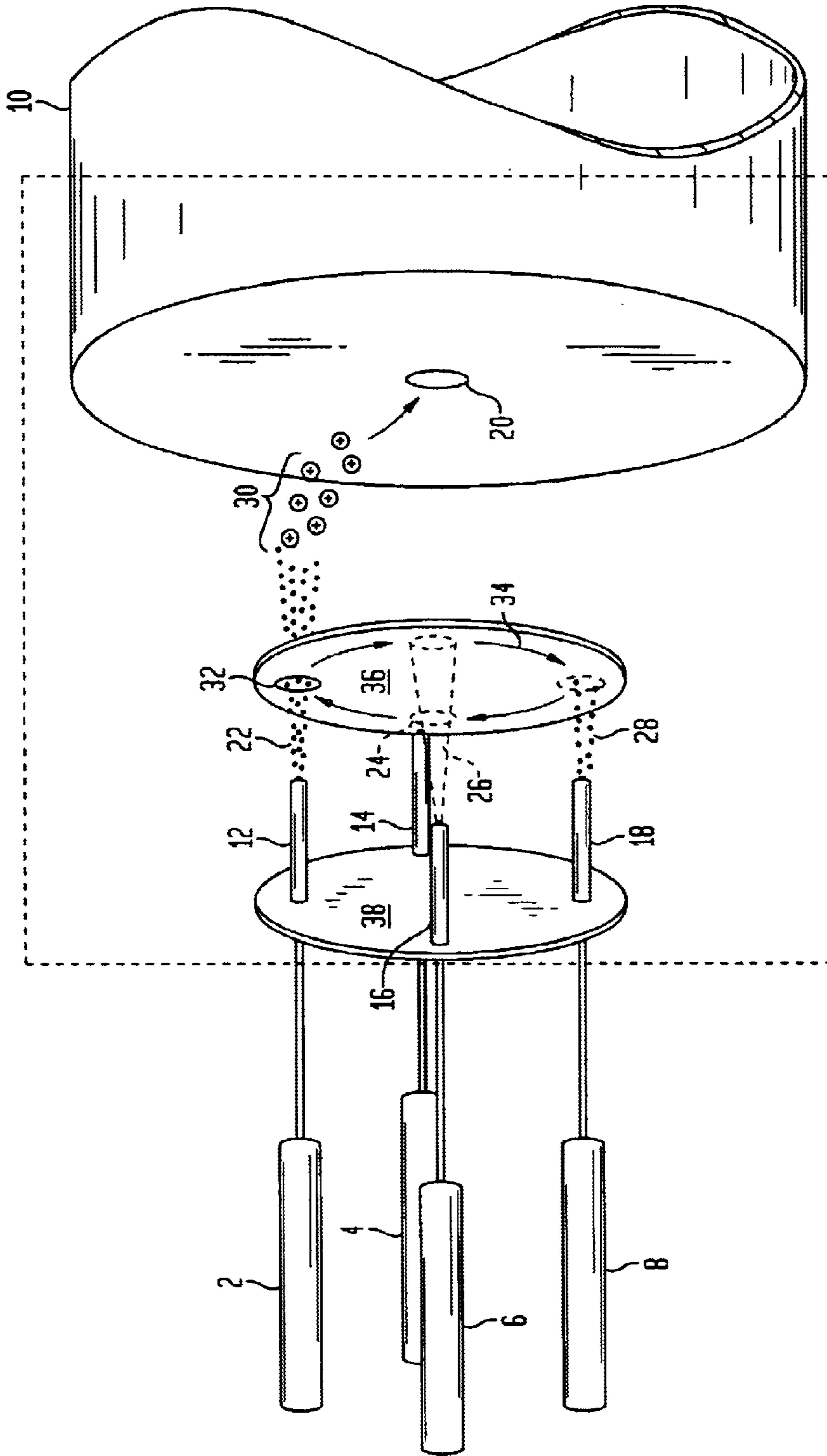
FIG. 1 (PRIOR ART)
