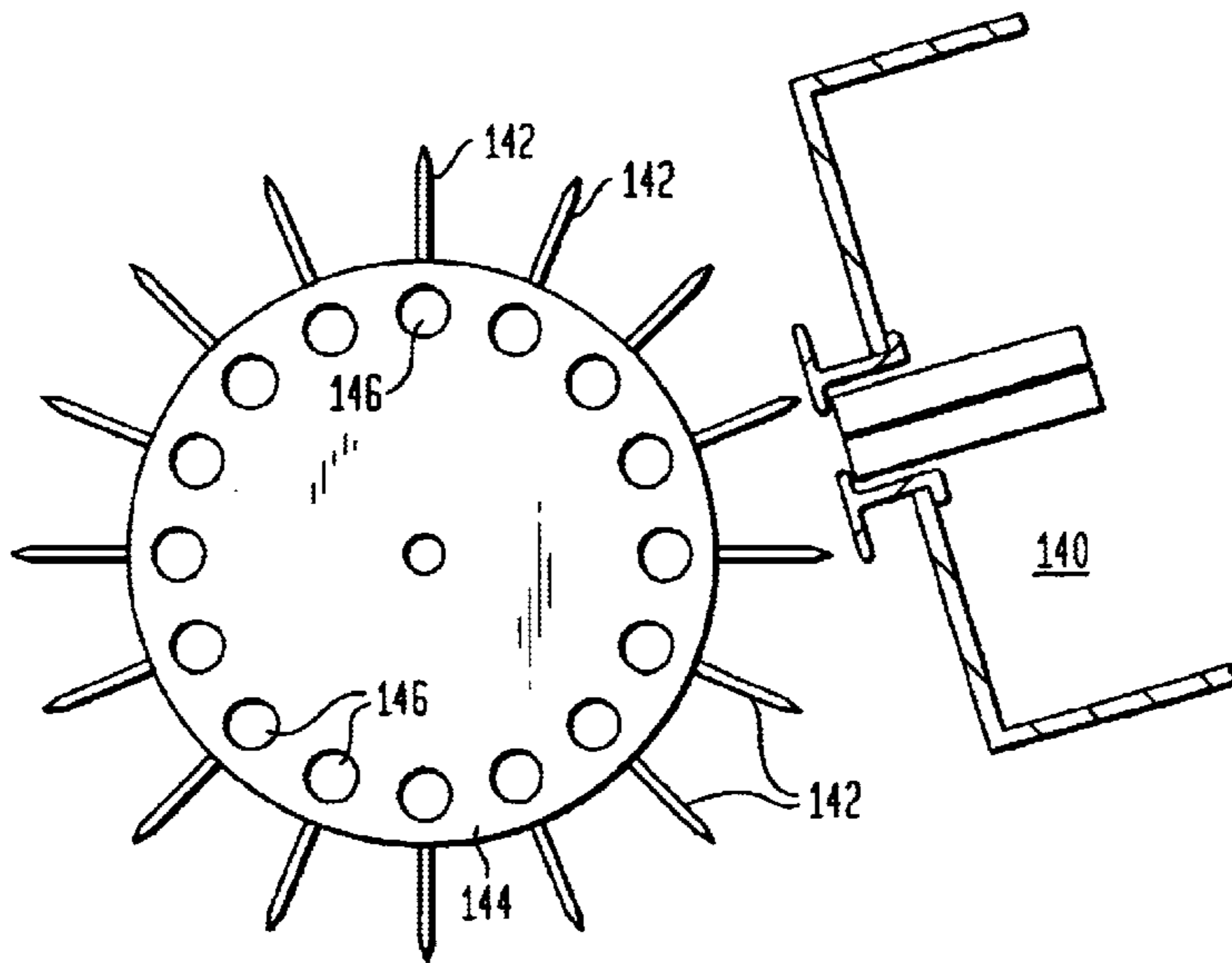
FIG. 5 (PRIOR ART)
