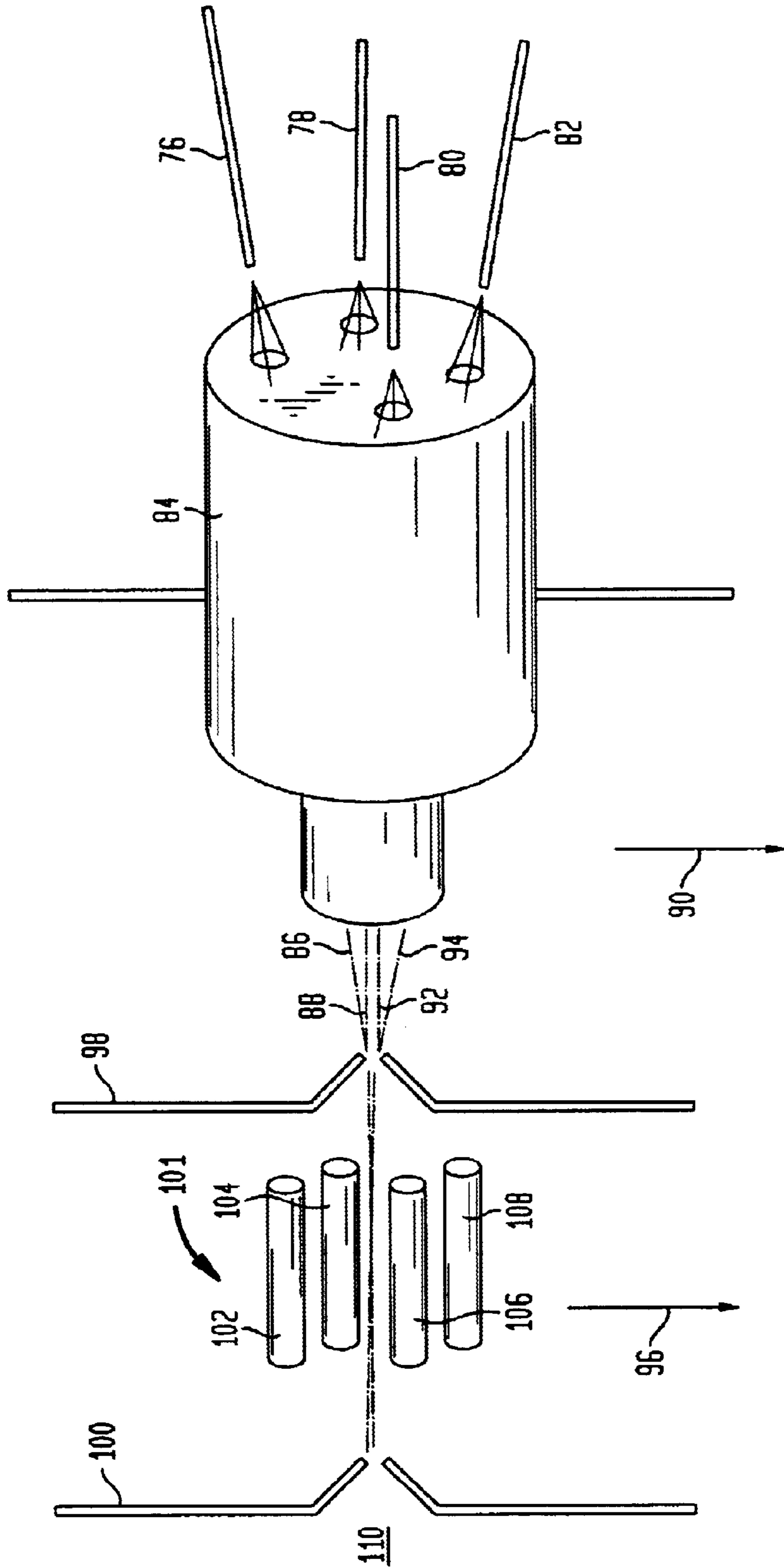
FIG. 3 (PRIOR ART)
