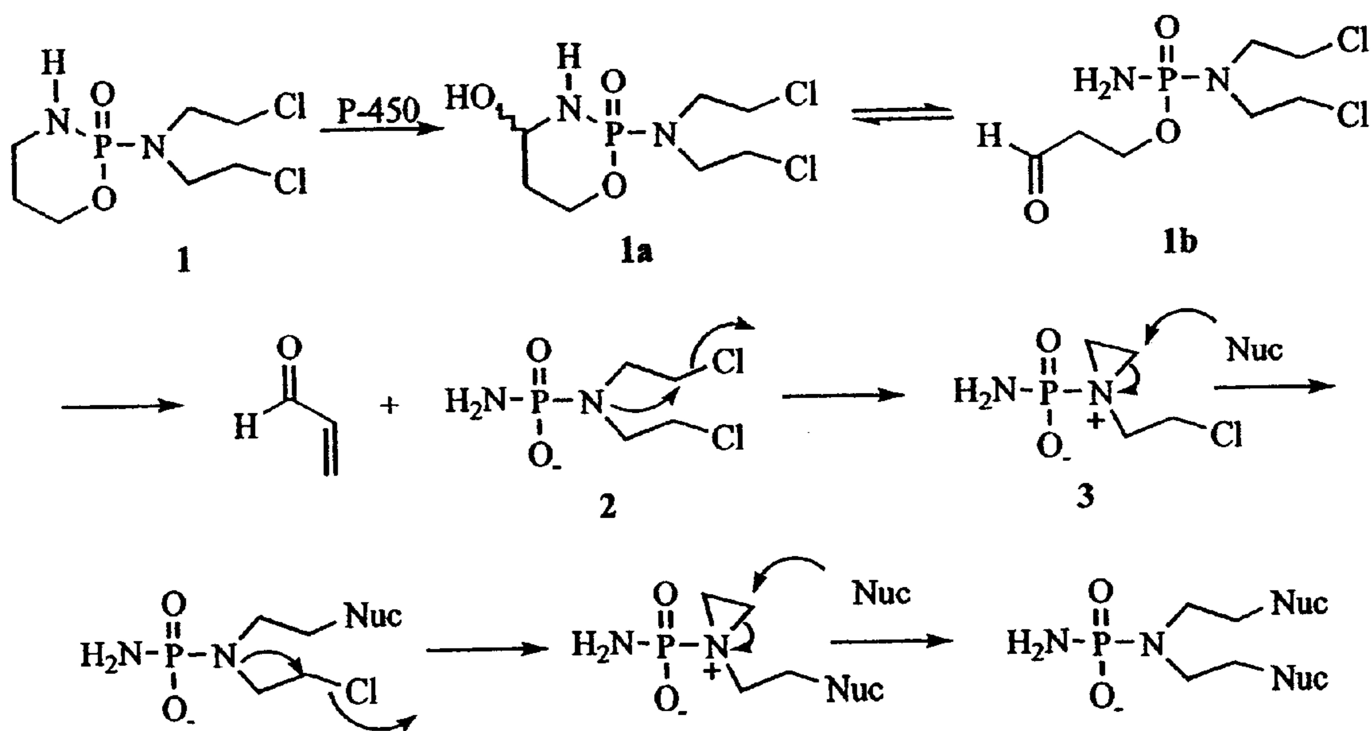
Scheme 1: Activation of cyclophosphamide and alkylation by phosphoramidate mustard 2
